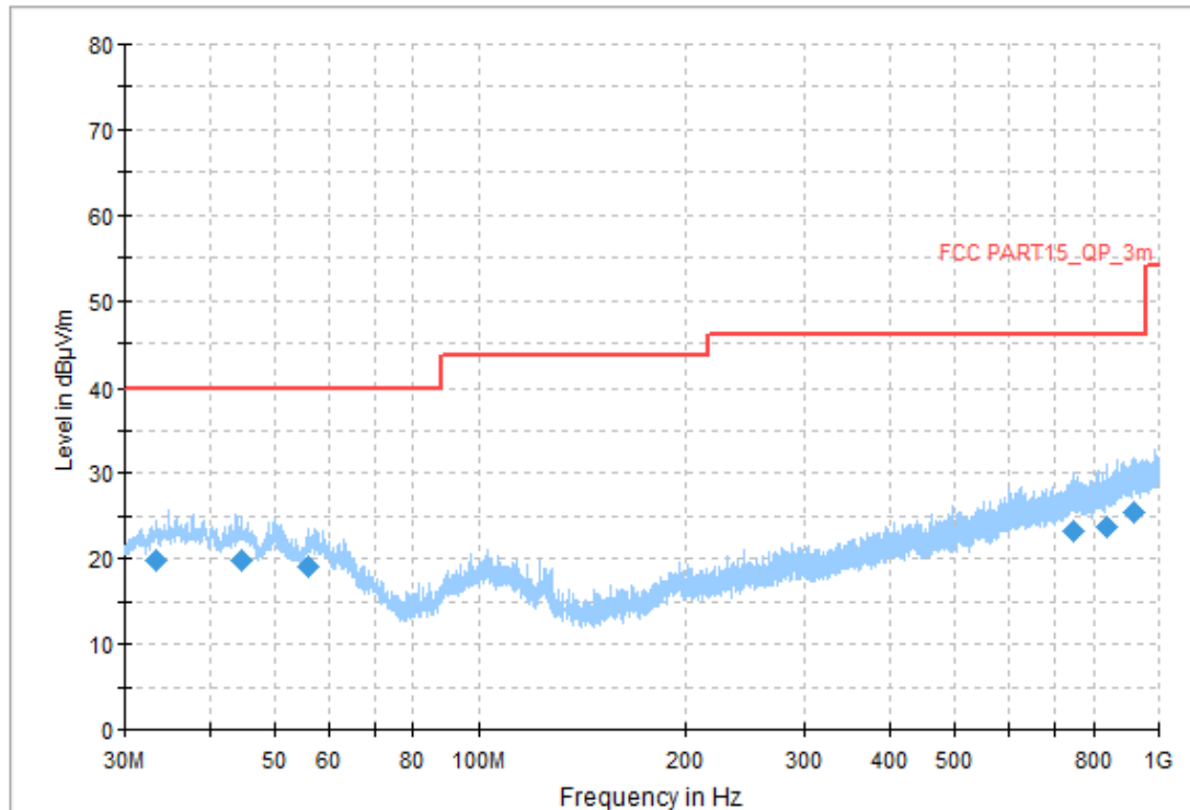
Figure A.1.1. Radiated Emission (GSM receiver 850MHz, 30MHz to 1GHz) Final_Result
