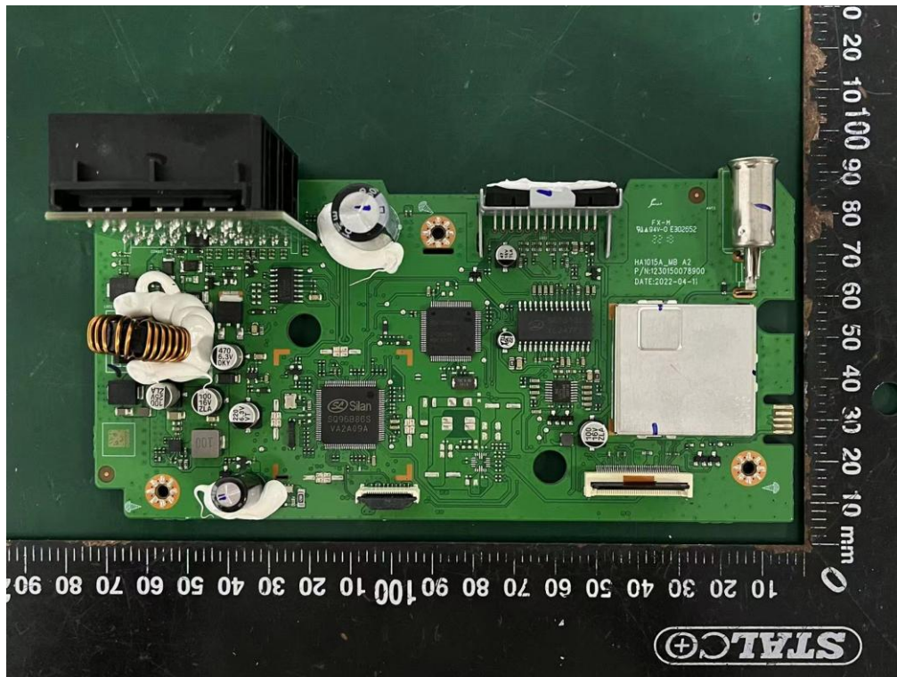
Internal photos M/N: ACR313UBA-IVE
