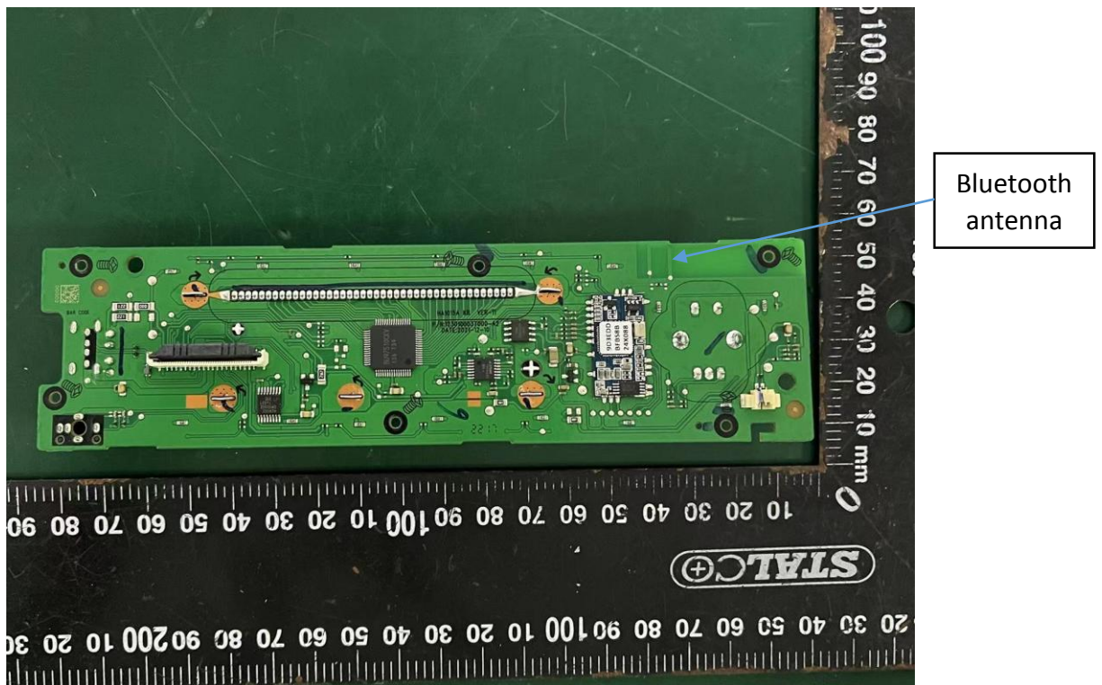
Internal photos M/N: ACR313UBA-IVE
