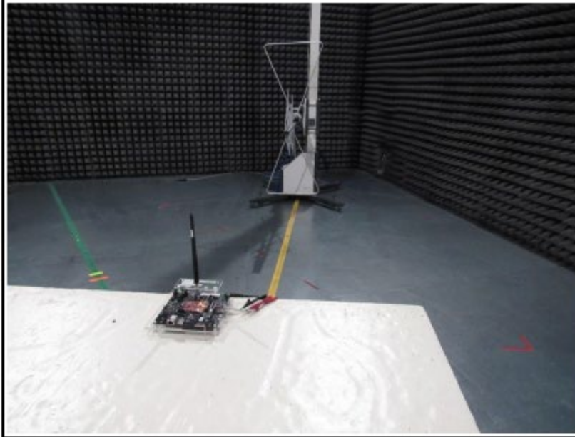
EUT Test Setup below 1 GH- Antenna 2
