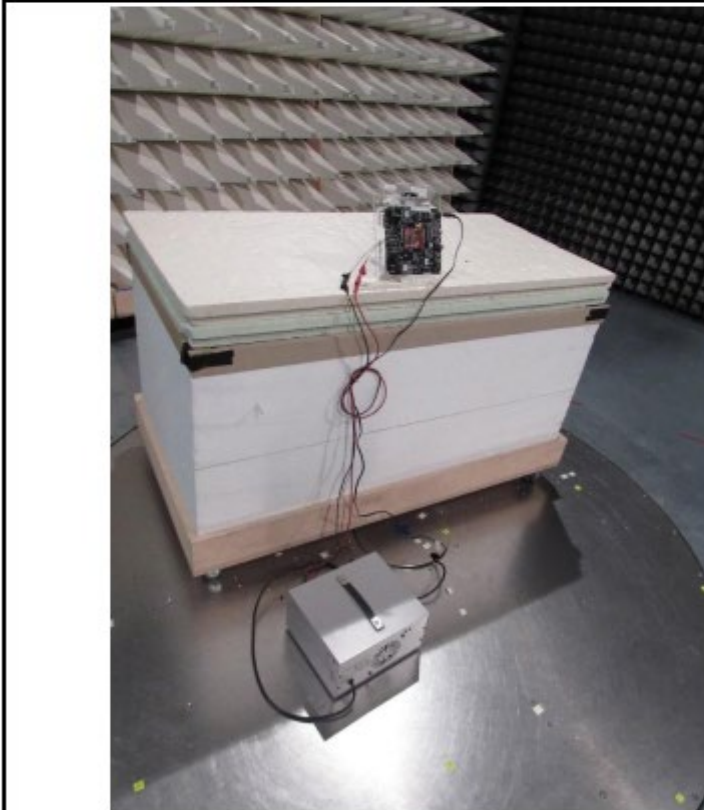
EUT Test Setup below 1 GH- Antenna 2
