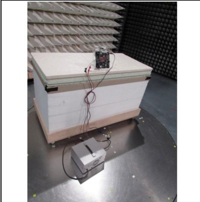
EUT Test Setup below 1 GH- Antenna 2
