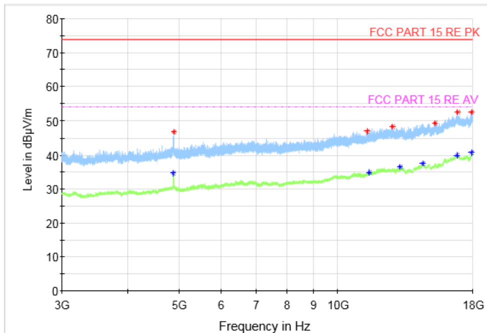
Fig.45 Radiated Spurious Emission (802.11g, CH6, 3 GHz-18 GHz)
