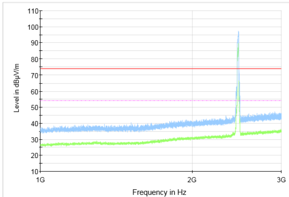
Fig.46 Radiated Spurious Emission (802.11g, CH11, 1 GHz-3 GHz)
