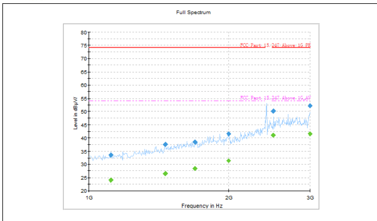
( \pi/4 -DQPSK_2402MHz, Antenna Vertical , 1GHz to 3GHz)
