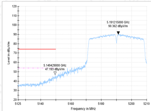
BANDEDGE-11AC(40M)-CH38-AV
