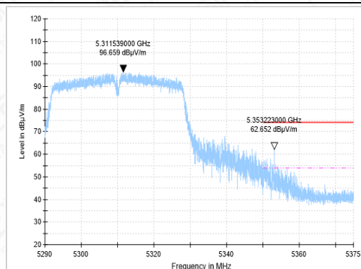
BANDEGE-11AC(40M)-CH62-PK
