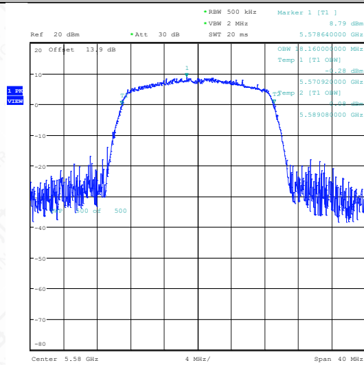
11AC20SISO-Ant1-5580
