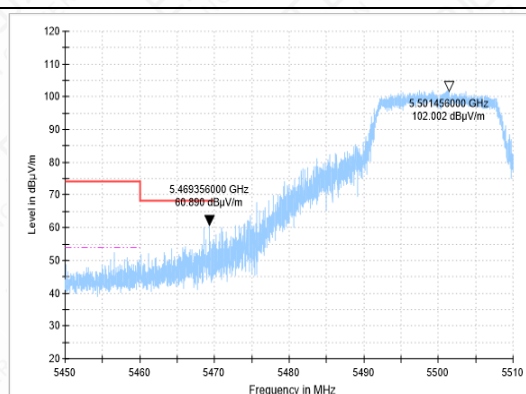
BANDEDGE-11A-CH100-PK
