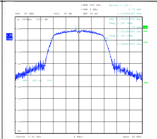
11A-Ant1-5320
