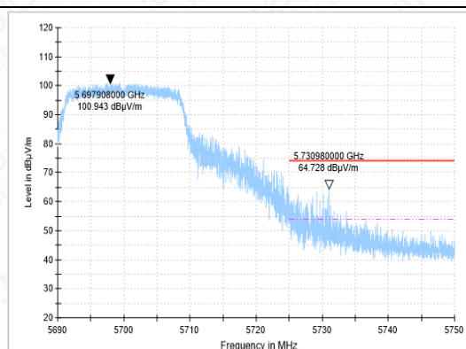
BANDEGE-11N-CH140-PK
