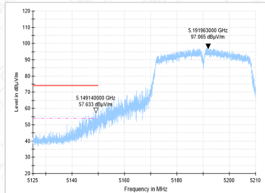
BANDEDGE-11AC(40M)-CH38-PK
