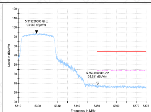
BANDEDGE-11A-CH64-AV
