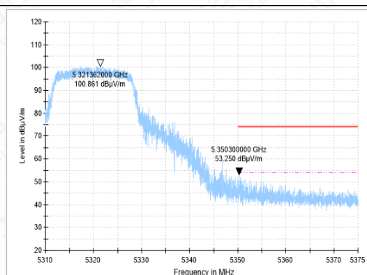
BANDEDGE-11A-CH64-PK
