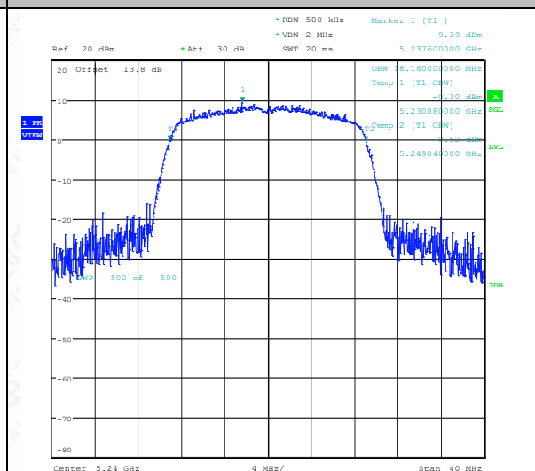
11AC20SISO-Ant1-5240
