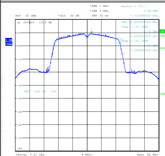
11N40SISO-Ant1-5510
