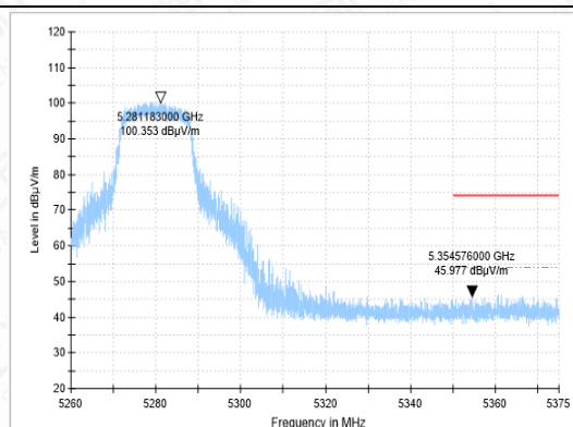
BANDEDGE-11A-CH56-PK
