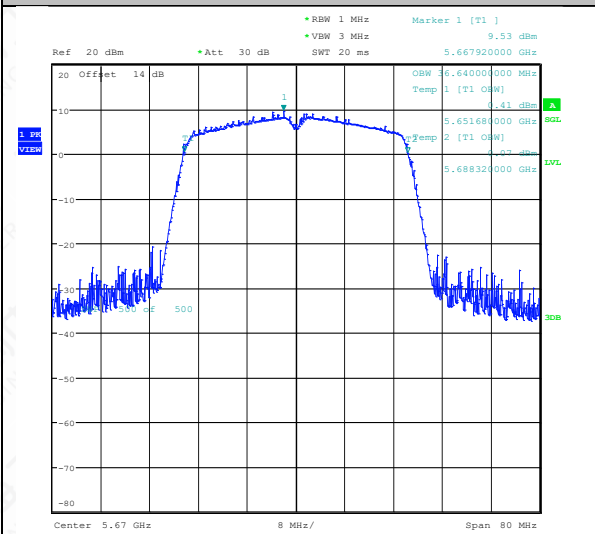
11AC40SISO-Ant1-5670
