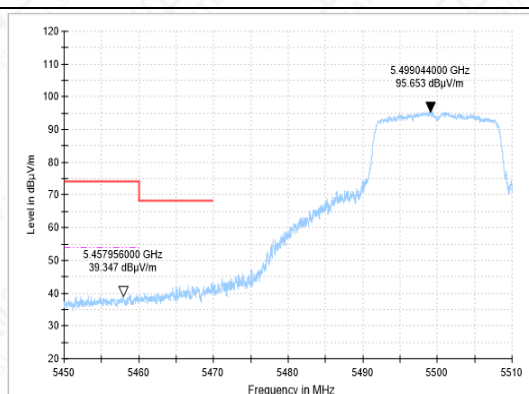
BANDEDGE-11A-CH100-AV
