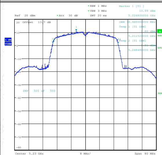
11N40SISO-Ant1-5230
