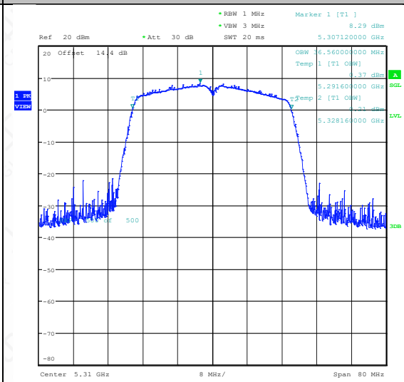
11AC40SISO-Ant1-5310
