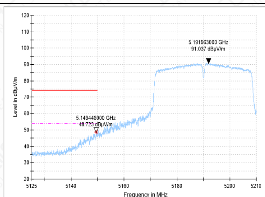
BANDEGE-11N(40M)-CH38-AV-16
