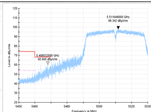
BANDEGE-11AC(40M)-CH102-PK-15
