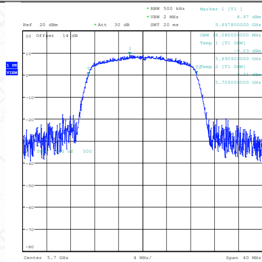
11AC20SISO-Ant1-5700
