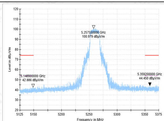
BANDEDGE-11A-CH52-PK
