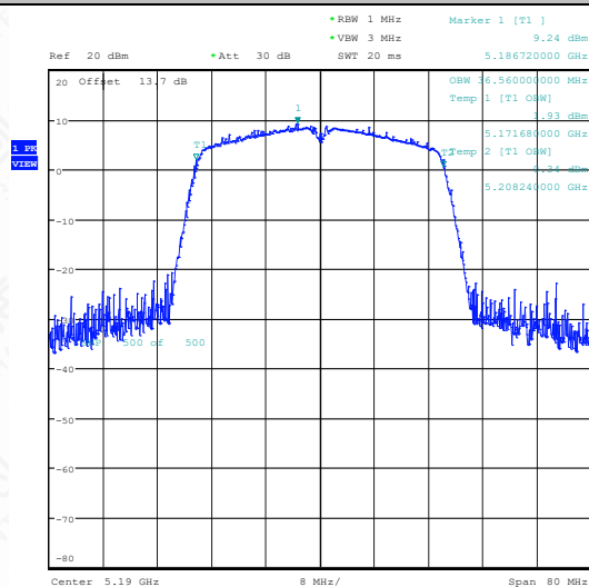
11AC40SISO-Ant1-5190
