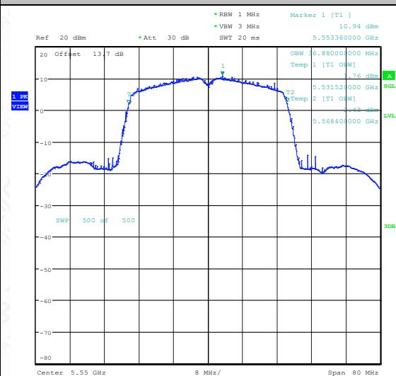
11N40SISO-Ant1-5550
