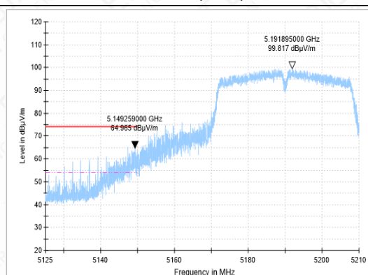
BANDEGE-11N(40M)-CH38-PK
