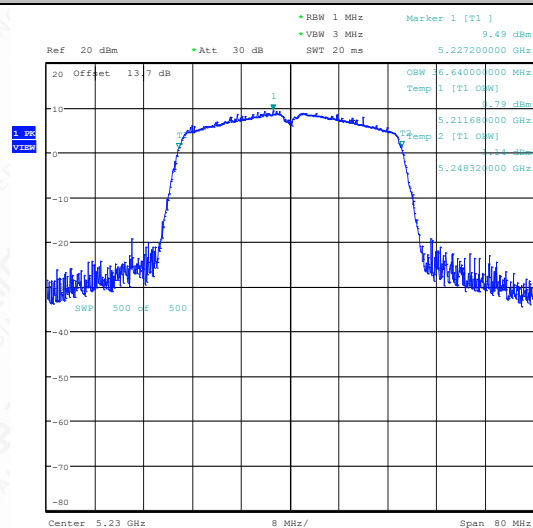
11AC40SISO-Ant1-5230
