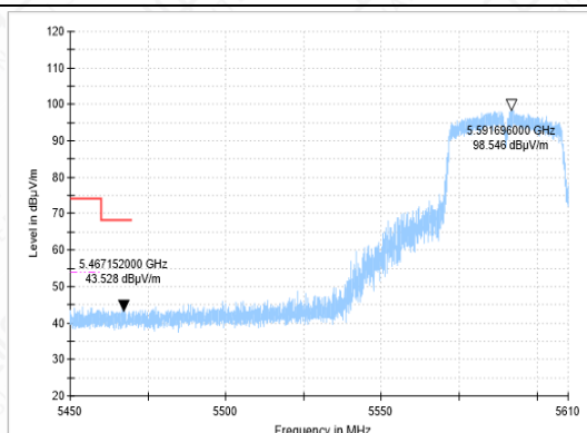
BANDEGE-11AC(40M)-CH118-PK
