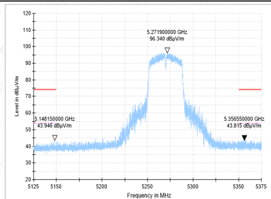
BANDEDGE-11AC(40M)-CH54-PK
