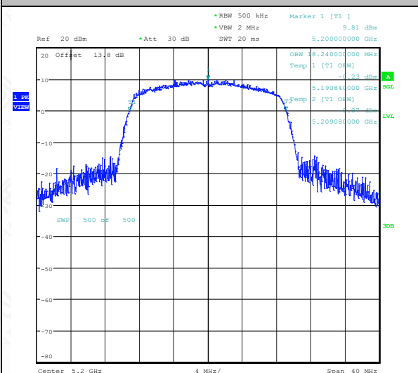
11AC20SISO-Ant1-5200
