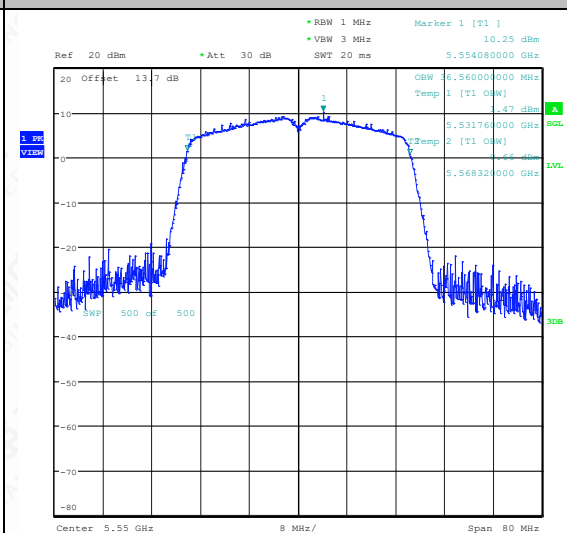
11AC40SISO-Ant1-5550
