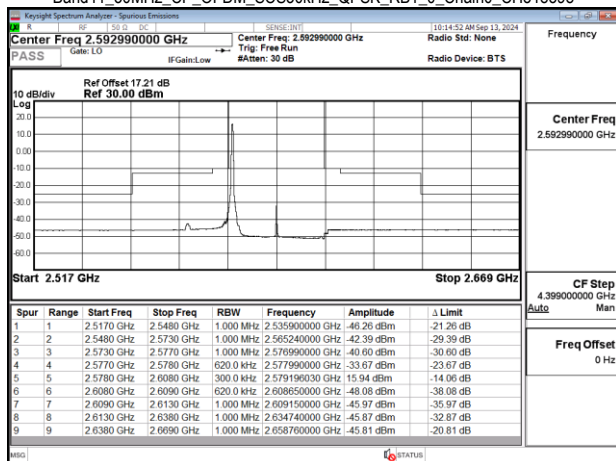
Band41_30MHz_CP_OFDM_SCS30kHz_QPSK_RB1_0_Chain0_CH518598
