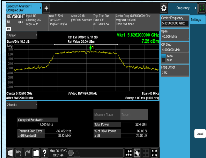
11AC20SISO-Ant2-5825
