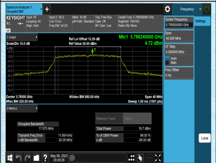
11AC20MIMO-Ant2-5785
