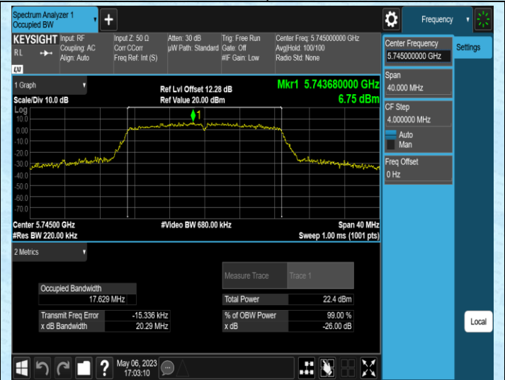
11AC20SISO-Ant1-5745
