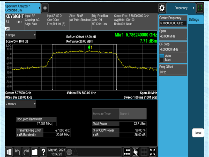
11N20SISO-Ant2-5785
