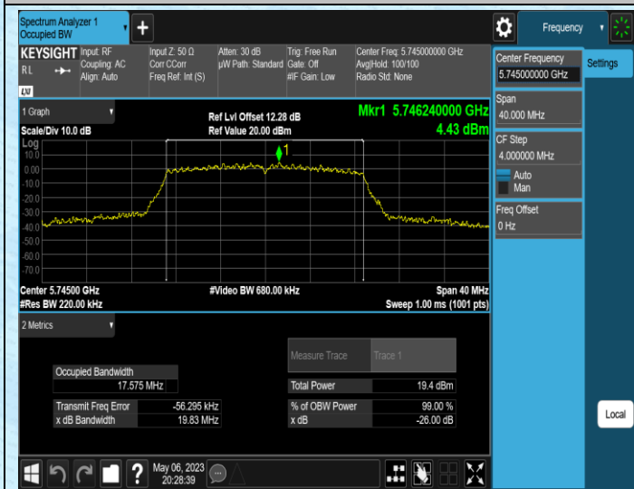
11AC20MIMO-Ant2-5745
