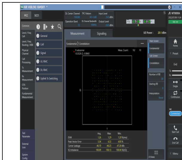
1-N13--15-10-M-5-DFT-256QAM-Outer_Full-50@0-A nt1-see graph-PASS
