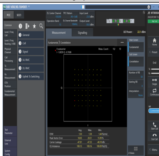
1-N13--15-10-M-4-DFT-64QAM-Outer_Full-50@0-A nt1-see graph-PASS
