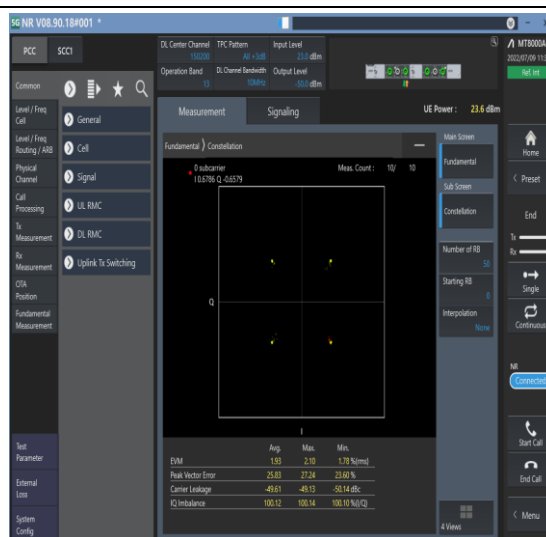
1-N13--15-10-M-2-DFT-QPSK-Outer_Full-50@0-Ant 1-see graph-PASS
