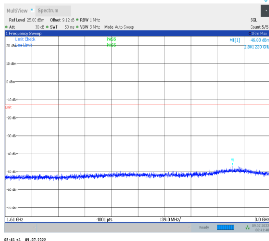
1-N13--15-10-M-1-DFT-PI2BPSK-Inner_1RB_Left-1 @1-1610-3000-Ant1--46.80--13-PASS
