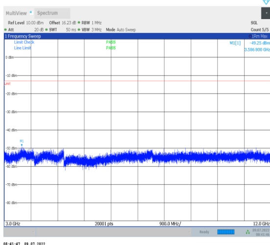
1-N13--15-10-M-1-DFT-PI2BPSK-Inner_1RB_Left-1 @1-3000-12000-Ant1--49.25--13-PASS
