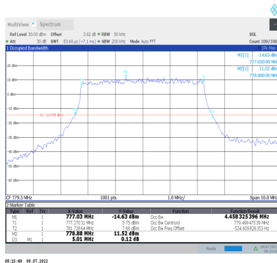
1-N13--15-5-L-4-DFT-64QAM-Outer_Full-25@0-Ant 1-4.458-5.010-≤5-PASS
