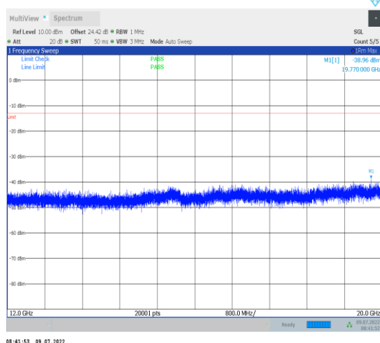
1-N13--15-10-M-1-DFT-PI2BPSK-Inner_1RB_Left-1 @1-12000-20000-Ant1--38.96--13-PASS
