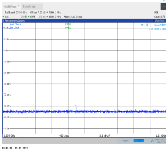
1-N13--15-10-M-1-DFT-PI2BPSK-Inner_1RB_Left-1 @1-1559-1610-Ant1--52.72--40-PASS
