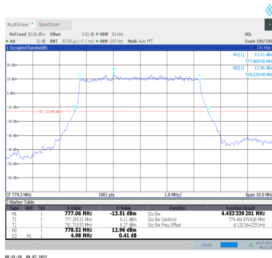
1-N13--15-5-L-2-DFT-PI2BPSK-Outer_Full-25@0-An t1-4.453-4.980-≤5-PASS
