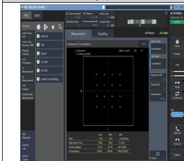
1-N13--15-10-M-7-CP-16QAM-Outer_Full-52@0-Ant1 -see graph-PASS
