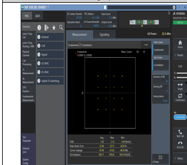
1-N13--15-10-M-3-DFT-16QAM-Outer_Full-50@0-Ant 1-see graph-PASS
