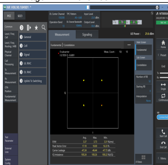
1-N13--15-10-M-6-CP-QPSK-Outer_Full-52@0-Ant 1-see graph-PASS
