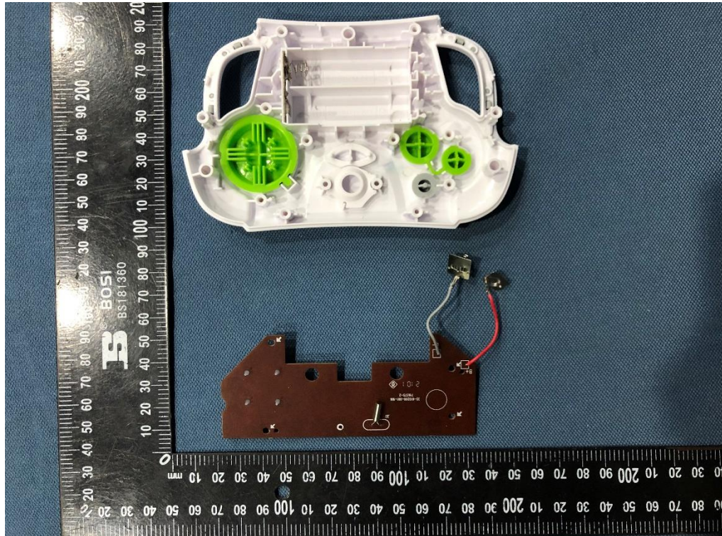
Internal View
