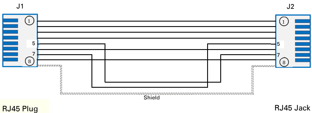
Figure 25 CMM4 power adapter cabling diagram
