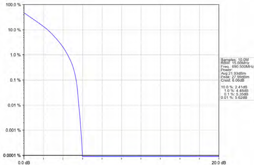
Band71_15MHz_QPSK_HCH_690.5MHz_RB_75_0_NTNV
