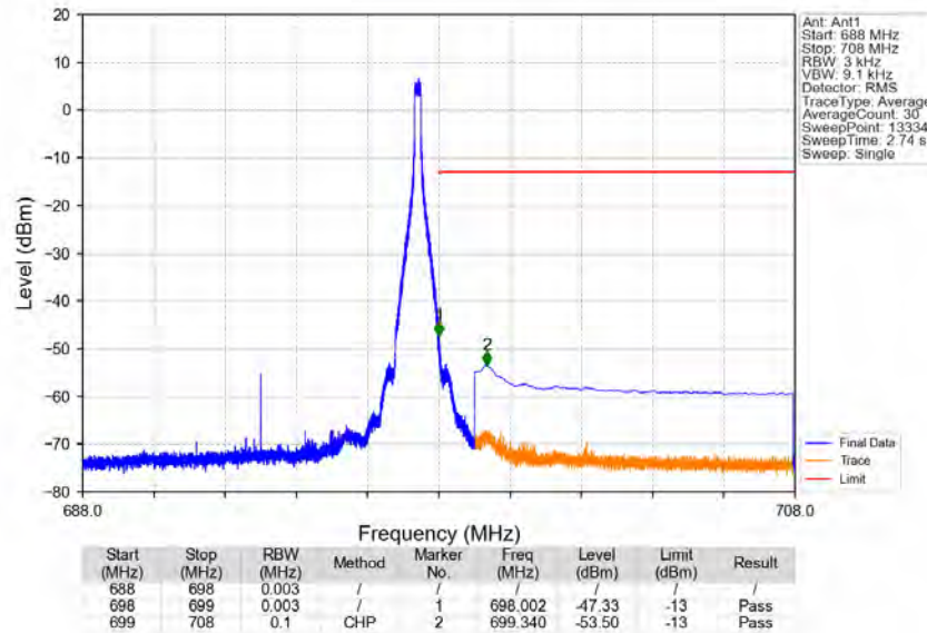
Band71_10MHz_16QAM_HCH_693MHz_RB_1_49_NTNV
