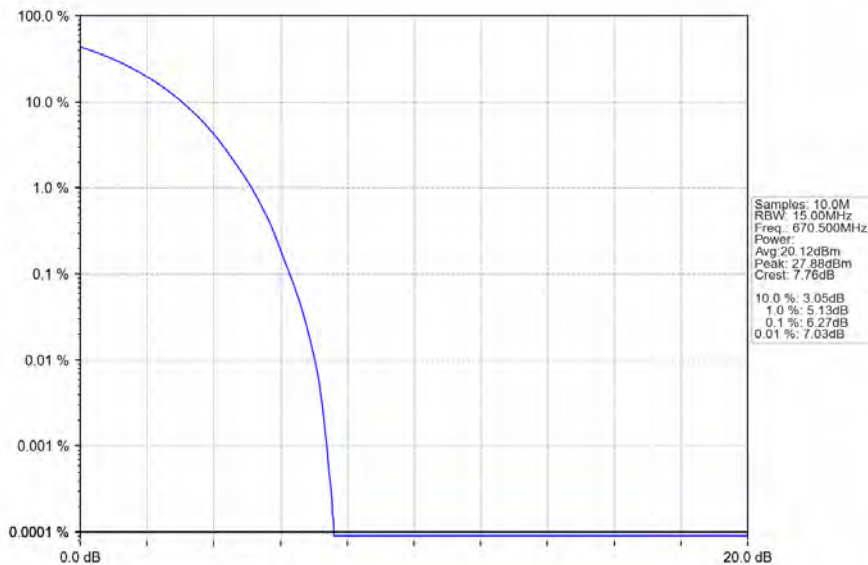
Band71_15MHz_64QAM_LCH_670.5MHz_RB_75_0_NTNV
