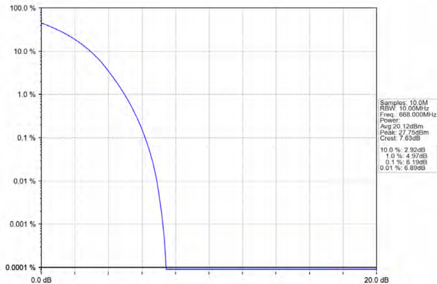
Band71_10MHz_64QAM_LCH_668MHz_RB_50_0_NTNV
