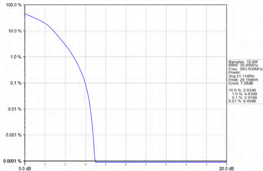
Band71_20MHz_16QAM_MCH_683MHz_RB_100_0_NTNV
