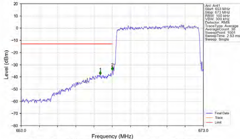
Band71_10MHz_64QAM_LCH_668MHz_RB_50_0_NTNV
