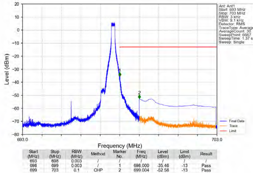
Band71_5MHz_16QAM_HCH_695.5MHz_RB_1_24_NTNV
