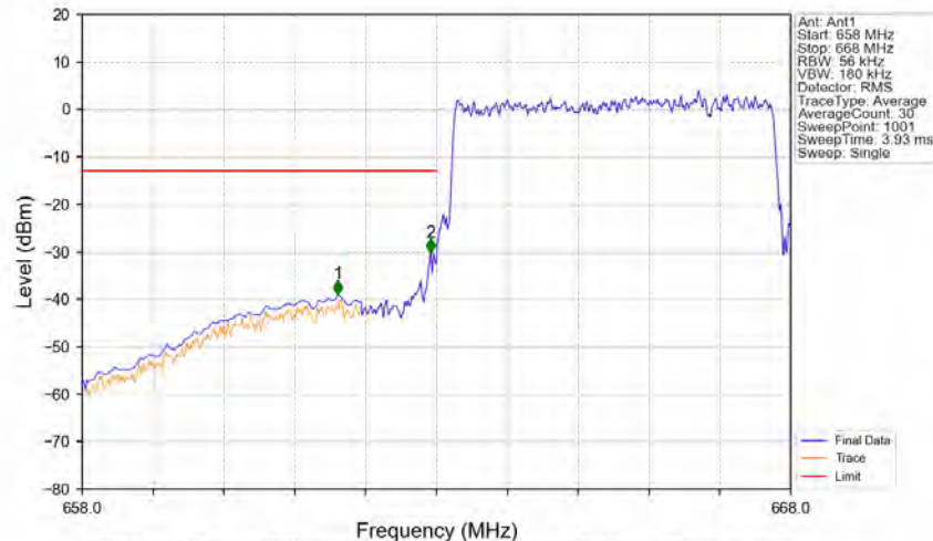
Band71_5MHz_64QAM_LCH_665.5MHz_RB_25_0_NTNV
