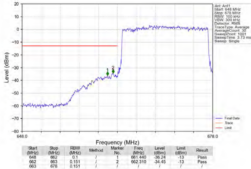
Band71_15MHz_QPSK_LCH_670.5MHz_RB_75_0_NTNV
