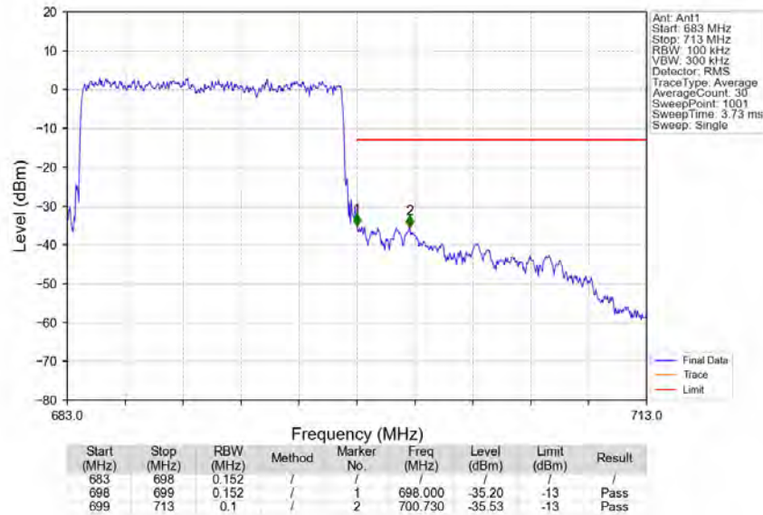
Band71_15MHz_QPSK_HCH_690.5MHz_RB_75_0_NTNV
