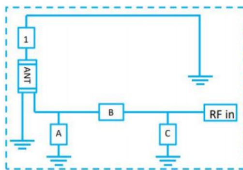
3216 Chip Antenna
