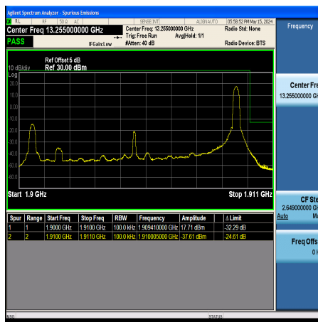
Band2_10MHz_16QAM_19150_1RB#49
