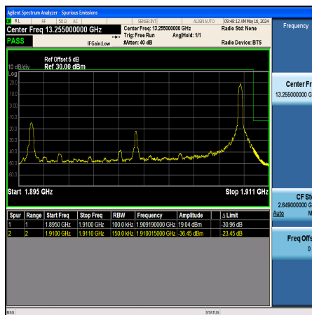
Band2_15MHz_QPSK_19125_1RB#74
