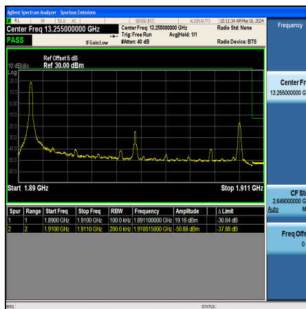
Band2_20MHz_QPSK_19100_1RB#0
