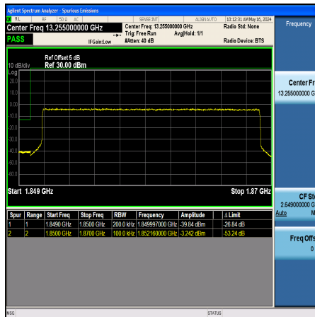
Band2_20MHz_QPSK_18700_100RB#0
