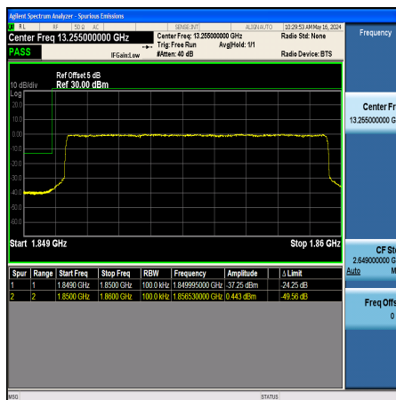
Band2_10MHz_QPSK_18650_50RB#0
