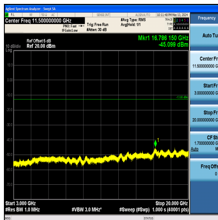
Band2_3MHz_QPSK_18900_1RB#0_3000~20000_3000~20000
