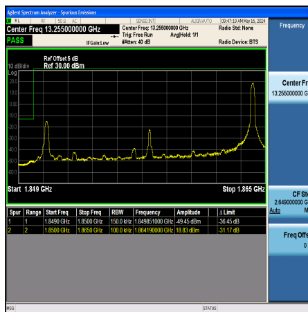
Band2_15MHz_QPSK_18675_1RB#74
