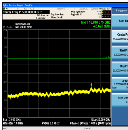
Band2_1.4MHz_QPSK_18900_1RB#0_3000~20000_3000~20000
