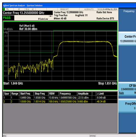
Band2_1.4MHz_QPSK_18607_6RB#0
