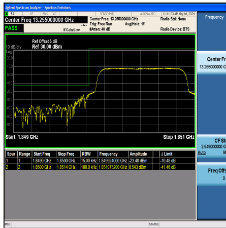
Band2_1.4MHz_16QAM_18607_6RB#0
