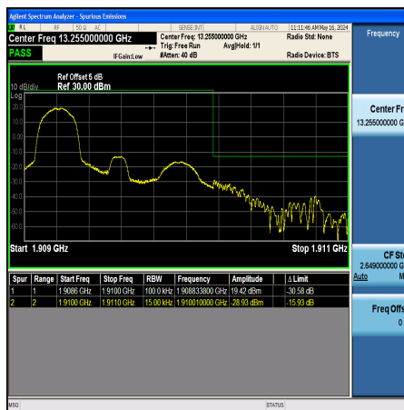
Band2_1.4MHz_QPSK_19193_1RB#0
