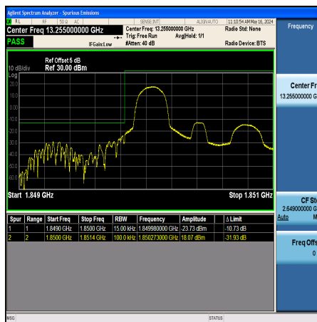
Band2_1.4MHz_16QAM_18607_1RB#0
