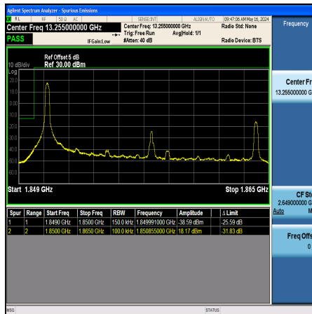
Band2_15MHz_16QAM_18675_1RB#0
