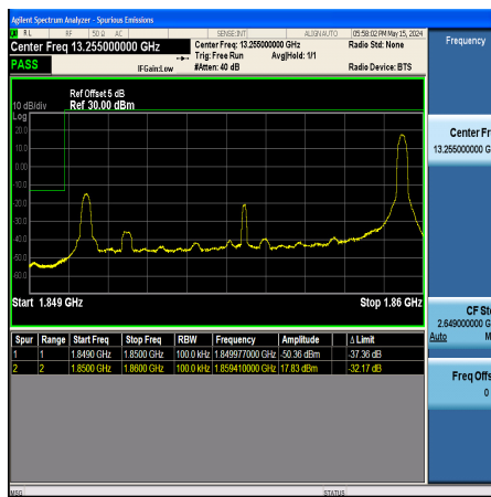
Band2_10MHz_16QAM_18650_1RB#49
