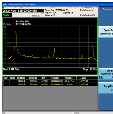
Band2_20MHz_16QAM_18700_1RB#0
