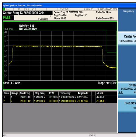
Band2_10MHz_QPSK_19150_50RB#0
