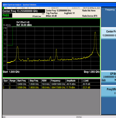
Band2_15MHz_16QAM_18675_1RB#74
