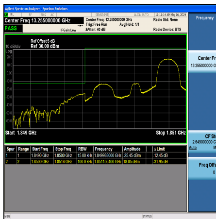
Band2_1.4MHz_16QAM_18607_1RB#5
