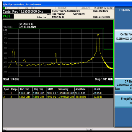
Band2_10MHz_QPSK_19150_1RB#49
