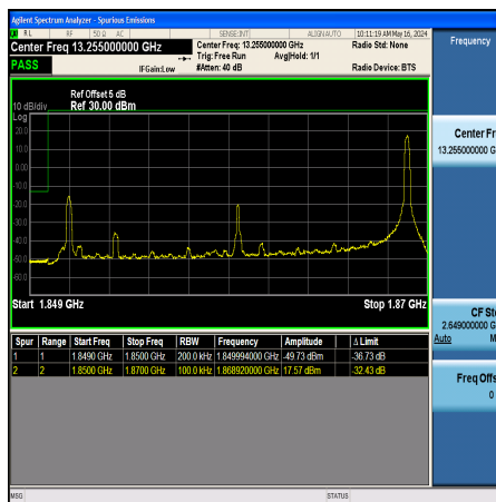
Band2_20MHz_16QAM_18700_1RB#99
