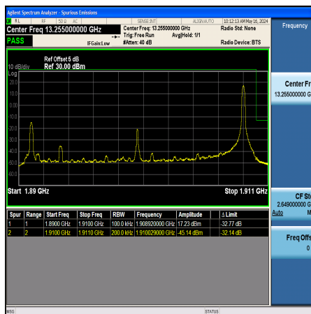
Band2_20MHz_16QAM_19100_1RB#99
