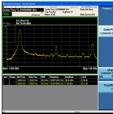
Band2_10MHz_16QAM_18650_1RB#0
