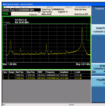
Band2_20MHz_QPSK_19100_1RB#99
