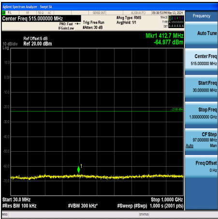
Band2_1.4MHz_QPSK_18607_1RB#0_30~1000_30~1000
