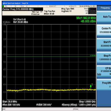
Band2_1.4MHz_QPSK_18900_1RB#0_30~1000_30~1000
