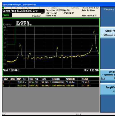
Band2_10MHz_QPSK_18650_1RB#49
