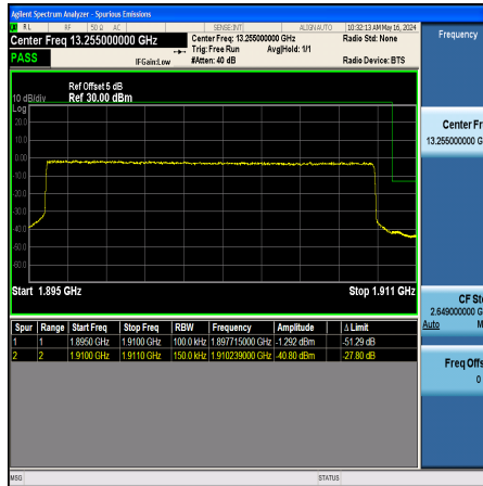
Band2_15MHz_QPSK_19125_75RB#0
