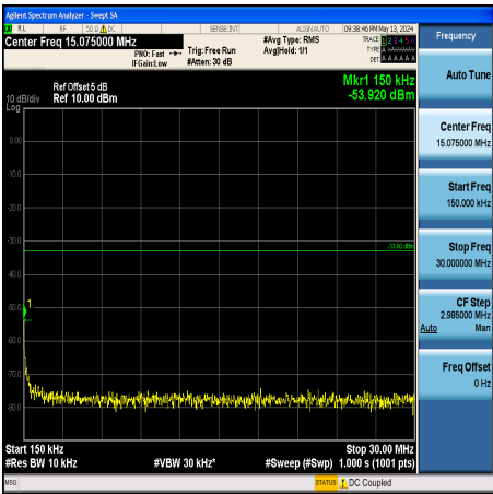
Band2_1.4MHz_QPSK_18607_1RB#0_0.15~30_0.15~30
