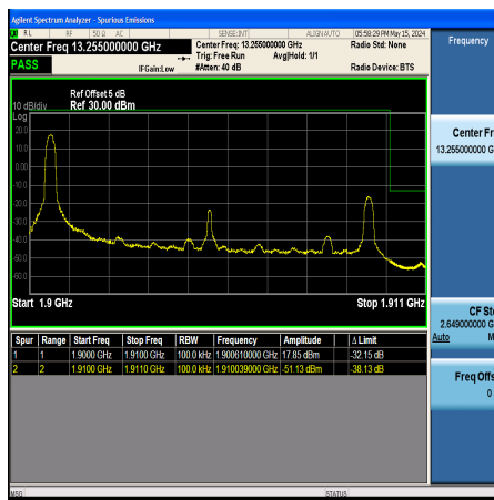
Band2_10MHz_16QAM_19150_1RB#0
