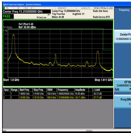
Band2_10MHz_QPSK_19150_1RB#0
