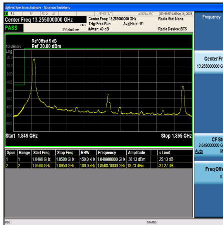
Band2_15MHz_QPSK_18675_1RB#0
