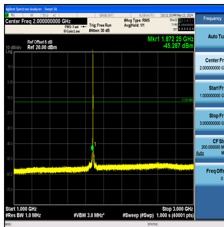
Band2_3MHz_QPSK_18900_1RB#0_1000~3000_1000~3000
