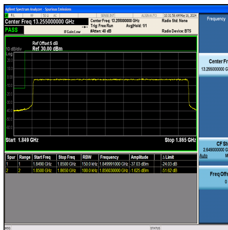
Band2_15MHz_QPSK_18675_75RB#0
