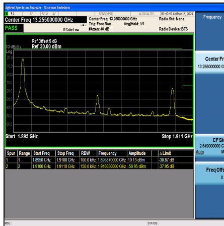
Band2_15MHz_QPSK_19125_1RB#0
