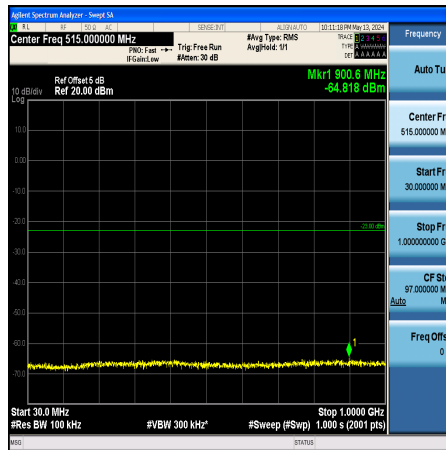
Band2_3MHz_QPSK_18900_1RB#0_30~1000_30~1000
