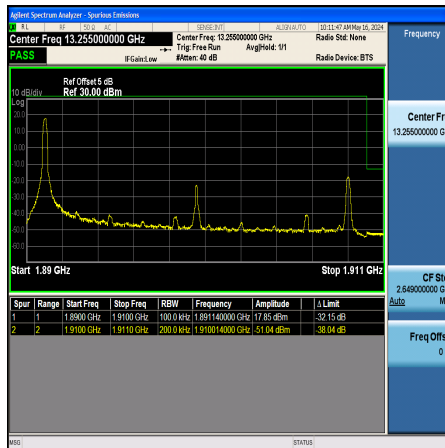
Band2_20MHz_16QAM_19100_1RB#0
