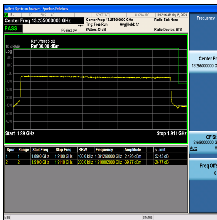
Band2_20MHz_QPSK_19100_100RB#0
