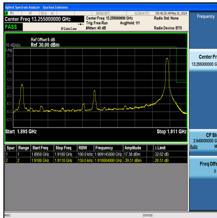
Band2_15MHz_16QAM_19125_1RB#74
