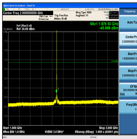
Band2_1.4MHz_QPSK_18900_1RB#0_1000~3000_1000~3000
