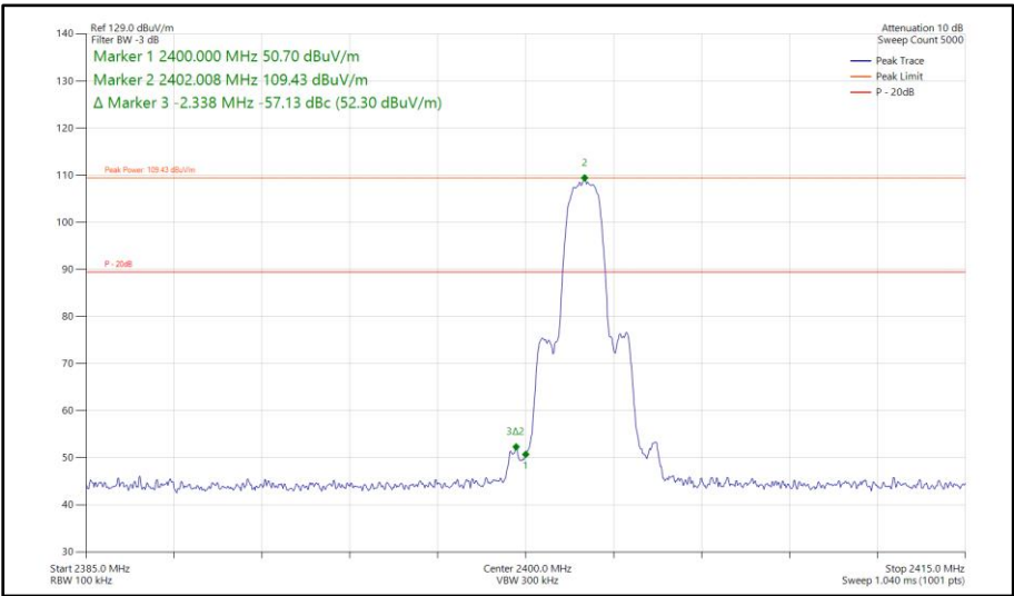
Figure 233 - Bluetooth 2-DH5, MIMO, Core 0 - Core 1 - 2402 MHz Band Edge Frequency 2400 MHz
