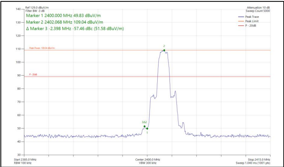
Figure 234 - Bluetooth 3-DH5, MIMO, Core 0 - Core 1 - 2402 MHz Band Edge Frequency 2400 MHz
