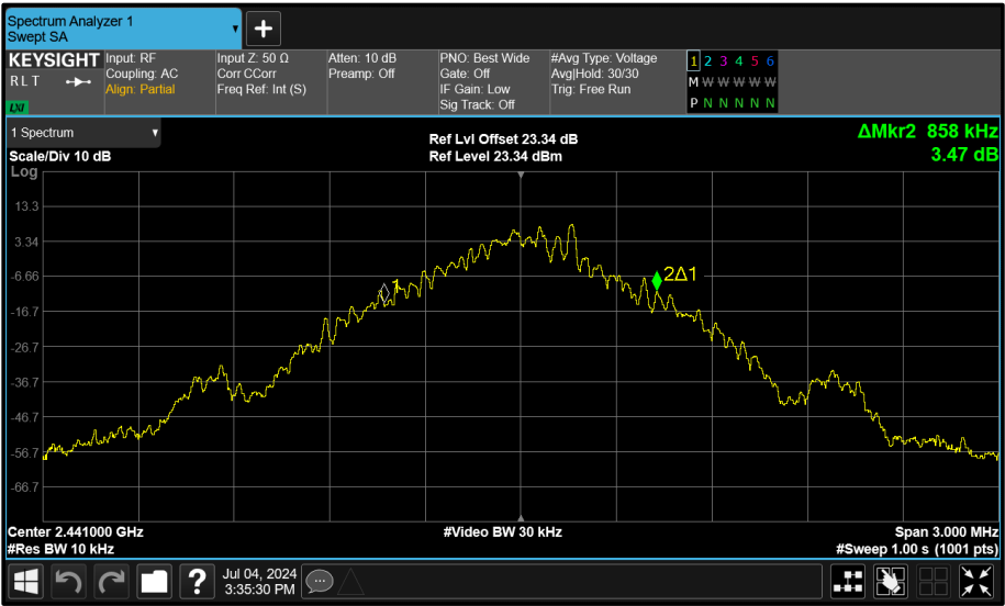
Figure 183 - Core 0 (A) 2441 MHz (CH39) 99% Bandwidth
