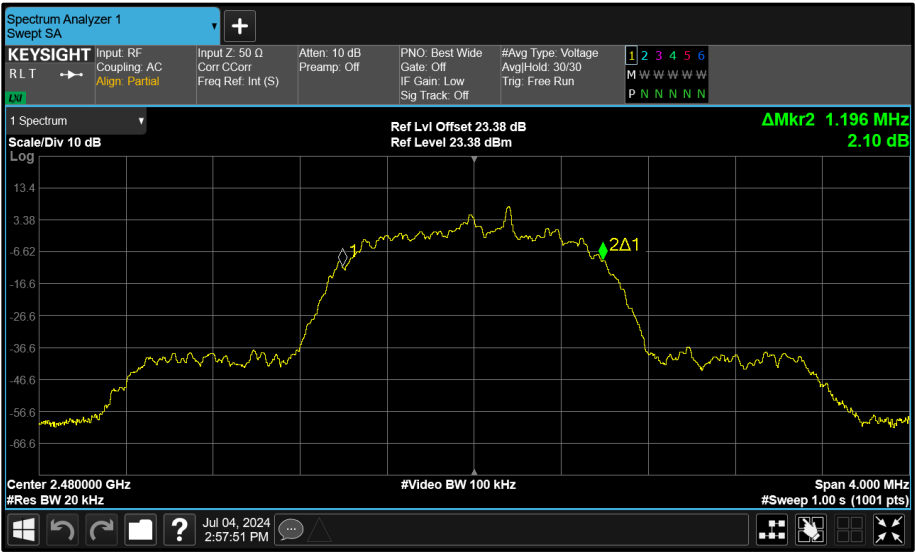
Figure 175 - Core 0 (A) 2480 MHz (CH78) 99% Bandwidth
