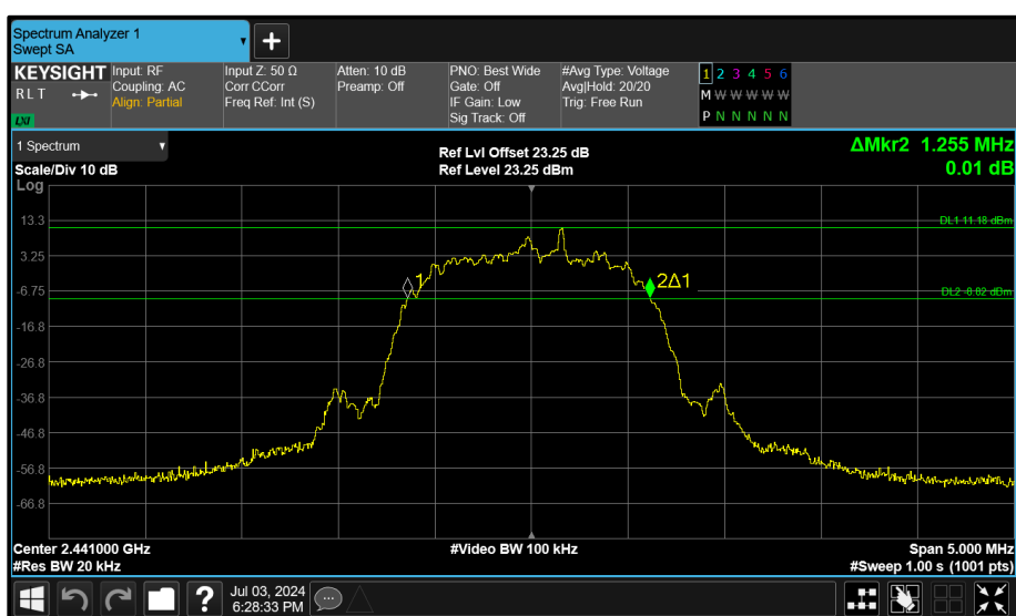
Figure 208 - Core 1 (B) 2441 MHz (CH39) 20 dB Bandwidth
