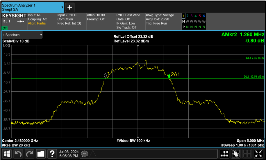
Figure 176 - Core 1 (B) 2480 MHz (CH78) 20 dB Bandwidth
