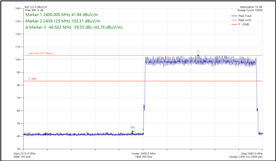
Figure 231 - Bluetooth 3-DH5, SISO, Core 2 - Hopping Band Edge Frequency 2400 MHz
