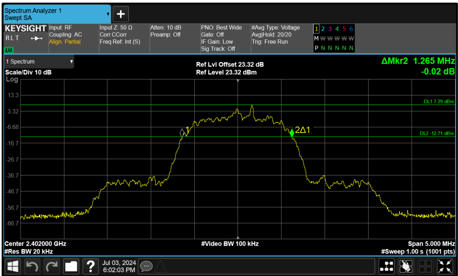
Figure 166 - Core 0 (A) 2402 MHz (CH0) 20 dB Bandwidth
