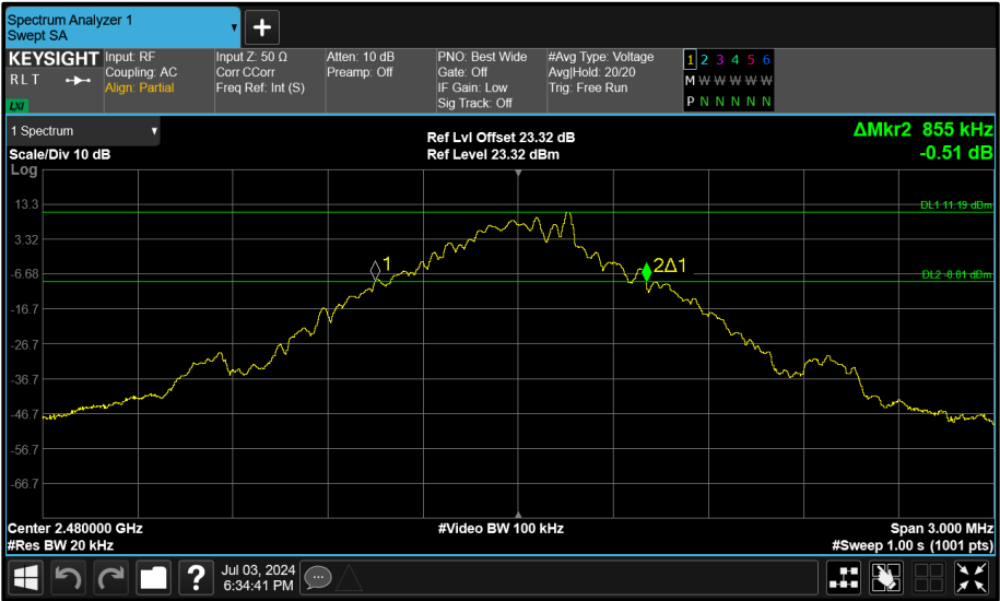
Figure 188 - Core 1 (B) 2480 MHz (CH78) 20 dB Bandwidth
