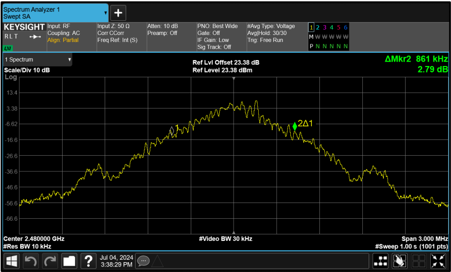
Figure 187 - Core 0 (A) 2480 MHz (CH78) 99% Bandwidth
