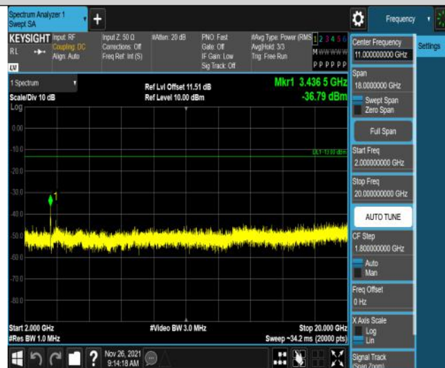
Band4-15MHz-16QAM-20025-75RB#0-Range3:2000~20000MHz
