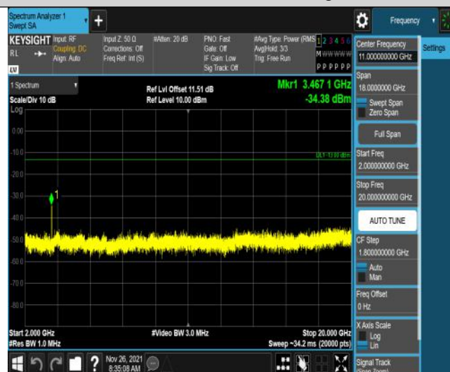
Band4-5MHz-16QAM-20175-25RB#0-Range3:2000~20000MHz
