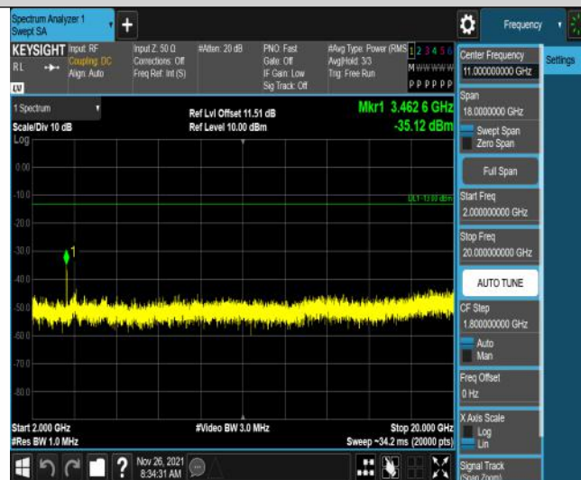
Band4-5MHz-QPSK-20175-25RB#0-Range3:2000~20000MHz
