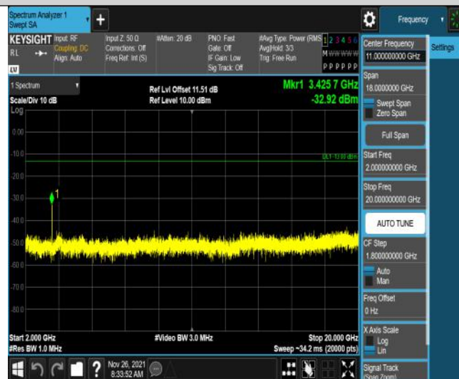
Band4-5MHz-16QAM-19975-25RB#0-Range3:2000~20000MHz
