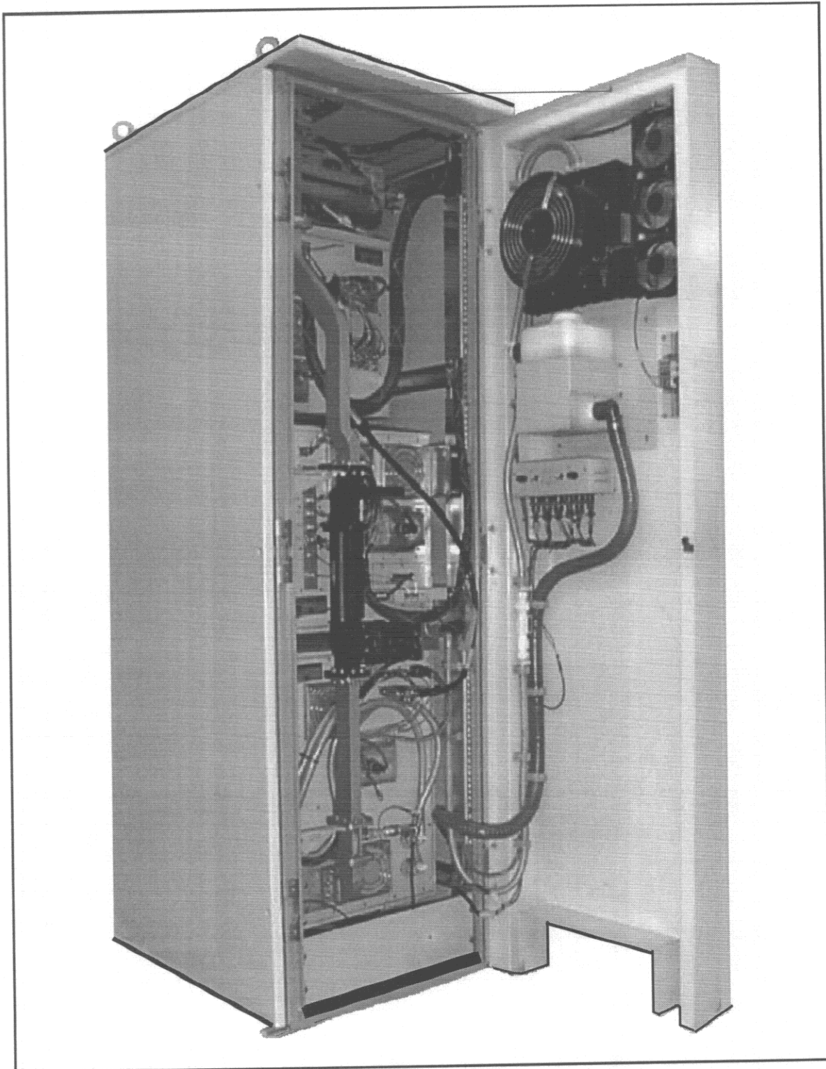
Figure 5. Transmitter Cabinet (maintenance condition).
