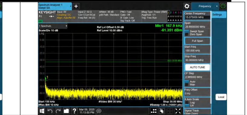
Band4-1513-1-0.15~30MHz-PASS
