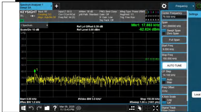
Band4-1513-1-0.009~0.15MHz-PASS
