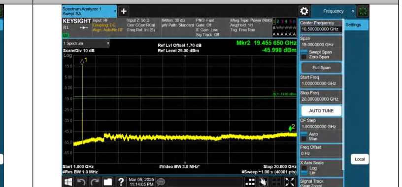
Band4-1513-1-1000~20000MHz-PASS
