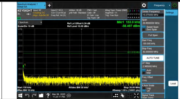
Band4-1513-5-0.15~30MHz-PASS
