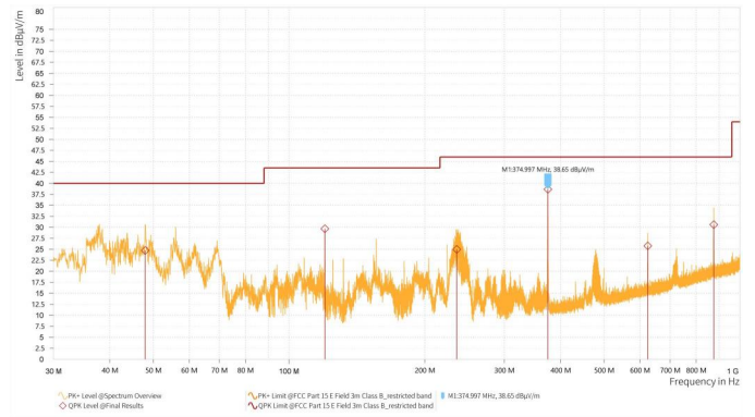
BT_DH5_2441_Low
