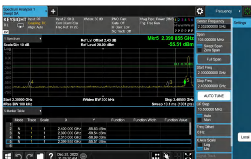
3DH5-Ant0-Hop_2402-PASS
