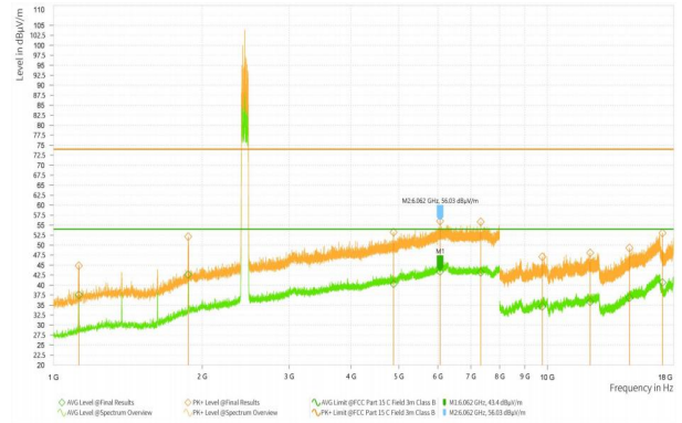
BT_DH5_2441_Low
