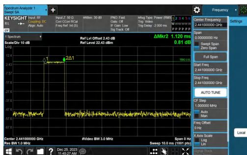
3DH5-Ant0-Hop-PASS
