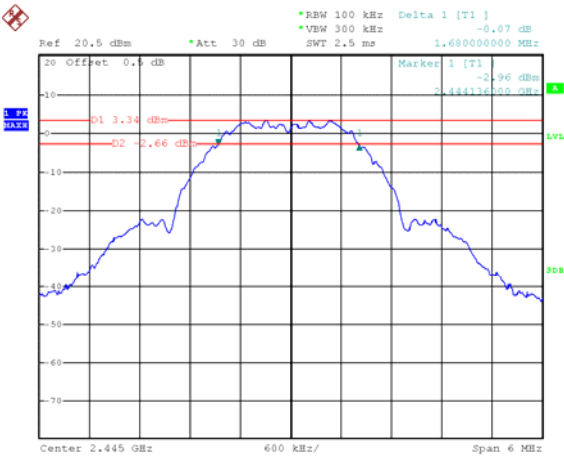
Mode: TX OQPSK channel 19
