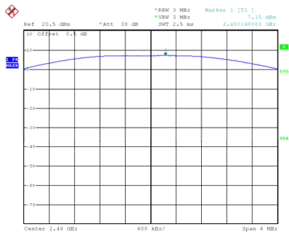
Mode: TX OQPSK channel 26
