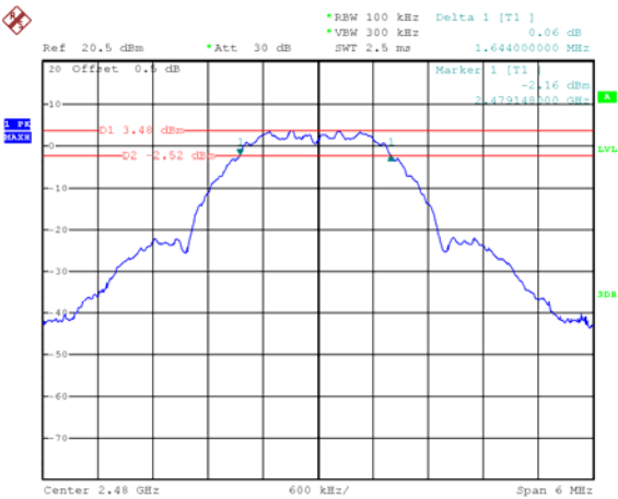
Mode: TX OQPSK channel 26
