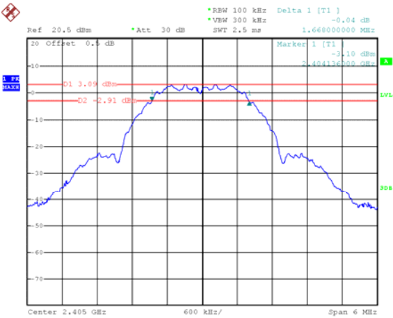
Mode: TX OQPSK channel 11
