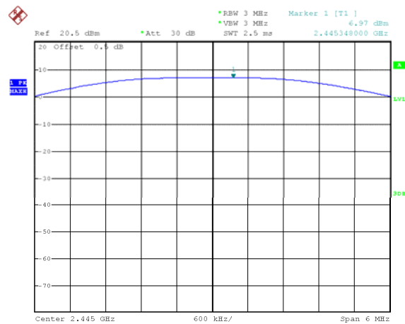
Mode: TX OQPSK channel 19
