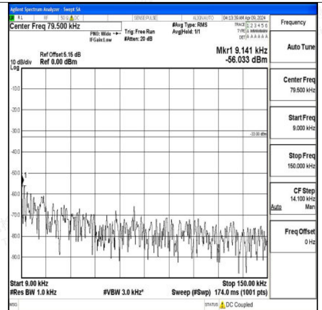
Band5_5MHz_16QAM_20625_1RB#0_0.009~0.15_0.009~0.15
