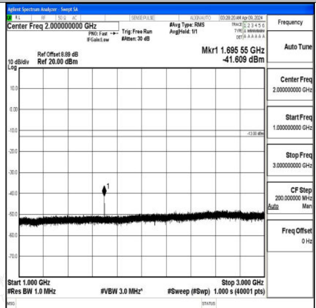
Band5_1.4MHz_QPSK_20643_1RB#0_1000~3000_1000~3 000
