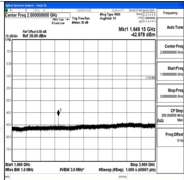
Band5_10MHz_QPSK_20450_1RB#0_1000~3000_1000~3000
