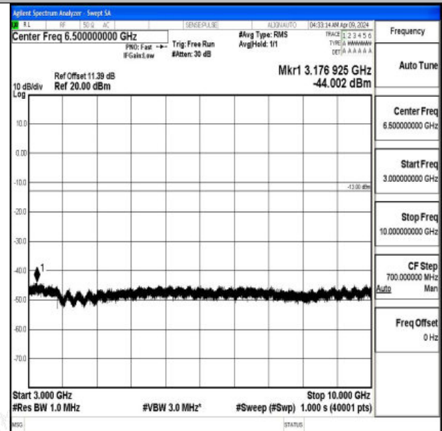
Band5_10MHz_16QAM_20600_1RB#0_3000~10000_3000 ~10000
