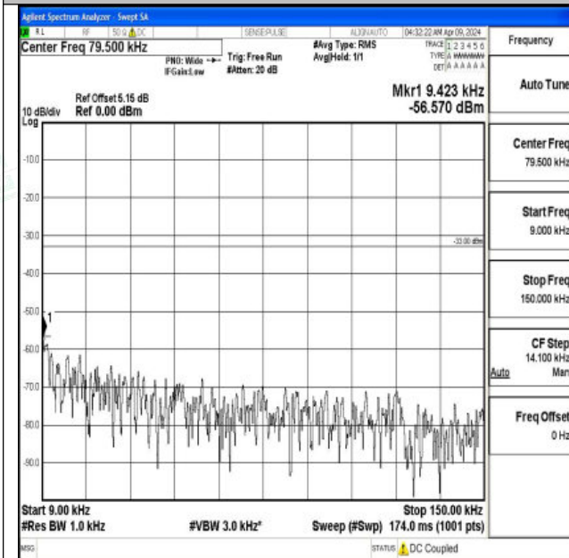
Band5_10MHz_QPSK_20600_1RB#0_0.009~0.15_0.009~ 0.15
