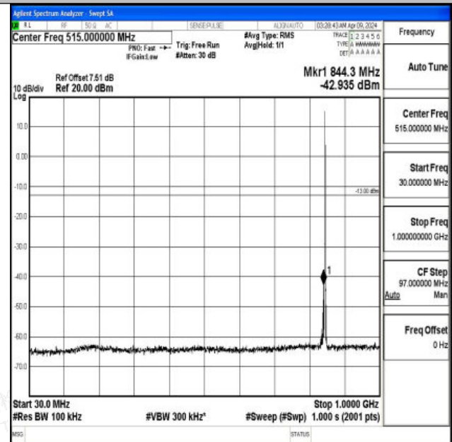
Band5_1.4MHz_16QAM_20643_1RB#0_30~1000_30~1000
