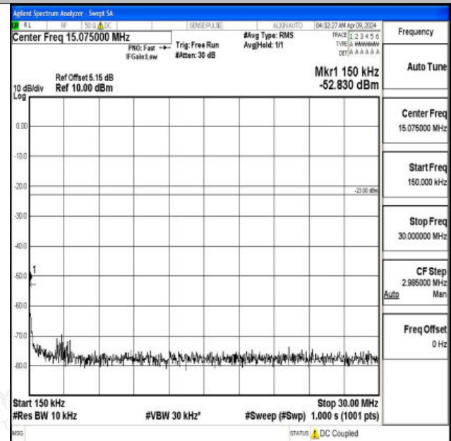
Band5_10MHz_QPSK_20600_1RB#0_0.15~30_0.15~30
