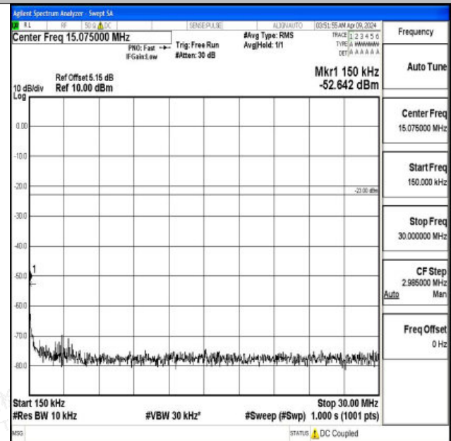
Band5_3MHz_QPSK_20415_1RB#0_0.15~30_0.15~30
