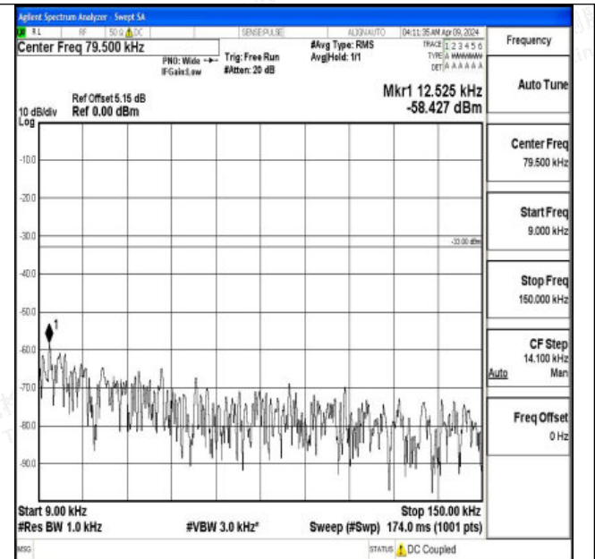
Band5_5MHz_16QAM_20425_1RB#0_0.009~0.15_0.009~0.15
