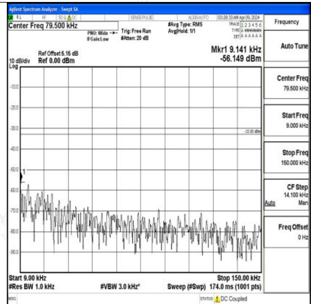
Band5_1.4MHz_16QAM_20643_1RB#0_0.009~0.15_0.009 ~0.15
