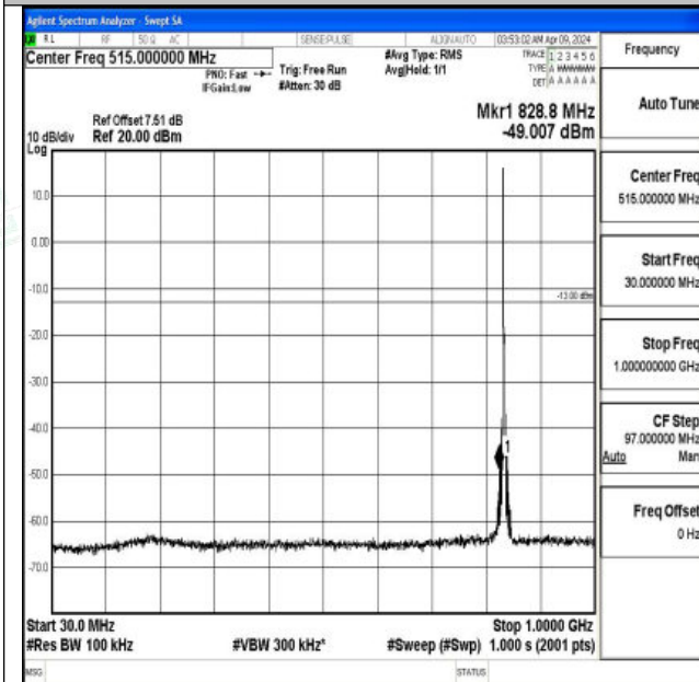
Band5_3MHz_QPSK_20525_1RB#0_30~1000_30~1000
