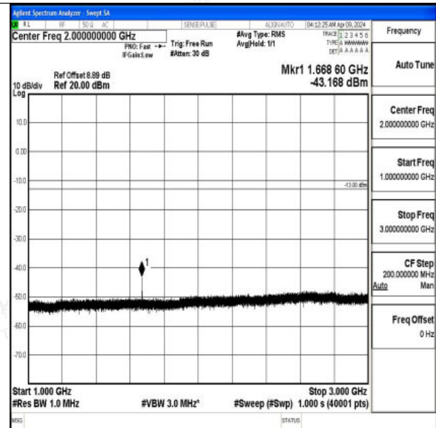
Band5_5MHz_QPSK_20525_1RB#0_1000~3000_1000~3000
