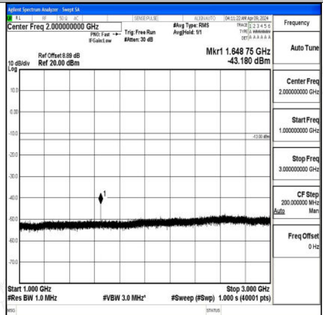
Band5_5MHz_QPSK_20425_1RB#0_1000~3000_1000~3000
