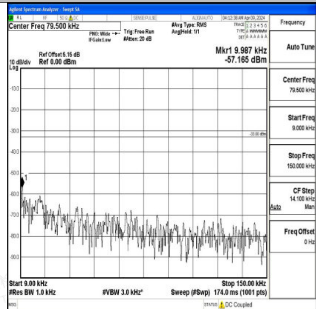
Band5_5MHz_16QAM_20525_1RB#0_0.009~0.15_0.009~0.15
