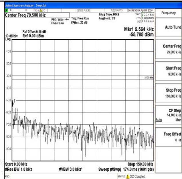
Band5_10MHz_16QAM_20450_1RB#0_0.009~0.15_0.009~0.15
