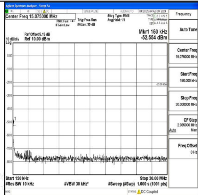
Band5_10MHz_QPSK_20450_1RB#0_0.15~30_0.15~30
