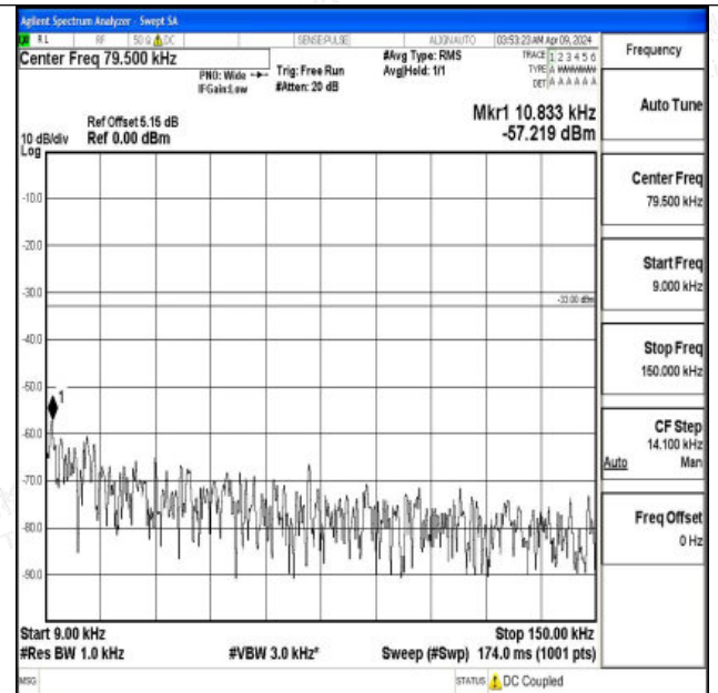
Band5_3MHz_16QAM_20525_1RB#0_0.009~0.15_0.009~0.15
