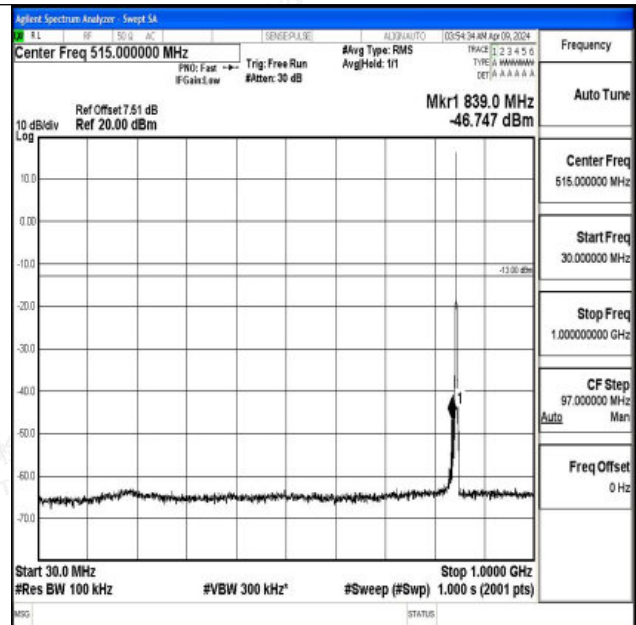
Band5_3MHz_16QAM_20635_1RB#0_30~1000_30~1000
