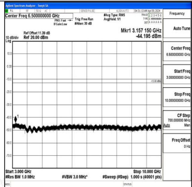
Band5_10MHz_16QAM_20450_1RB#0_3000~10000_3000 ~10000
