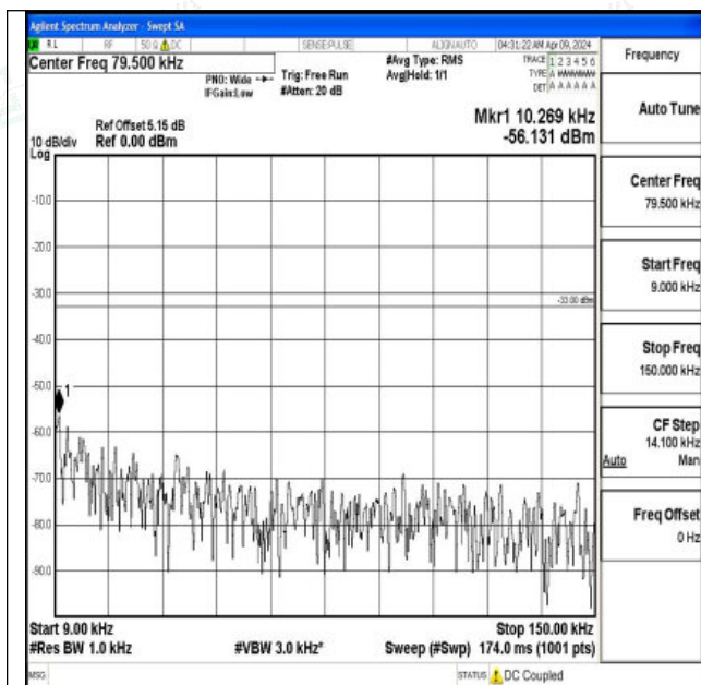
Band5_10MHz_QPSK_20525_1RB#0_0.009~0.15_0.009~0.15
