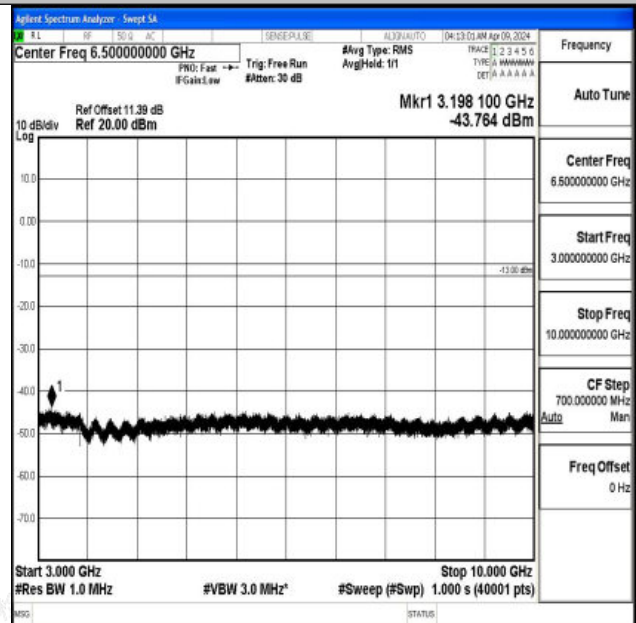
Band5_5MHz_16QAM_20525_1RB#0_3000~10000_3000~10000
