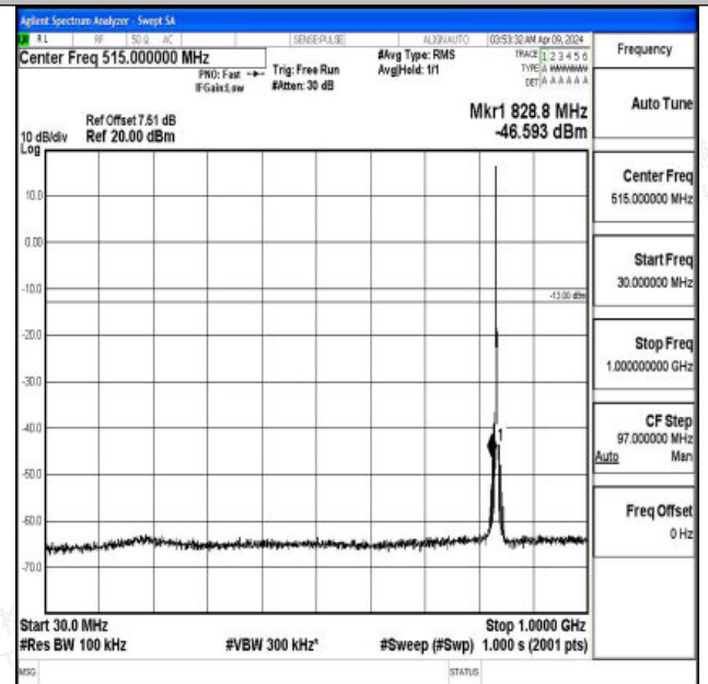
Band5_3MHz_16QAM_20525_1RB#0_30~1000_30~1000
