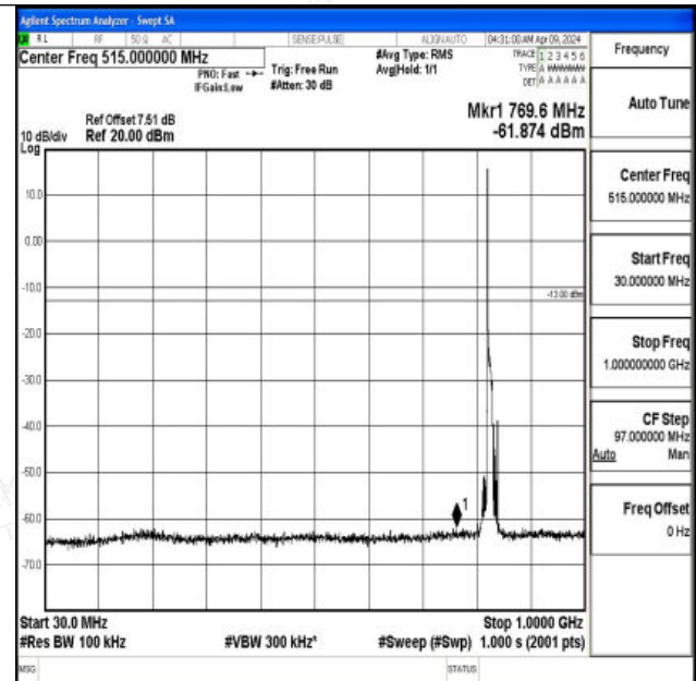
Band5_10MHz_16QAM_20450_1RB#0_30~1000_30~1000
