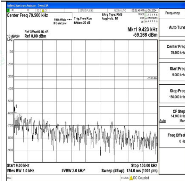
Band5_3MHz_QPSK_20415_1RB#0_0.009~0.15_0.009~0.15
