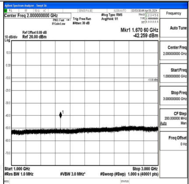
Band5_3MHz_QPSK_20525_1RB#0_1000~3000_1000~3000
