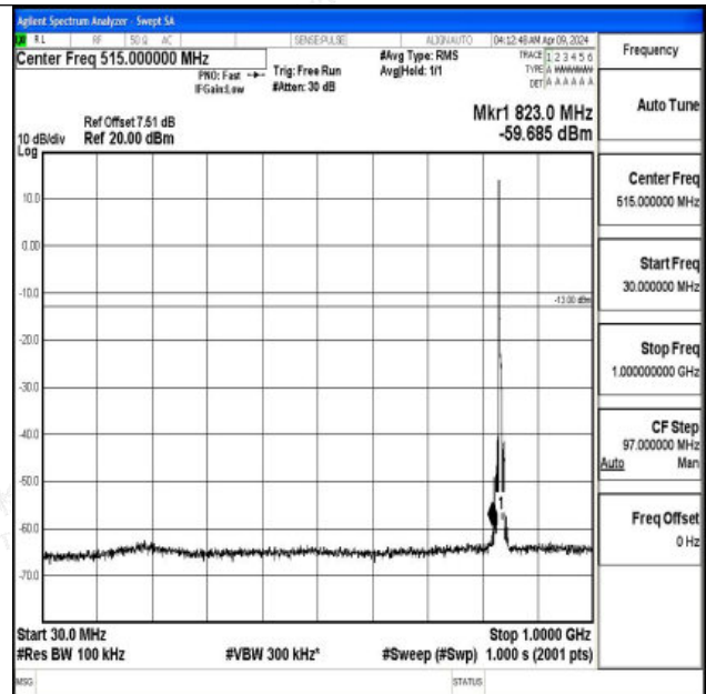
Band5_5MHz_16QAM_20525_1RB#0_30~1000_30~1000
