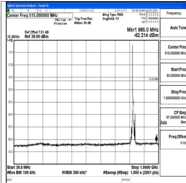
Band5_10MHz_QPSK_20450_1RB#0_30~1000_30~1000
