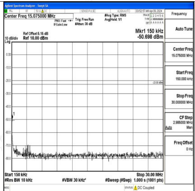
Band5_3MHz_QPSK_20525_1RB#0_0.15~30_0.15~30
