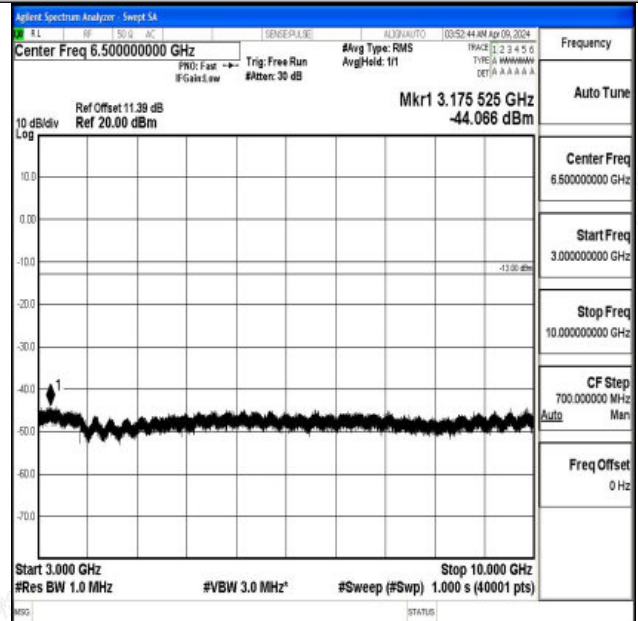
Band5_3MHz_16QAM_20415_1RB#0_3000~10000_3000~10000
