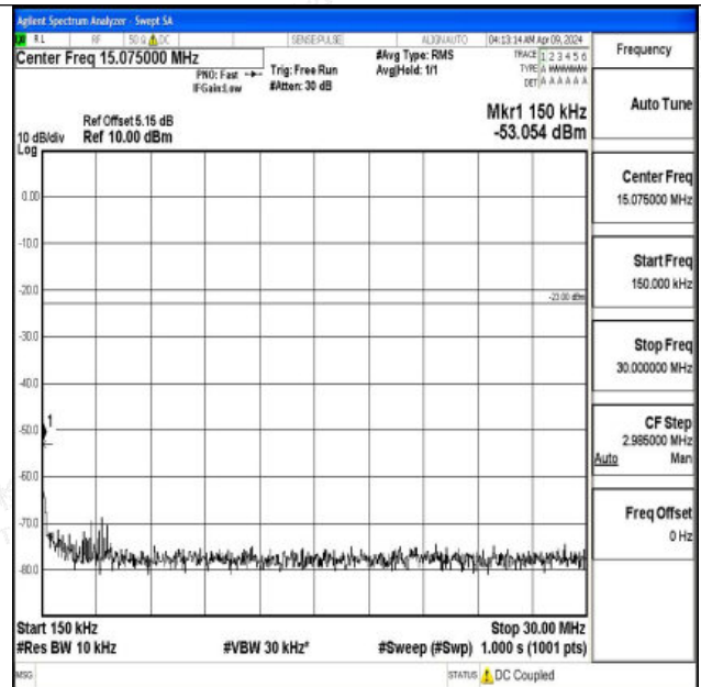
Band5_5MHz_QPSK_20625_1RB#0_0.15~30_0.15~30
