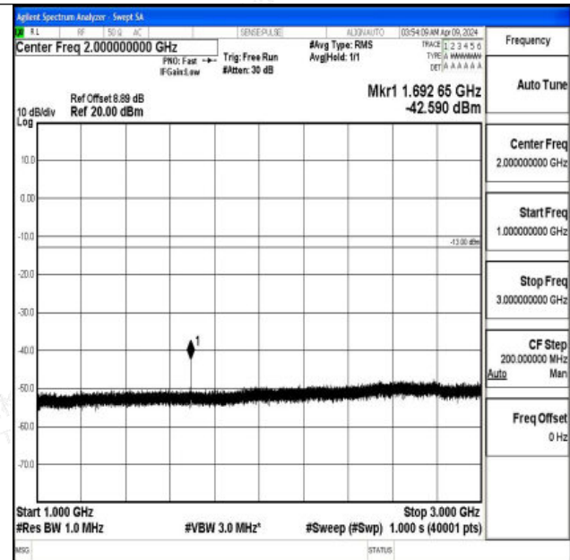
Band5_3MHz_QPSK_20635_1RB#0_1000~3000_1000~3000
