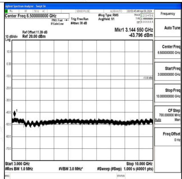
Band5_3MHz_16QAM_20525_1RB#0_3000~10000_3000~10000
