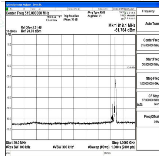
Band5_10MHz_QPSK_20600_1RB#0_30~1000_30~1000
