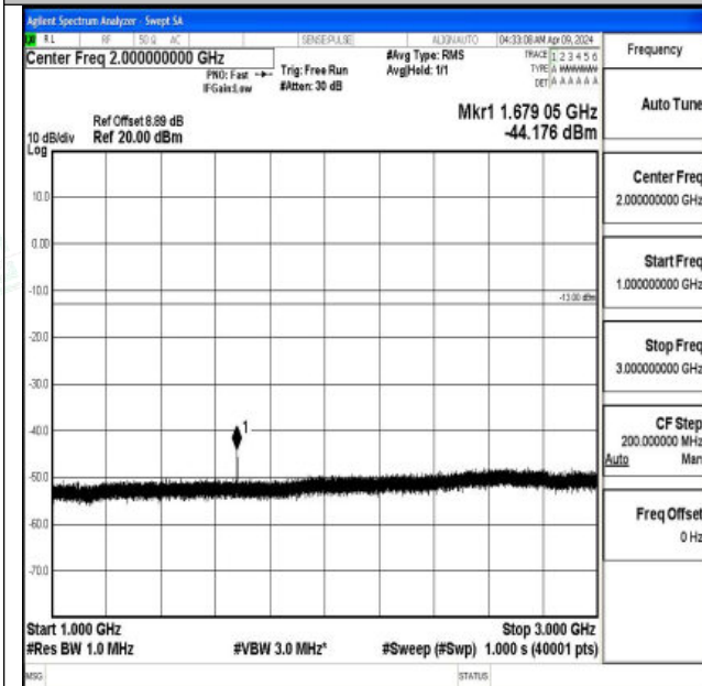
Band5_10MHz_16QAM_20600_1RB#0_1000~3000_1000 ~3000
