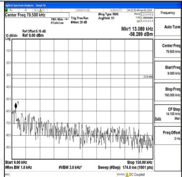
Band5_10MHz_16QAM_20600_1RB#0_0.009~0.15_0.009~0.15
