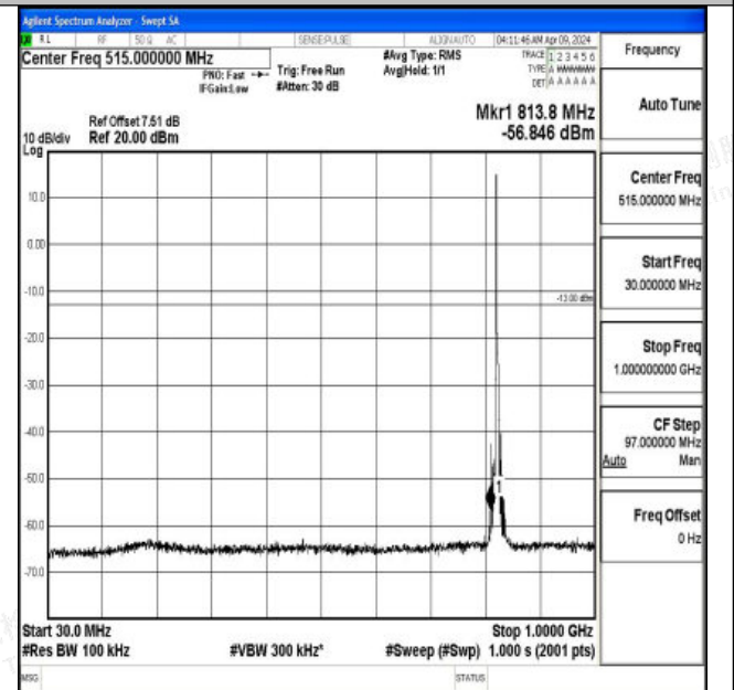
Band5_5MHz_16QAM_20425_1RB#0_30~1000_30~1000
