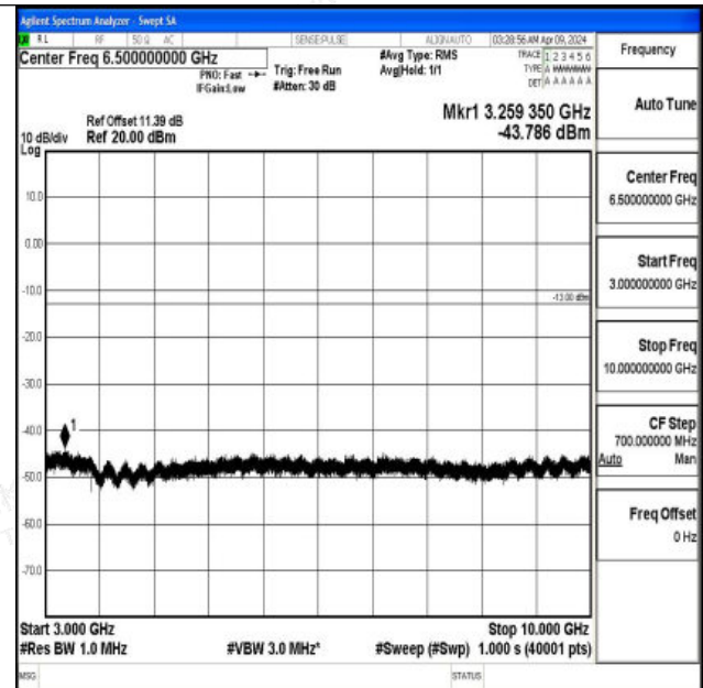
Band5_1.4MHz_16QAM_20643_1RB#0_3000~10000_3000 ~10000
