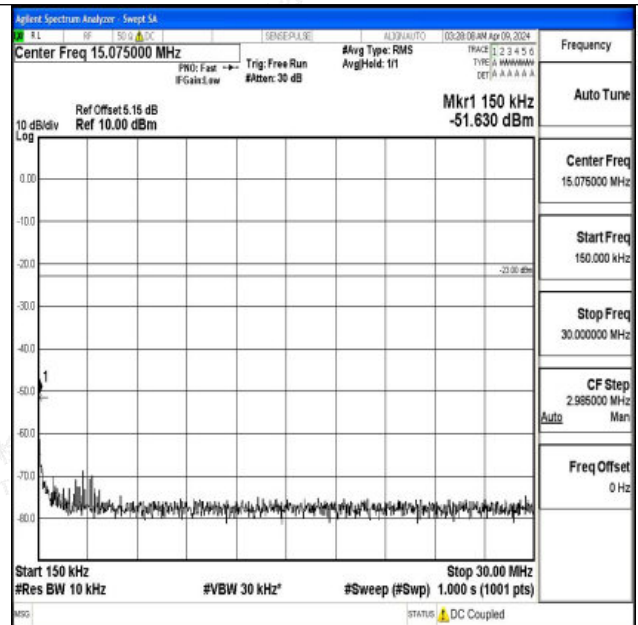
Band5_1.4MHz_QPSK_20643_1RB#0_0.15~30_0.15~30
