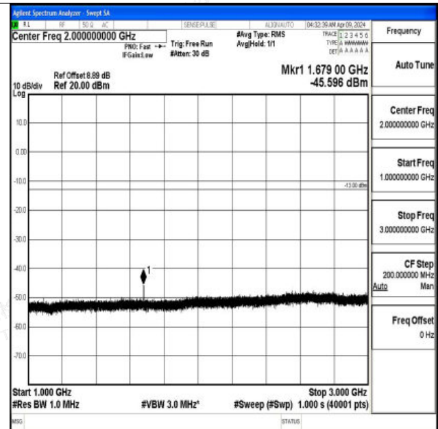
Band5_10MHz_QPSK_20600_1RB#0_1000~3000_1000~3000
