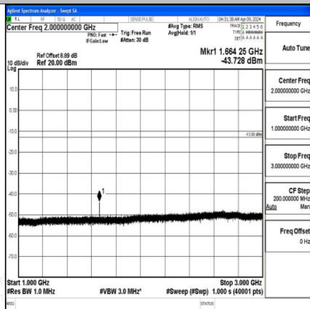
Band5_10MHz_QPSK_20525_1RB#0_1000~3000_1000~3000
