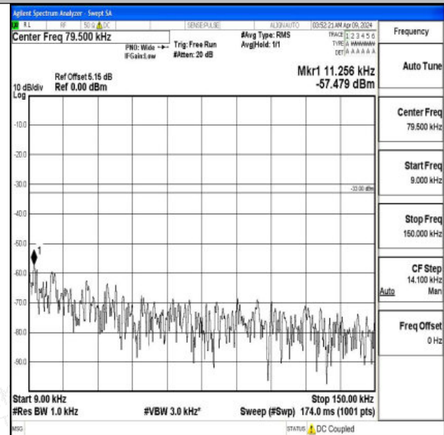
Band5_3MHz_16QAM_20415_1RB#0_0.009~0.15_0.009~0.15
