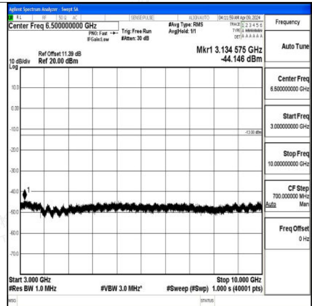
Band5_5MHz_16QAM_20425_1RB#0_3000~10000_3000~10000
