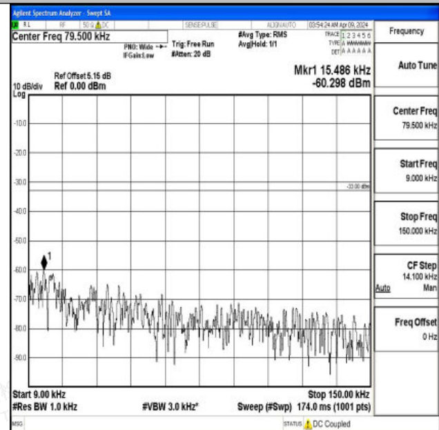
Band5_3MHz_16QAM_20635_1RB#0_0.009~0.15_0.009~0.15
