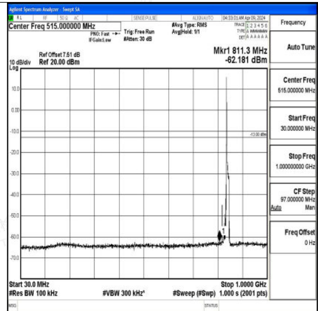
Band5_10MHz_16QAM_20600_1RB#0_30~1000_30~1000
