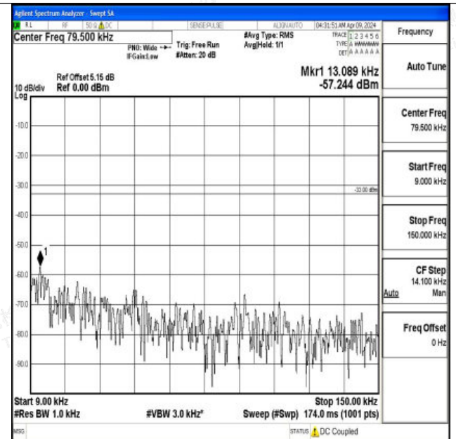
Band5_10MHz_16QAM_20525_1RB#0_0.009~0.15_0.009~0.15
