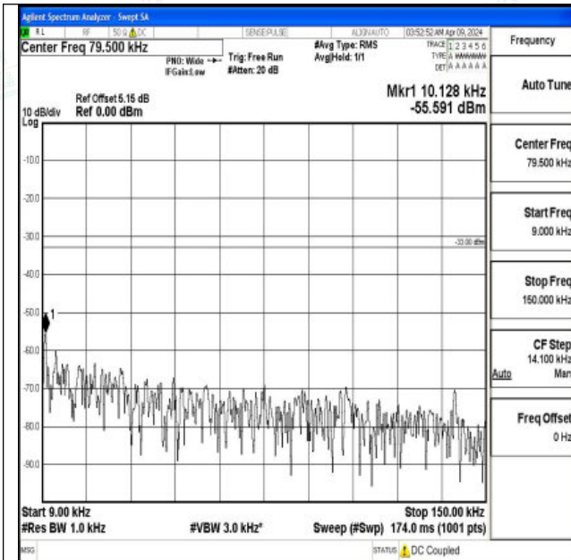
Band5_3MHz_QPSK_20525_1RB#0_0.009~0.15_0.009~0.15
