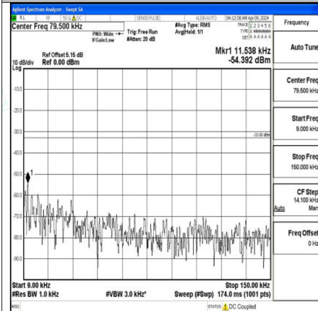
Band5_5MHz_QPSK_20525_1RB#0_0.009~0.15_0.009~0.15
