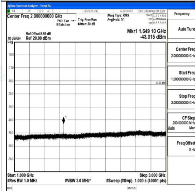
Band5_10MHz_16QAM_20450_1RB#0_1000~3000_1000 ~3000
