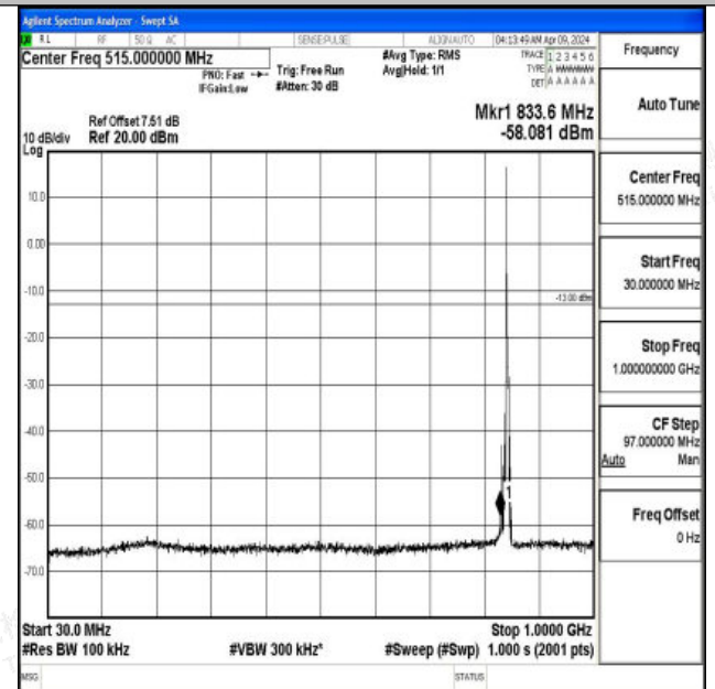
Band5_5MHz_16QAM_20625_1RB#0_30~1000_30~1000
