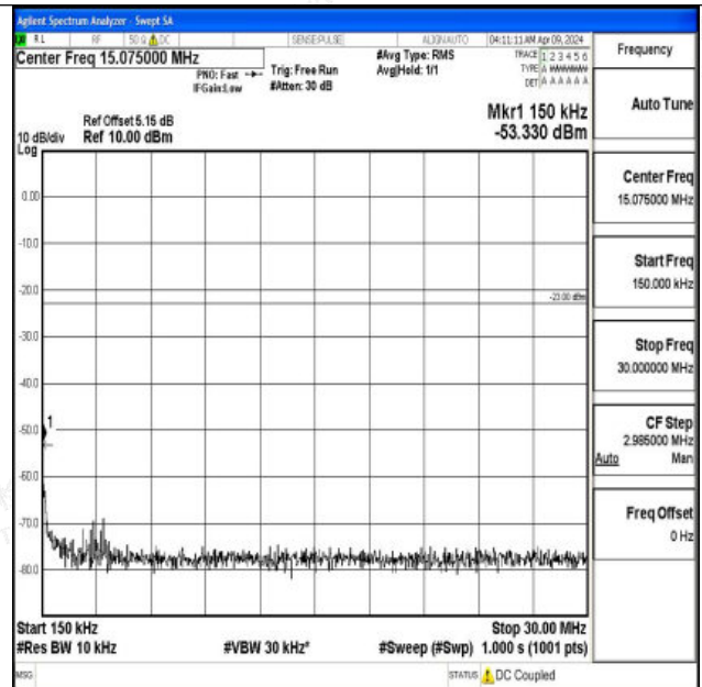
Band5_5MHz_QPSK_20425_1RB#0_0.15~30_0.15~30
