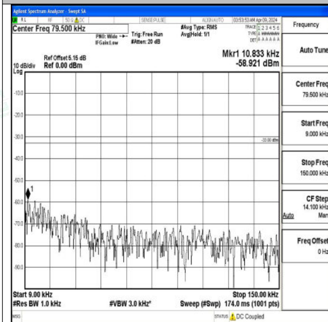
Band5_3MHz_QPSK_20635_1RB#0_0.009~0.15_0.009~0.15
