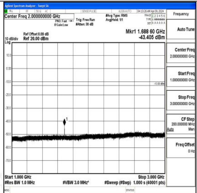
Band5_5MHz_QPSK_20625_1RB#0_1000~3000_1000~3000
