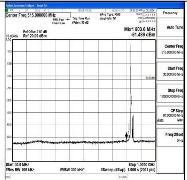
Band5_10MHz_16QAM_20525_1RB#0_30~1000_30~1000
