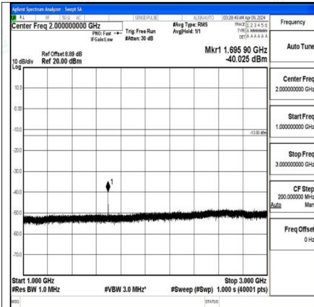
Band5_1.4MHz_16QAM_20643_1RB#0_1000~3000_1000 ~3000
