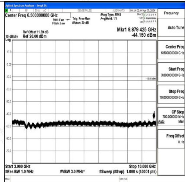
Band5_5MHz_16QAM_20625_1RB#0_3000~10000_3000~10000
