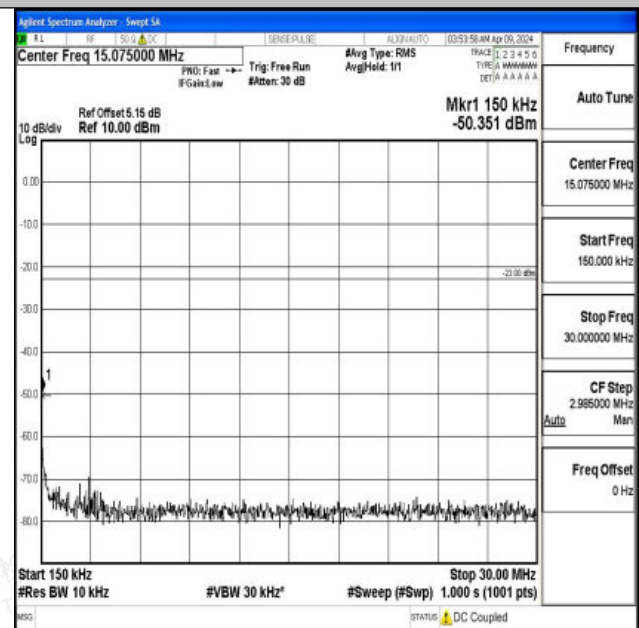
Band5_3MHz_QPSK_20635_1RB#0_0.15~30_0.15~30
