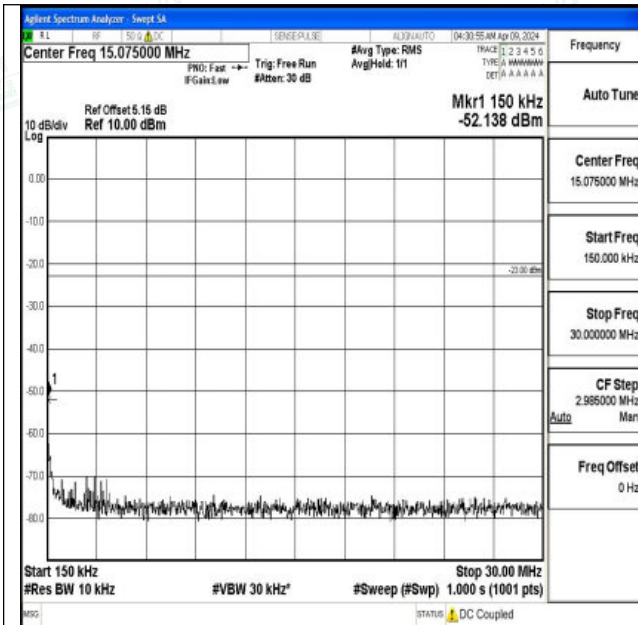
Band5_10MHz_16QAM_20450_1RB#0_0.15~30_0.15~30
