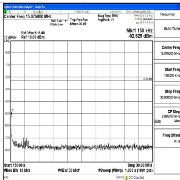
Band5_10MHz_QPSK_20525_1RB#0_0.15~30_0.15~30
