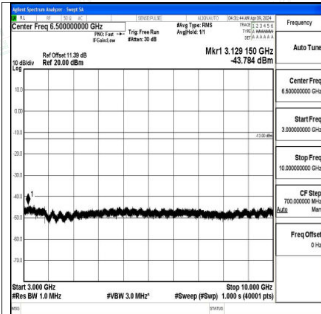
Band5_10MHz_QPSK_20525_1RB#0_3000~10000_3000~10000
