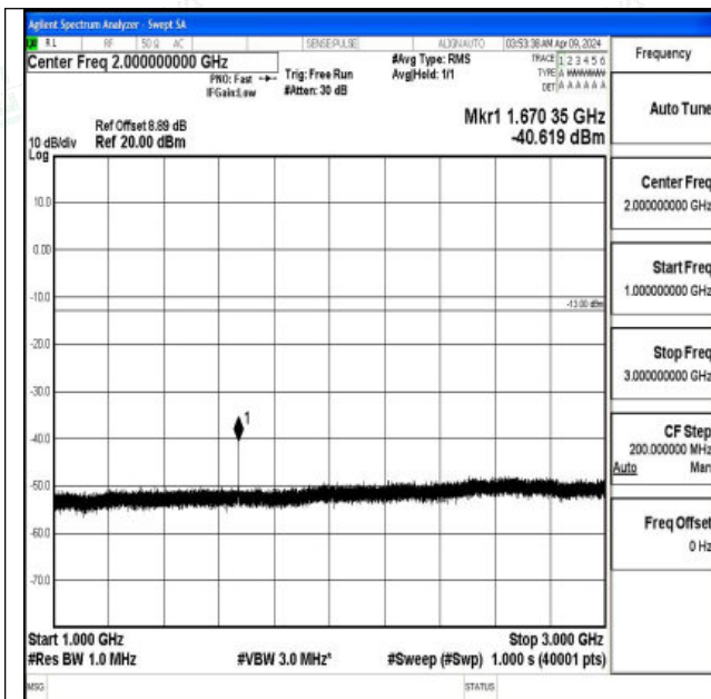
Band5_3MHz_16QAM_20525_1RB#0_1000~3000_1000~3000
