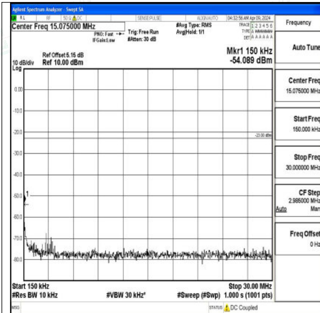
Band5_10MHz_16QAM_20600_1RB#0_0.15~30_0.15~30
