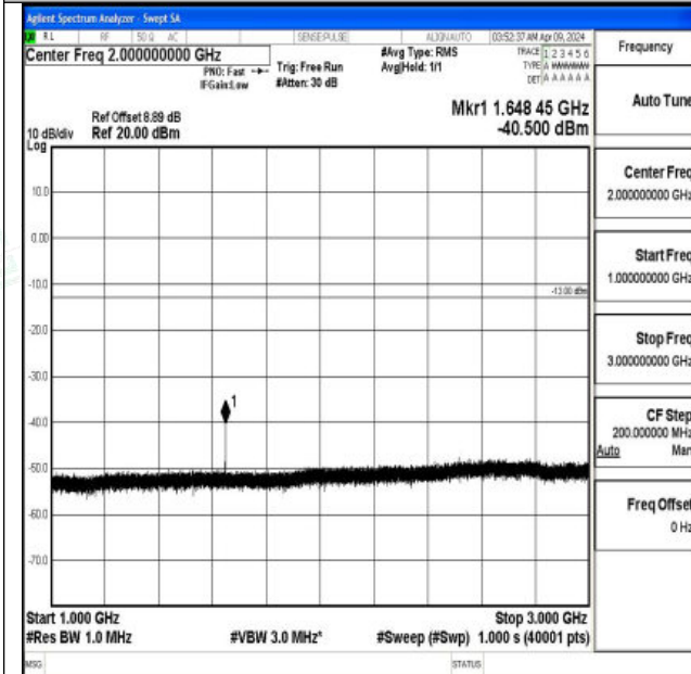
Band5_3MHz_16QAM_20415_1RB#0_1000~3000_1000~3000
