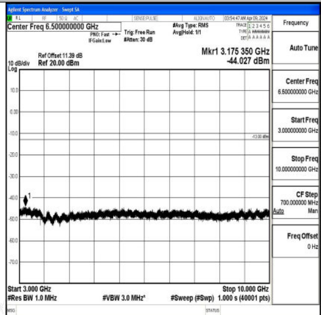
Band5_3MHz_16QAM_20635_1RB#0_3000~10000_3000~10000
