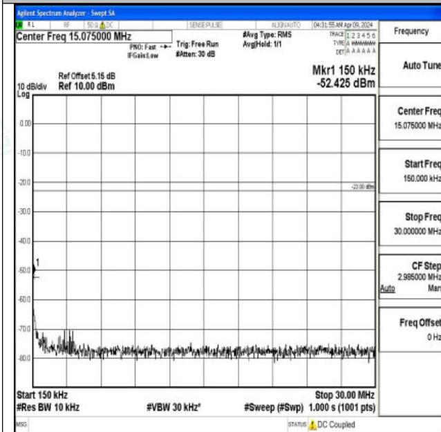
Band5_10MHz_16QAM_20525_1RB#0_0.15~30_0.15~30
