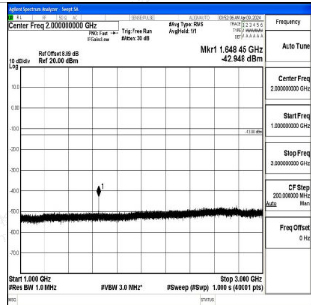
Band5_3MHz_QPSK_20415_1RB#0_1000~3000_1000~3000
