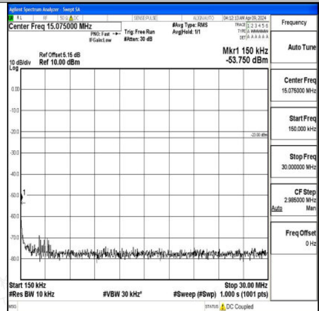
Band5_5MHz_QPSK_20525_1RB#0_0.15~30_0.15~30
