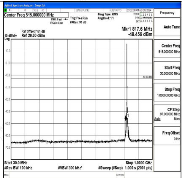
Band5_3MHz_16QAM_20415_1RB#0_30~1000_30~1000
