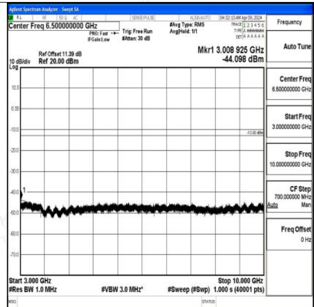
Band5_10MHz_16QAM_20525_1RB#0_3000~10000_3000 ~10000
