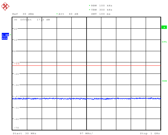
NB-IOT Band 4 CH Middle 30MHz~1GHz
