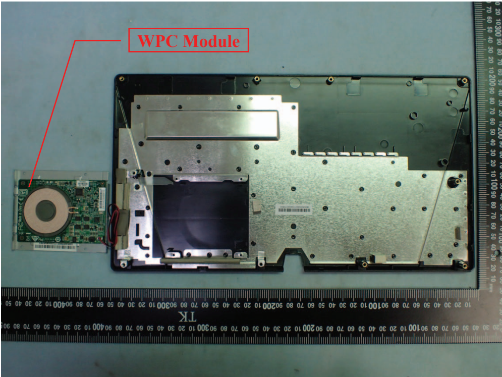
Figure 6 Personal Computer (D17W8), Internal View
