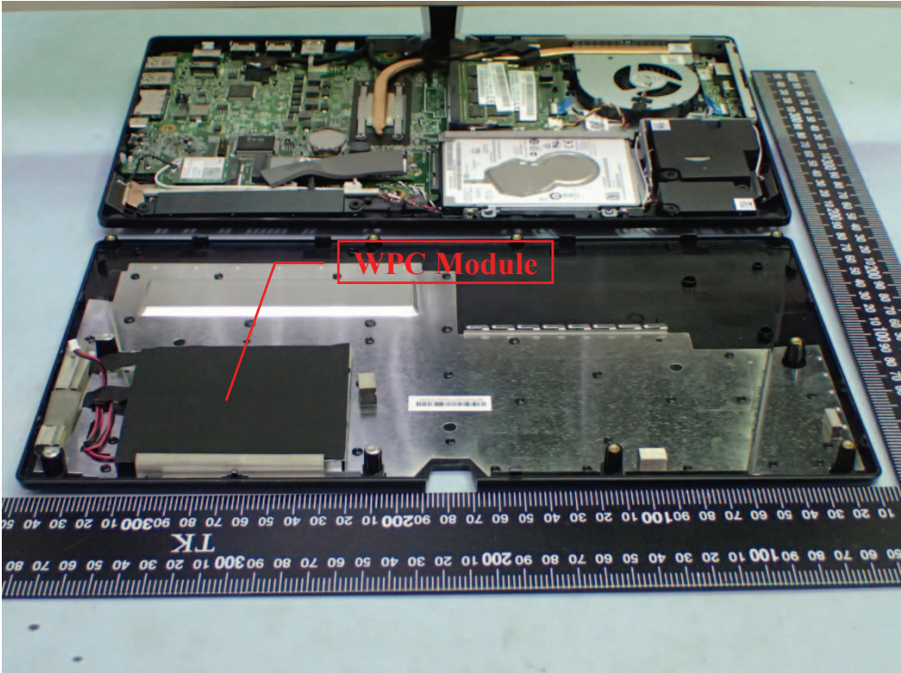
Figure 5 Personal Computer (D17W8), Internal View (Removed Base Cover)
