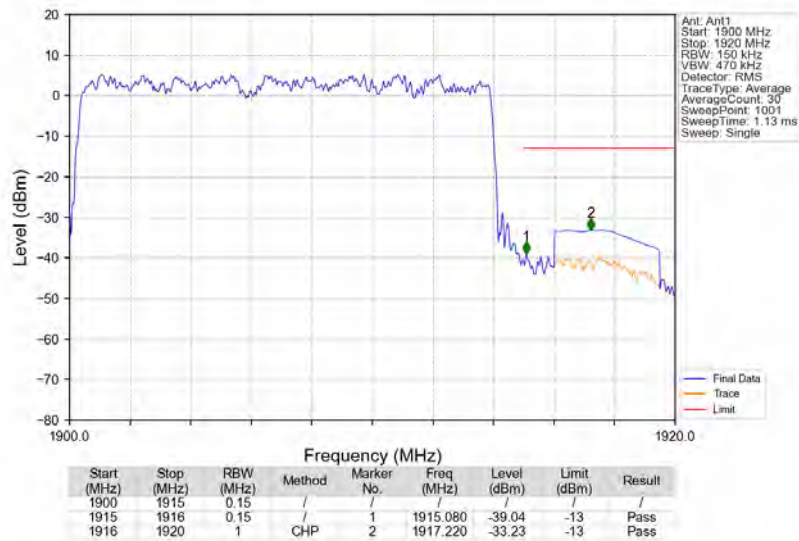
n25_15kHz_SISO_NTNV_15MHz_DFT-s-OFDM_QPSK_1907.5MHz_Outer_Full
