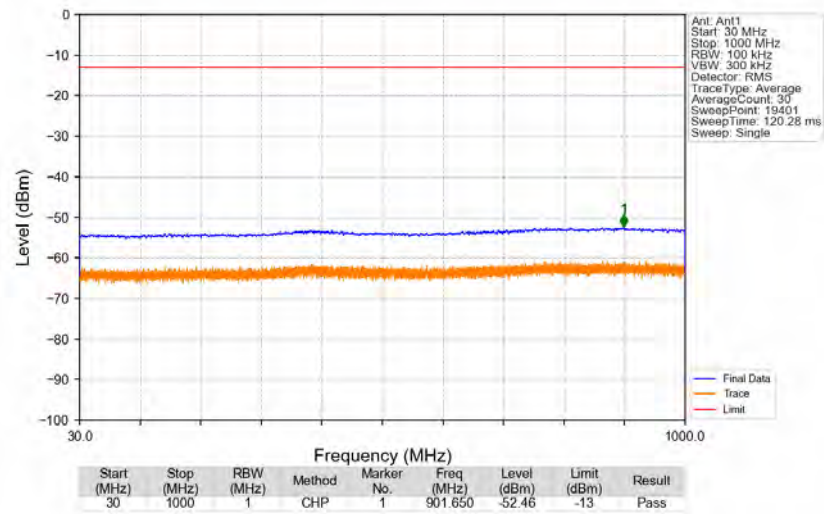
n25_15kHz_SISO_NTNV_20MHz_DFT-s-OFDM_QPSK_1905MHz_Edge_1RB_Right
