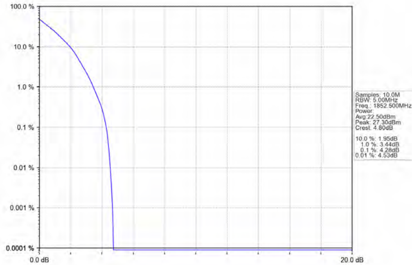
n25_15kHz_SISO_NTNV_5MHz_DFT-s-OFDM PI/2 BPSK_1852.5MHz_Outer_Full
