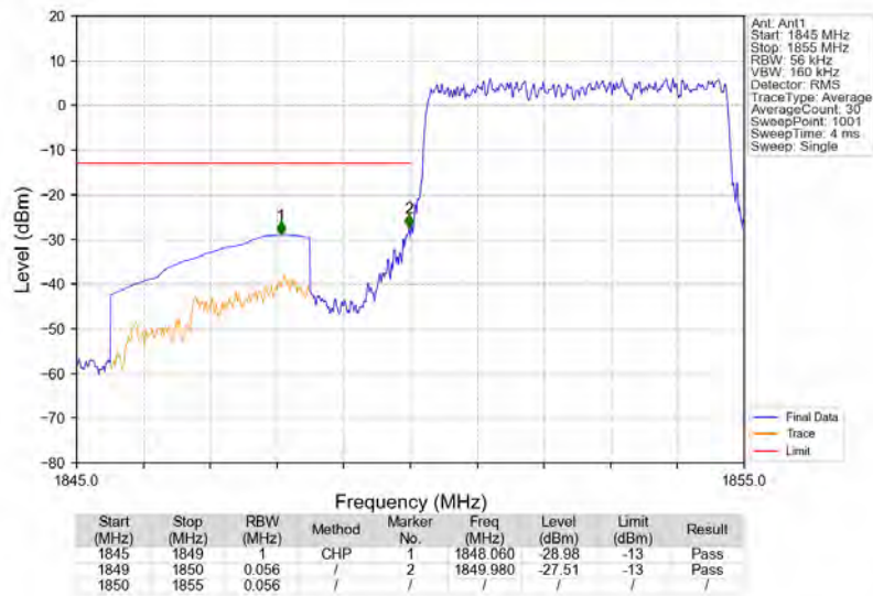
n25_15kHz_SISO_NTNV_5MHz_DFT-s-OFDM PI/2 BPSK_1852.5MHz_Outer_Full
