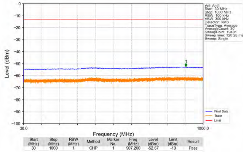
n25_15kHz_SISO_NTNV_20MHz_DFT-s-OFDM_QPSK_1882.5MHz_Edge_1RB_Left
