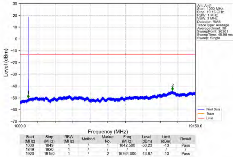
n25_15kHz_SISO_NTNV_10MHz_CP-OFDM_QPSK_1855MHz_Edge_1RB_Left
