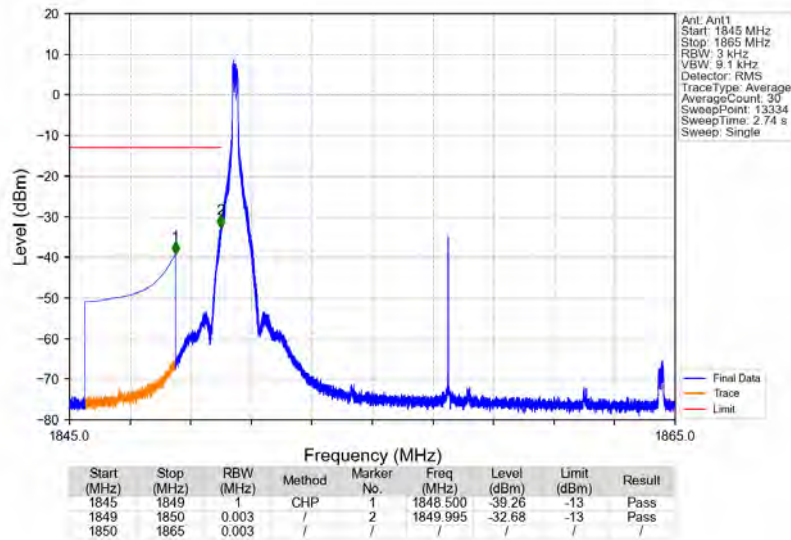
n25_15kHz_SISO_NTNV_15MHz_DFT-s-OFDM PI/2 BPSK_1857.5MHz_Edge_1RB_Left
