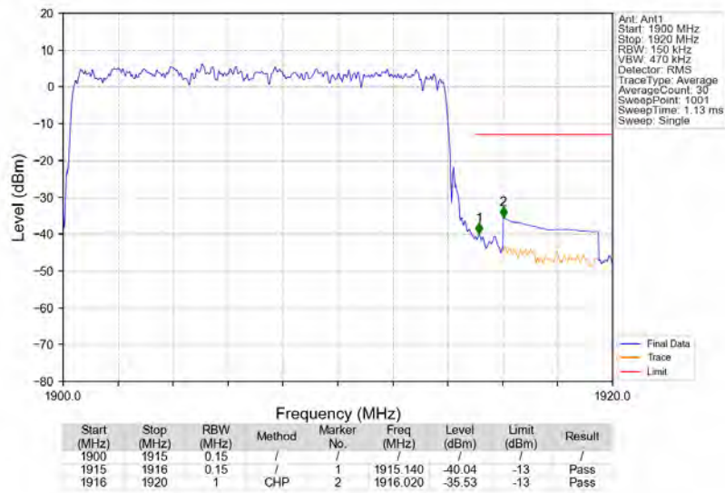
n25_15kHz_SISO_NTNV_15MHz_DFT-s-OFDM_PI/2_BPSK_1907.5MHz_Outer_Full
