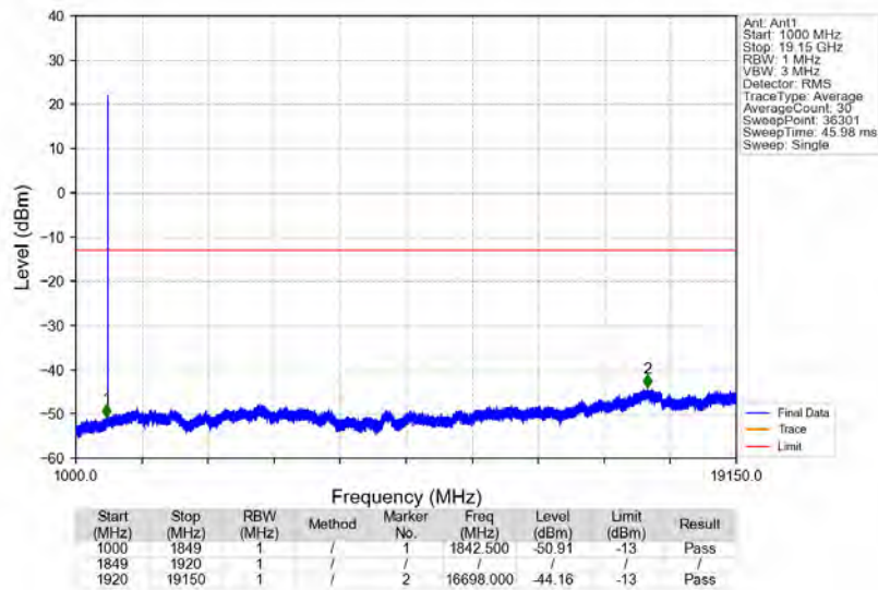
n25_15kHz_SISO_NTNV_10MHz_DFT-s-OFDM PI/2 BPSK 1882.5MHz_Edge_1RB_Left
