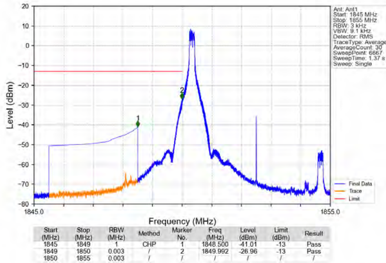
n25_15kHz_SISO_NTNV_5MHz_DFT-s-OFDM PI/2 BPSK_1852.5MHz_Edge_1RB_Left
