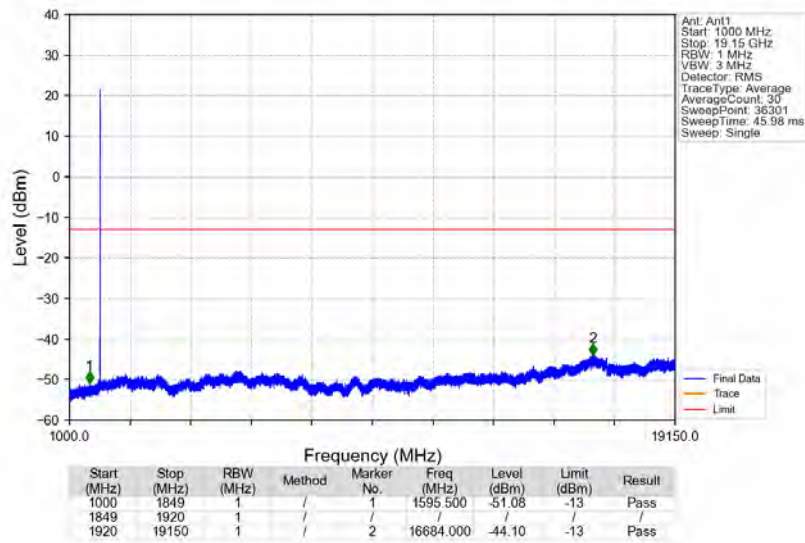
n25_15kHz_SISO_NTNV_10MHz_DFT-s-OFDM_PI/2_BPSK_1910MHz_Edge_1RB_Right
