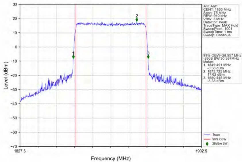
n25_15kHz_SISO_NTNV_30MHz_DFT-s-OFDM_QPSK_1865MHz_Outer_Full
