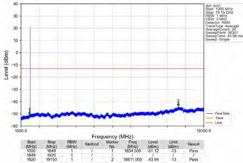
n25_15kHz_SISO_NTNV_15MHz_DFT-s-OFDM_QPSK_1907.5MHz_Edge_1RB_Right
