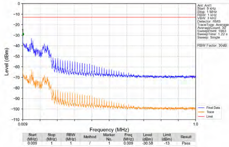
n25_15kHz_SISO_NTNV_5MHz_DFT-s-OFDM PI/2 BPSK_1882.5MHz_Edge_1RB_Left
