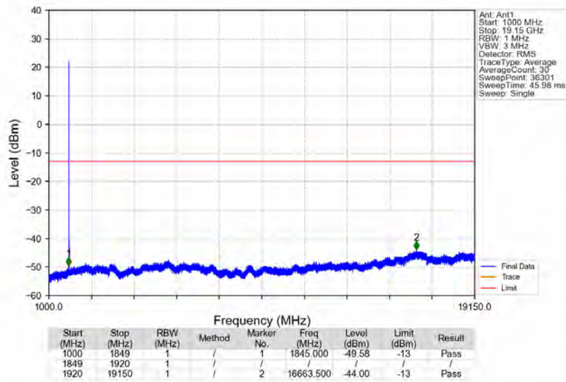
n25_15kHz_SISO_NTNV_10MHz_DFT-s-OFDM PI/2 BPSK_1855MHz_Edge_1RB_Left
