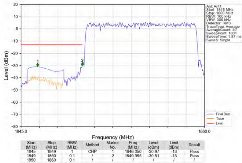
n25_15kHz_SISO_NTNV_10MHz_DFT-s-OFDM PI/2 BPSK_1855MHz_Outer_Full
