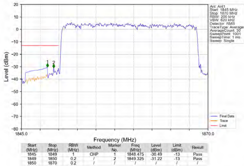
n25_15kHz_SISO_NTNV_20MHz_DFT-s-OFDM PI/2 BPSK_1860MHz_Outer_Full
