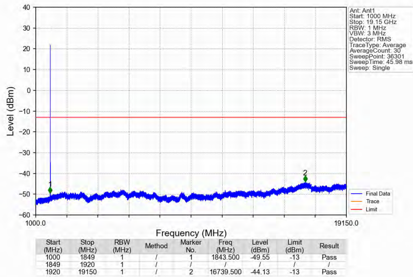
n25_15kHz_SISO_NTNV_15MHz_DFT-s-OFDM_PI/2_BPSK_1857.5MHz_Edge_1RB_Left
