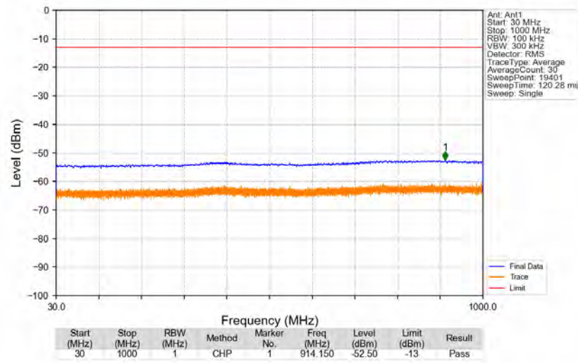
n25_15kHz_SISO_NTNV_10MHz_CP-OFDM_QPSK_1882.5MHz_Edge_1RB_Left
