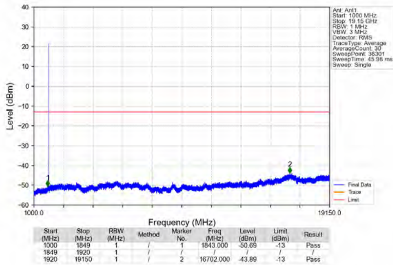
n25_15kHz_SISO_NTNV_15MHz_DFT-s-OFDM_PI/2_BPSK_1907.5MHz_Edge_1RB_Right
