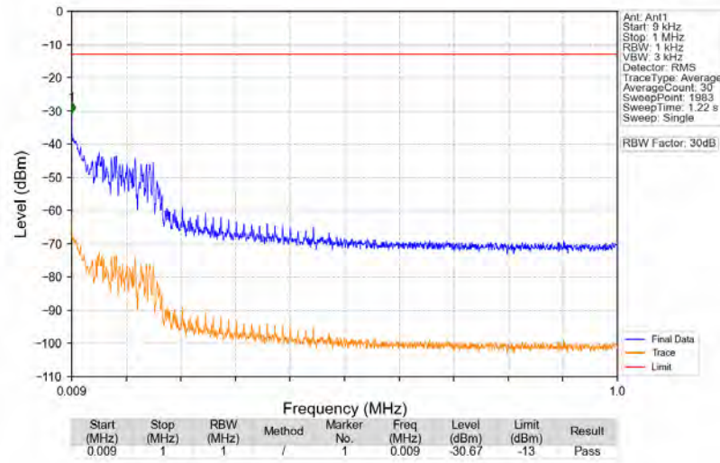
n25_15kHz_SISO_NTNV_5MHz_DFT-s-OFDM_QPSK_1882.5MHz_Edge_1RB_Left
