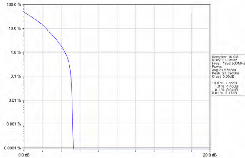
n25_15kHz_SISO_NTNV_5MHz_DFT-s-OFDM_QPSK_1852.5MHz_Outer_Full
