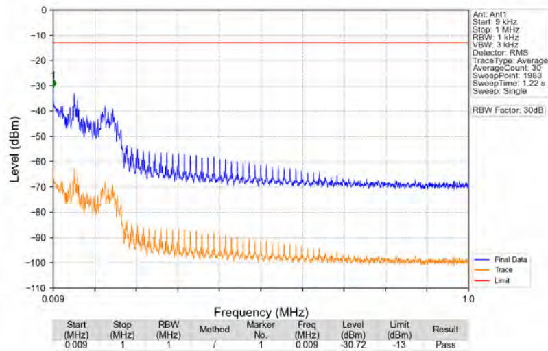
n25_15kHz_SISO_NTNV_20MHz_DFT-s-OFDM_PI/2_BPSK_1905MHz_Edge_1RB_Right
