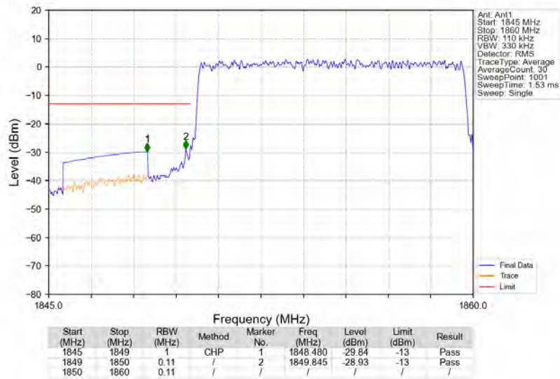
n25_15kHz_SISO_NTNV_10MHz_CP-OFDM_QPSK_1855MHz_Outer_Full
