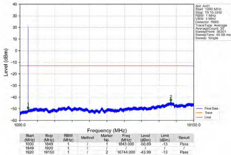
n25_15kHz_SISO_NTNV_5MHz_DFT-s-OFDM_QPSK_1852.5MHz_Edge_1RB_Left
