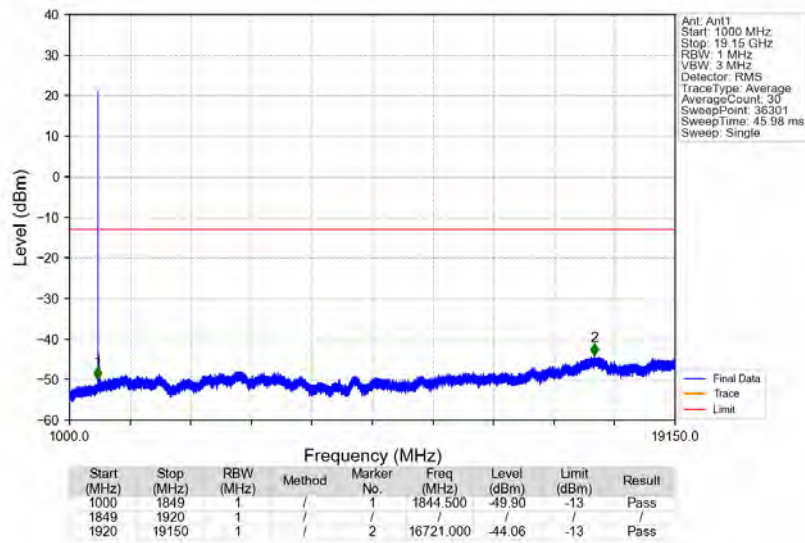
n25_15kHz_SISO_NTNV_20MHz_DFT-s-OFDM PI/2 BPSK_1860MHz_Edge_1RB_Left
