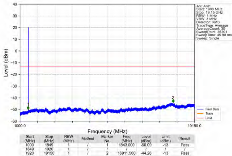
n25_15kHz_SISO_NTNV_10MHz_CP-OFDM_QPSK_1882.5MHz_Edge_1RB_Left
