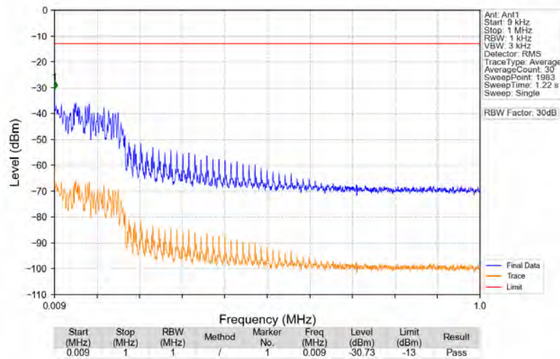
n25_15kHz_SISO_NTNV_5MHz_DFT-s-OFDM_QPSK_1852.5MHz_Edge_1RB_Left
