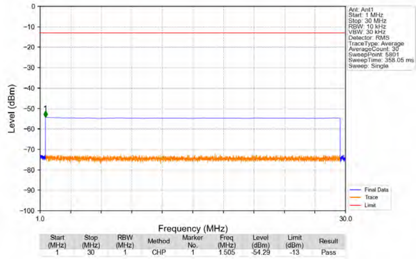
n25_15kHz_SISO_NTNV_10MHz_DFT-s-OFDM_PI/2_BPSK_1855MHz_Edge_1RB_Left
