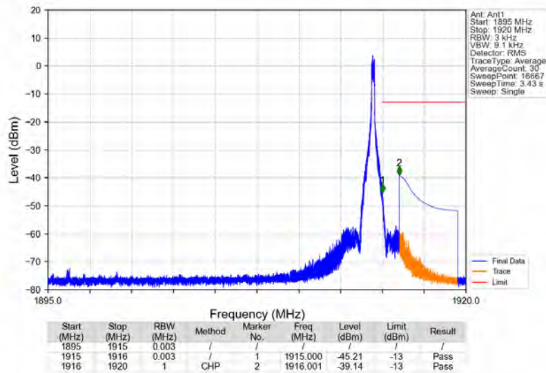
n25_15kHz_SISO_NTNV_20MHz_DFT-s-OFDM_PI/2_BPSK_1905MHz_Edge_1RB_Right
