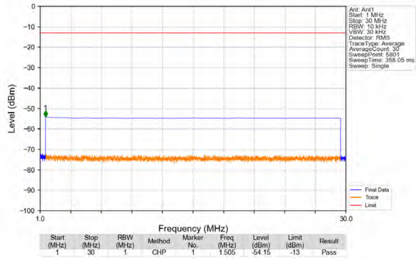
n25_15kHz_SISO_NTNV_10MHz_DFT-s-OFDM_PI/2_BPSK_1910MHz_Edge_1RB_Right
