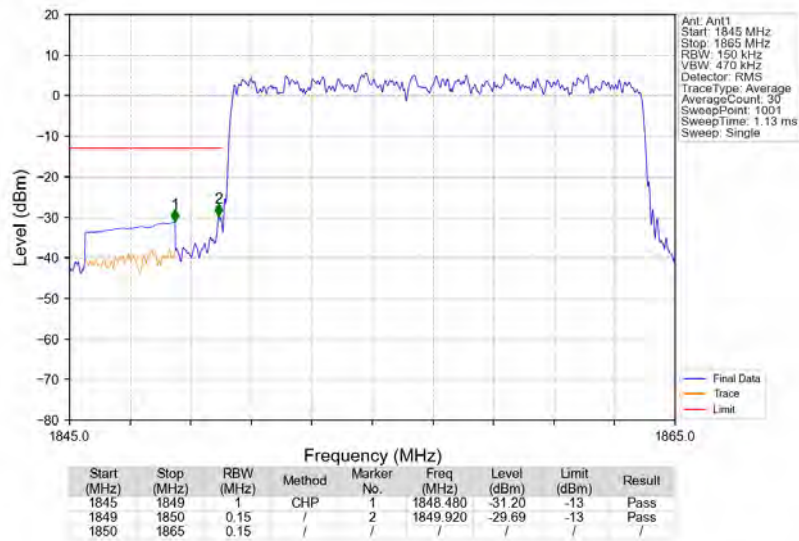
n25_15kHz_SISO_NTNV_15MHz_DFT-s-OFDM_QPSK_1857.5MHz_Outer_Full
