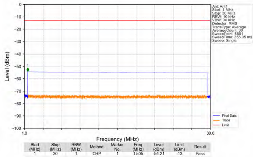
n25_15kHz_SISO_NTNV_5MHz_DFT-s-OFDM_QPSK_1852.5MHz_Edge_1RB_Left
