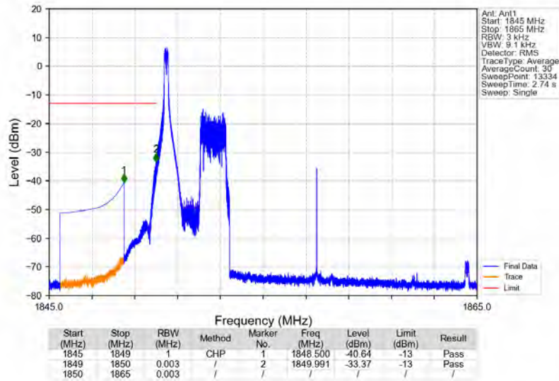
n25_15kHz_SISO_NTNV_15MHz_DFT-s-OFDM_QPSK_1857.5MHz_Edge_1RB_Left
