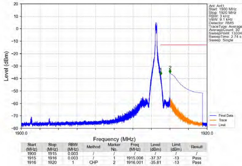
n25_15kHz_SISO_NTNV_15MHz_DFT-s-OFDM QPSK_1907.5MHz_Edge_1RB_Right
