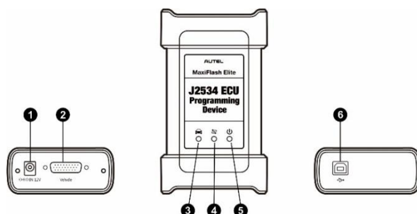
Figure 2-5 J2534 ECU Programming Device – for MaxiPro MP908P
