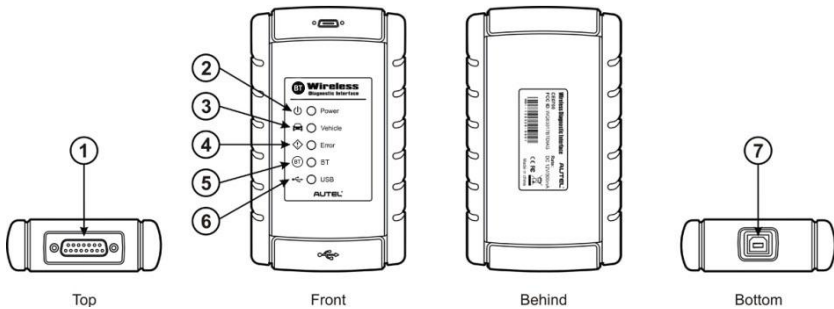
Figure 2-4 Wireless Diagnostic Interface – for MaxiPro
