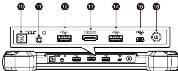
Figure 2-3 MaxiPro Tablet Top View
