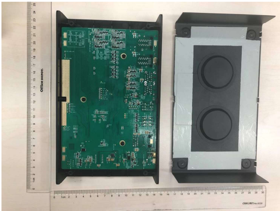
Figure 4. Internal view - 1
