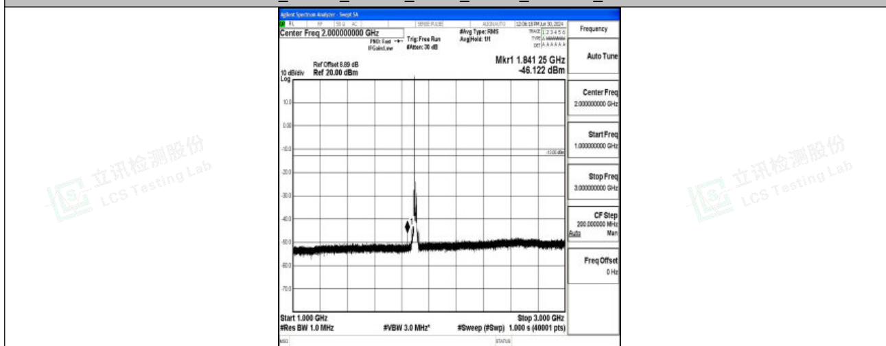
Band2_20MHz_16QAM_19100_1RB#0_1000~3000_1000~3000
