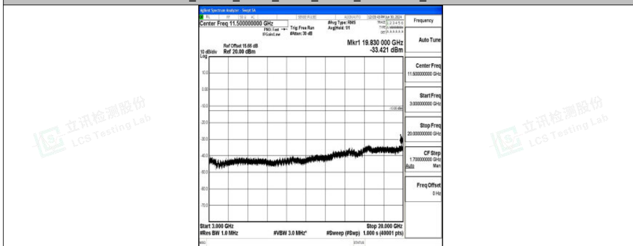
Band2_20MHz_QPSK_18700_1RB#0_3000~20000_3000~20000
