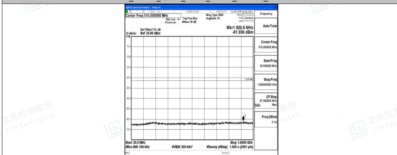
Band2_10MHz_QPSK_18900_1RB#0_30~1000_30~1000
