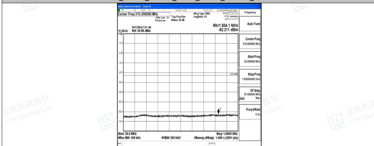
Band2_15MHz_16QAM_19125_1RB#0_30~1000_30~1000
