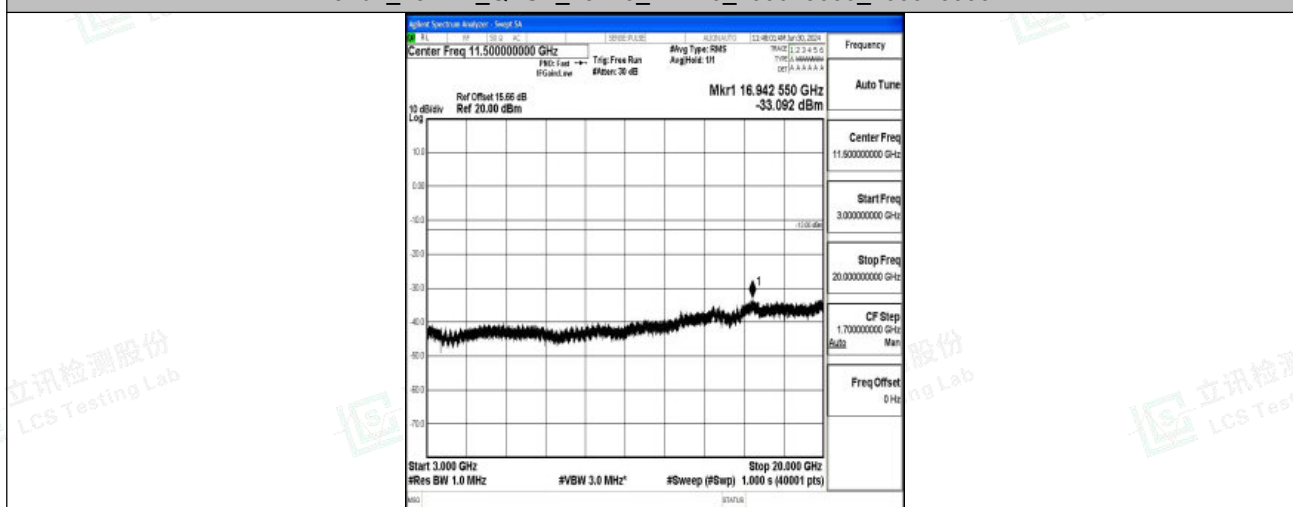
Band2_15MHz_QPSK_19125_1RB#0_3000~20000_3000~20000
