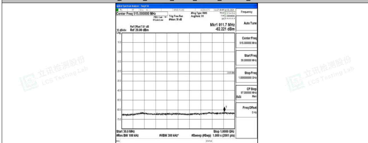
Band2_10MHz_16QAM_18650_1RB#0_30~1000_30~1000
