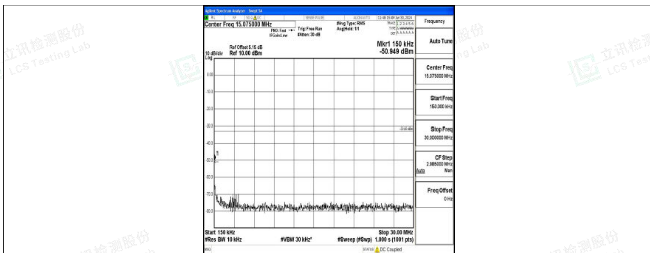
Band2_15MHz_16QAM_19125_1RB#0_0.15~30_0.15~30
