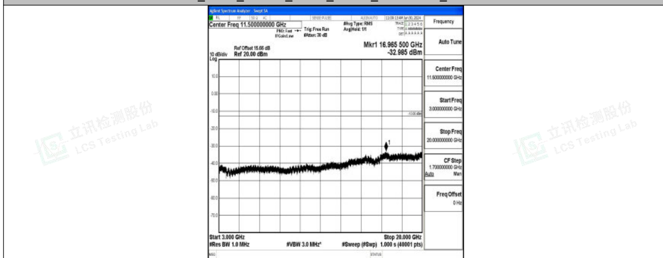
Band2_5MHz_16QAM_18900_1RB#0_3000~20000_3000~20000
