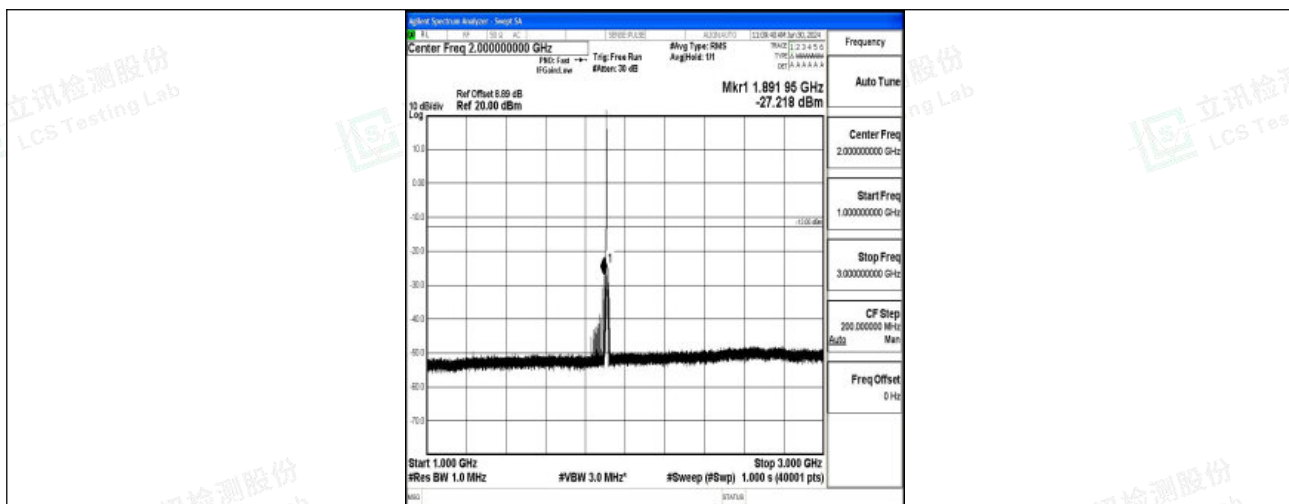
Band2_5MHz_QPSK_19175_1RB#0_1000~3000_1000~3000
