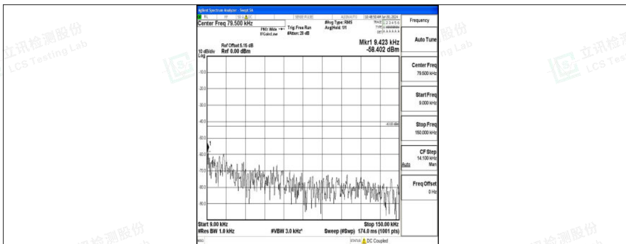
Band2_3MHz_QPSK_19185_1RB#0_0.009~0.15_0.009~0.15
