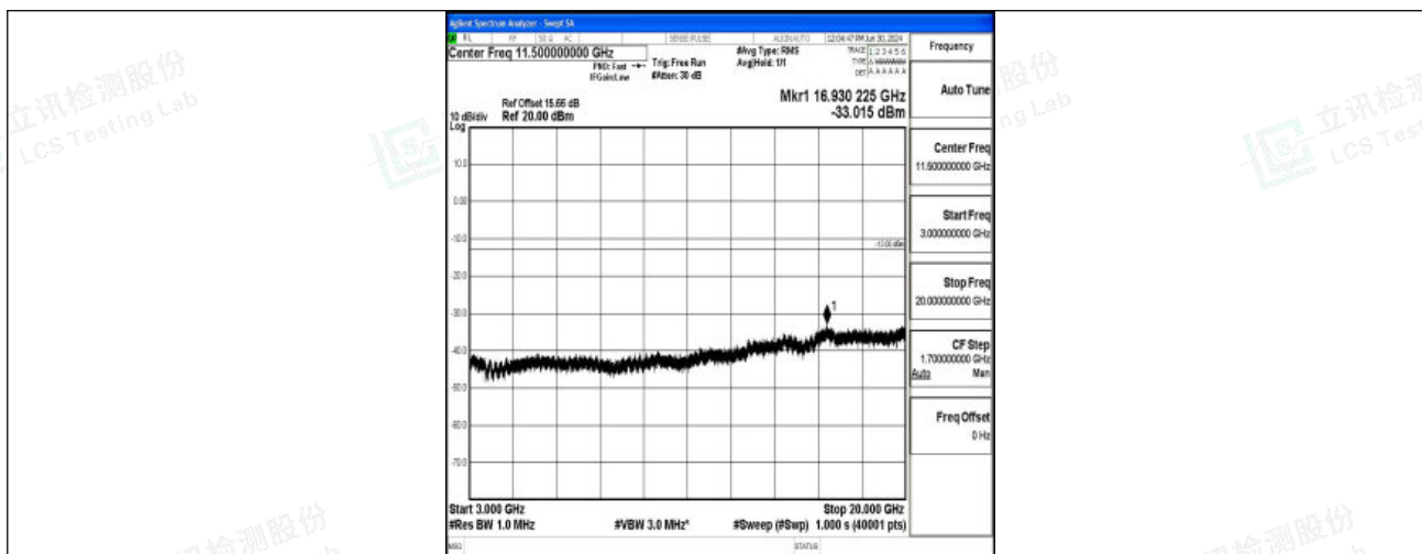
Band2_20MHz_QPSK_18900_1RB#0_3000~20000_3000~20000
