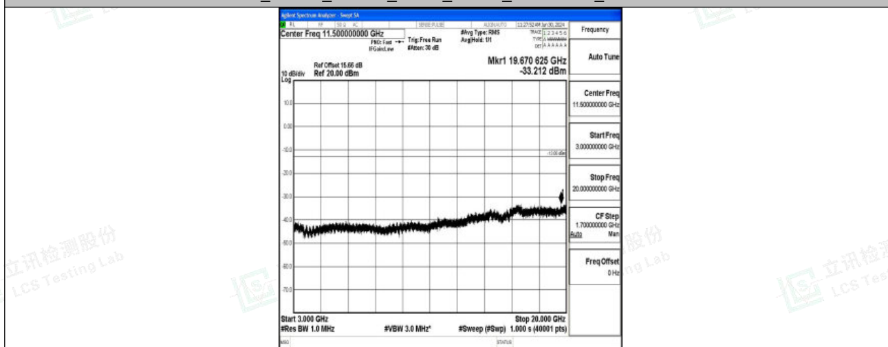
Band2_10MHz_16QAM_18650_1RB#0_3000~20000_3000~20000
