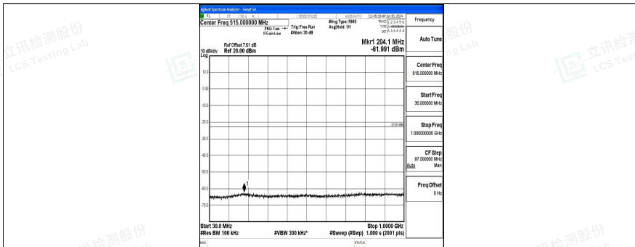
Band2_15MHz_QPSK_18675_1RB#0_30~1000_30~1000
