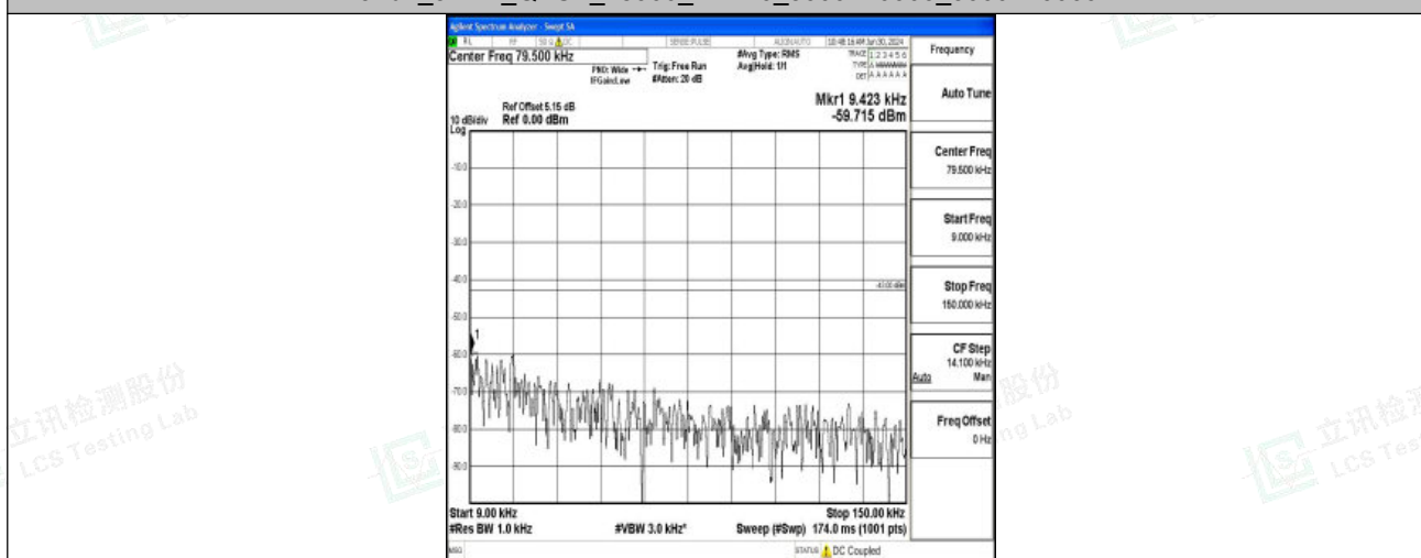
Band2_3MHz_16QAM_18900_1RB#0_0.009~0.15_0.009~0.15
