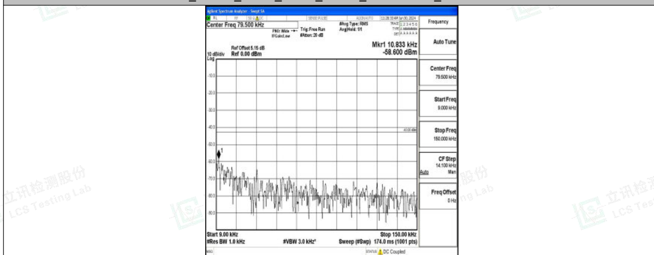
Band2_10MHz_16QAM_18900_1RB#0_0.009~0.15_0.009~0.15
