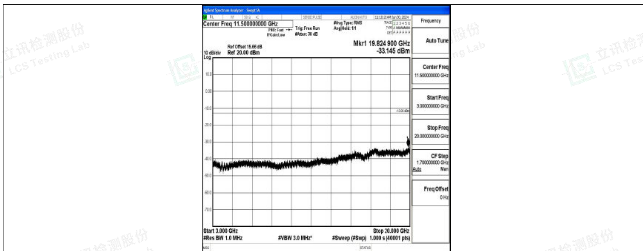
Band2_5MHz_16QAM_19175_1RB#0_3000~20000_3000~20000
