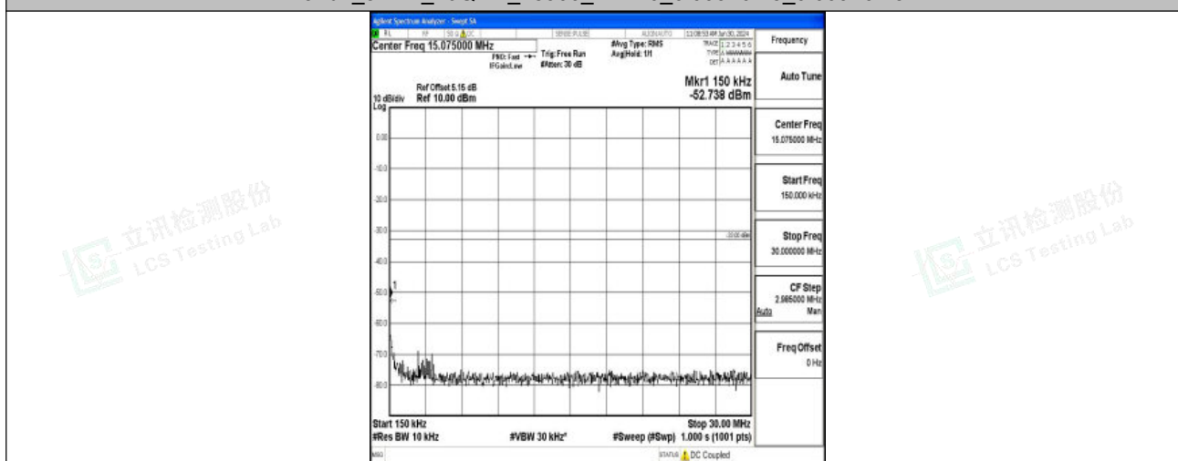
Band2_5MHz_16QAM_18900_1RB#0_0.15~30_0.15~30
