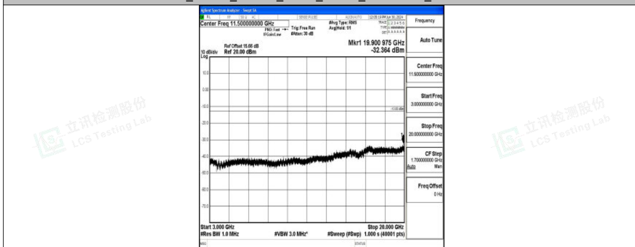
Band2_20MHz_16QAM_18900_1RB#0_3000~20000_3000~20000
