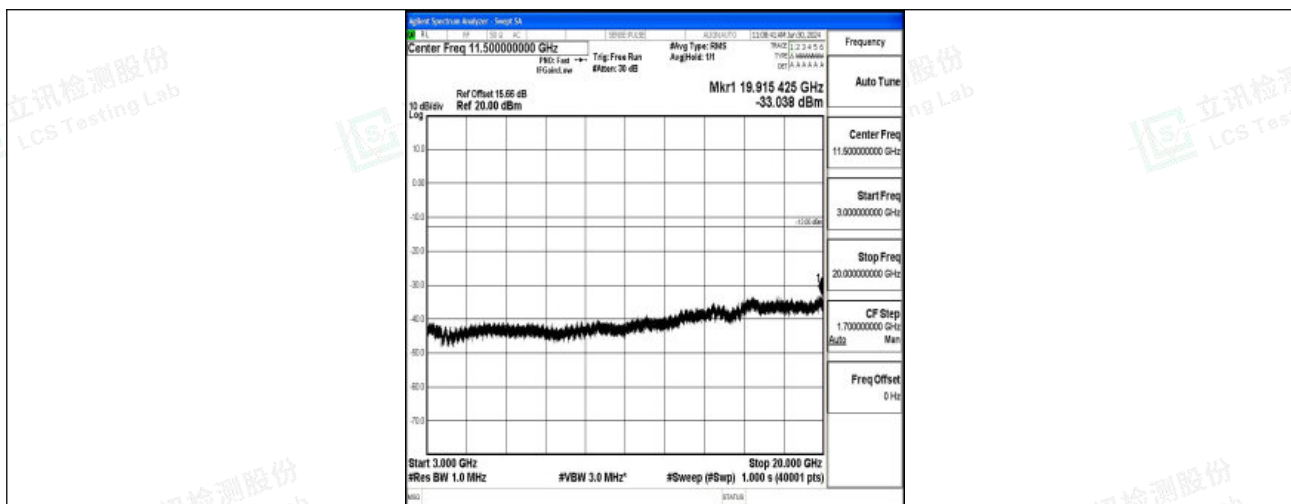
Band2_5MHz_QPSK_18900_1RB#0_3000~20000_3000~20000
