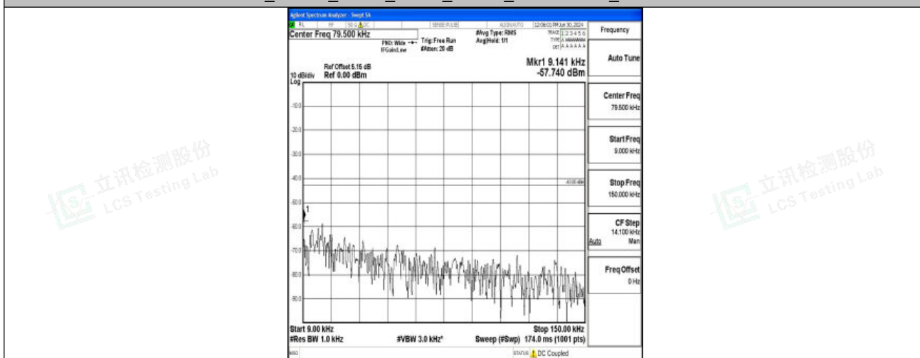
Band2_20MHz_16QAM_19100_1RB#0_0.009~0.15_0.009~0.15
