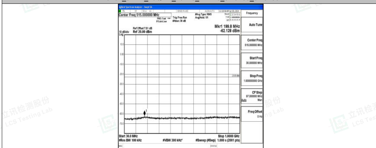
Band2_5MHz_16QAM_19175_1RB#0_30~1000_30~1000
