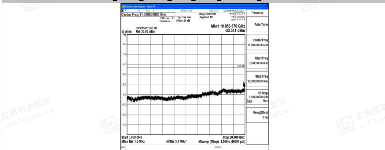
Band2_15MHz_16QAM_18675_1RB#0_3000~20000_3000~20000
