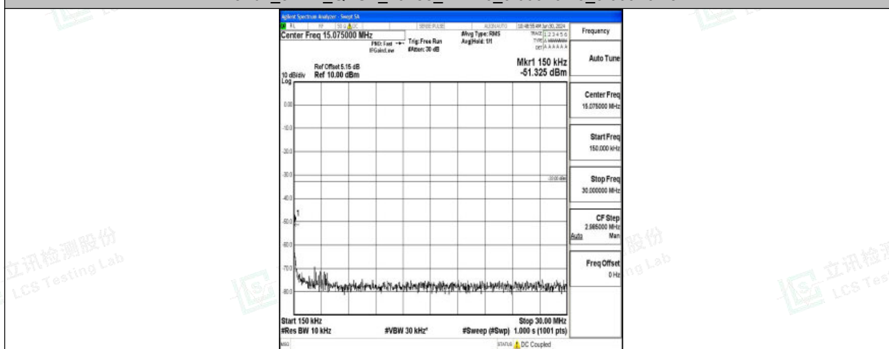
Band2_3MHz_QPSK_19185_1RB#0_0.15~30_0.15~30
