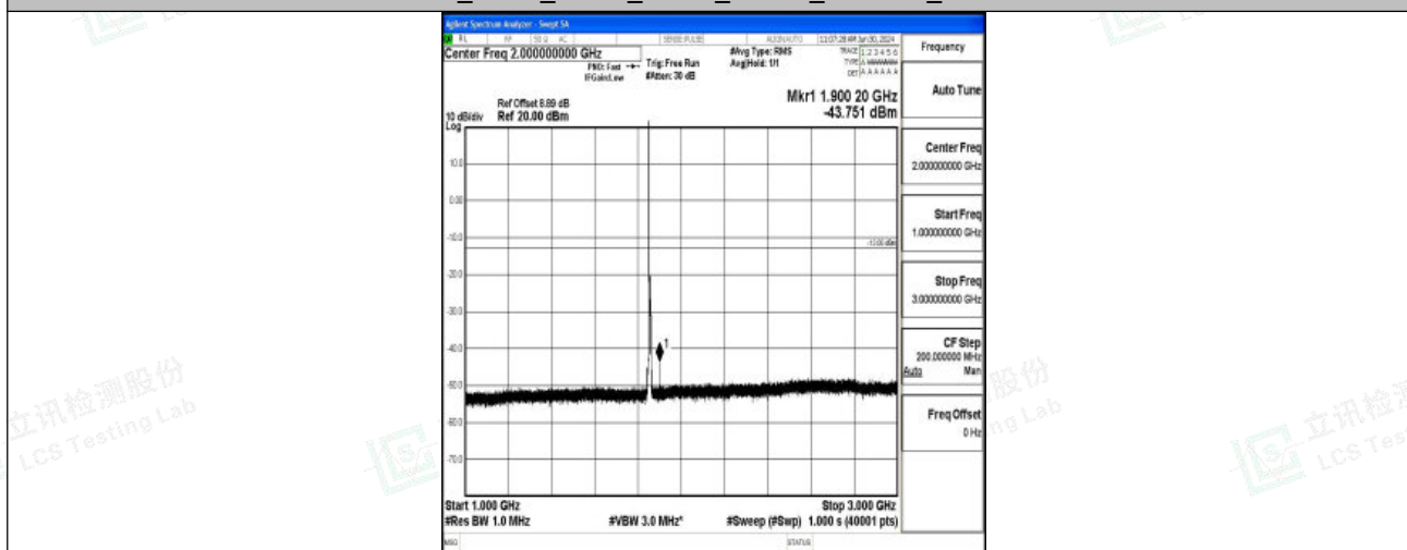
Band2_5MHz_QPSK_18625_1RB#0_1000~3000_1000~3000
