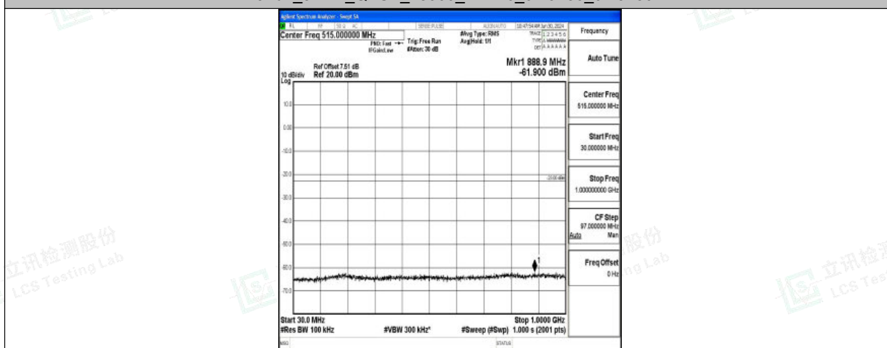
Band2_3MHz_QPSK_18900_1RB#0_30~1000_30~1000
