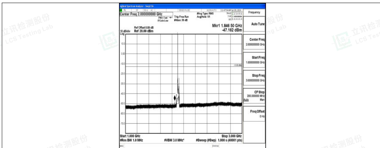
Band2_15MHz_QPSK_19125_1RB#0_1000~3000_1000~3000
