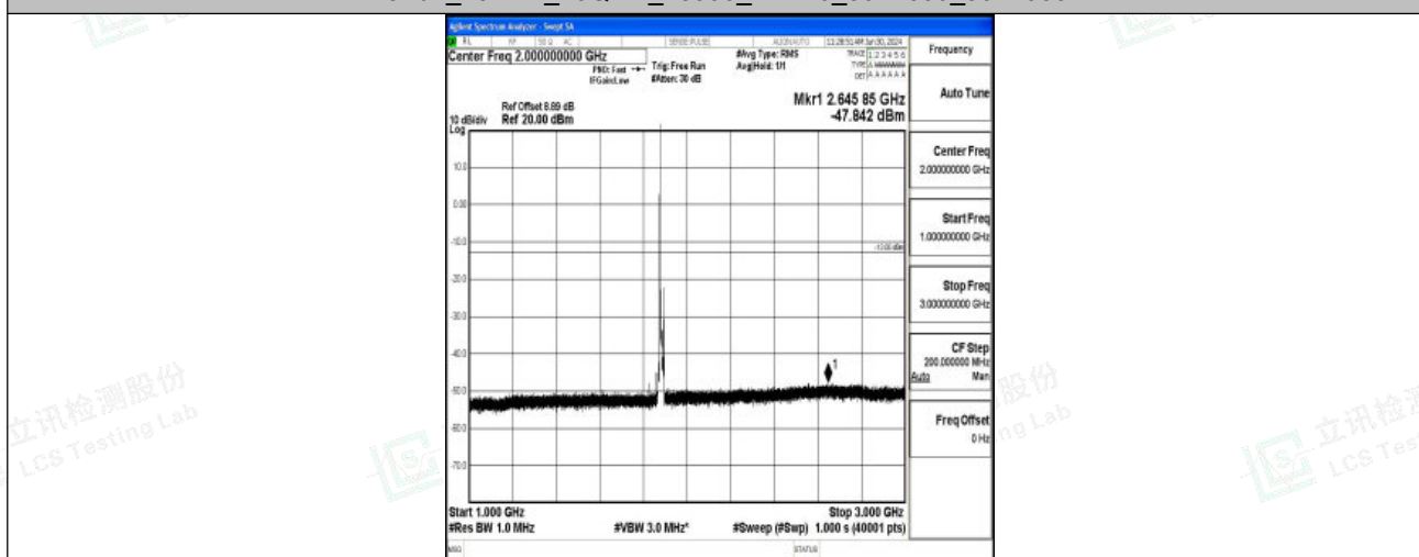
Band2_10MHz_16QAM_18900_1RB#0_1000~3000_1000~3000
