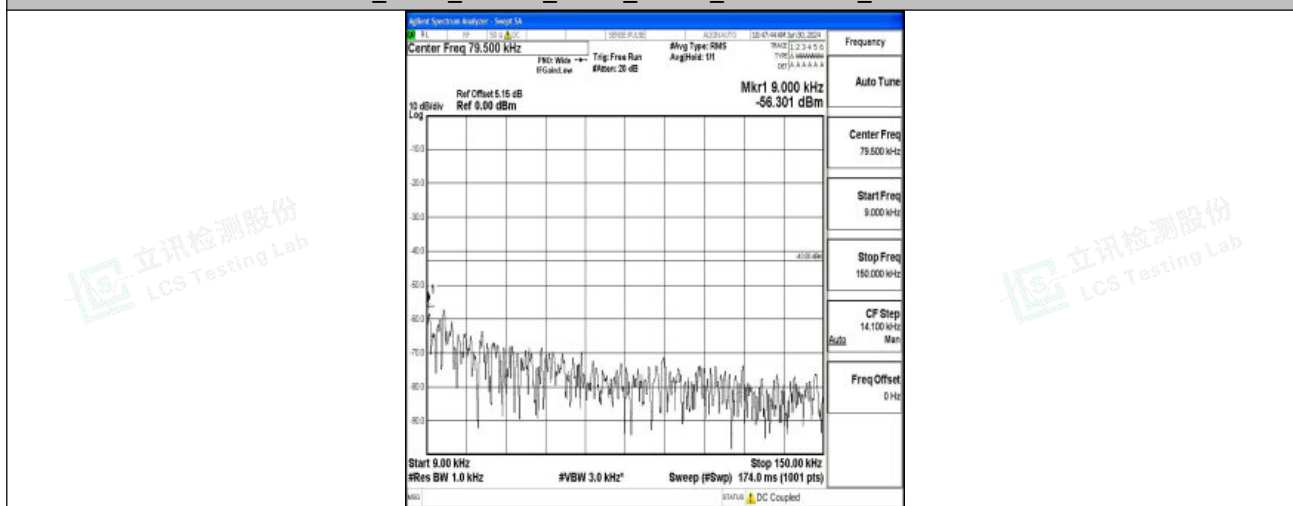
Band2_3MHz_QPSK_18900_1RB#0_0.009~0.15_0.009~0.15
