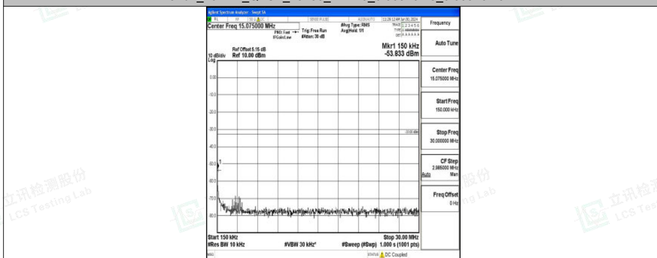
Band2_10MHz_QPSK_19150_1RB#0_0.15~30_0.15~30
