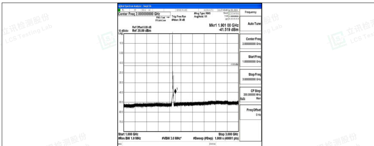
Band2_10MHz_16QAM_18650_1RB#0_1000~3000_1000~3000
