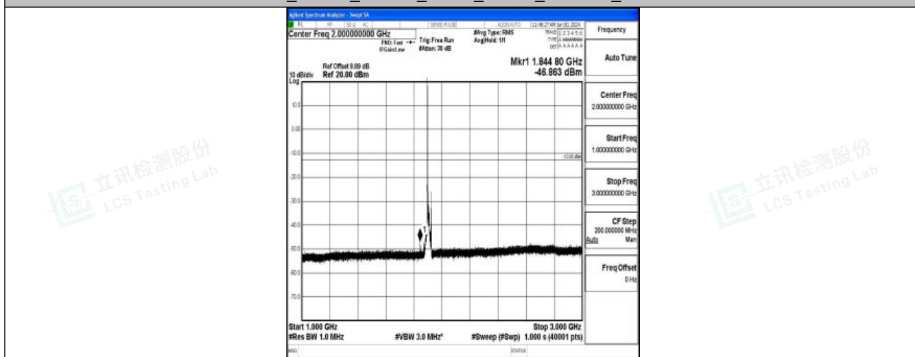
Band2_15MHz_16QAM_19125_1RB#0_1000~3000_1000~3000
