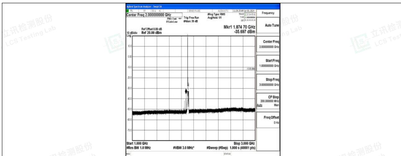
Band2_10MHz_QPSK_19150_1RB#0_1000~3000_1000~3000
