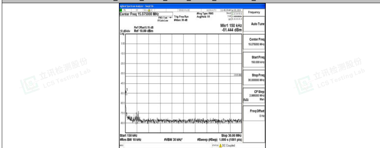
Band2_15MHz_QPSK_18675_1RB#0_0.15~30_0.15~30
