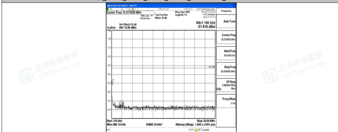
Band2_5MHz_QPSK_18625_1RB#0_0.15~30_0.15~30
