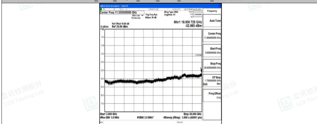
Band2_3MHz_16QAM_18615_1RB#0_3000~20000_3000~20000
