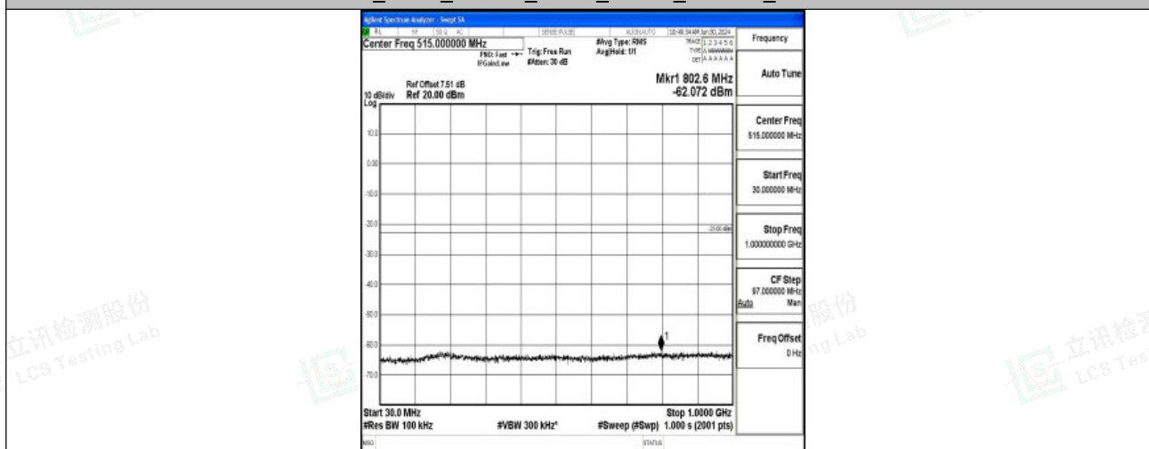
Band2_3MHz_16QAM_19185_1RB#0_30~1000_30~1000
