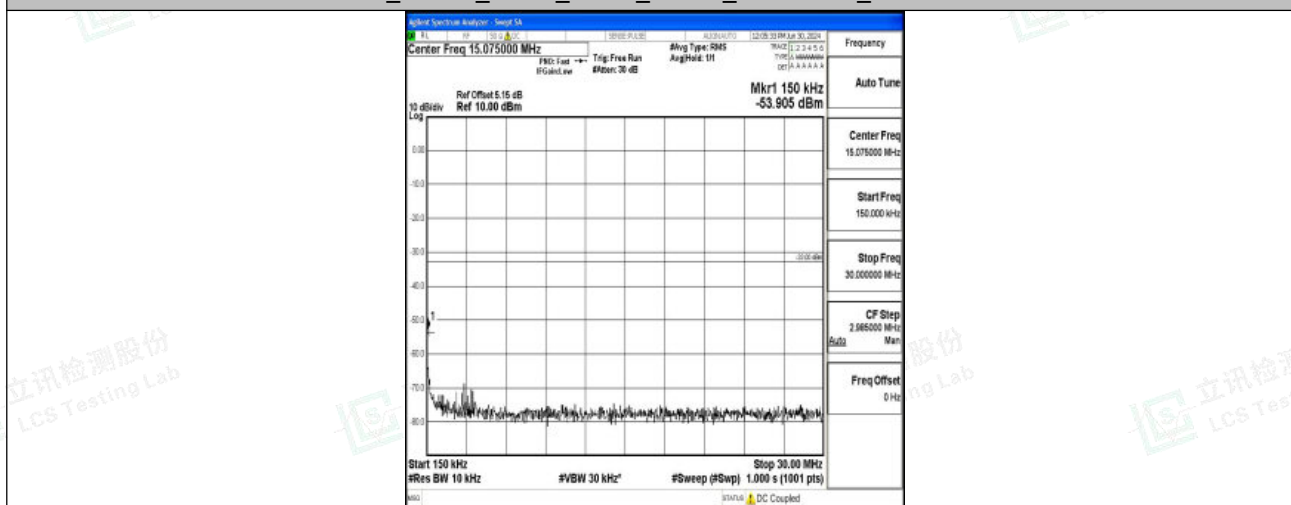
Band2_20MHz_QPSK_19100_1RB#0_0.15~30_0.15~30
