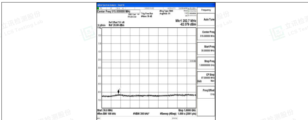
Band2_20MHz_16QAM_18900_1RB#0_30~1000_30~1000
