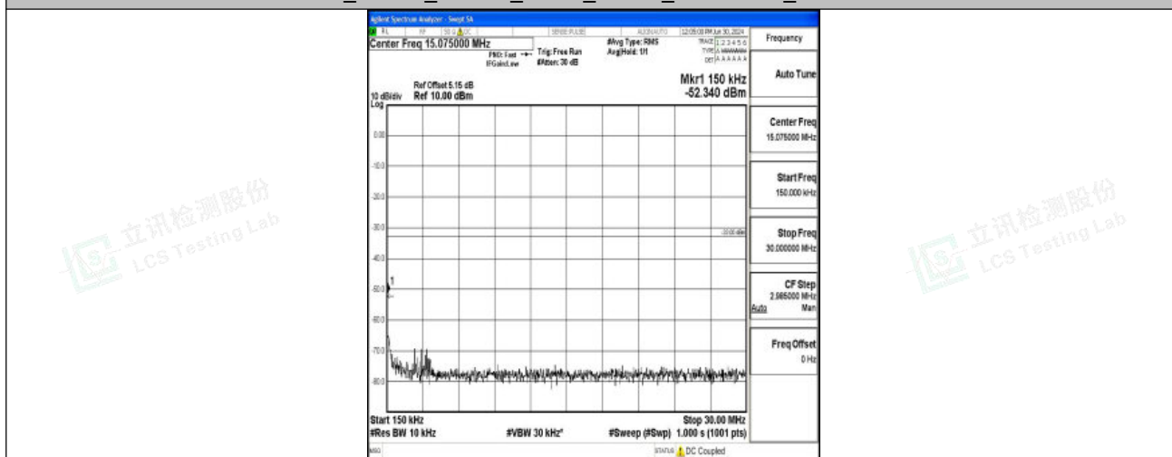
Band2_20MHz_16QAM_18900_1RB#0_0.15~30_0.15~30
