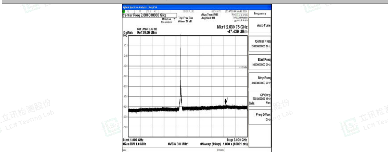
Band2_15MHz_16QAM_18900_1RB#0_1000~3000_1000~3000
