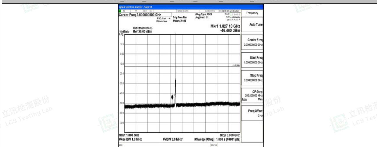
Band2_5MHz_16QAM_18900_1RB#0_1000~3000_1000~3000
