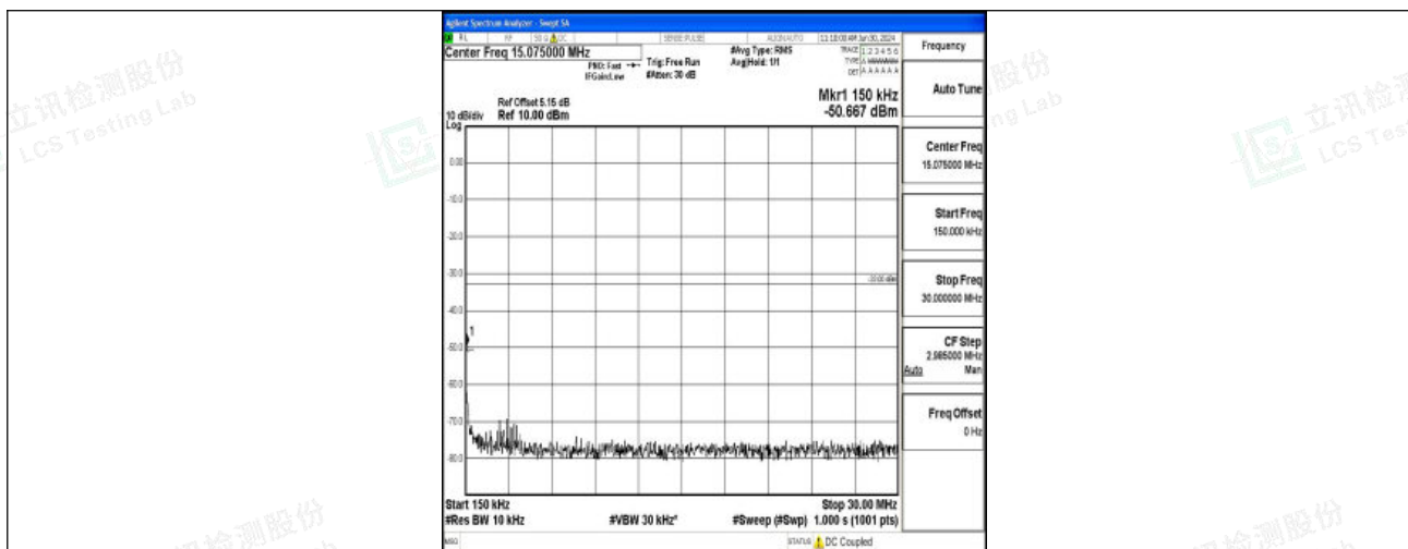
Band2_5MHz_16QAM_19175_1RB#0_0.15~30_0.15~30
