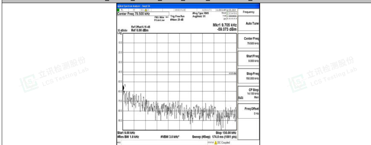
Band2_10MHz_QPSK_18900_1RB#0_0.009~0.15_0.009~0.15
