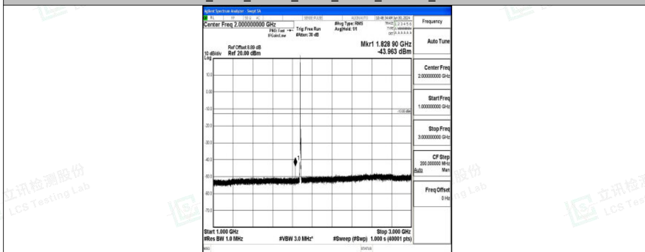
Band2_3MHz_16QAM_18900_1RB#0_1000~3000_1000~3000
