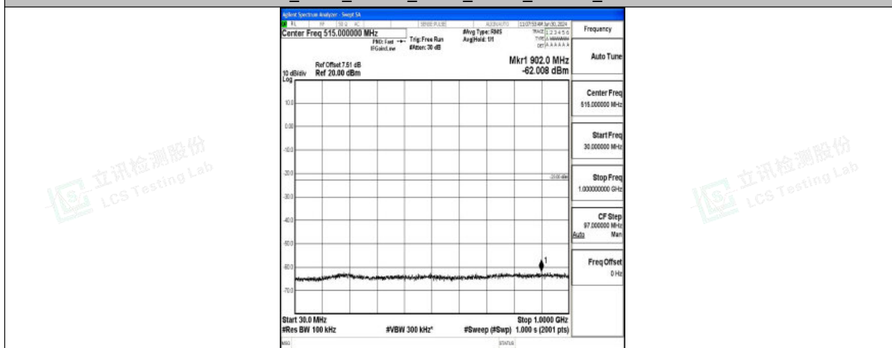
Band2_5MHz_16QAM_18625_1RB#0_30~1000_30~1000
