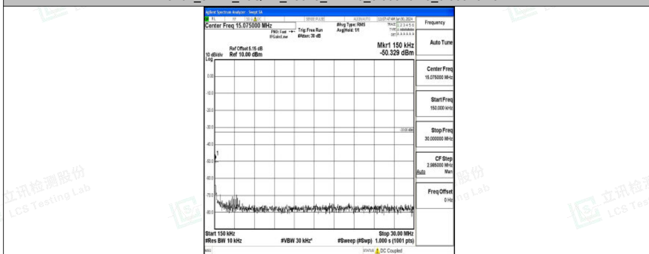
Band2_5MHz_16QAM_18625_1RB#0_0.15~30_0.15~30
