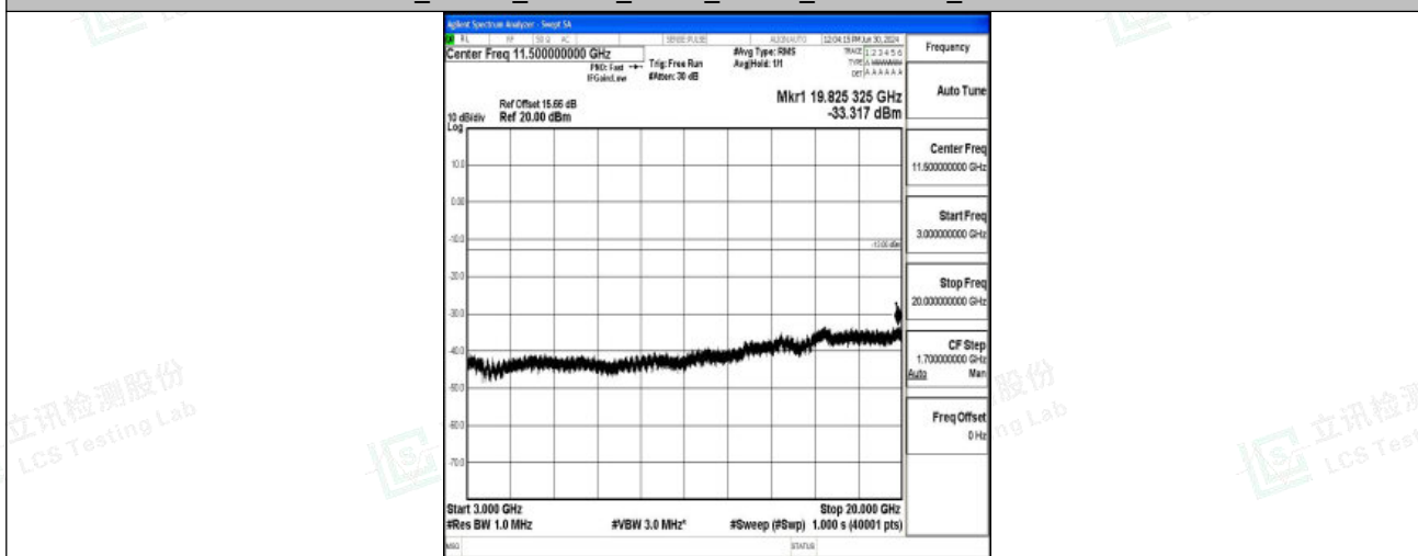
Band2_20MHz_16QAM_18700_1RB#0_3000~20000_3000~20000
