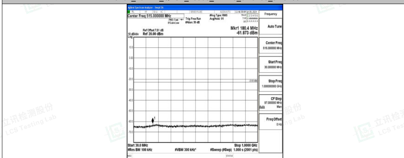
Band2_15MHz_QPSK_18900_1RB#0_30~1000_30~1000
