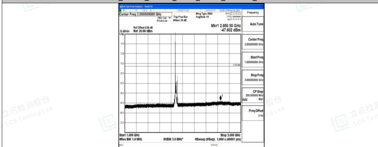
Band2_20MHz_16QAM_18900_1RB#0_1000~3000_1000~3000
