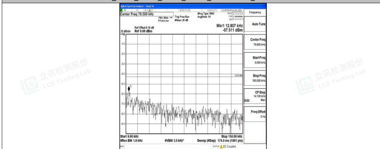
Band2_5MHz_16QAM_19175_1RB#0_0.009~0.15_0.009~0.15
