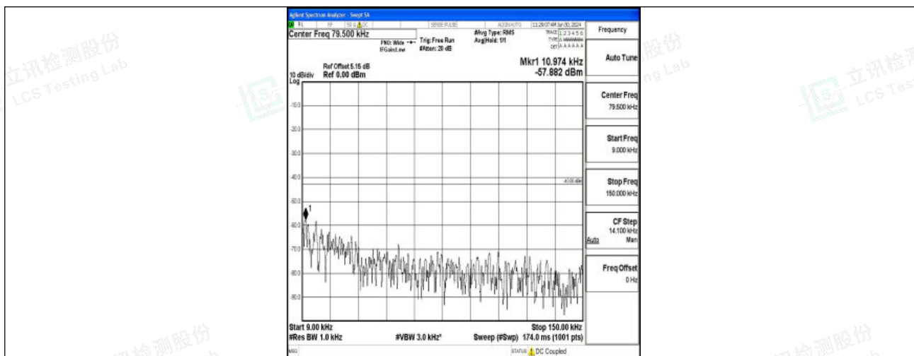
Band2_10MHz_QPSK_19150_1RB#0_0.009~0.15_0.009~0.15
