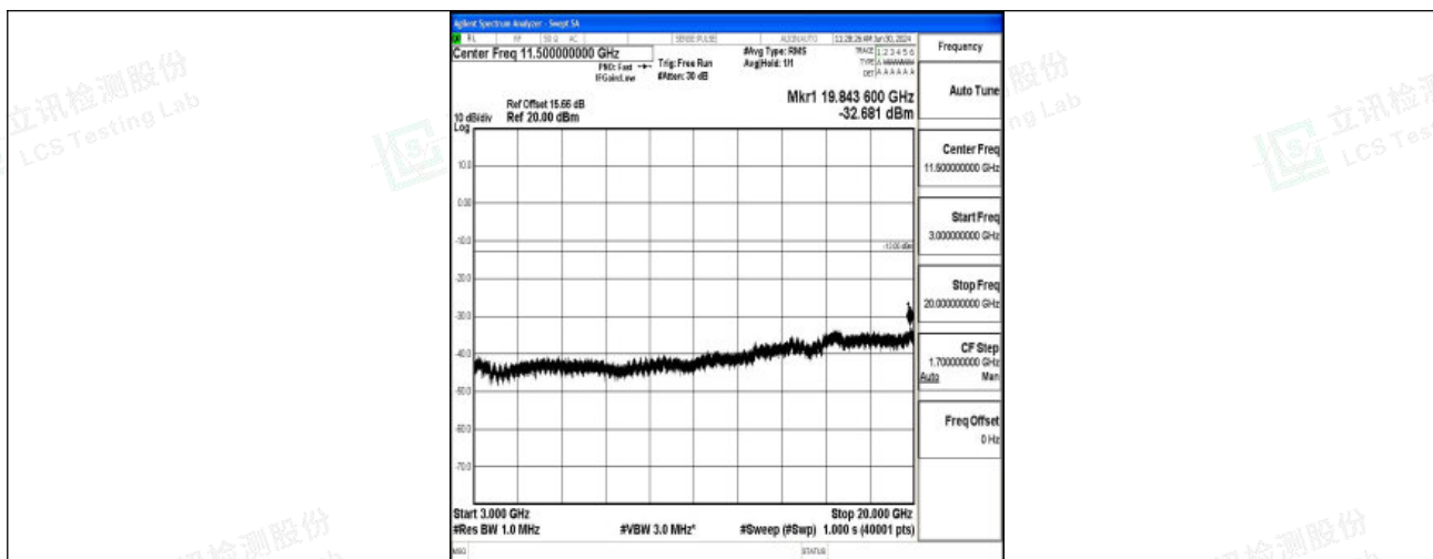
Band2_10MHz_QPSK_18900_1RB#0_3000~20000_3000~20000
