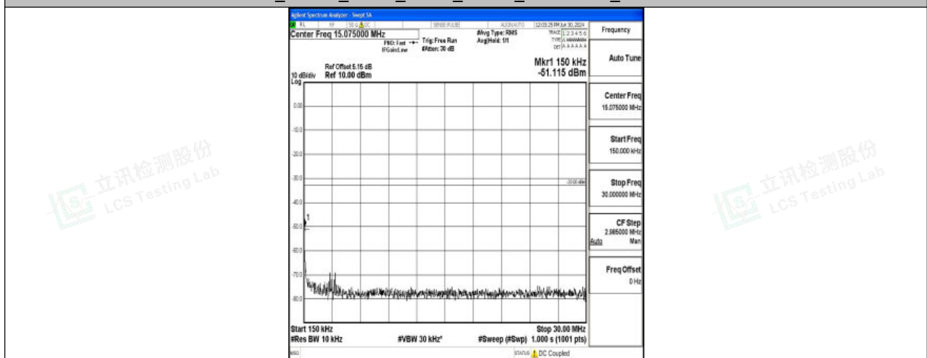
Band2_20MHz_QPSK_18700_1RB#0_0.15~30_0.15~30
