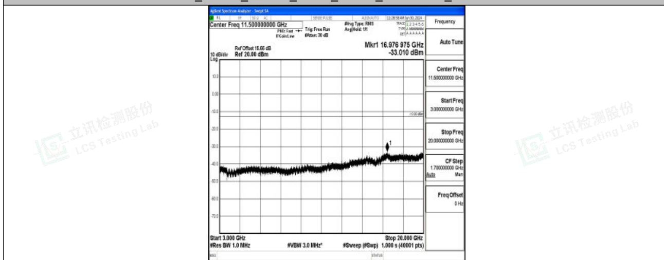
Band2_10MHz_16QAM_18900_1RB#0_3000~20000_3000~20000
