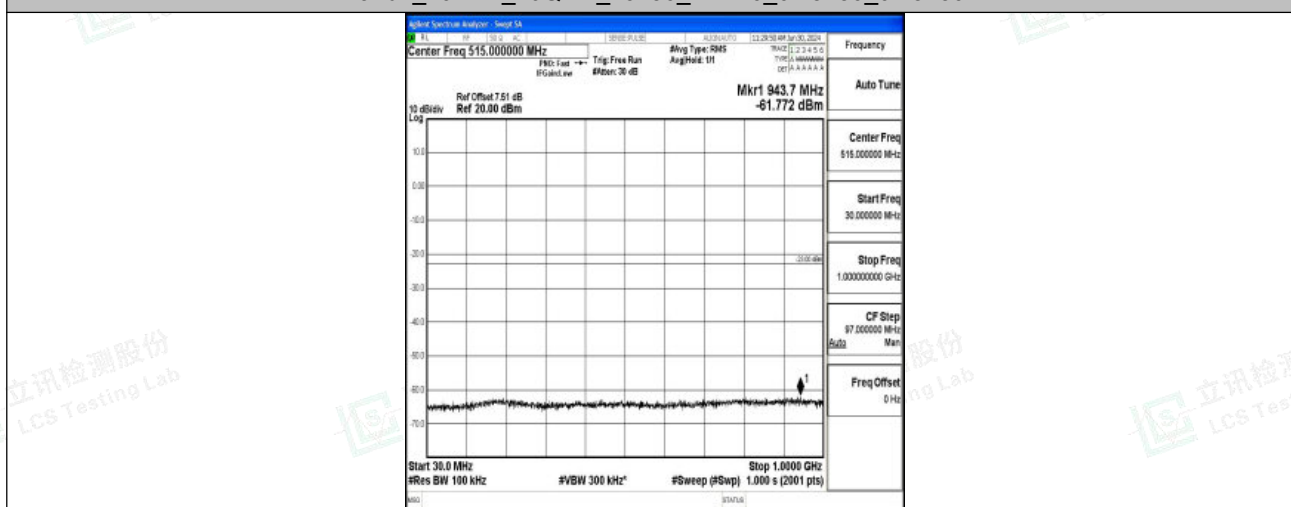
Band2_10MHz_16QAM_19150_1RB#0_30~1000_30~1000
