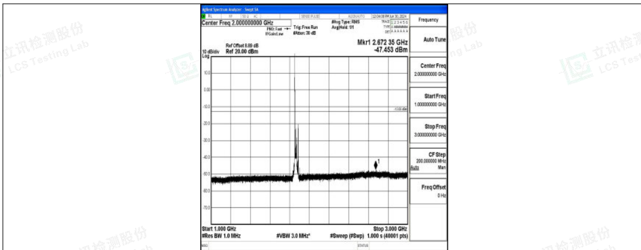
Band2_20MHz_16QAM_18700_1RB#0_1000~3000_1000~3000
