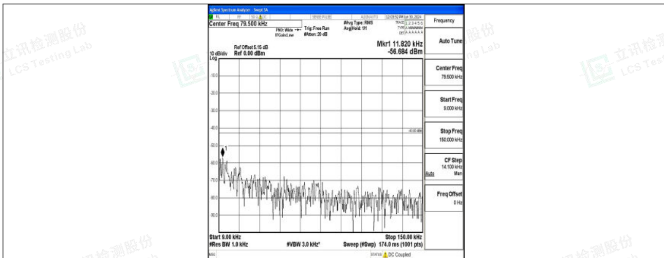
Band2_20MHz_16QAM_18700_1RB#0_0.009~0.15_0.009~0.15
