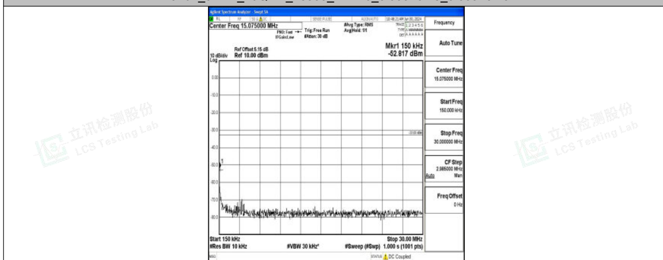
Band2_3MHz_16QAM_18900_1RB#0_0.15~30_0.15~30
