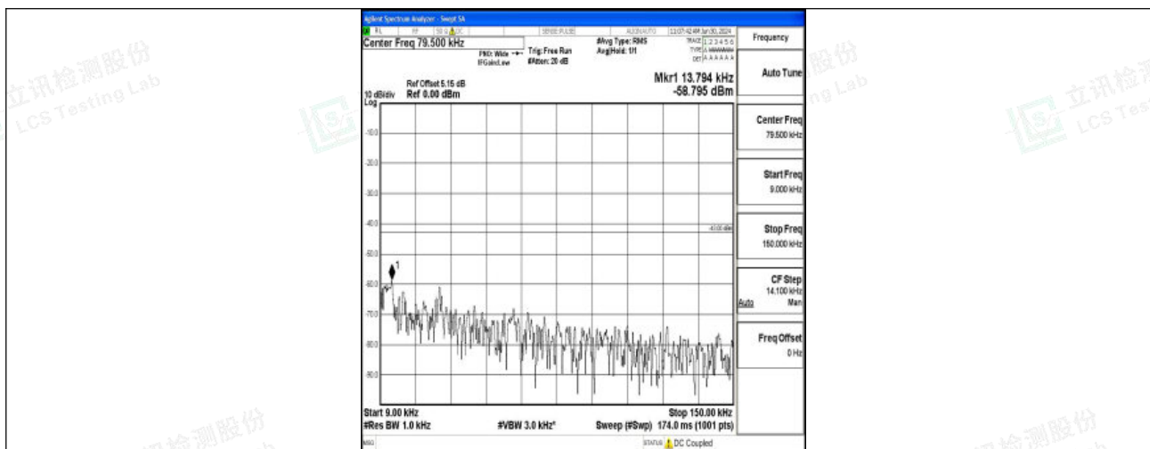
Band2_5MHz_16QAM_18625_1RB#0_0.009~0.15_0.009~0.15
