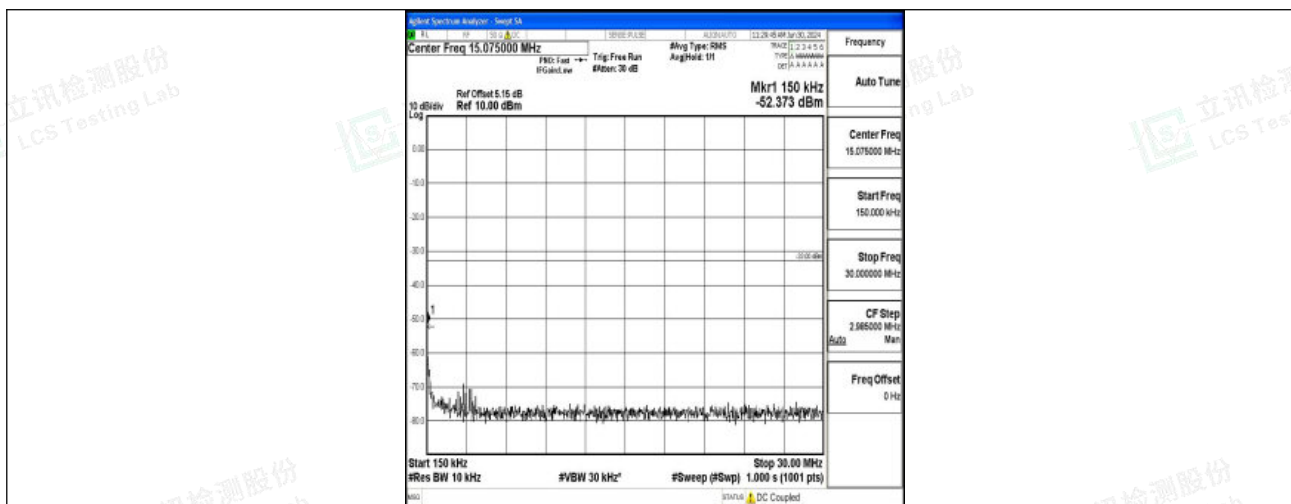
Band2_10MHz_16QAM_19150_1RB#0_0.15~30_0.15~30
