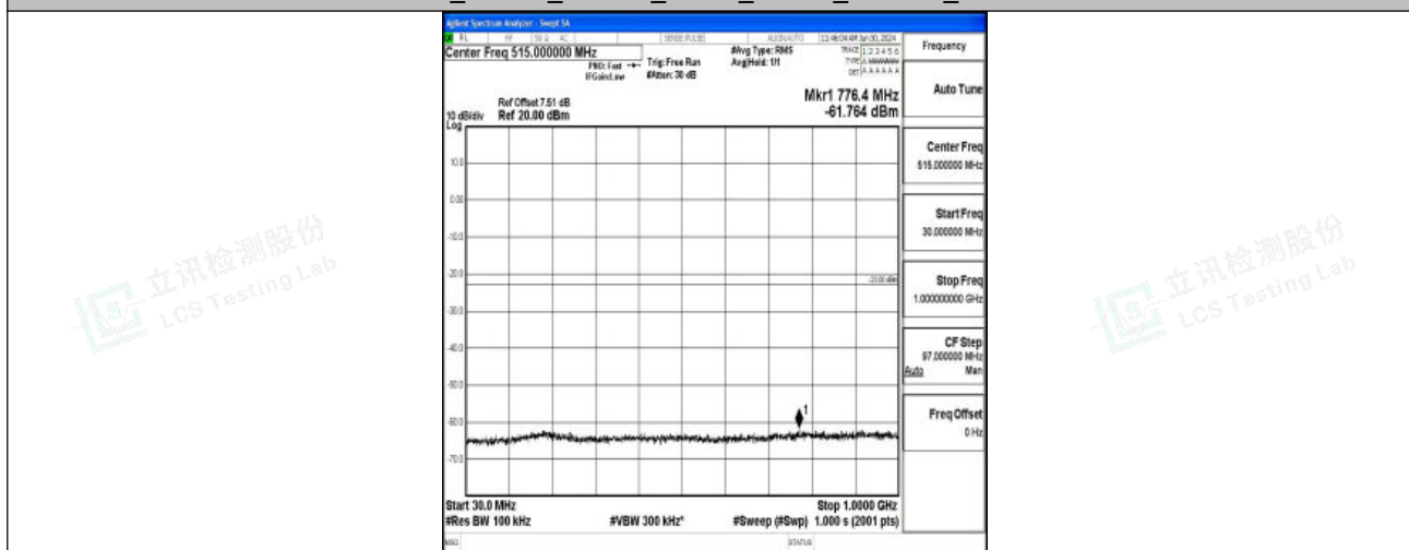
Band2_15MHz_16QAM_18675_1RB#0_30~1000_30~1000
