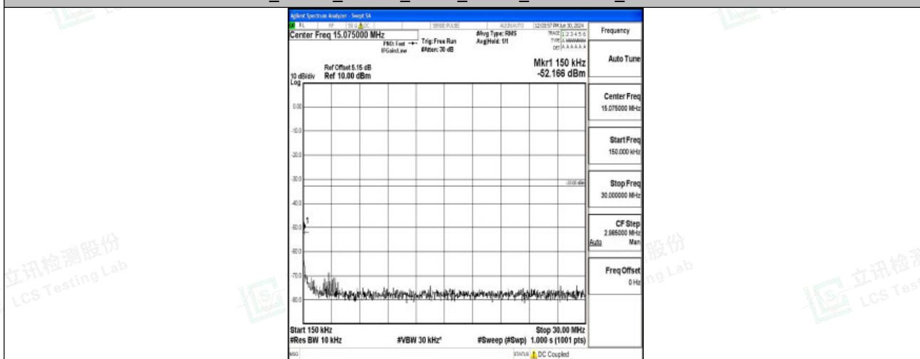
Band2_20MHz_16QAM_18700_1RB#0_0.15~30_0.15~30
