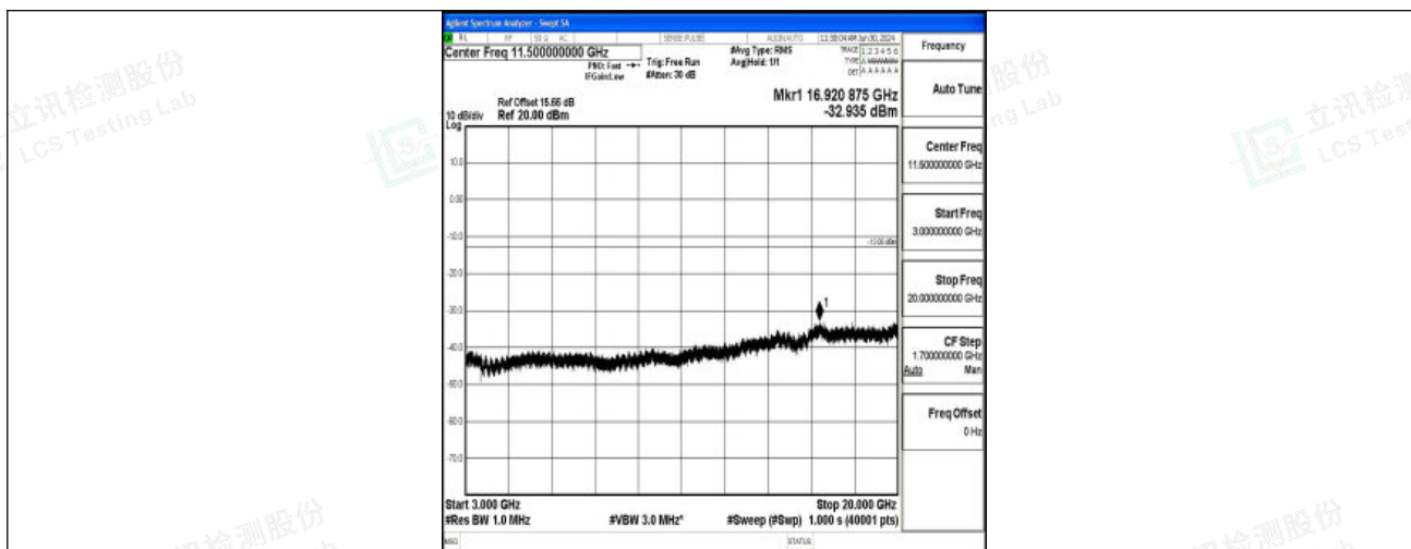
Band2_10MHz_16QAM_19150_1RB#0_3000~20000_3000~20000
