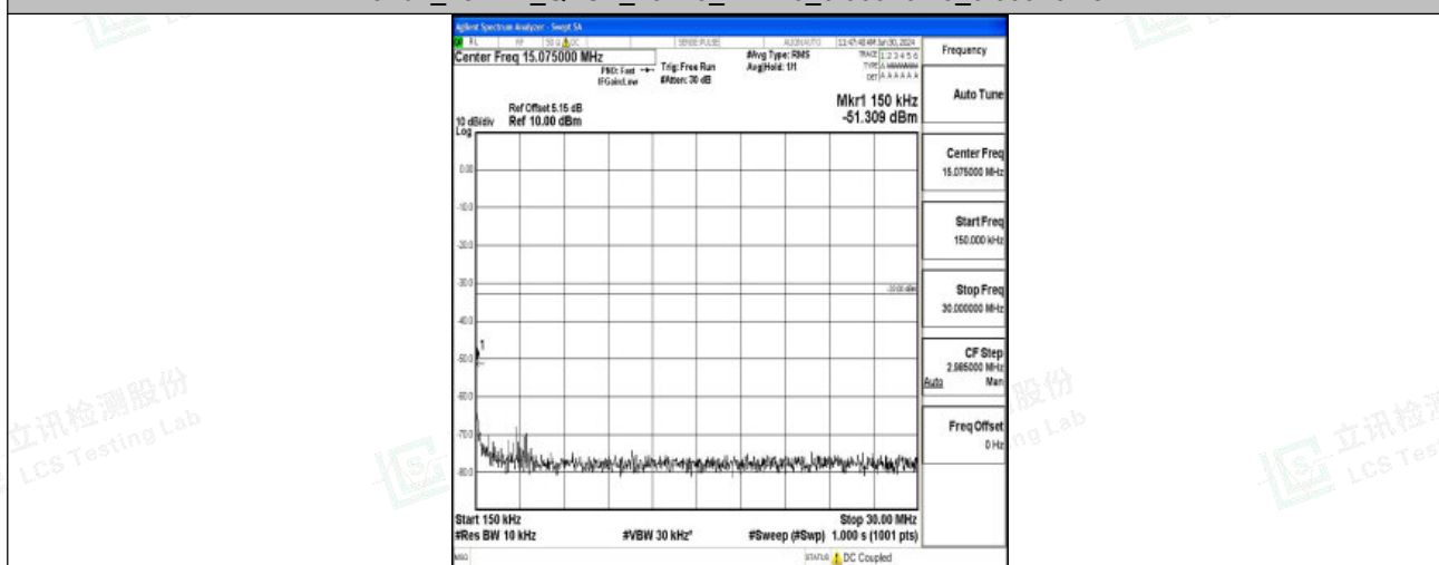
Band2_15MHz_QPSK_19125_1RB#0_0.15~30_0.15~30
