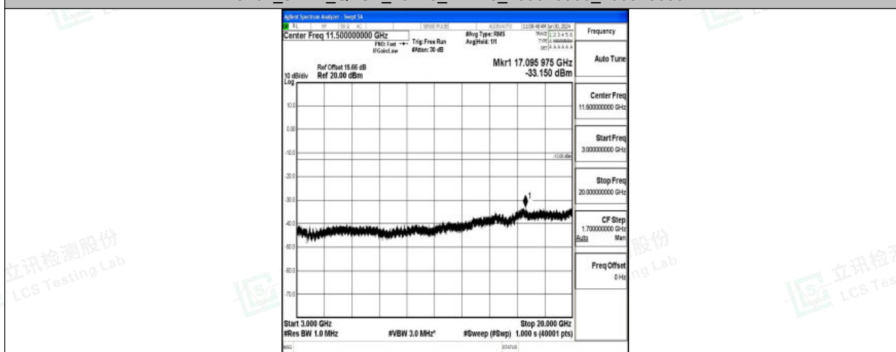
Band2_5MHz_QPSK_19175_1RB#0_3000~20000_3000~20000
