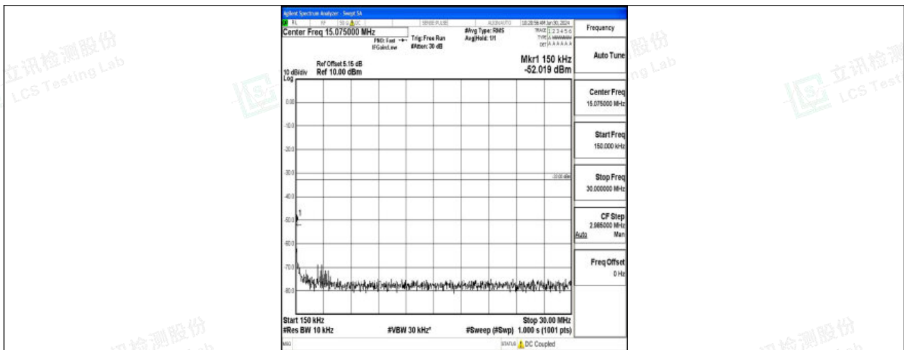
Band2_1.4MHz_16QAM_19193_1RB#0_0.15~30_0.15~30
