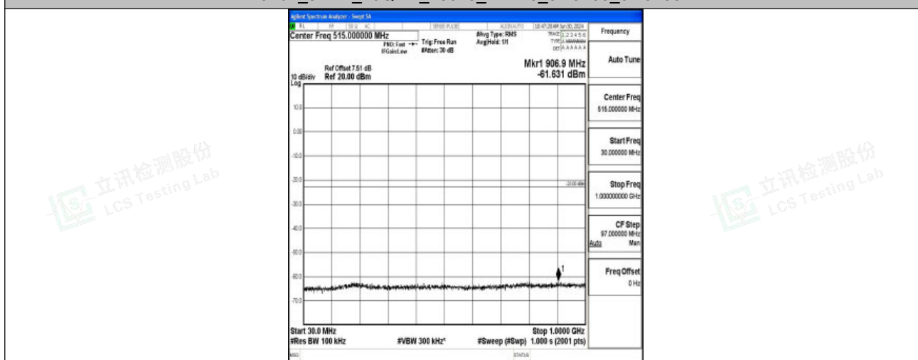
Band2_3MHz_16QAM_18615_1RB#0_30~1000_30~1000
