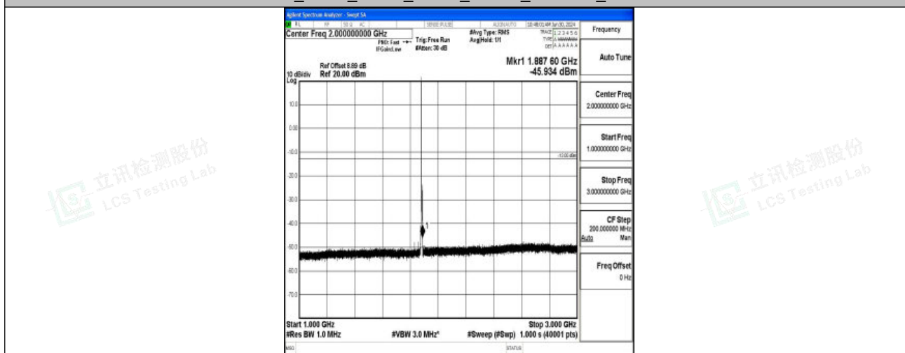
Band2_3MHz_QPSK_18900_1RB#0_1000~3000_1000~3000
