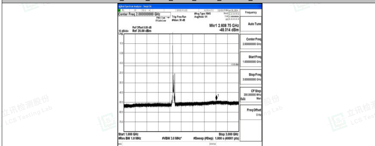
Band2_20MHz_QPSK_18700_1RB#0_1000~3000_1000~3000
