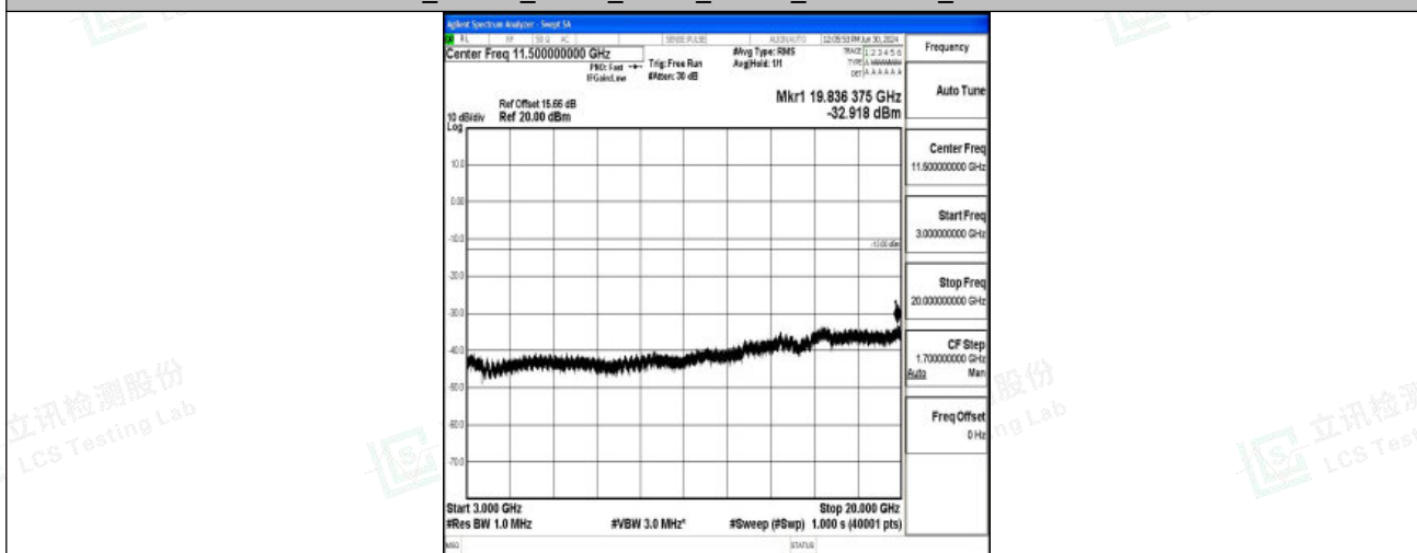
Band2_20MHz_QPSK_19100_1RB#0_3000~20000_3000~20000
