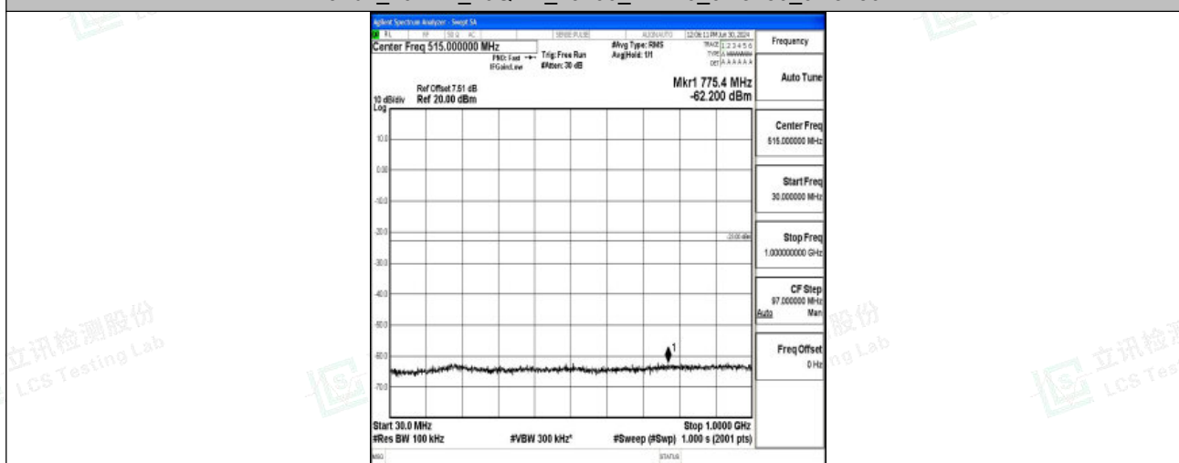
Band2_20MHz_16QAM_19100_1RB#0_30~1000_30~1000
