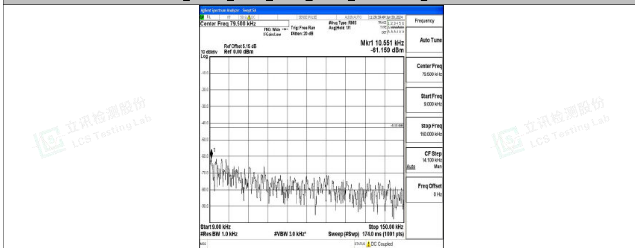
Band2_10MHz_16QAM_19150_1RB#0_0.009~0.15_0.009~0.15
