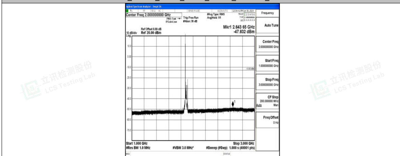
Band2_20MHz_QPSK_18900_1RB#0_1000~3000_1000~3000
