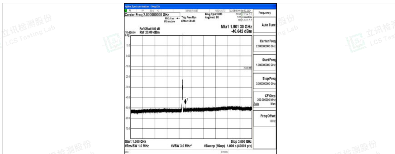
Band2_5MHz_16QAM_18625_1RB#0_1000~3000_1000~3000
