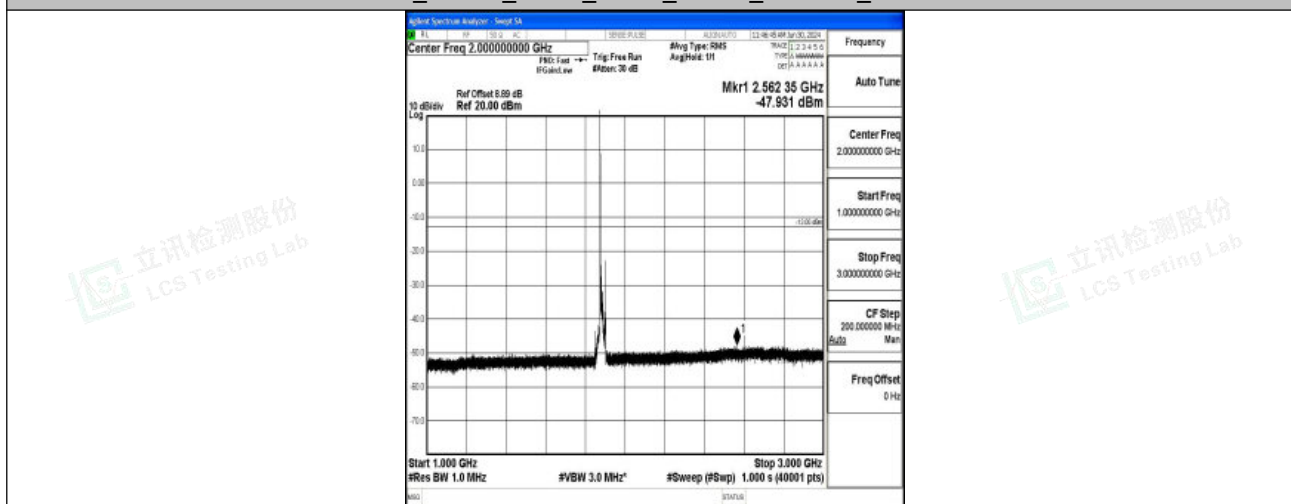
Band2_15MHz_QPSK_18900_1RB#0_1000~3000_1000~3000
