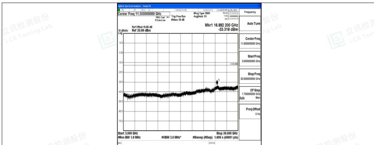
Band2_15MHz_QPSK_18900_1RB#0_3000~20000_3000~20000
