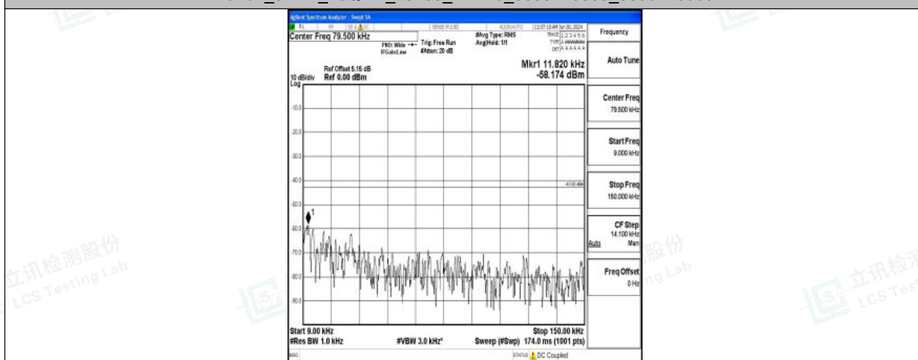
Band2_5MHz_QPSK_18625_1RB#0_0.009~0.15_0.009~0.15
