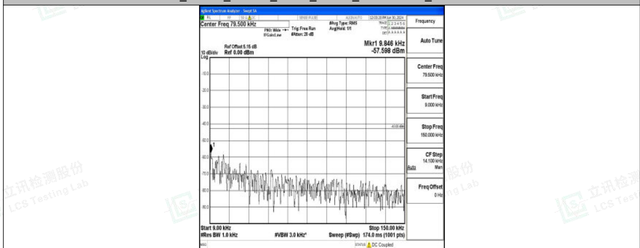
Band2_20MHz_QPSK_18700_1RB#0_0.009~0.15_0.009~0.15
