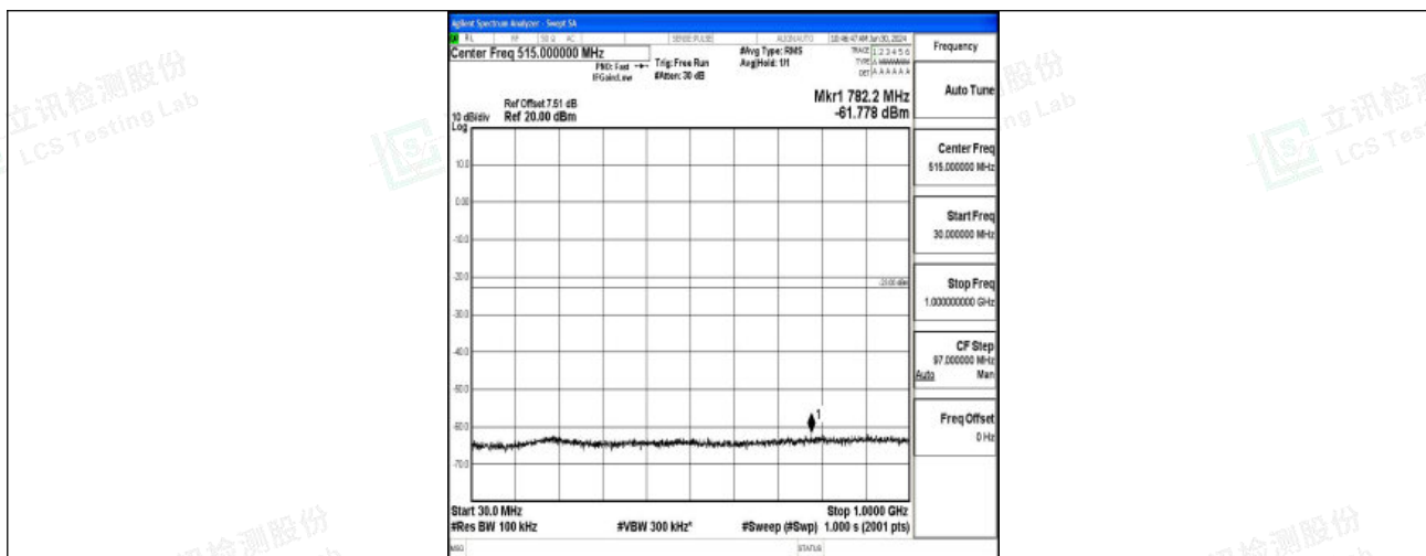
Band2_3MHz_QPSK_18615_1RB#0_30~1000_30~1000
