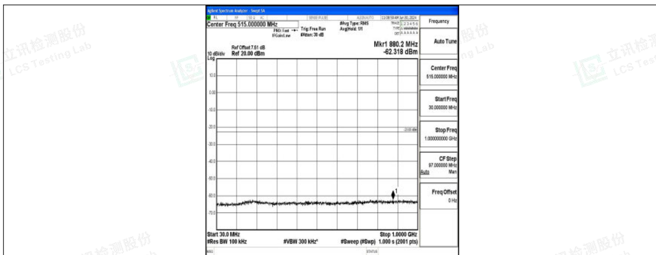
Band2_5MHz_16QAM_18900_1RB#0_30~1000_30~1000
