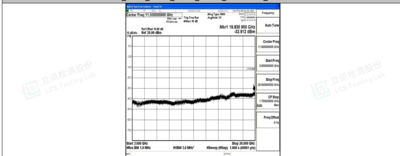
Band2_3MHz_QPSK_18615_1RB#0_3000~20000_3000~20000
