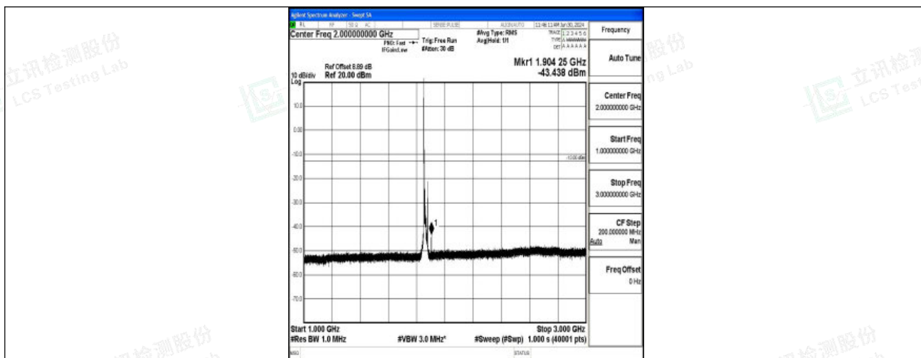
Band2_15MHz_16QAM_18675_1RB#0_1000~3000_1000~3000
