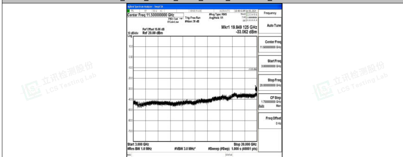
Band2_3MHz_16QAM_18900_1RB#0_3000~20000_3000~20000
