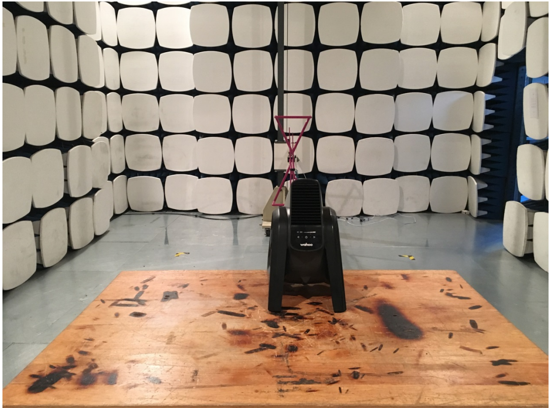
Radiated Emission
