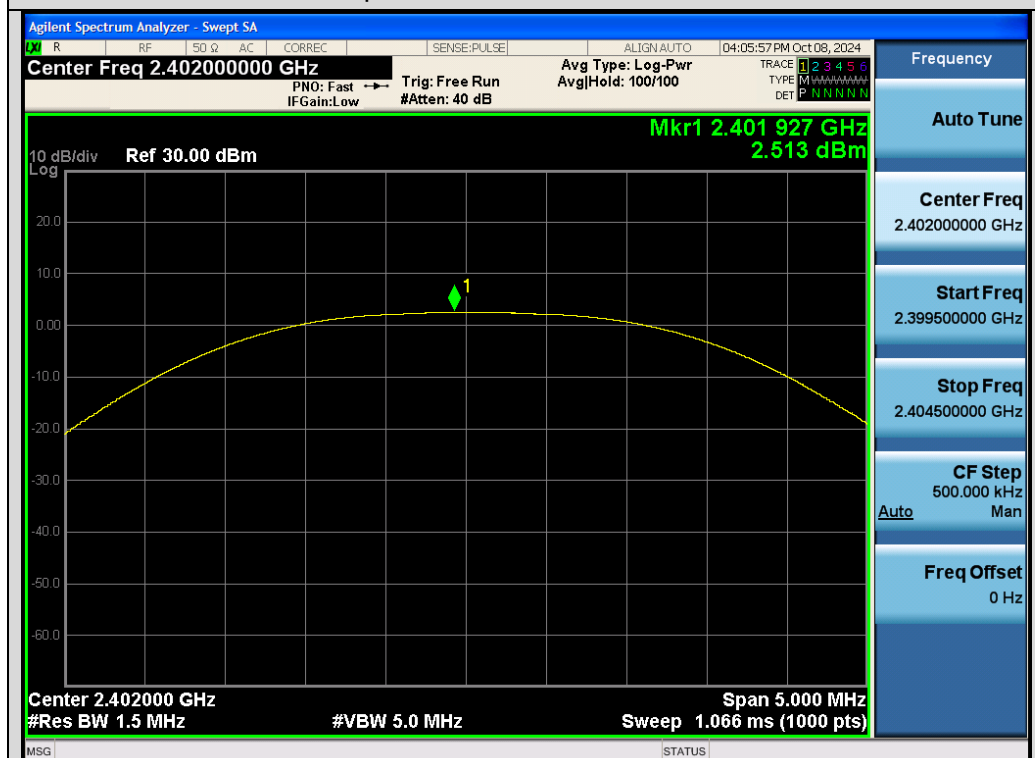
Test_Graph_2.4G_ANT2_2402_Peak Power
