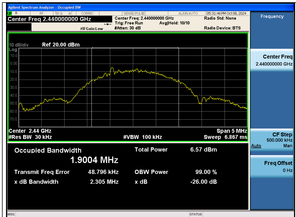
Test_Graph_2.4G_ANT1_2440_OBW
