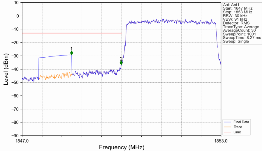
Band2_3MHz_16QAM_LCH_1851.5MHz_RB_15_0_NTNV
