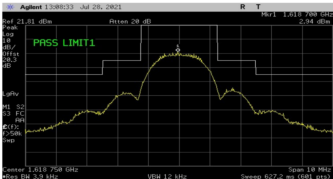
Plot 6 – Emission Mask - High Channel
