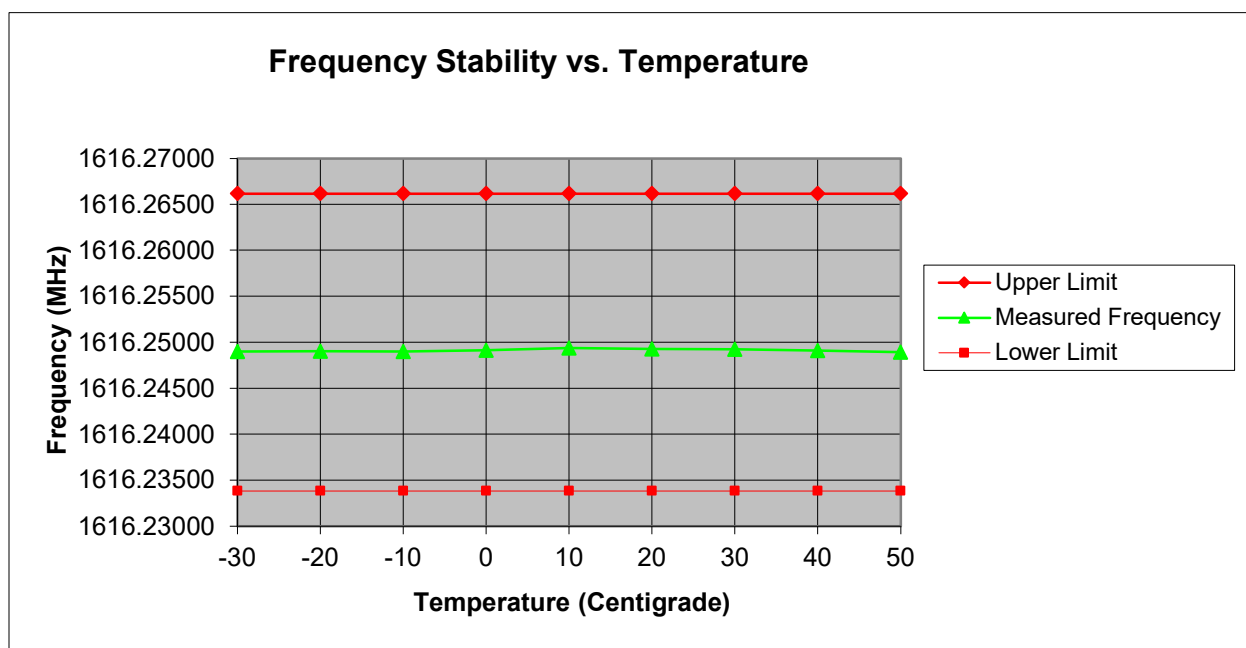
Plot 27 – Temperature vs Frequency
