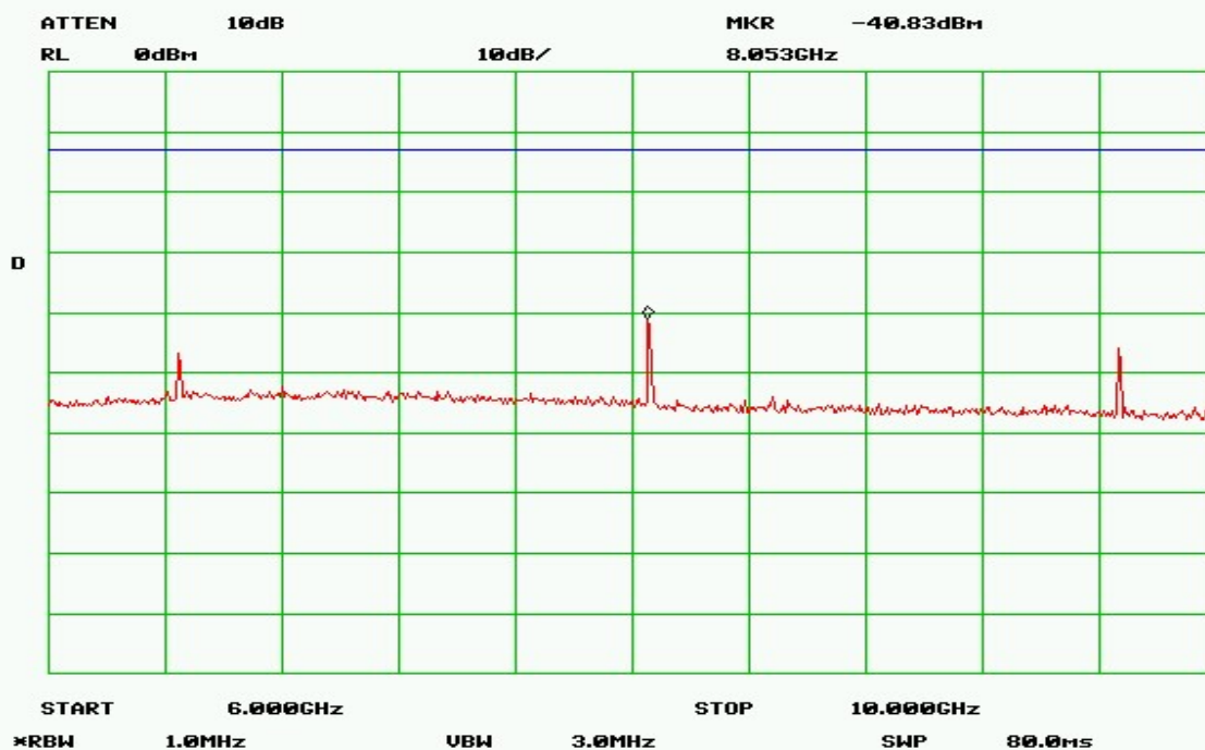
Plot 10 – Lowest Channel - 6GHz to 10 GHz
