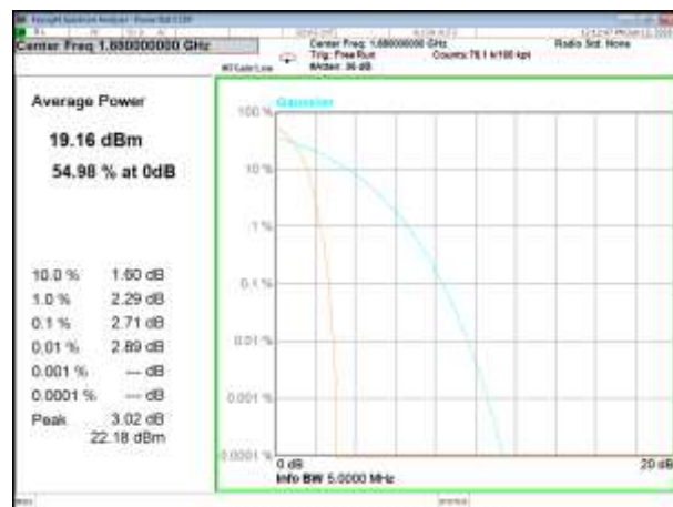
WCDMA B2_Middle
