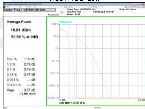
HSDPA B2_High
