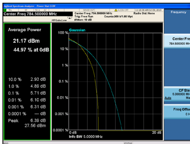
Band13 / 5MHz / High CH / 16QAM
