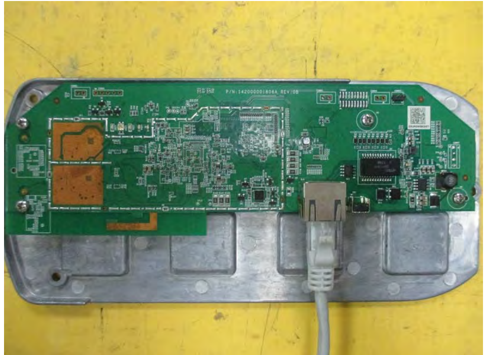
CLOSE-UP VIEW
