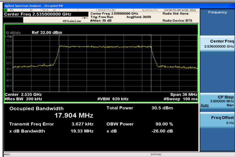
Band7-20MHz-QPSK-21100-100RB#0-17.904
