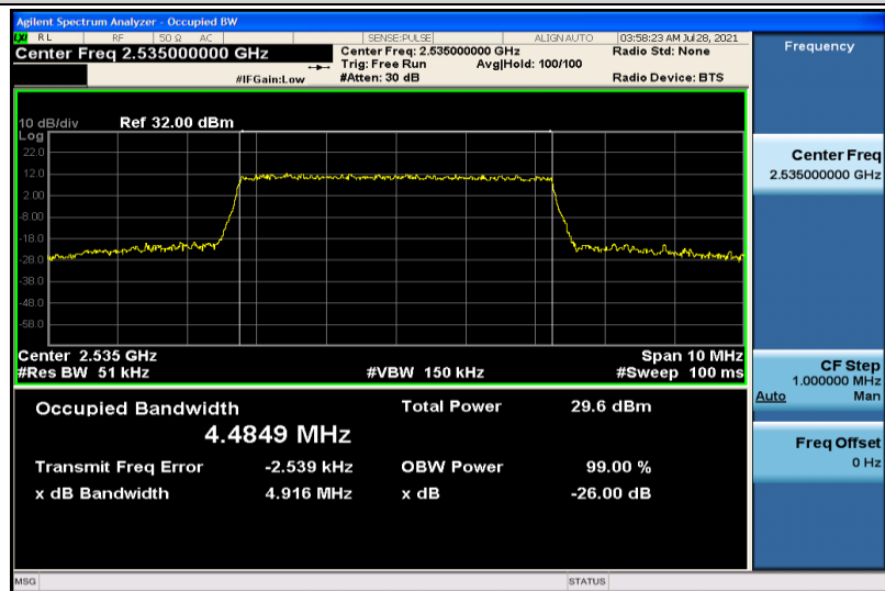
Band7-5MHz-16QAM-21100-25RB#0-4.4849
