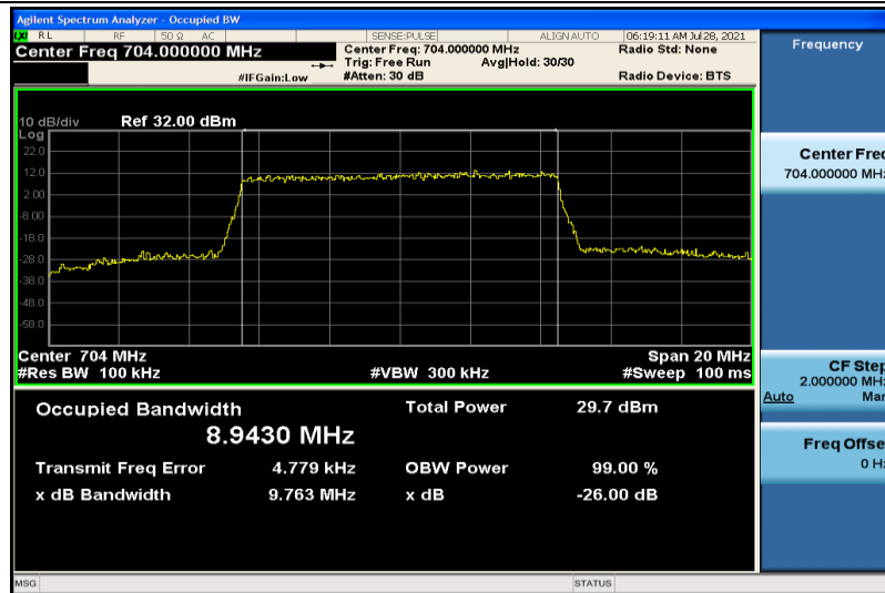
Band12-10MHz-16QAM-23060-50RB#0-8.9430
