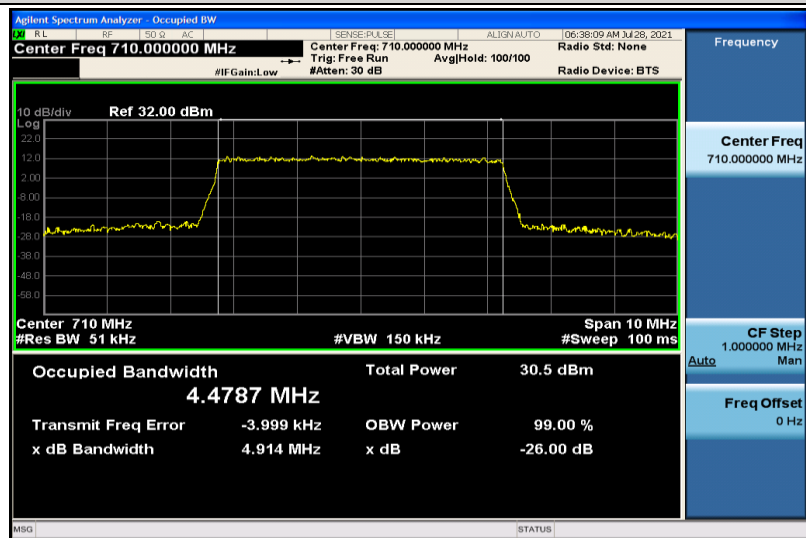
Band17-5MHz-QPSK-23790-25RB#0-4.4787
