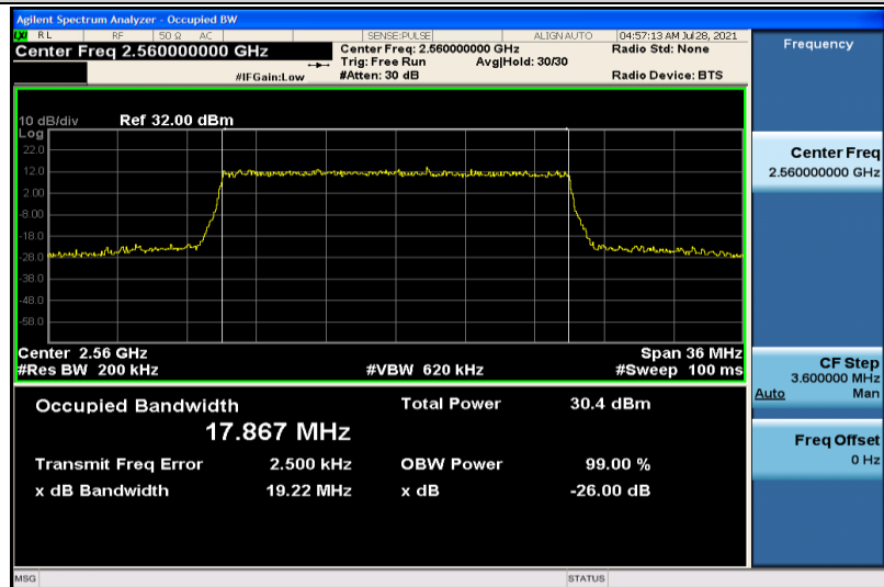
Band7-20MHz-QPSK-21350-100RB#0-17.867
