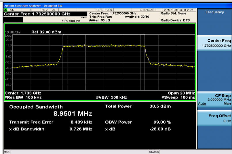
Band4-10MHz-QPSK-20175-50RB#0-8.9501
