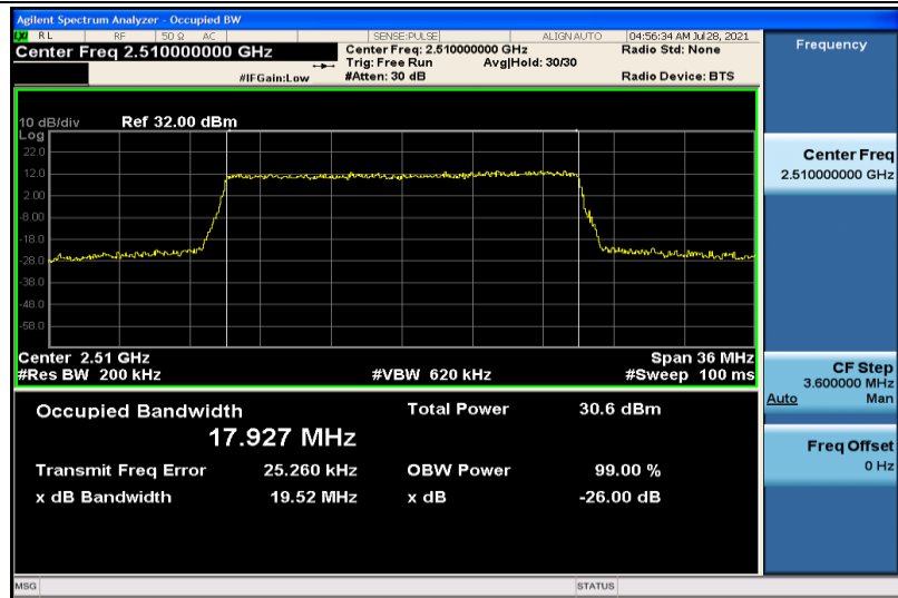
Band7-20MHz-QPSK-20850-100RB#0-17.927
