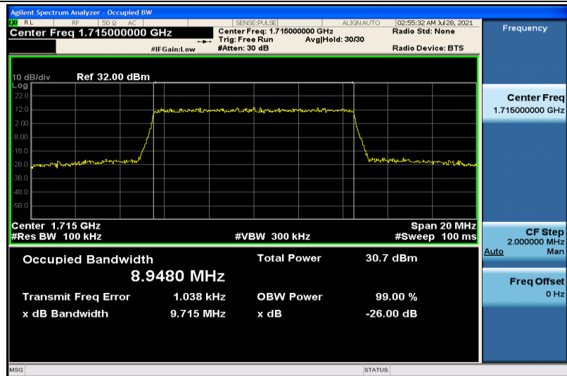
Band4-10MHz-QPSK-20000-50RB#0-8.9480
