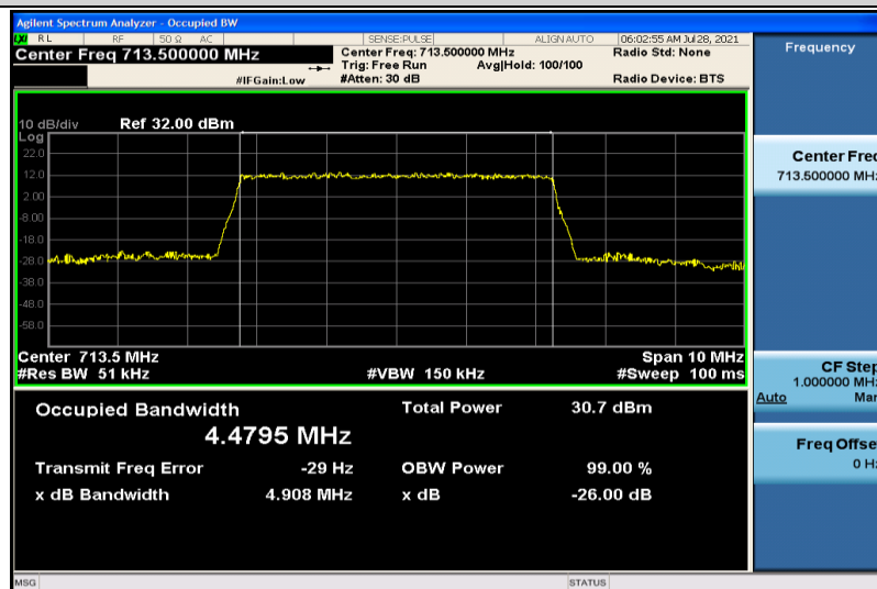
Band12-5MHz-QPSK-23155-25RB#0-4.4795
