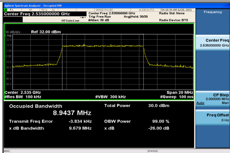
Band7-10MHz-QPSK-21100-50RB#0-8.9437
