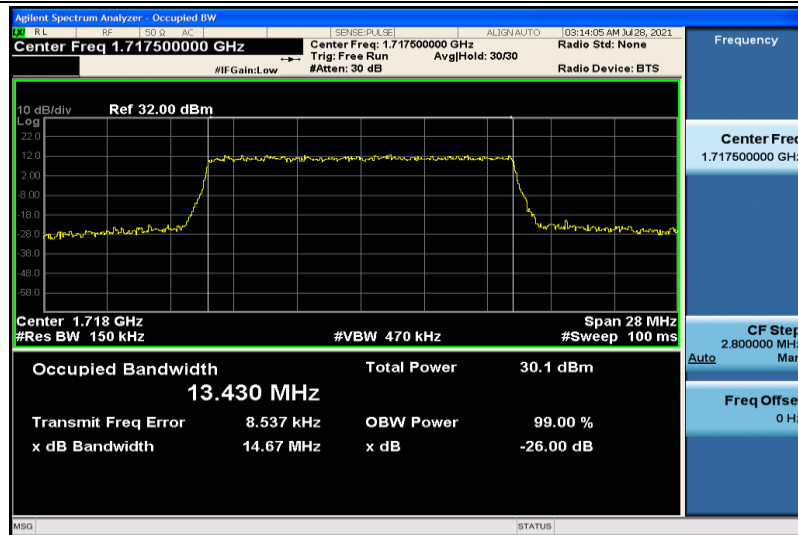
Band4-15MHz-16QAM-20025-75RB#0-13.430
