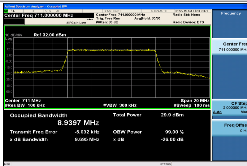
Band17-10MHz-16QAM-23800-50RB#0-8.9397
