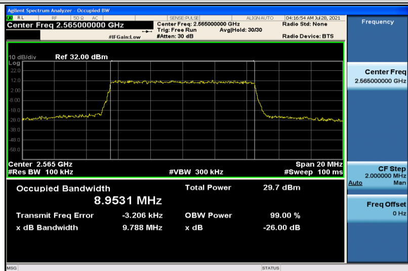
Band7-10MHz-QPSK-21400-50RB#0-8.9531
