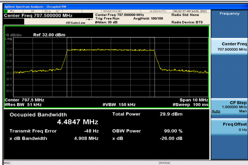
Band12-5MHz-16QAM-23095-25RB#0-4.4847
