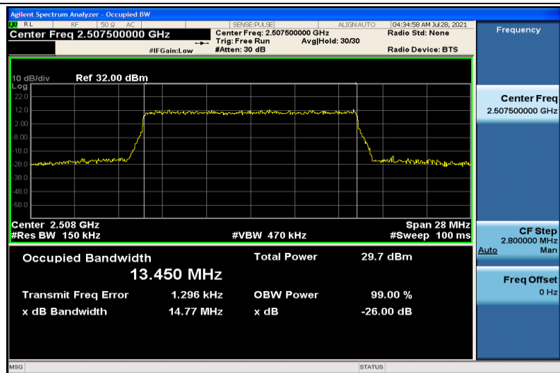
Band7-15MHz-16QAM-20825-75RB#0-13.450
