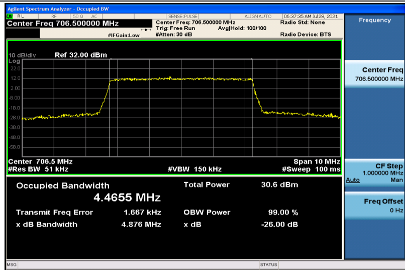
Band17-5MHz-QPSK-23755-25RB#0-4.4655
