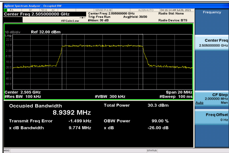
Band7-10MHz-QPSK-20800-50RB#0-8.9392
