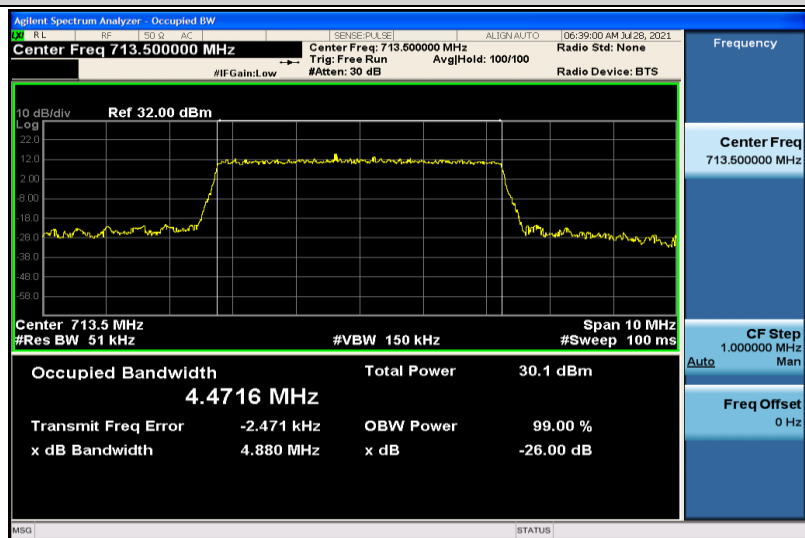
Band17-5MHz-16QAM-23825-25RB#0-4.4716
