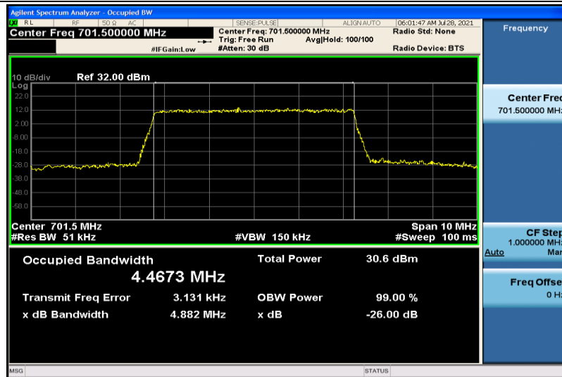
Band12-5MHz-QPSK-23035-25RB#0-4.4673
