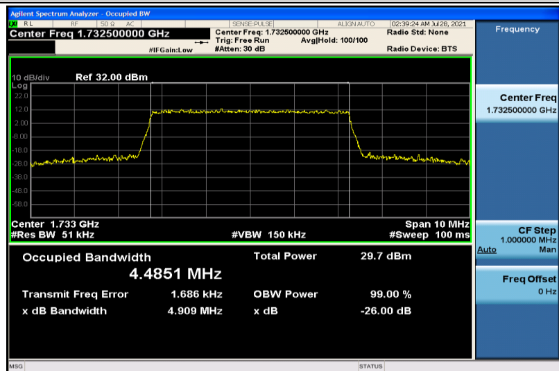
Band4-5MHz-16QAM-20175-25RB#0-4.4851
