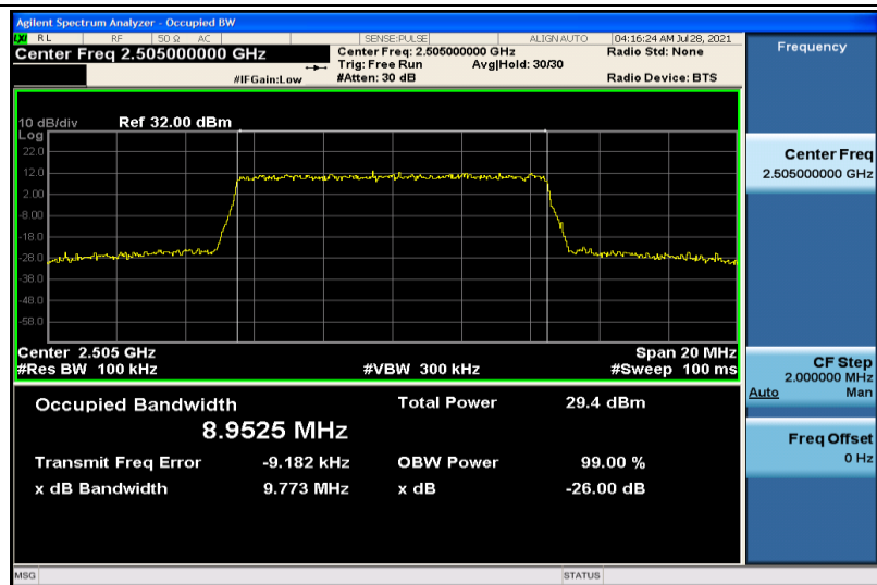
Band7-10MHz-16QAM-20800-50RB#0-8.9525
