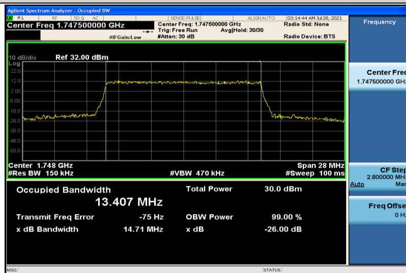
Band4-15MHz-16QAM-20325-75RB#0-13.407
