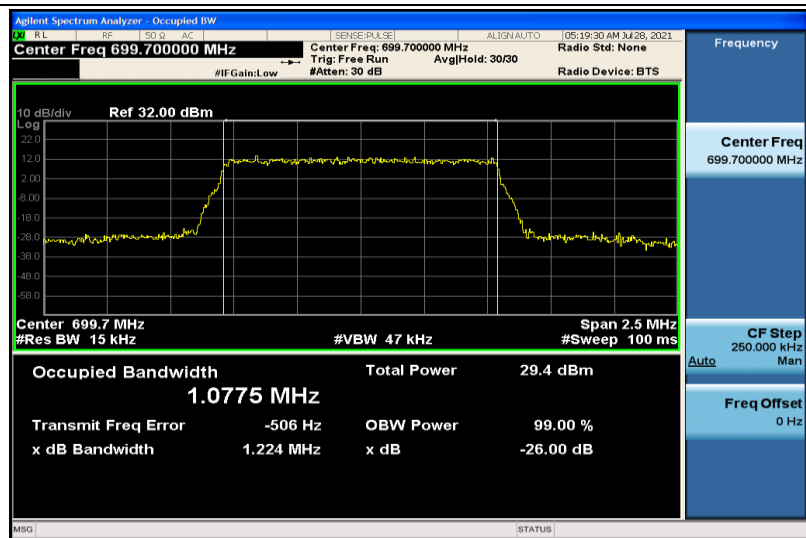
Band12-1.4MHz-QPSK-23017-6RB#0-1.0775
