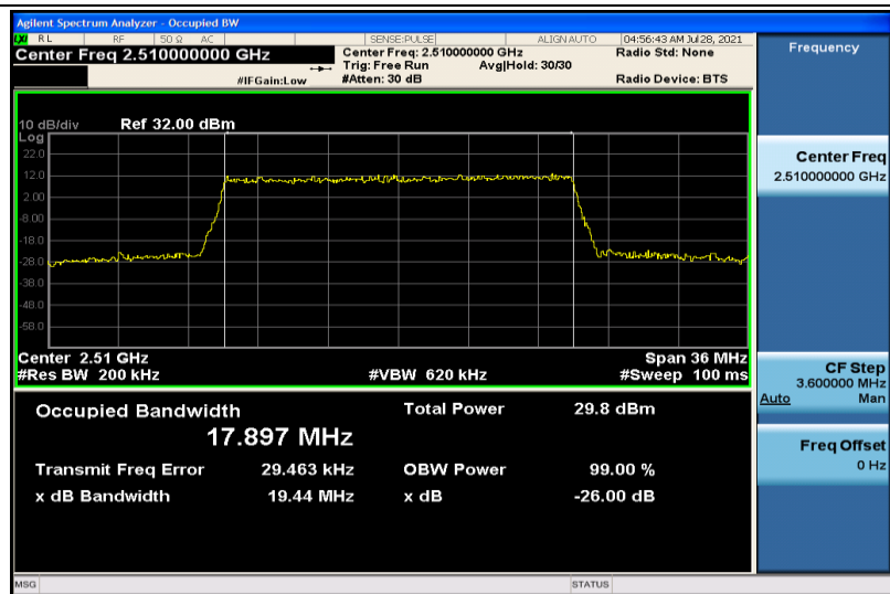
Band7-20MHz-16QAM-20850-100RB#0-17.897
