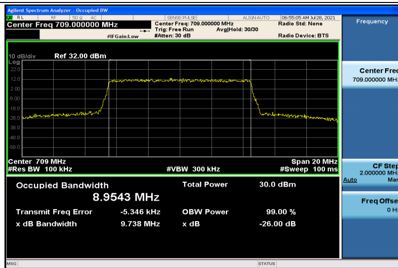
Band17-10MHz-16QAM-23780-50RB#0-8.9543
