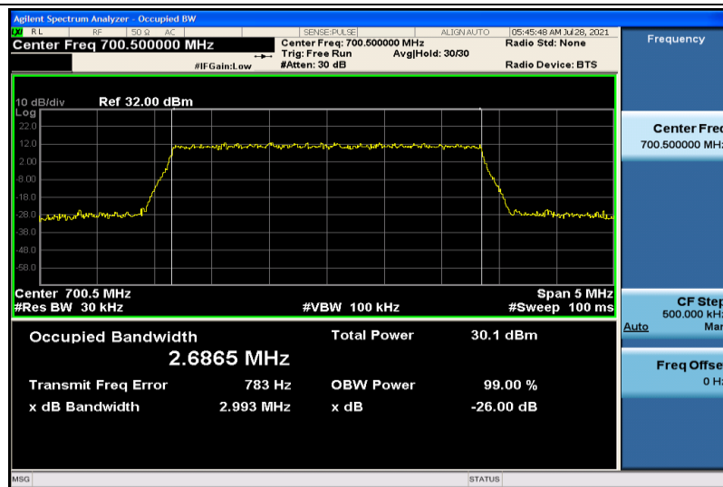
Band12-3MHz-QPSK-23025-15RB#0-2.6865
