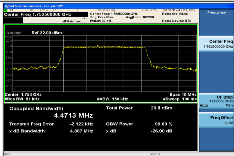
Band4-5MHz-16QAM-20375-25RB#0-4.4713
