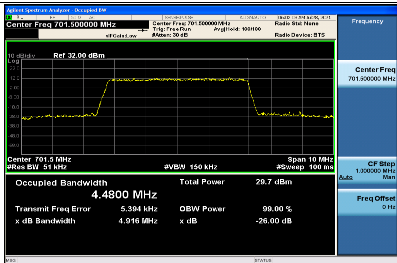
Band12-5MHz-16QAM-23035-25RB#0-4.4800
