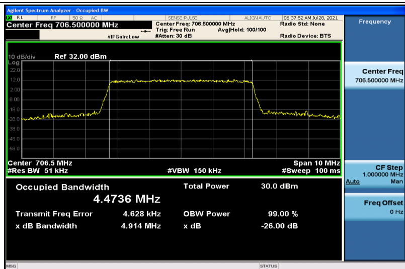
Band17-5MHz-16QAM-23755-25RB#0-4.4736
