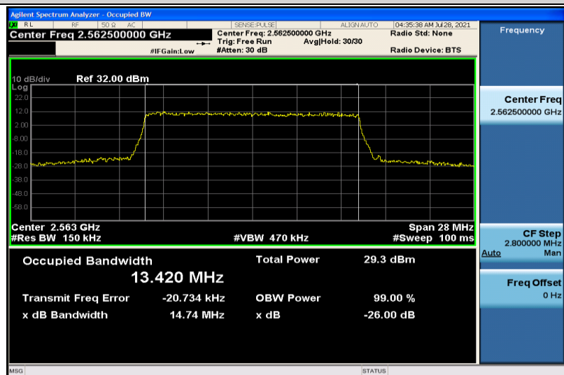
Band7-15MHz-16QAM-21375-75RB#0-13.420
