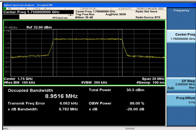
Band4-10MHz-QPSK-20350-50RB#0-8.9516
