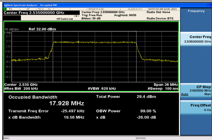
Band7-20MHz-16QAM-21100-100RB#0-17.928
