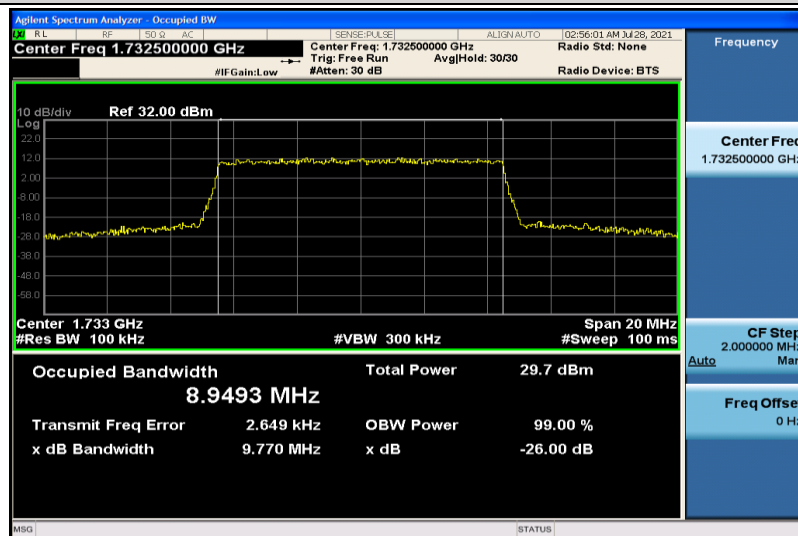
Band4-10MHz-16QAM-20175-50RB#0-8.9493
