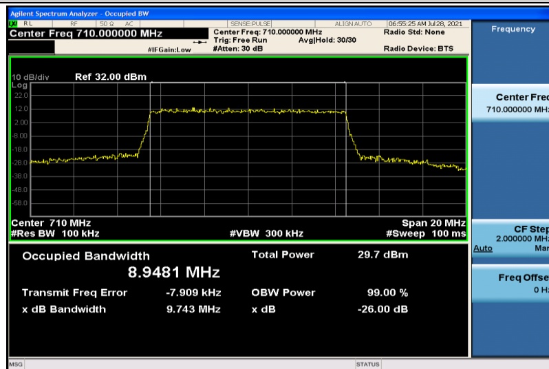
Band17-10MHz-16QAM-23790-50RB#0-8.9481
