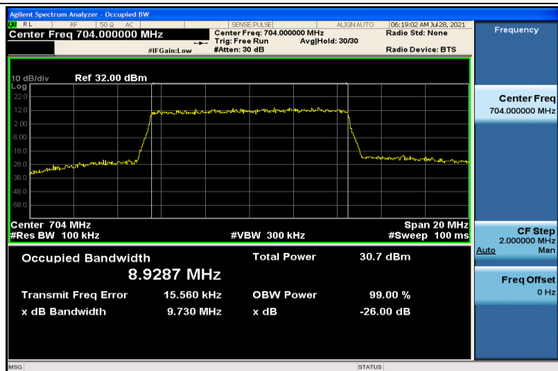
Band12-10MHz-QPSK-23060-50RB#0-8.9287
