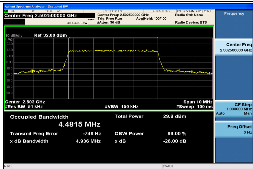
Band7-5MHz-16QAM-20775-25RB#0-4.4815
