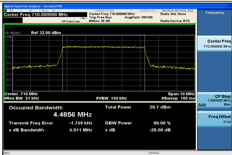
Band17-5MHz-16QAM-23790-25RB#0-4.4856
