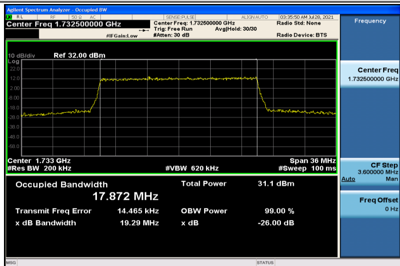
Band4-20MHz-QPSK-20175-100RB#0-17.872
