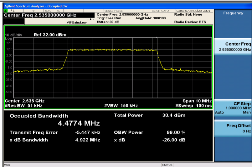
Band7-5MHz-QPSK-21100-25RB#0-4.4774
