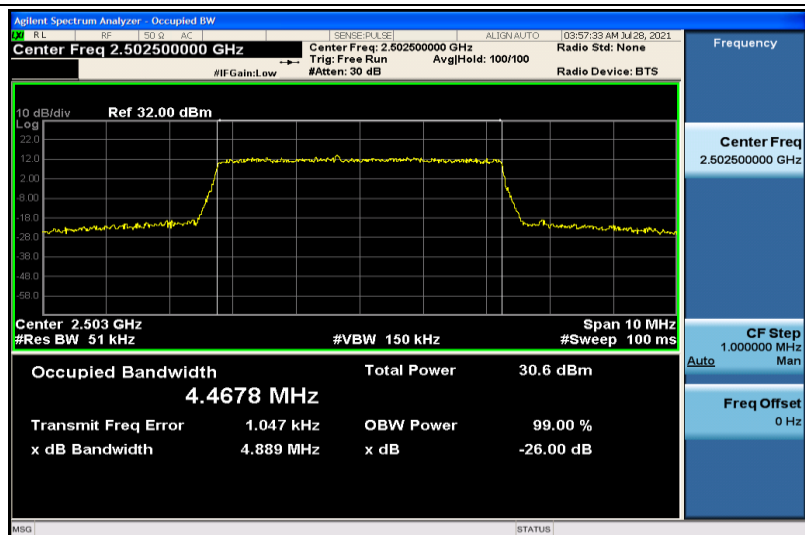
Band7-5MHz-QPSK-20775-25RB#0-4.4678
