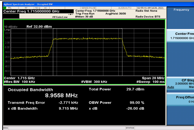
Band4-10MHz-16QAM-20000-50RB#0-8.9558
