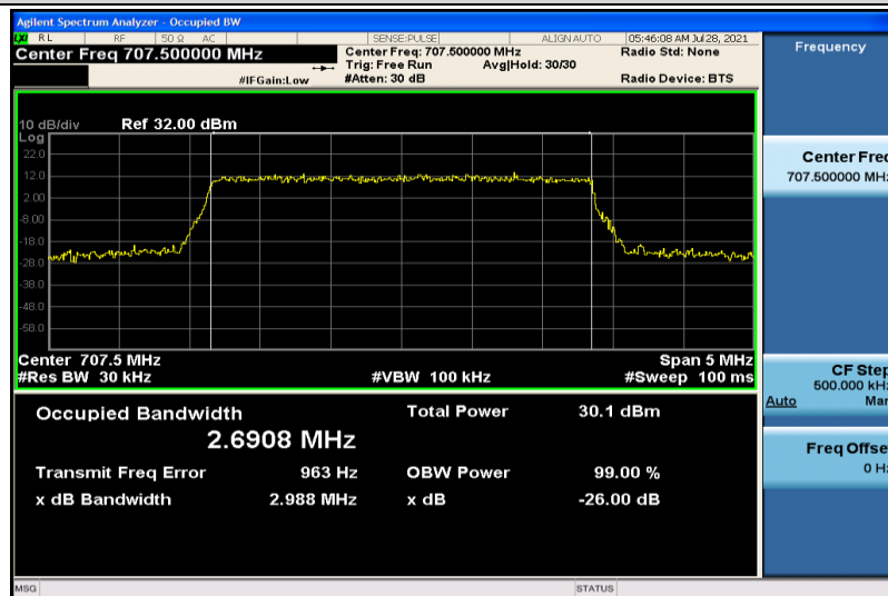
Band12-3MHz-QPSK-23095-15RB#0-2.6908
