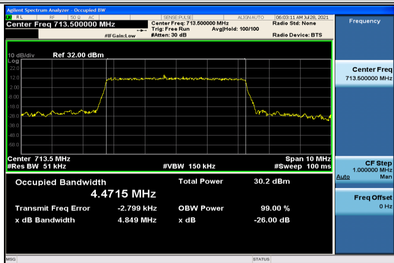
Band12-5MHz-16QAM-23155-25RB#0-4.4715
