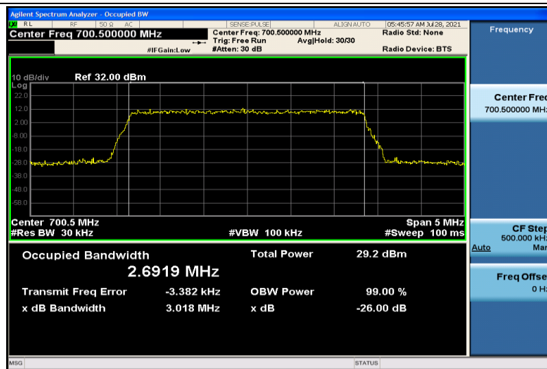
Band12-3MHz-16QAM-23025-15RB#0-2.6919
