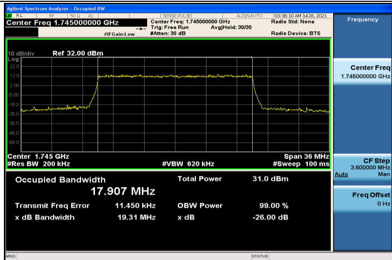
Band4-20MHz-QPSK-20300-100RB#0-17.907
