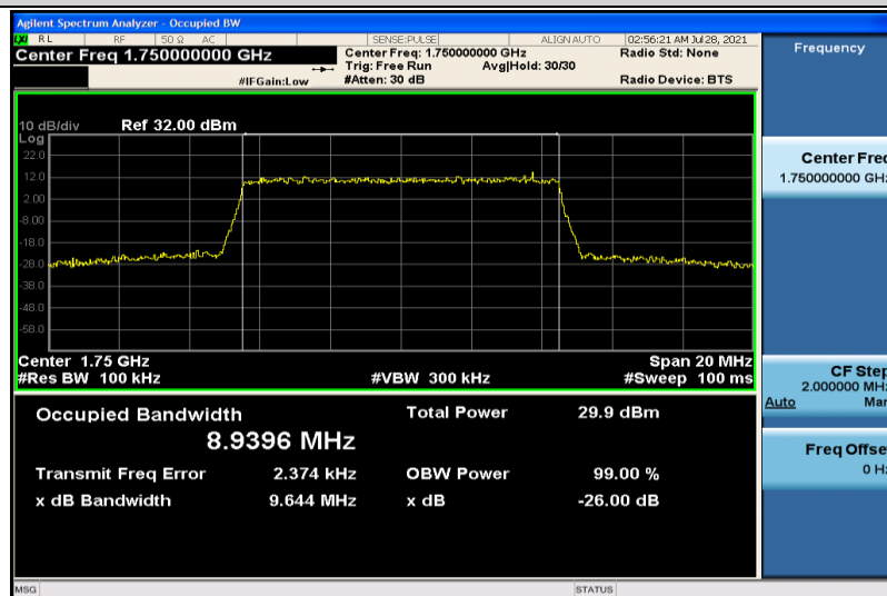
Band4-10MHz-16QAM-20350-50RB#0-8.9396
