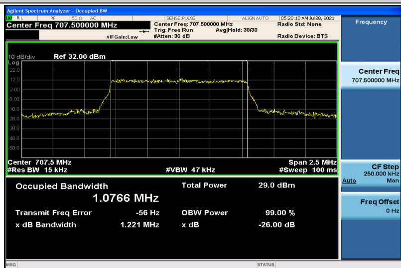
Band12-1.4MHz-16QAM-23095-6RB#0-1.0766
