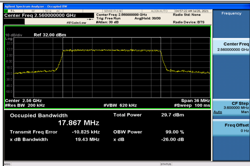
Band7-20MHz-16QAM-21350-100RB#0-17.867
