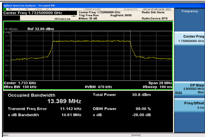
Band4-15MHz-QPSK-20175-75RB#0-13.389
