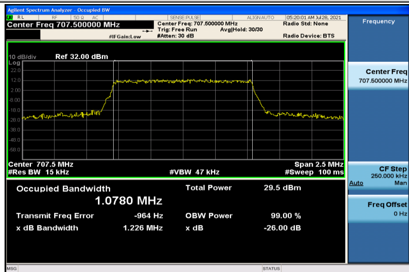
Band12-1.4MHz-QPSK-23095-6RB#0-1.0780
