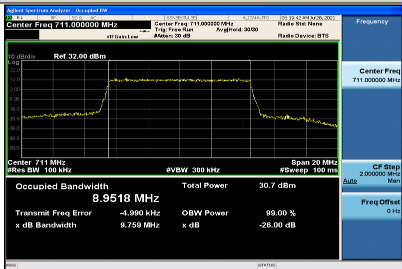
Band12-10MHz-QPSK-23130-50RB#0-8.9518
