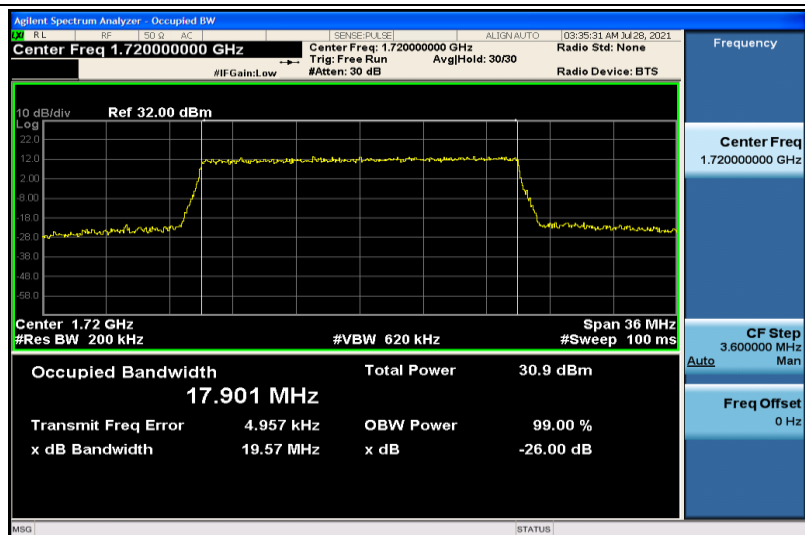
Band4-20MHz-QPSK-20050-100RB#0-17.901
