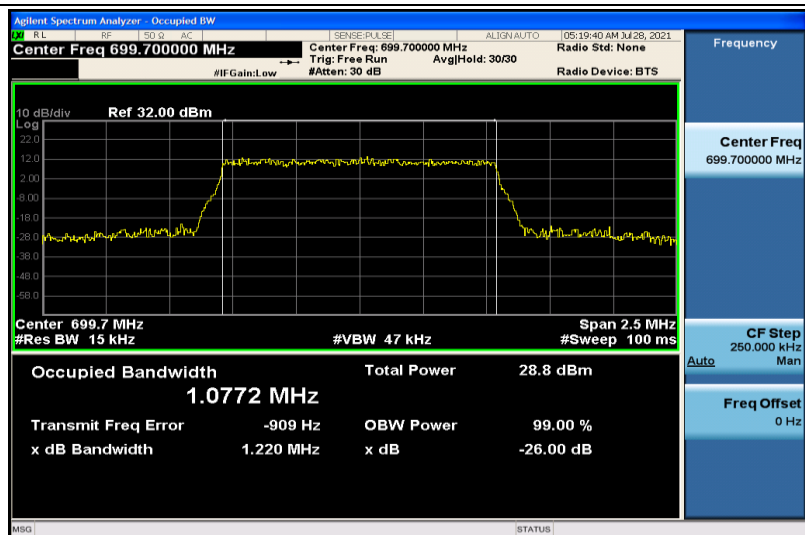
Band12-1.4MHz-16QAM-23017-6RB#0-1.0772
