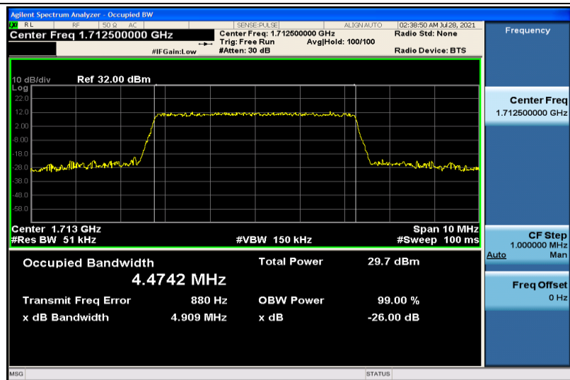
Band4-5MHz-16QAM-19975-25RB#0-4.4742
