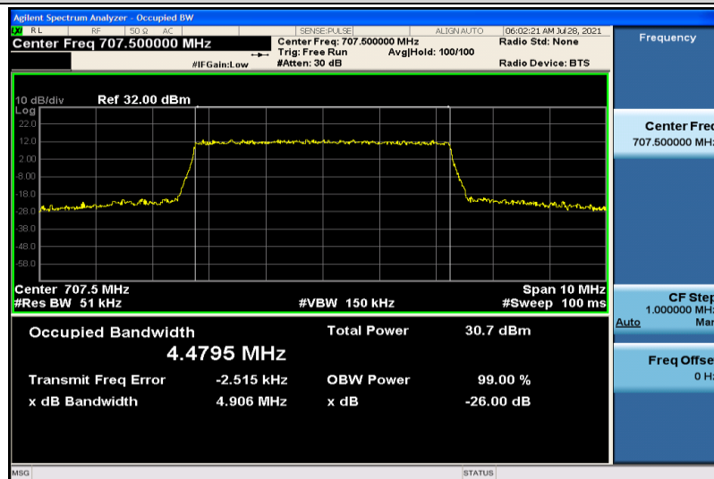
Band12-5MHz-QPSK-23095-25RB#0-4.4795
