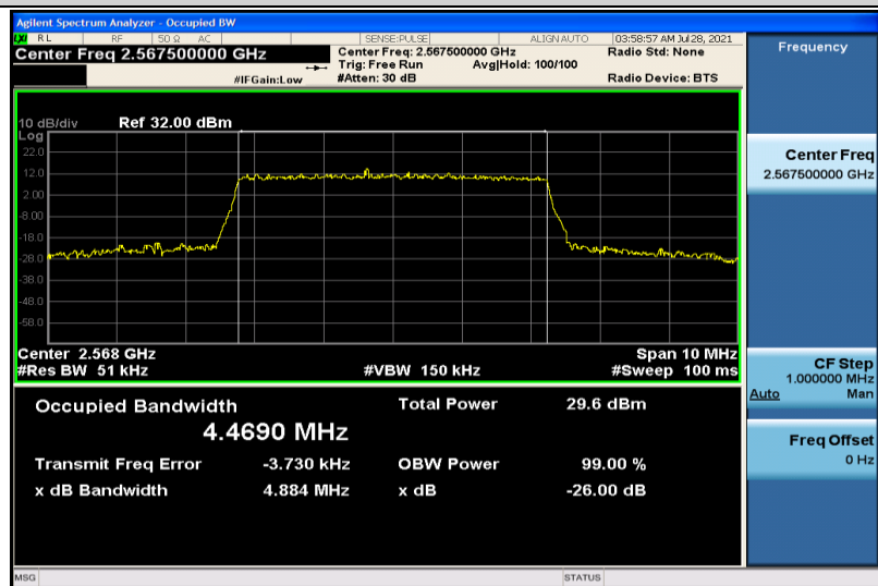
Band7-5MHz-16QAM-21425-25RB#0-4.4690
