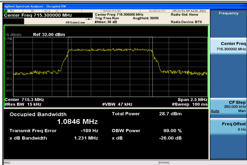
Band12-1.4MHz-16QAM-23173-6RB#0-1.0846
