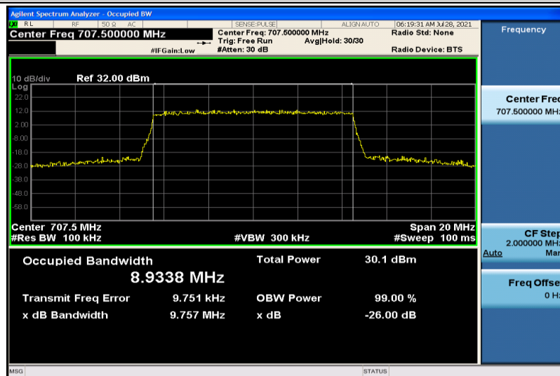
Band12-10MHz-16QAM-23095-50RB#0-8.9338
