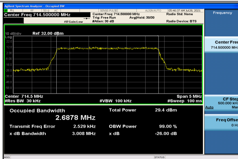
Band12-3MHz-16QAM-23165-15RB#0-2.6878
