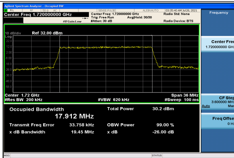
Band4-20MHz-16QAM-20050-100RB#0-17.912
