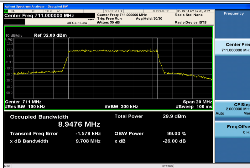
Band12-10MHz-16QAM-23130-50RB#0-8.9476
