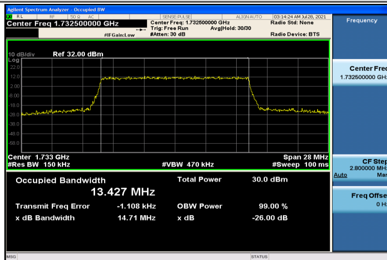
Band4-15MHz-16QAM-20175-75RB#0-13.427
