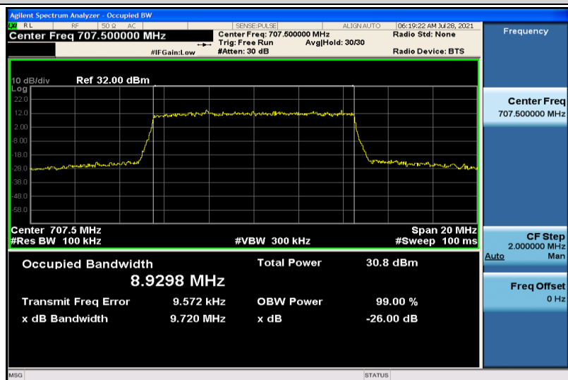
Band12-10MHz-QPSK-23095-50RB#0-8.9298
