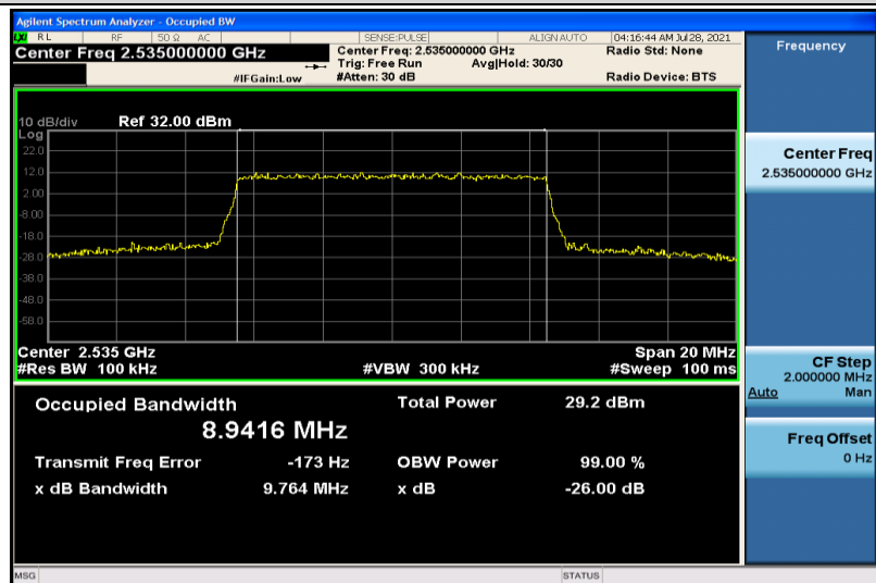
Band7-10MHz-16QAM-21100-50RB#0-8.9416
