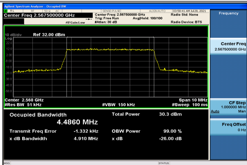
Band7-5MHz-QPSK-21425-25RB#0-4.4860
