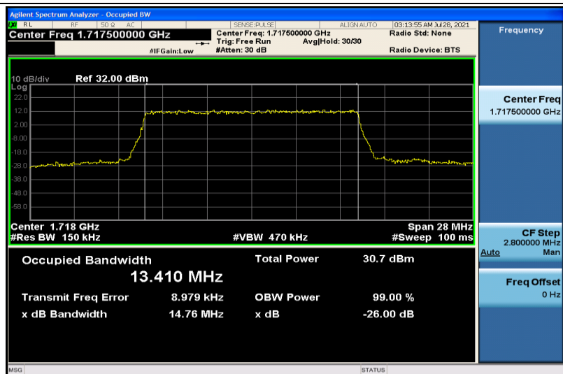
Band4-15MHz-QPSK-20025-75RB#0-13.410
