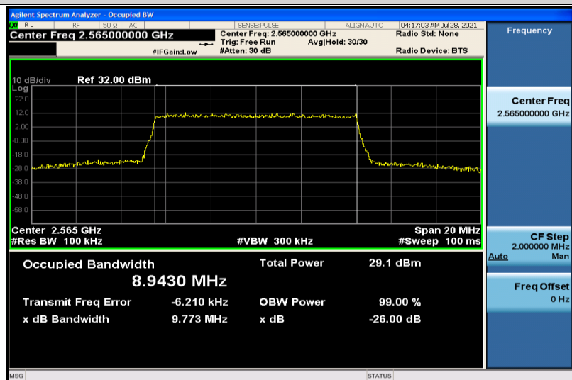
Band7-10MHz-16QAM-21400-50RB#0-8.9430
