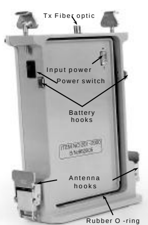
Figure 4.2 Unshielded Transmitter
