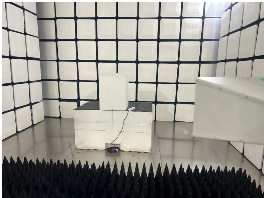
Above 1GHz
