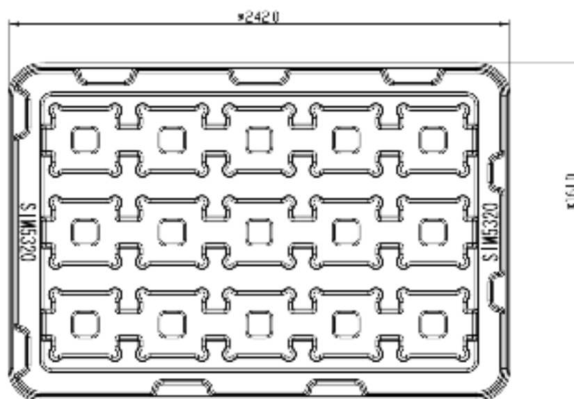
Figure 38: Tray drawing
