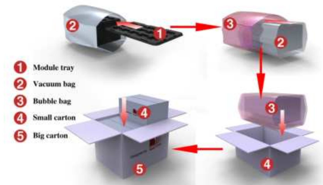
Figure 37: packaging diagram
