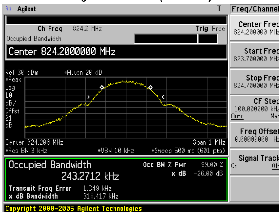
Figure Channel 128 (824.20MHz)
