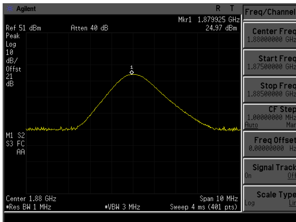
Channel 661
