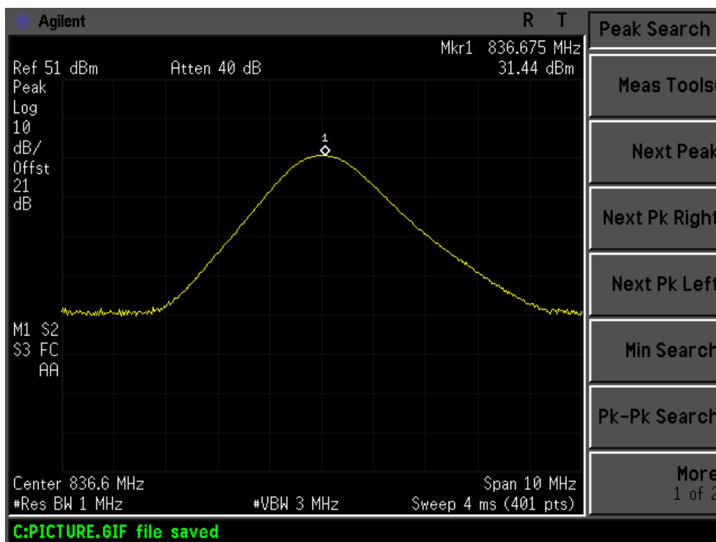
Channel 190
