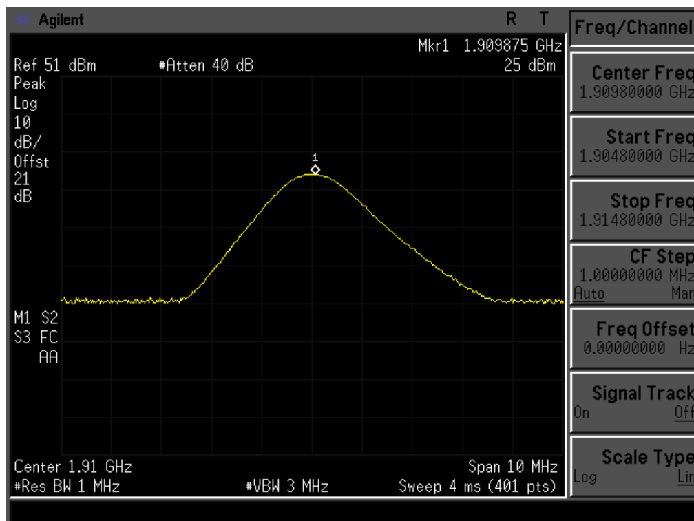
Channel 810
