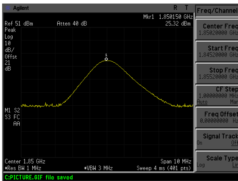
Channel 512
