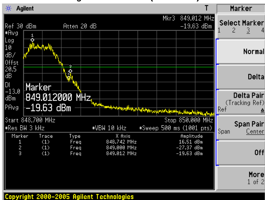
Figure Channel 251 (848.80MHz)
