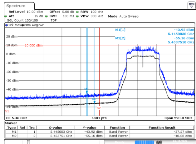
BE-R-LOW, MIMO-B, 802.11ax40-HE0, Ch102
