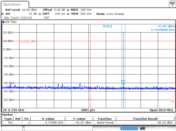
BE-NR-HIGH, SISO-B, 802.11ax160-HE0, Ch114
