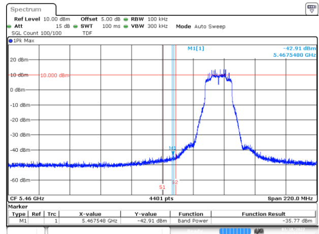
BE-NR-LOW, MIMO-B, 802.11ax20-HE0, Ch100
