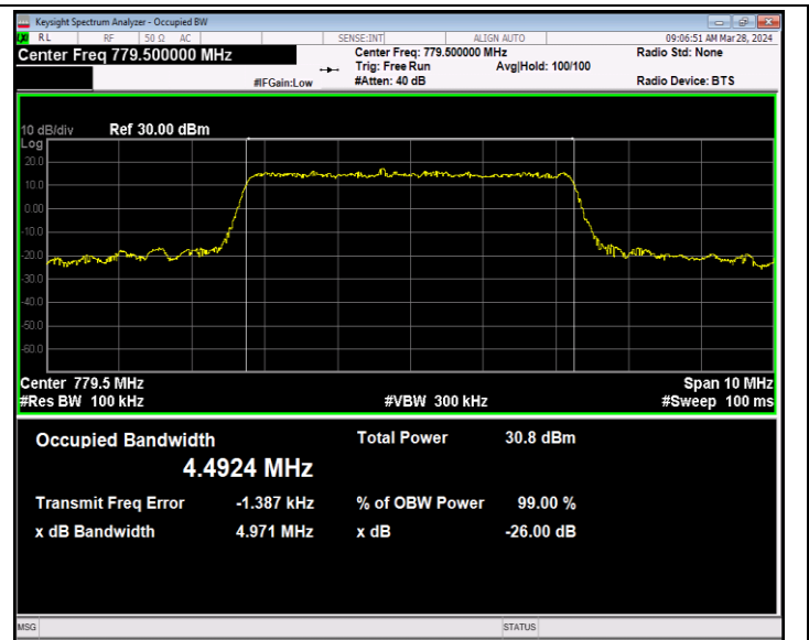
Band13-5MHz-16QAM-23205-25RB#0-PASS
