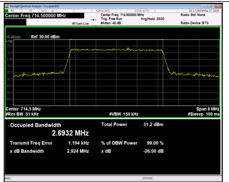
Band12-3MHz-QPSK-23165-15RB#0-PASS
