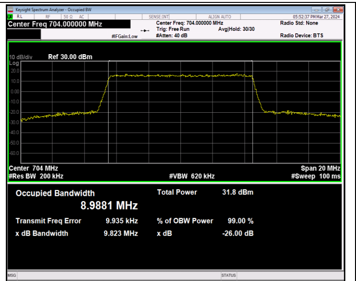
Band12-10MHz-QPSK-23060-50RB#0-PASS
