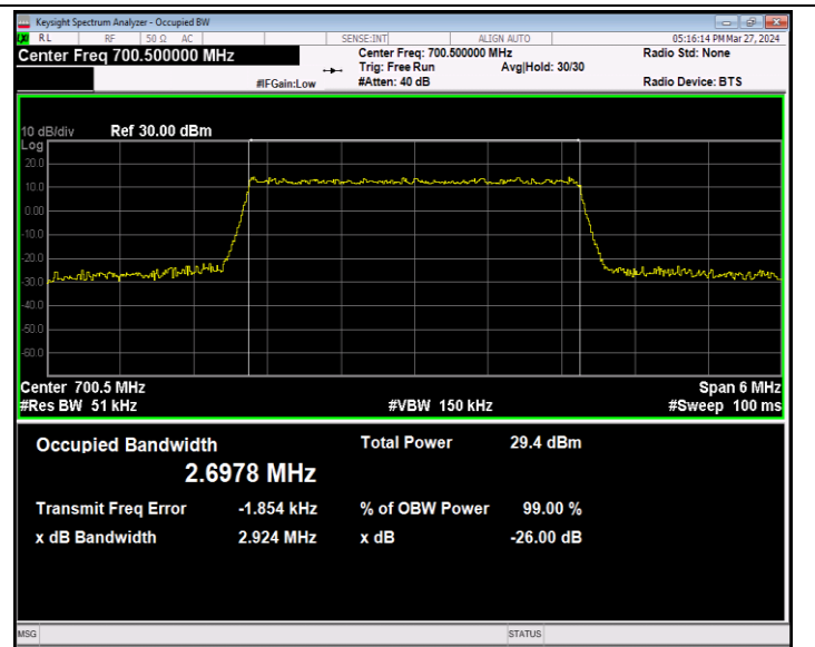
Band12-3MHz-64QAM-23025-15RB#0-PASS
