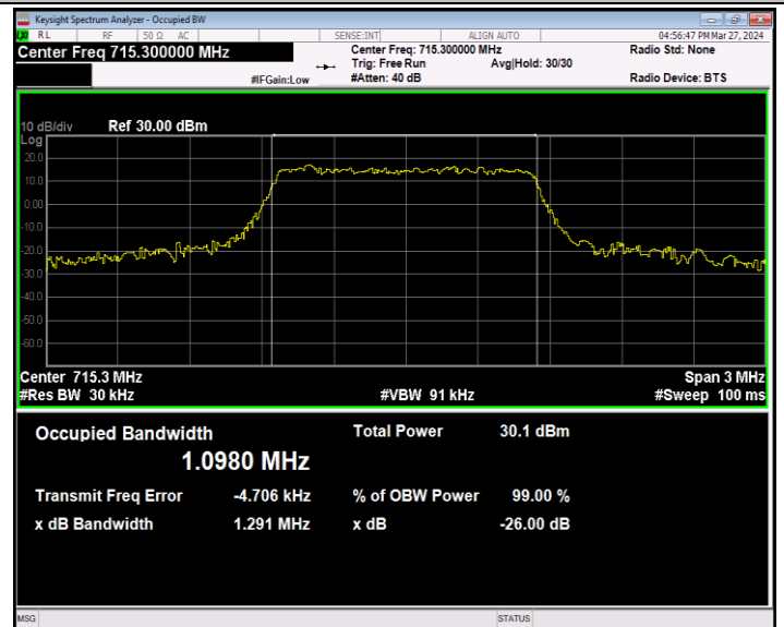
Band12-1.4MHz-16QAM-23173-6RB#0-PASS
