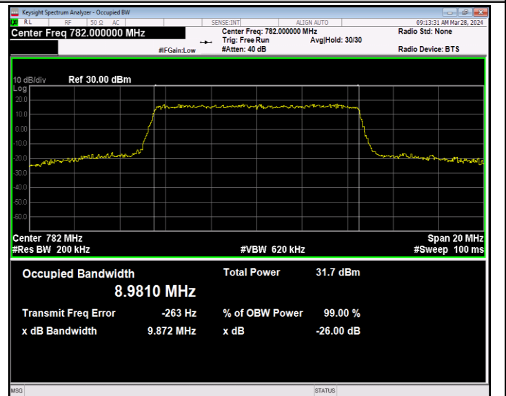
Band13-10MHz-QPSK-23230-50RB#0-PASS
