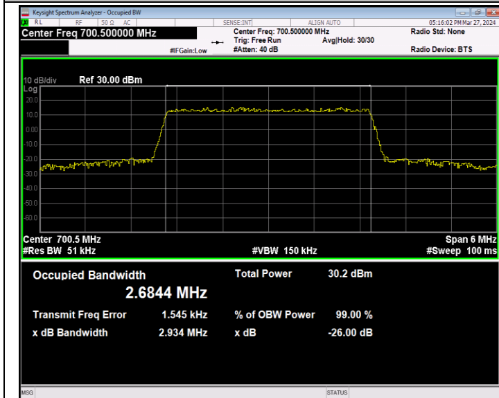
Band12-3MHz-16QAM-23025-15RB#0-PASS
