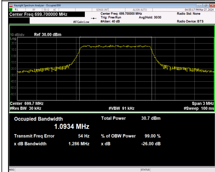
Band12-1.4MHz-QPSK-23017-6RB#0-PASS
