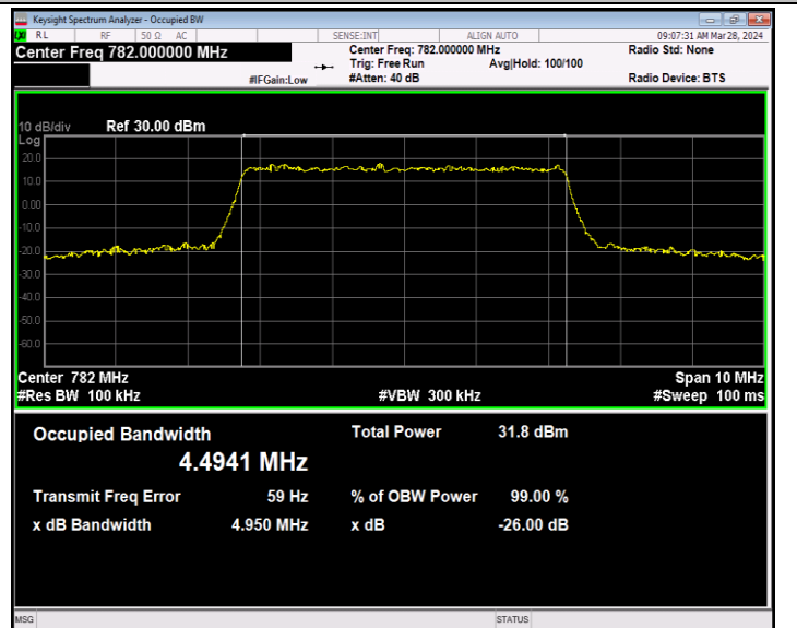
Band13-5MHz-QPSK-23230-25RB#0-PASS
