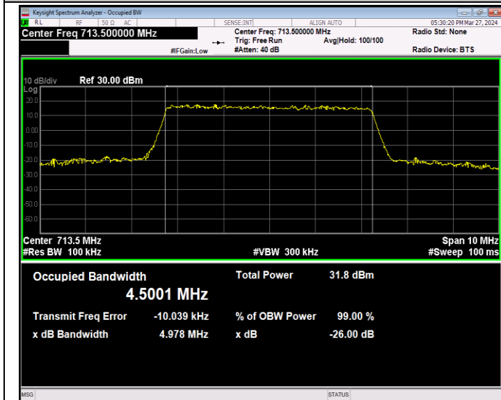
Band12-5MHz-QPSK-23155-25RB#0-PASS
