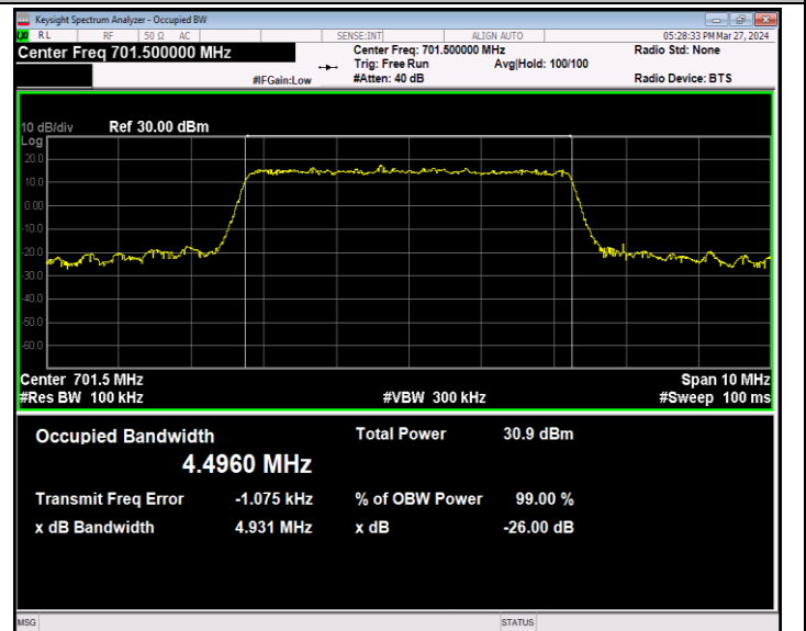
Band12-5MHz-16QAM-23035-25RB#0-PASS
