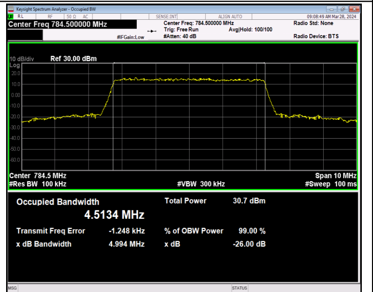
Band13-5MHz-16QAM-23255-25RB#0-PASS
