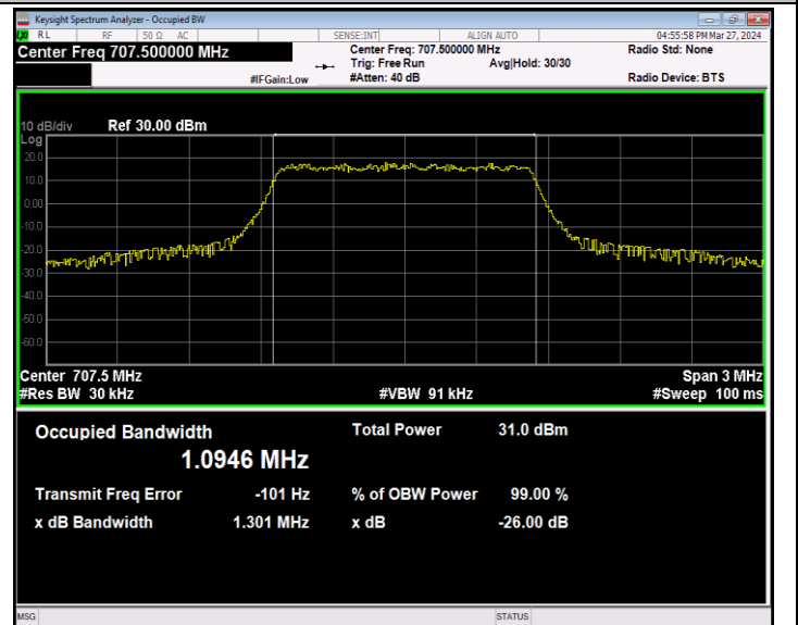
Band12-1.4MHz-QPSK-23095-6RB#0-PASS
