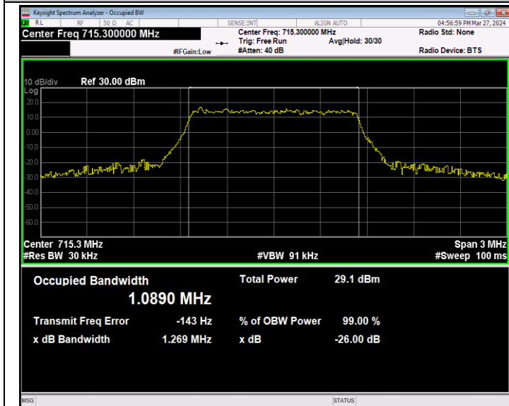
Band12-1.4MHz-64QAM-23173-6RB#0-PASS
