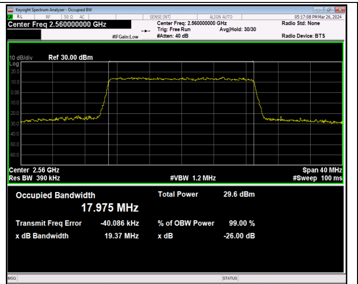
Band7-20MHz-64QAM-21350-100RB#0-PASS
