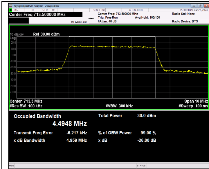
Band12-5MHz-64QAM-23155-25RB#0-PASS
