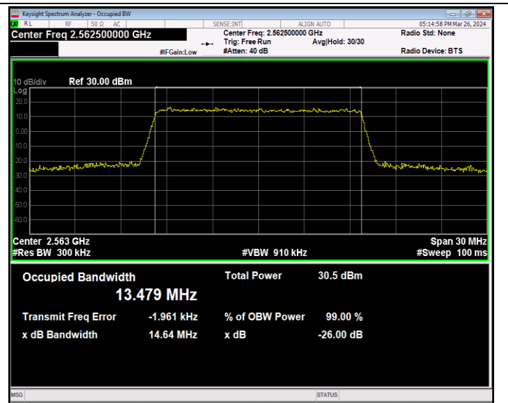
Band7-15MHz-16QAM-21375-75RB#0-PASS
