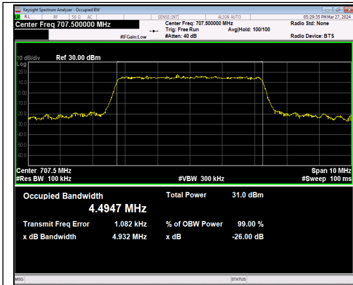
Band12-5MHz-16QAM-23095-25RB#0-PASS
