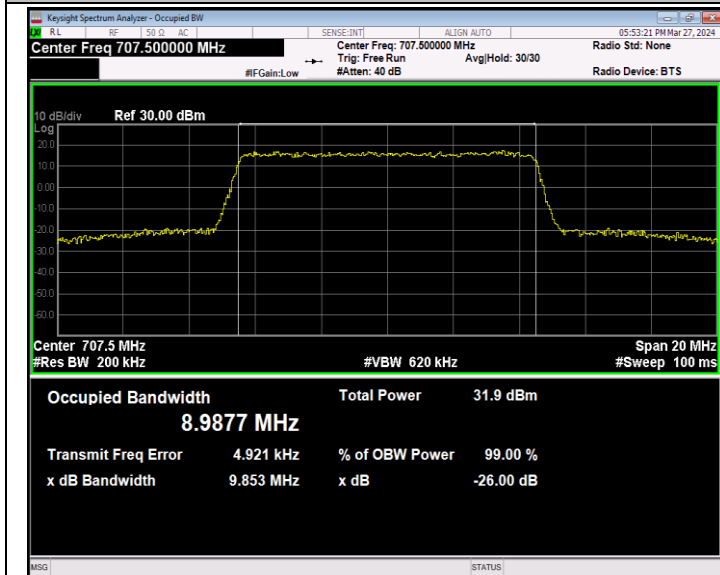
Band12-10MHz-QPSK-23095-50RB#0-PASS
