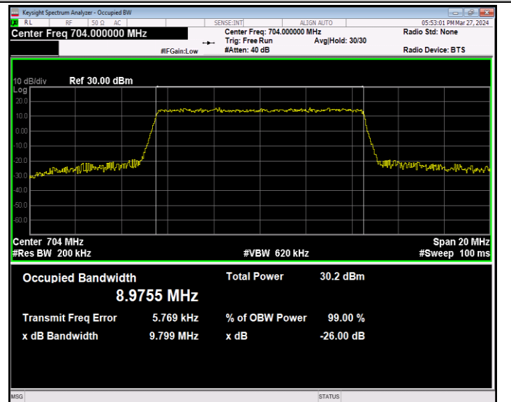
Band12-10MHz-64QAM-23060-50RB#0-PASS
