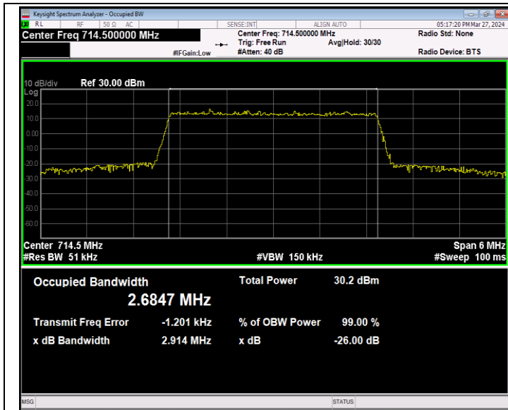
Band12-3MHz-16QAM-23165-15RB#0-PASS
