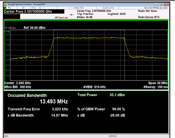
Band7-15MHz-16QAM-20825-75RB#0-PASS
