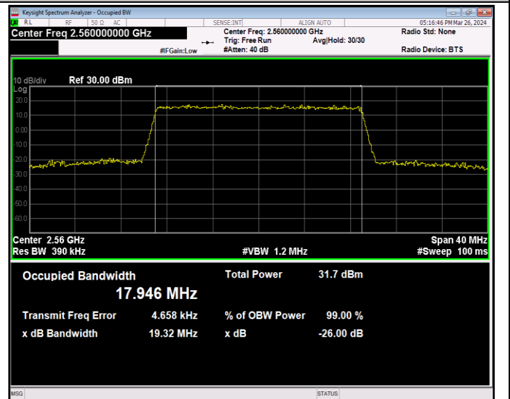
Band7-20MHz-QPSK-21350-100RB#0-PASS
