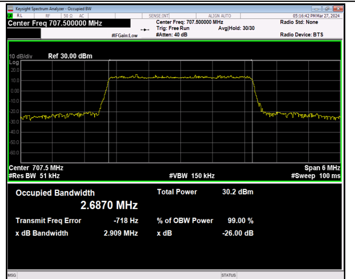
Band12-3MHz-16QAM-23095-15RB#0-PASS
