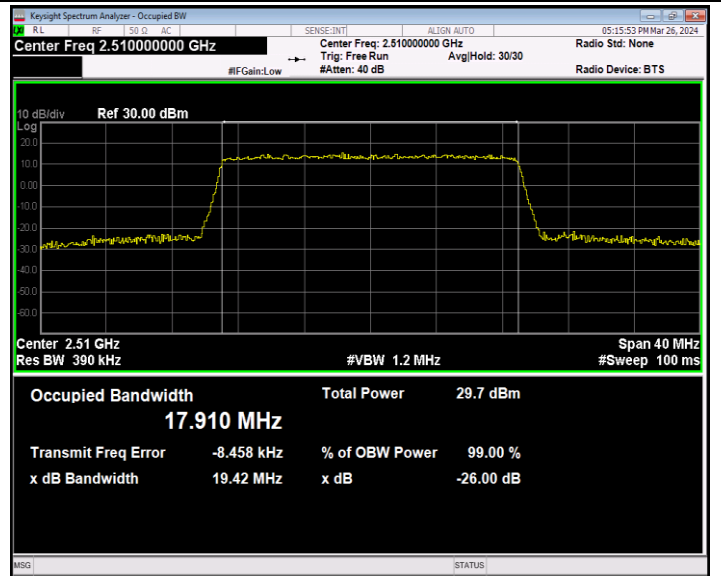
Band7-20MHz-64QAM-20850-100RB#0-PASS
