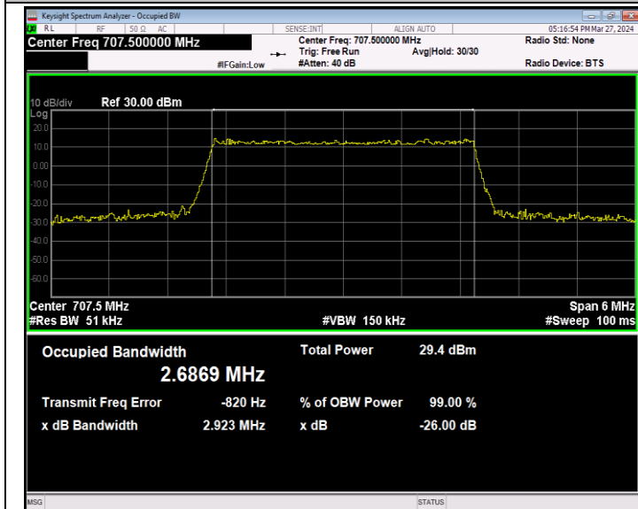
Band12-3MHz-64QAM-23095-15RB#0-PASS
