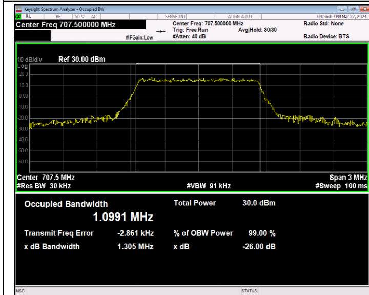
Band12-1.4MHz-16QAM-23095-6RB#0-PASS
