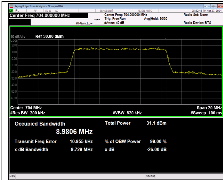
Band12-10MHz-16QAM-23060-50RB#0-PASS
