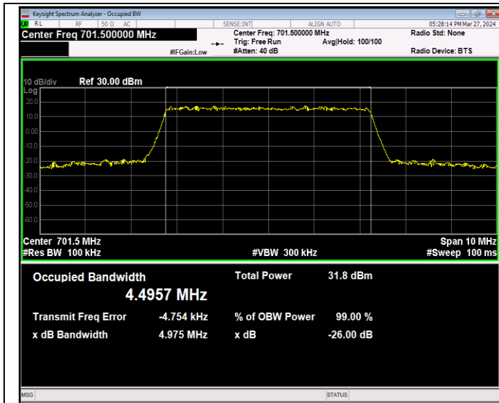
Band12-5MHz-QPSK-23035-25RB#0-PASS
