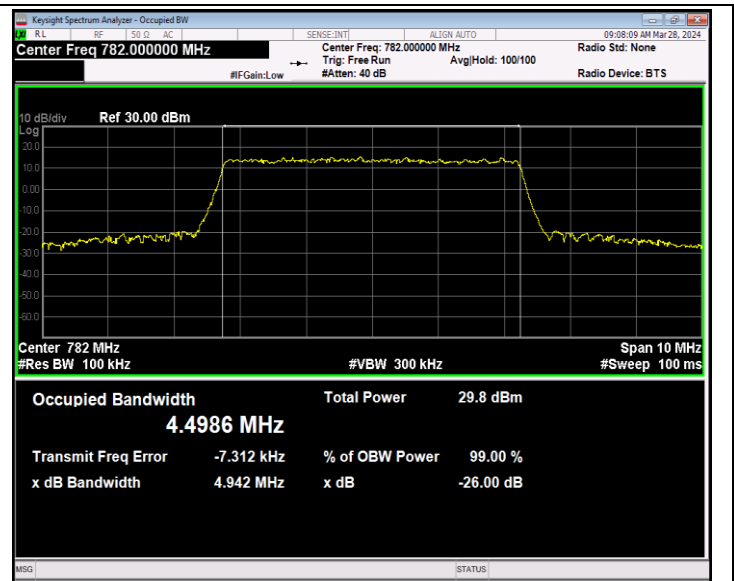
Band13-5MHz-64QAM-23230-25RB#0-PASS
