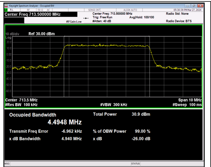
Band12-5MHz-16QAM-23155-25RB#0-PASS
