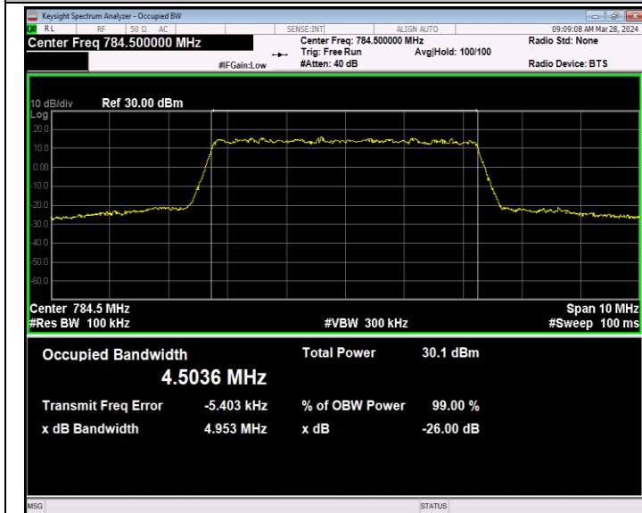
Band13-5MHz-64QAM-23255-25RB#0-PASS
