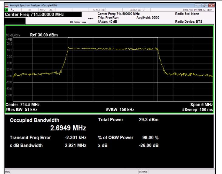
Band12-3MHz-64QAM-23165-15RB#0-PASS
