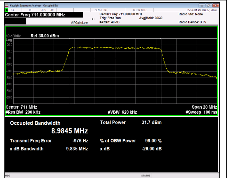
Band12-10MHz-QPSK-23130-50RB#0-PASS
