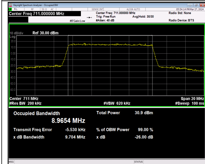
Band12-10MHz-16QAM-23130-50RB#0-PASS
