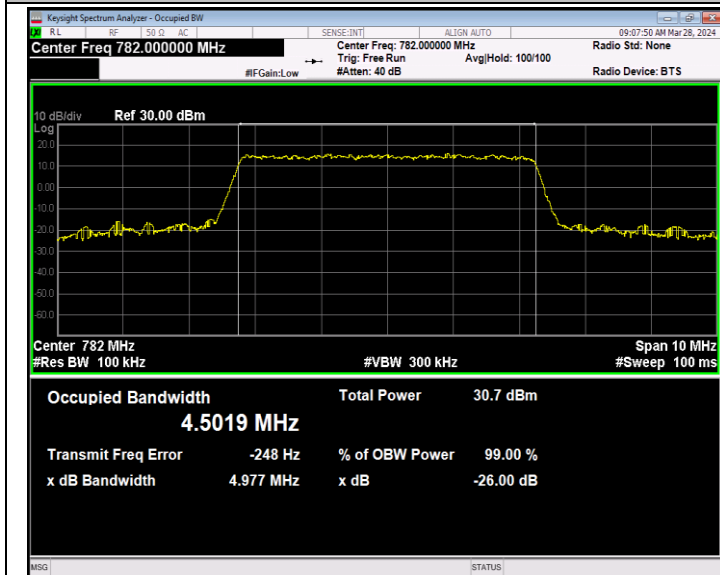
Band13-5MHz-16QAM-23230-25RB#0-PASS
