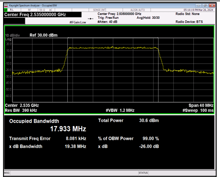
Band7-20MHz-16QAM-21100-100RB#0-PASS
