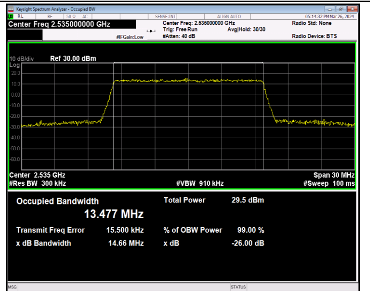
Band7-15MHz-64QAM-21100-75RB#0-PASS
