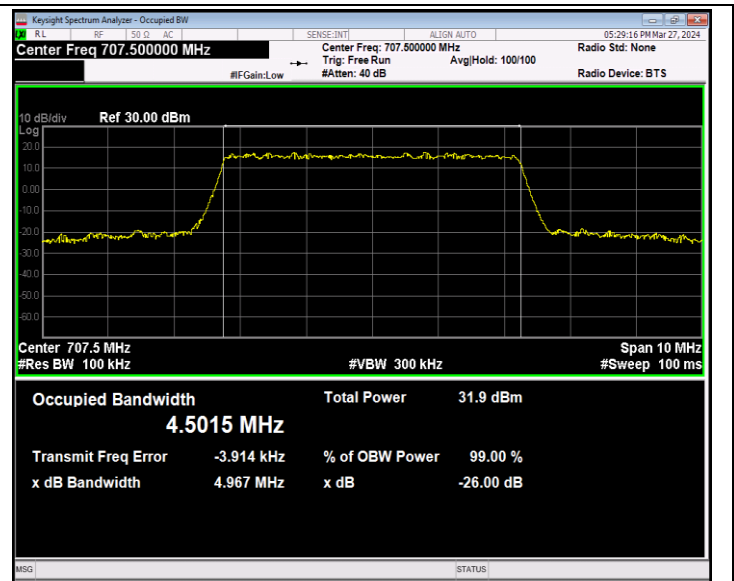
Band12-5MHz-QPSK-23095-25RB#0-PASS
