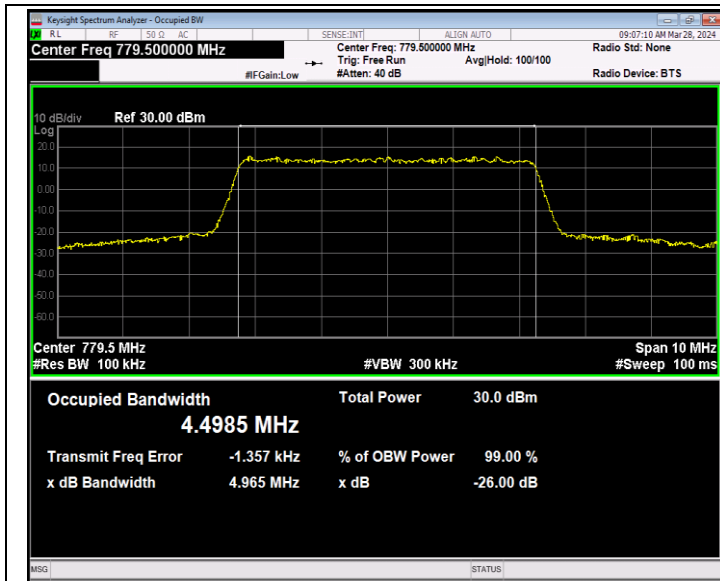
Band13-5MHz-64QAM-23205-25RB#0-PASS
