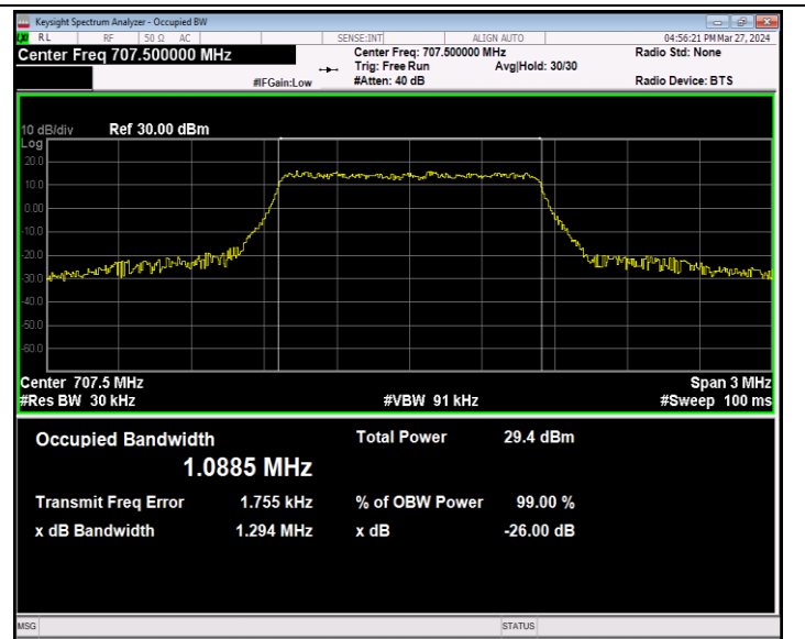
Band12-1.4MHz-64QAM-23095-6RB#0-PASS
