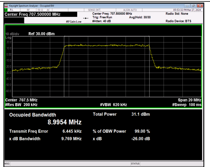
Band12-10MHz-16QAM-23095-50RB#0-PASS
