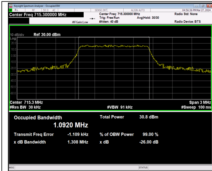
Band12-1.4MHz-QPSK-23173-6RB#0-PASS
