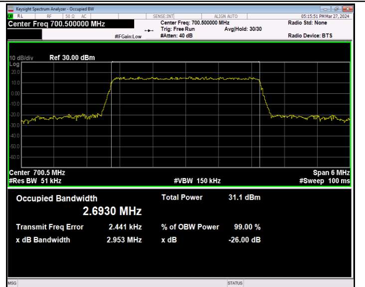
Band12-3MHz-QPSK-23025-15RB#0-PASS
