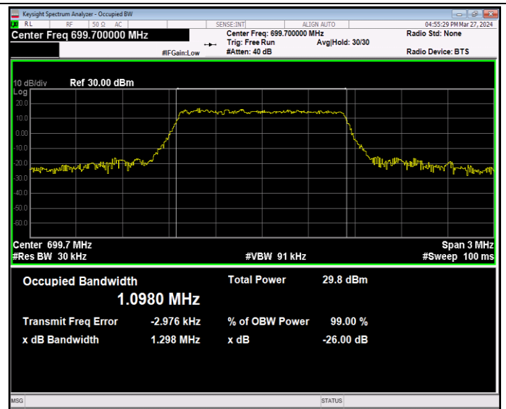
Band12-1.4MHz-16QAM-23017-6RB#0-PASS
