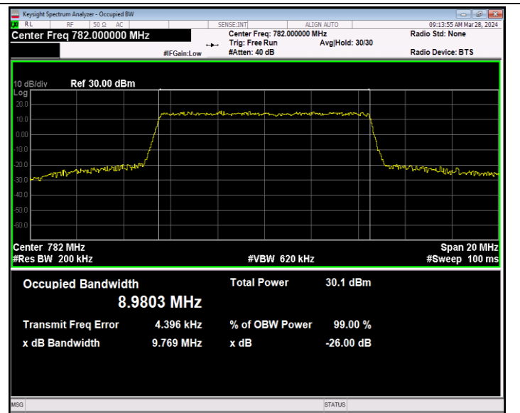
Band13-10MHz-64QAM-23230-50RB#0-PASS
