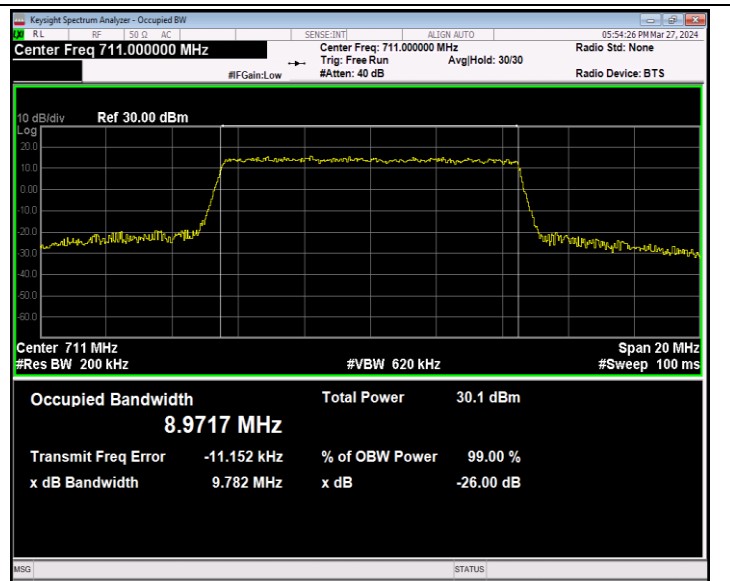
Band12-10MHz-64QAM-23130-50RB#0-PASS
