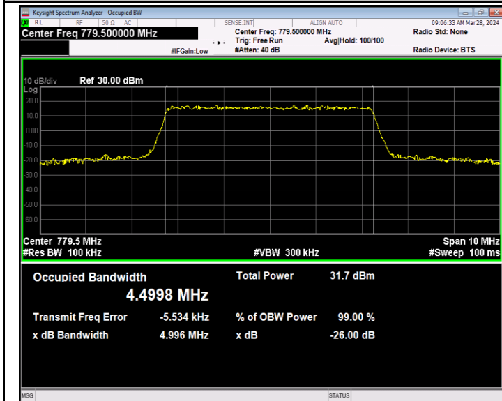
Band13-5MHz-QPSK-23205-25RB#0-PASS
