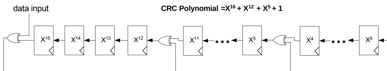
Figure 36. CRC Implementation
