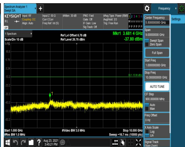
Band17-10MHz-QPSK-23790:1000~10000MHz
