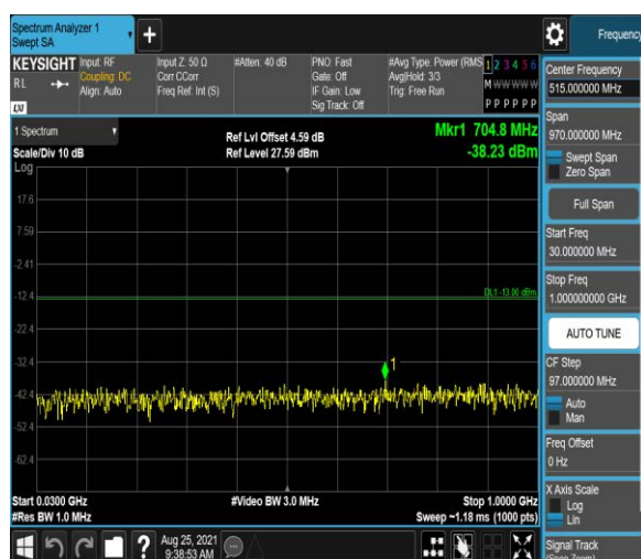
Band66-1.4MHz-QPSK-132665:30~1000MHz
