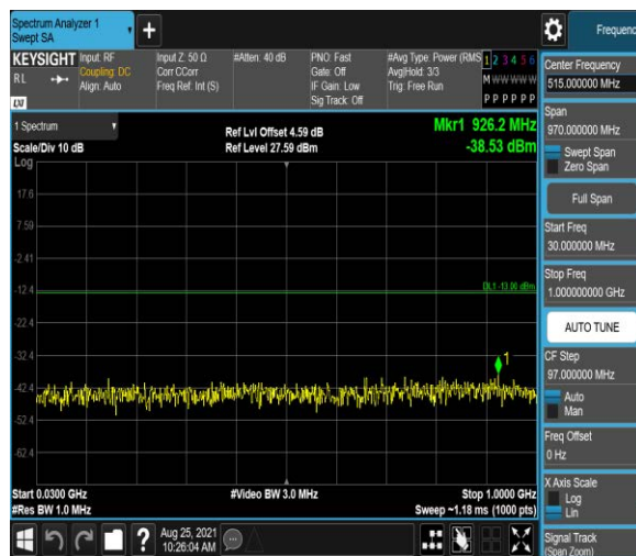
Band66-20MHz-16QAM-132572:30~1000MHz
