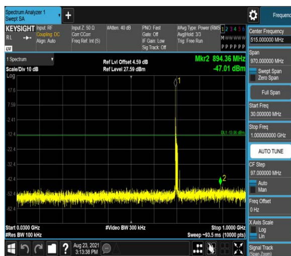
Band12-10MHz-QPSK-23130:30~1000MHz
