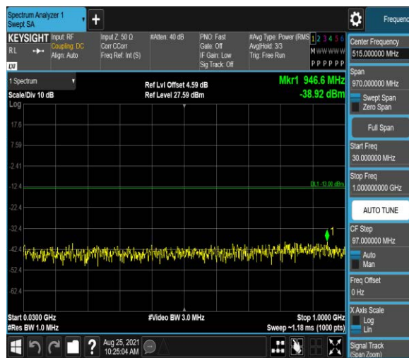
Band66-20MHz-16QAM-132322:30~1000MHz
