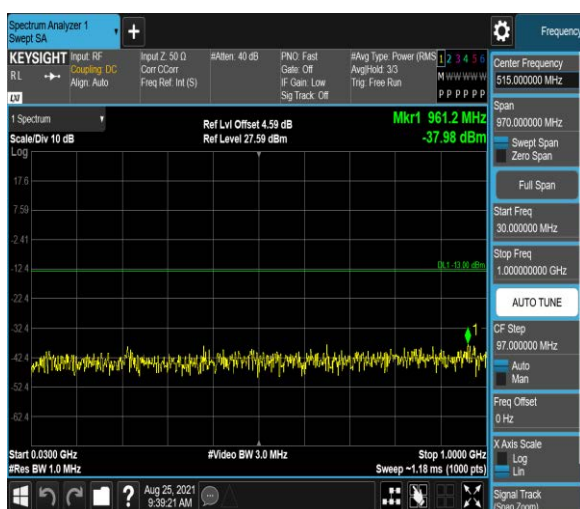
Band66-1.4MHz-16QAM-132665:30~1000MHz
