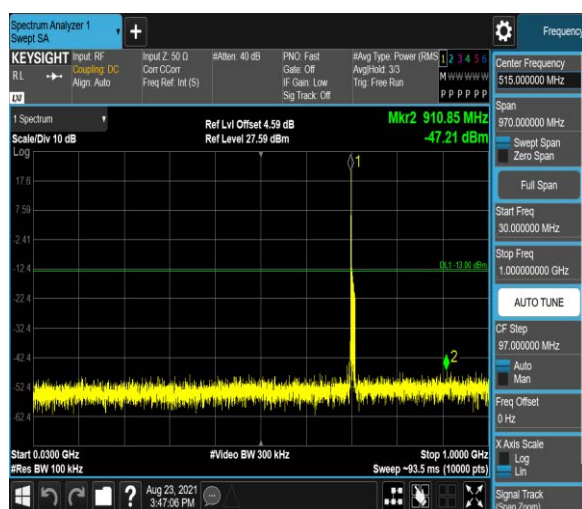
Band17-10MHz-QPSK-23800:30~1000MHz
