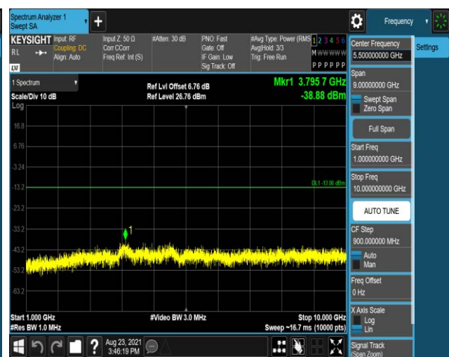
Band17-10MHz-QPSK-23800:1000~10000MHz
