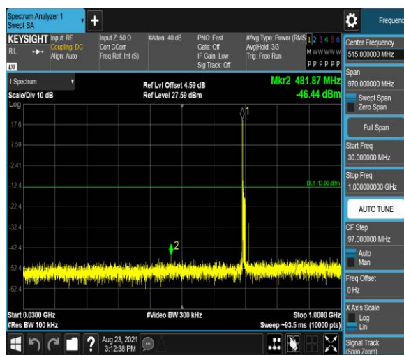
Band12-10MHz-QPSK-23095:30~1000MHz
