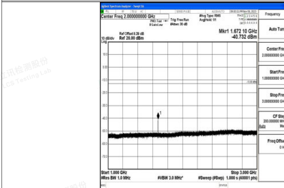
Band5_1.4MHz_QPSK_20525_1RB#0_1000~3000_1000~3000
