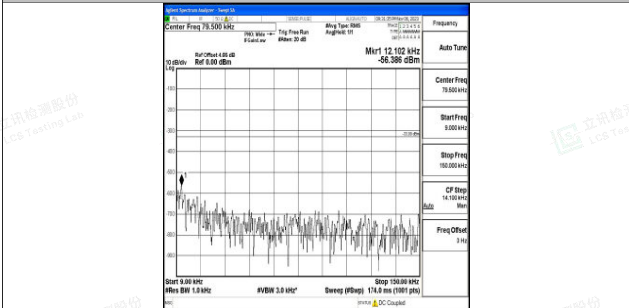
Band5_3MHz_QPSK_20525_1RB#0_0.009~0.15_0.009~0.15
