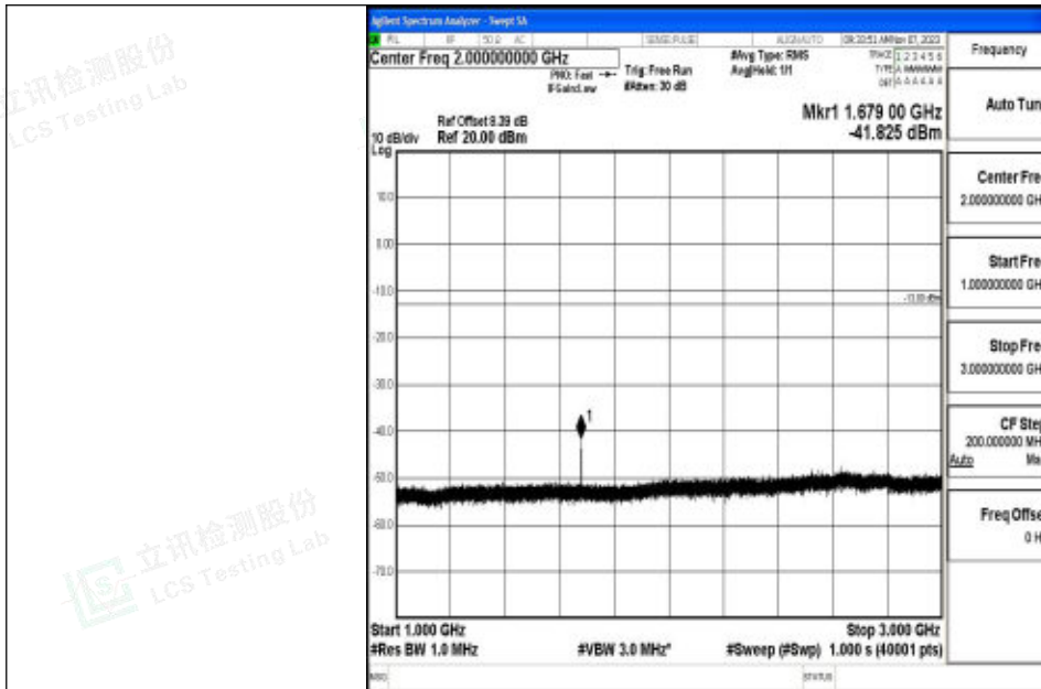
Band5_10MHz_16QAM_20600_1RB#0_1000~3000_1000~3000
