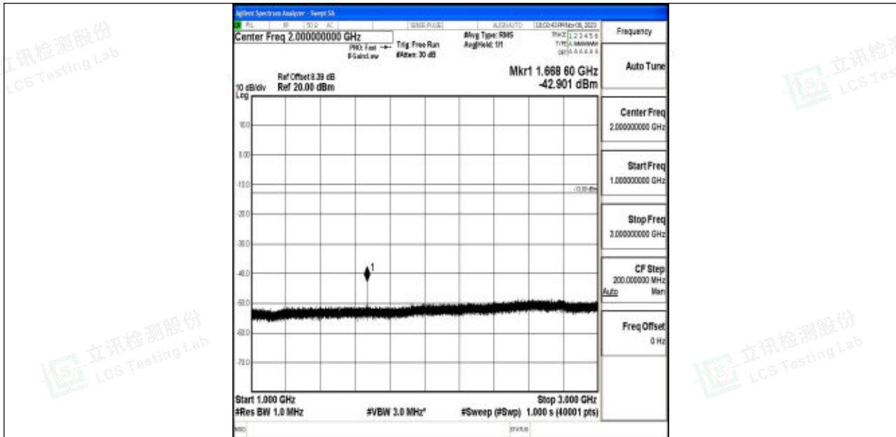
Band5_5MHz_16QAM_20525_1RB#0_1000~3000_1000~3000
