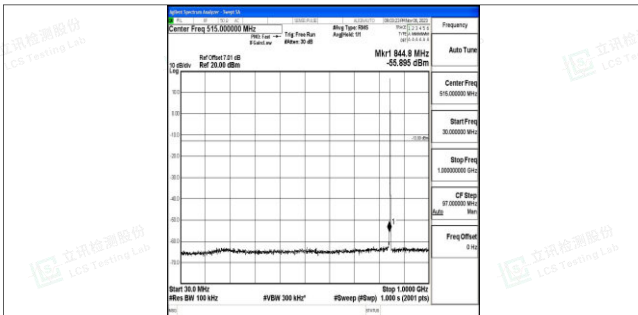
Band5_1.4MHz_16QAM_20643_1RB#0_30~1000_30~1000
