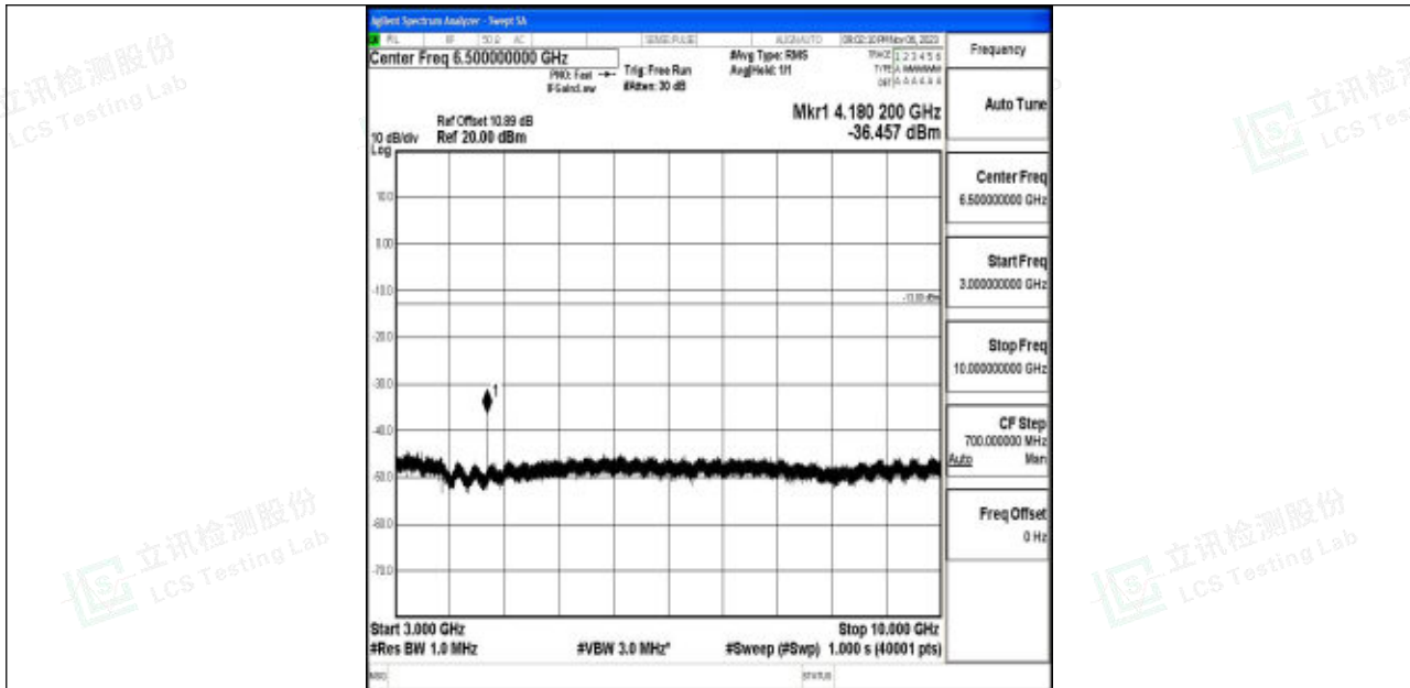
Band5_1.4MHz_64QAM_20525_1RB#0_3000~10000_3000~10000
