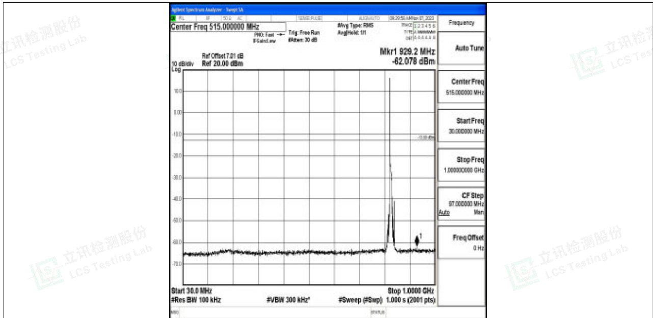
Band5_10MHz_64QAM_20450_1RB#0_30~1000_30~1000
