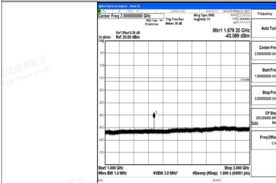
Band5_10MHz_QPSK_20600_1RB#0_1000~3000_1000~3000
