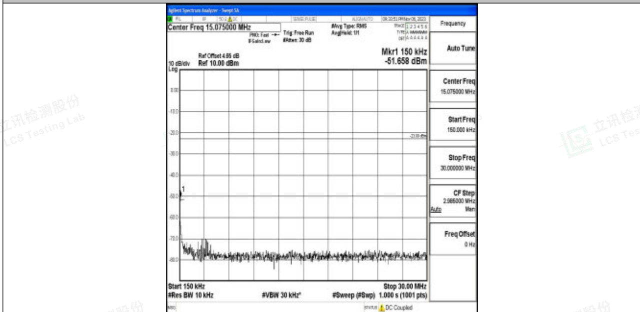
Band5_3MHz_QPSK_20635_1RB#0_0.15~30_0.15~30
