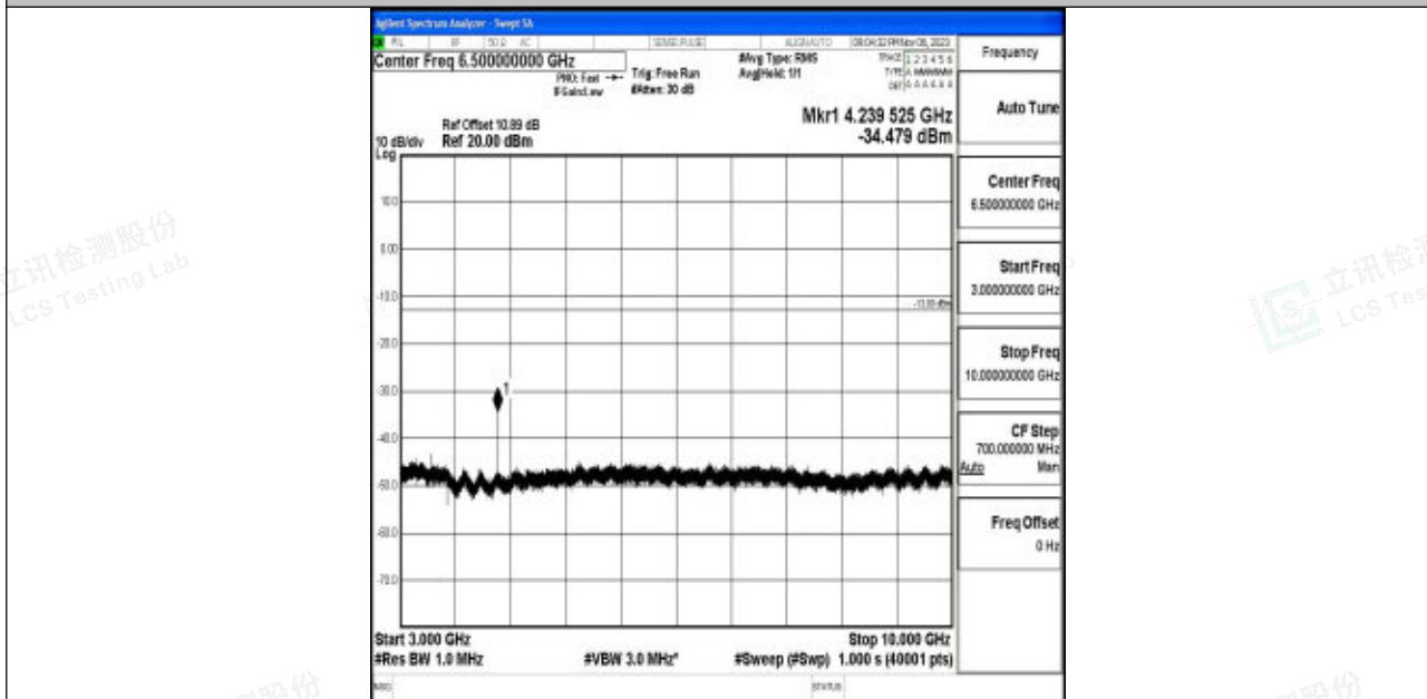
Band5_1.4MHz_64QAM_20643_1RB#0_3000~10000_3000~10000
