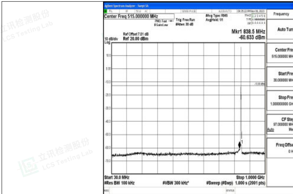
Band5_3MHz_64QAM_20635_1RB#0_30~1000_30~1000
