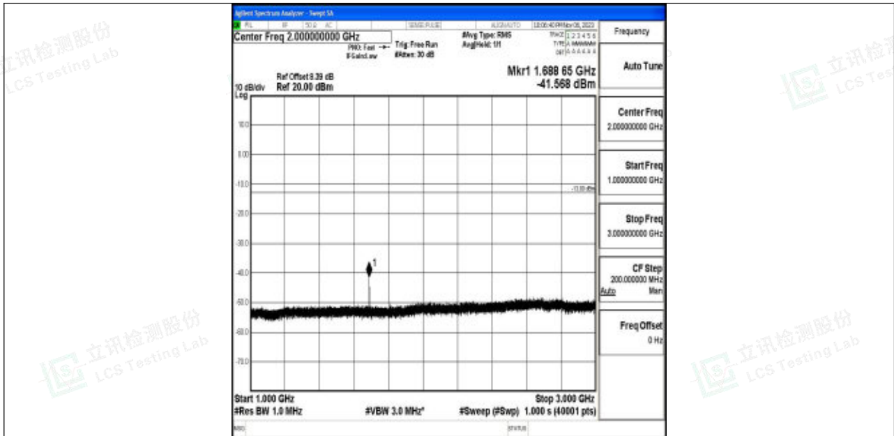
Band5_5MHz_64QAM_20625_1RB#0_1000~3000_1000~3000
