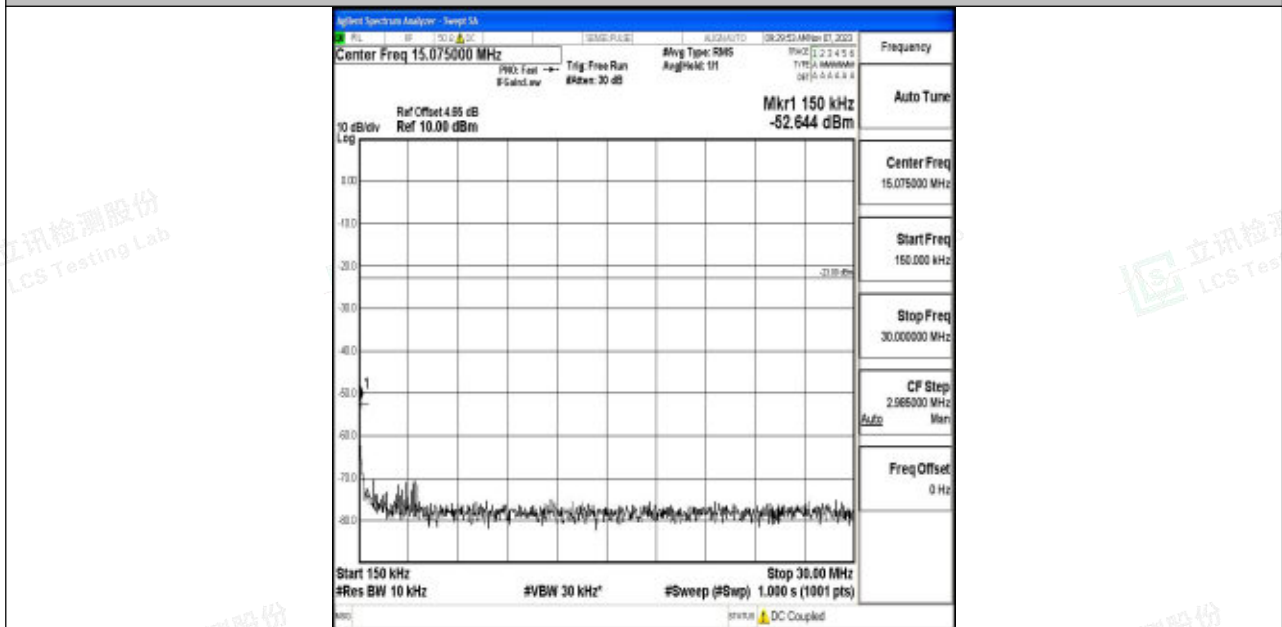
Band5_10MHz_64QAM_20450_1RB#0_0.15~30_0.15~30
