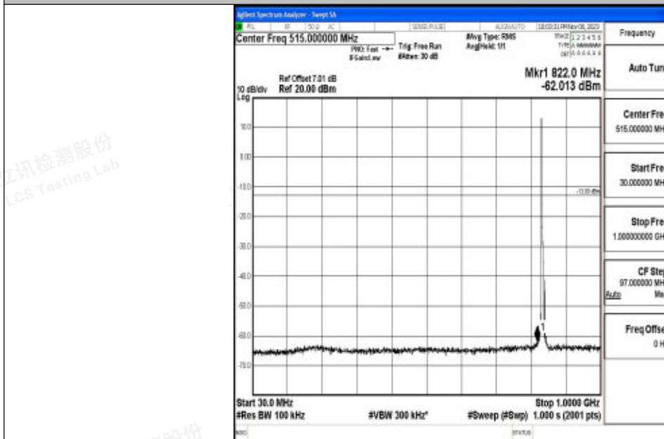
Band5_5MHz_16QAM_20525_1RB#0_30~1000_30~1000
