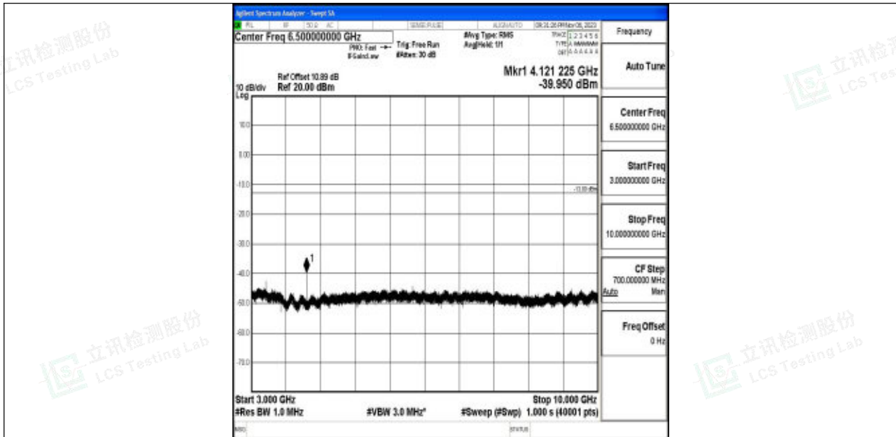
Band5_3MHz_64QAM_20415_1RB#0_3000~10000_3000~10000
