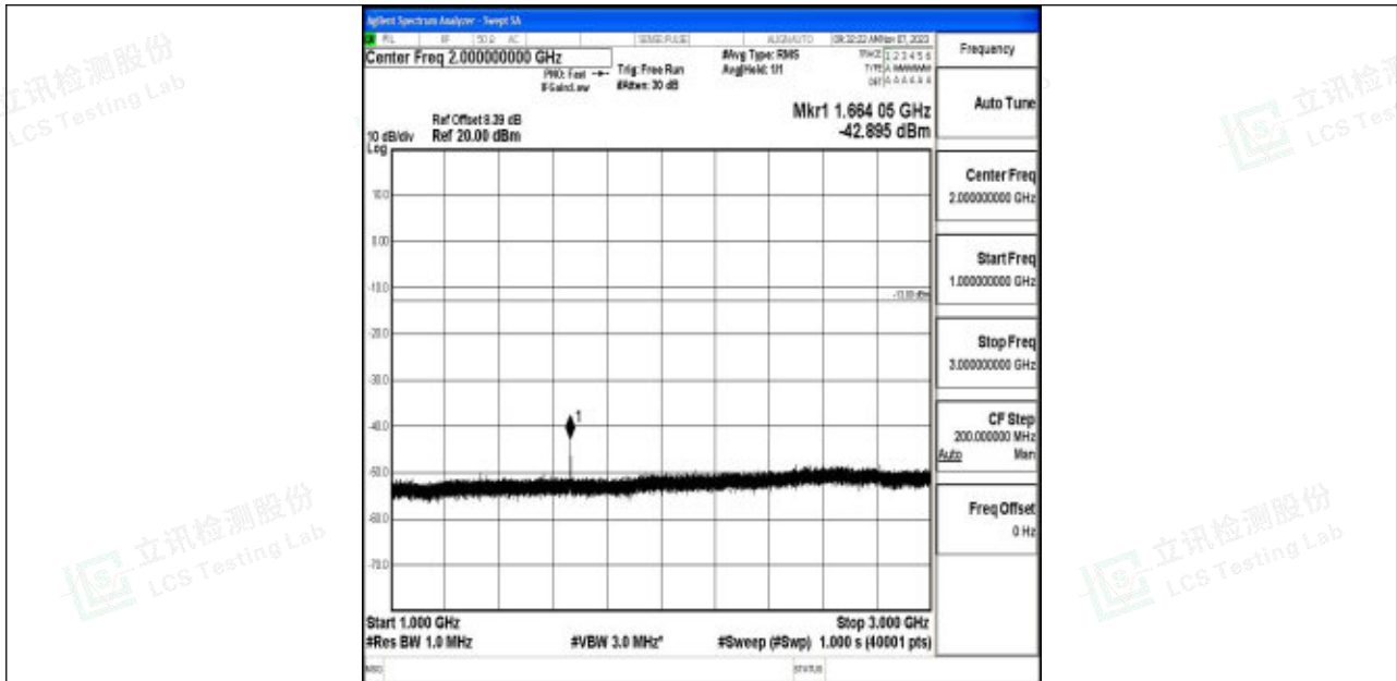
Band5_10MHz_64QAM_20525_1RB#0_1000~3000_1000~3000
