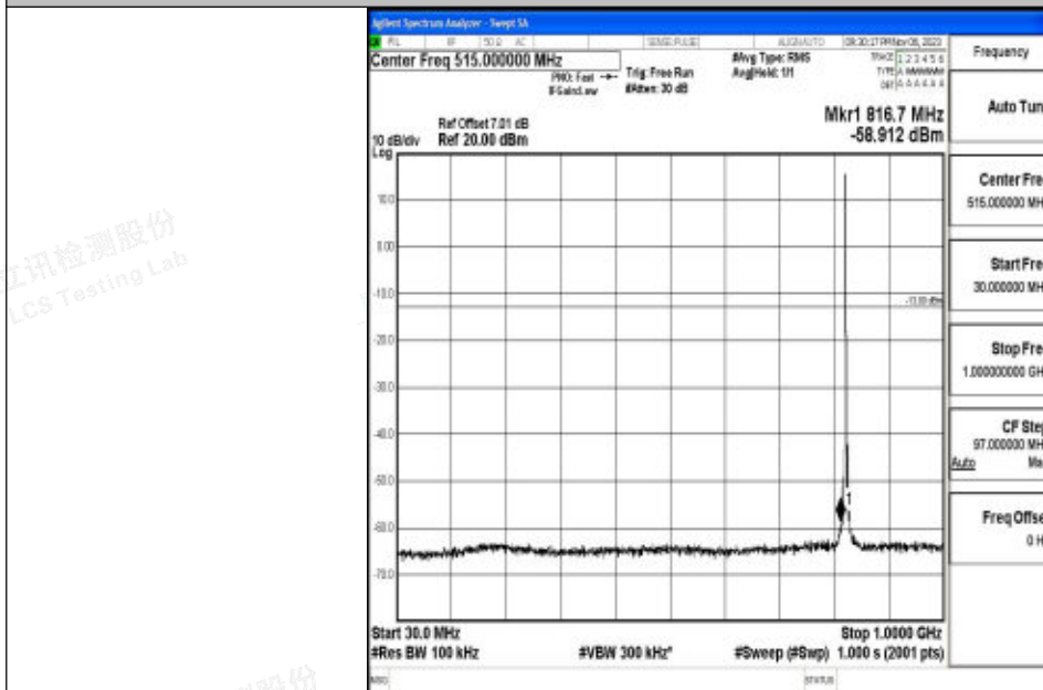
Band5_3MHz_16QAM_20415_1RB#0_30~1000_30~1000
