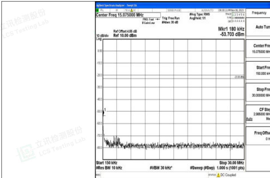
Band5_3MHz_16QAM_20415_1RB#0_0.15~30_0.15~30
