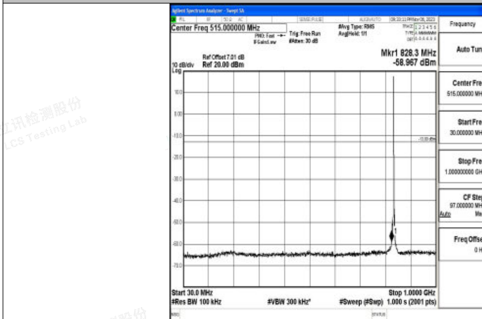
Band5_3MHz_64QAM_20525_1RB#0_30~1000_30~1000
