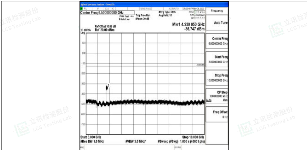
Band5_3MHz_64QAM_20635_1RB#0_3000~10000_3000~10000
