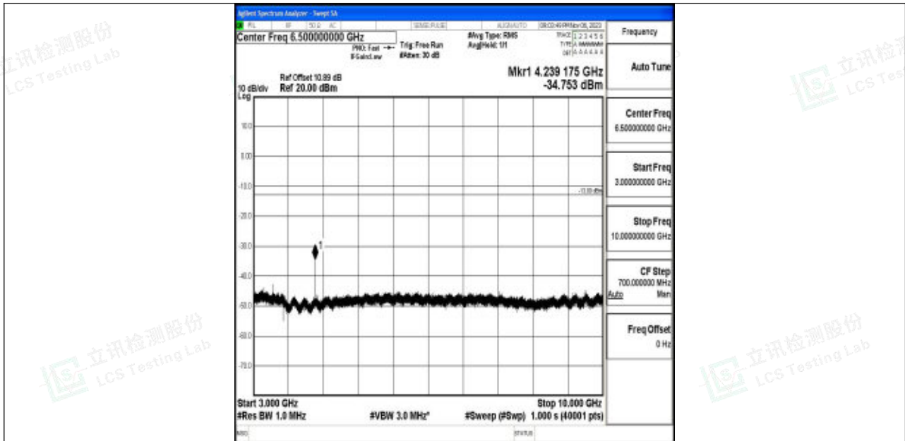
Band5_1.4MHz_16QAM_20643_1RB#0_3000~10000_3000~10000
