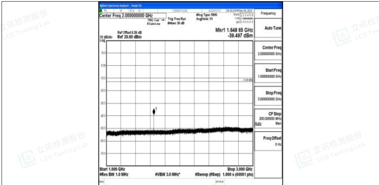
Band5_3MHz_16QAM_20415_1RB#0_1000~3000_1000~3000
