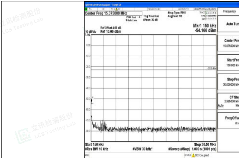
Band5_5MHz_QPSK_20625_1RB#0_0.15~30_0.15~30
