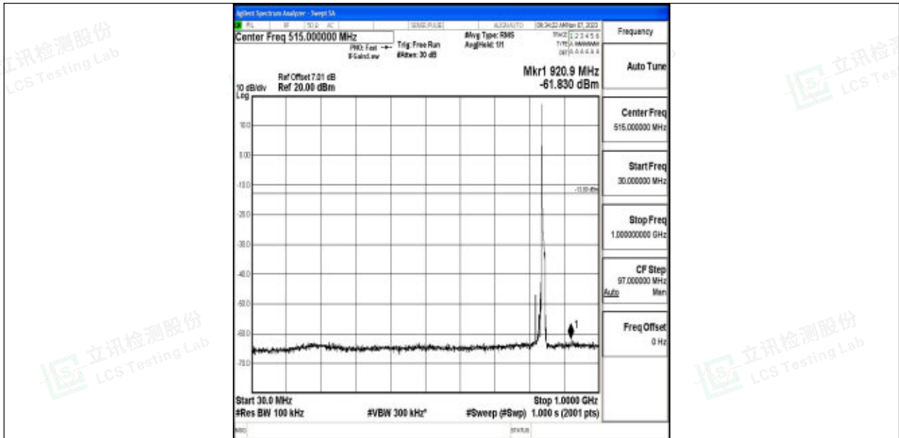
Band5_10MHz_64QAM_20600_1RB#0_30~1000_30~1000
