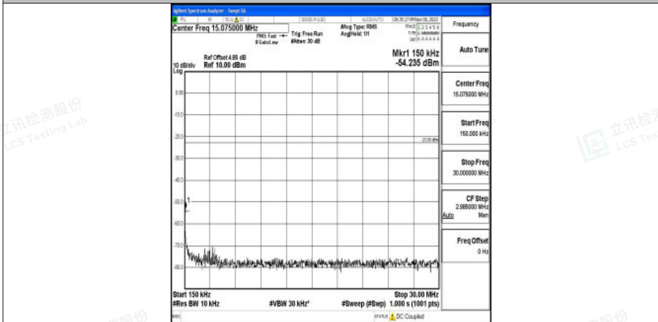
Band5_3MHz_64QAM_20635_1RB#0_0.15~30_0.15~30
