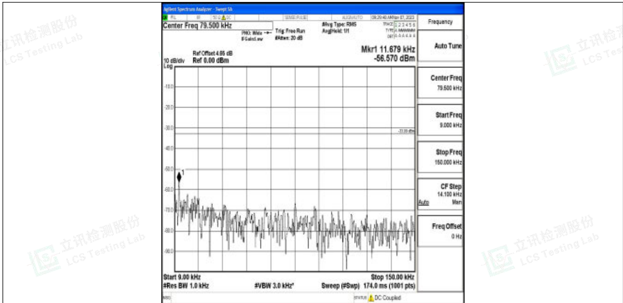
Band5_10MHz_64QAM_20450_1RB#0_0.009~0.15_0.009~0.15
