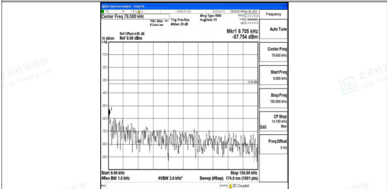
Band5_1.4MHz_16QAM_20525_1RB#0_0.009~0.15_0.009~0.15
