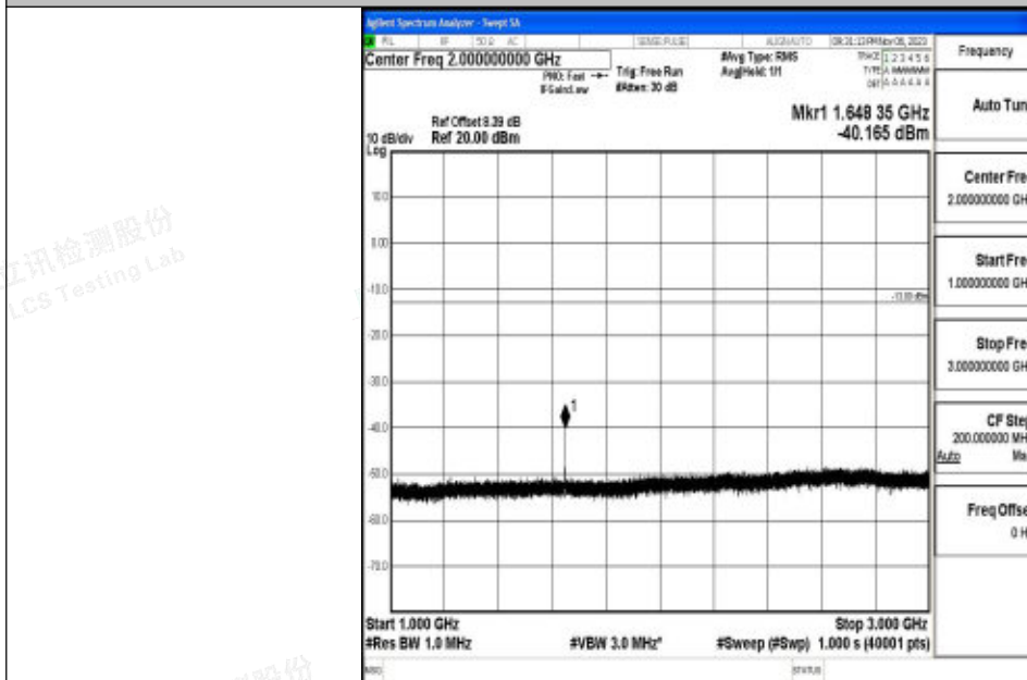
Band5_3MHz_64QAM_20415_1RB#0_1000~3000_1000~3000
