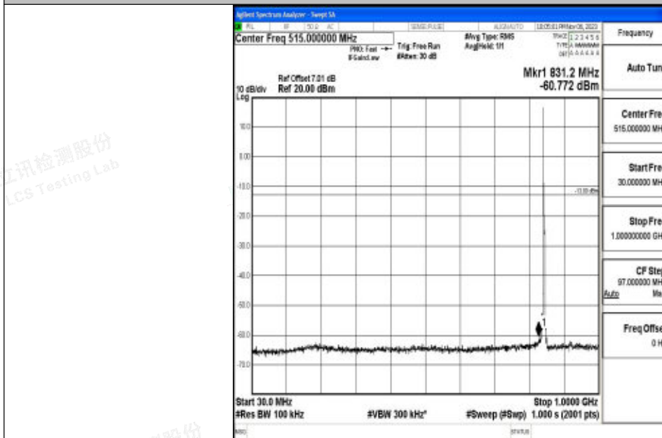
Band5_5MHz_QPSK_20625_1RB#0_30~1000_30~1000
