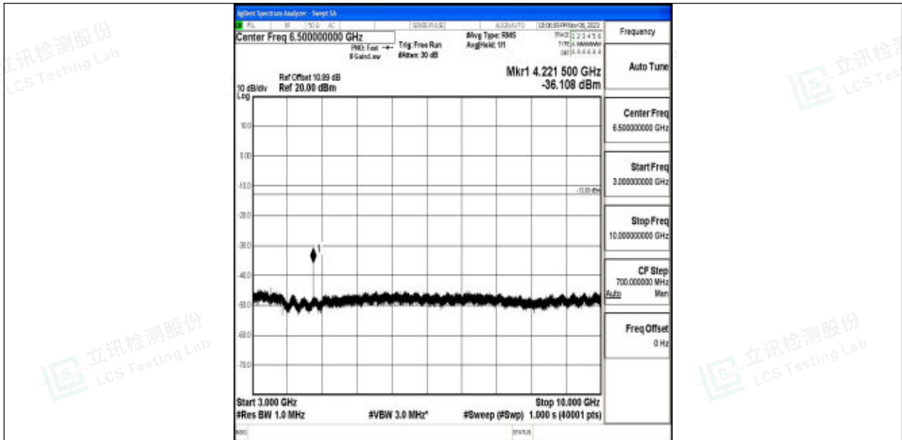
Band5_5MHz_16QAM_20625_1RB#0_3000~10000_3000~10000
