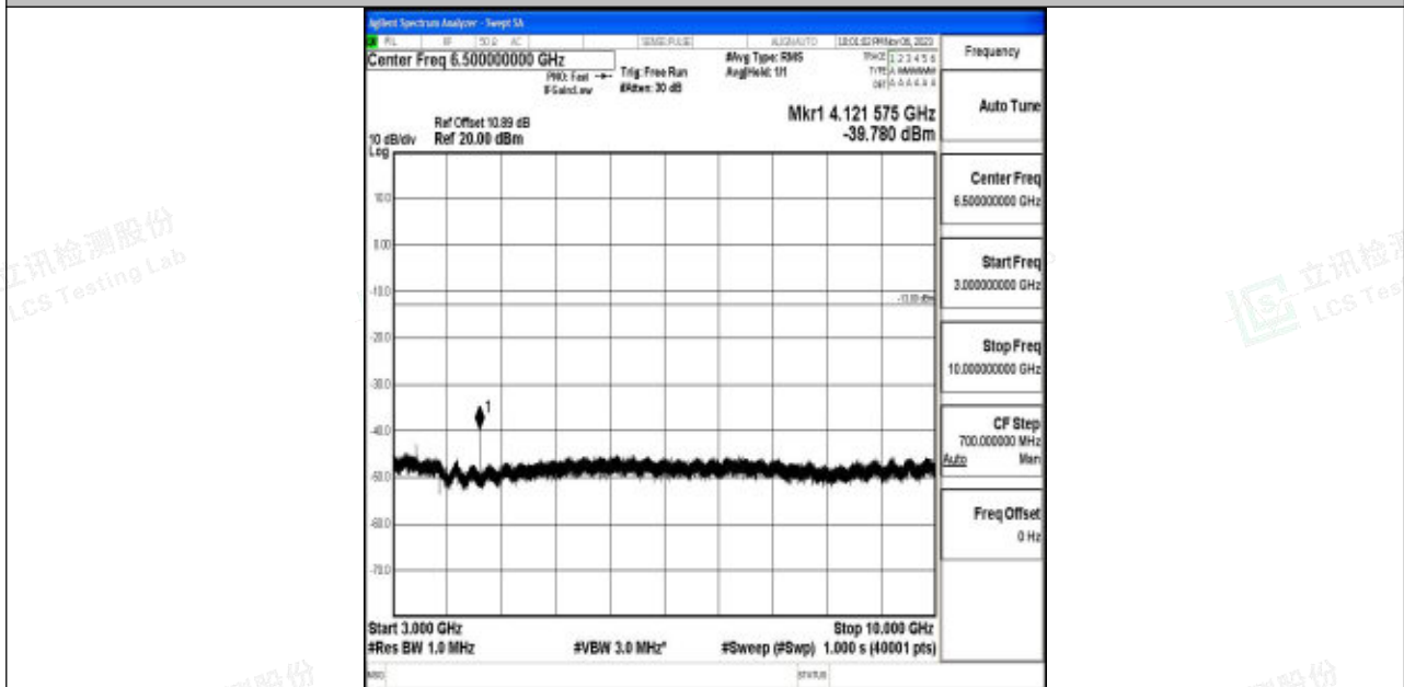
Band5_5MHz_QPSK_20425_1RB#0_3000~10000_3000~10000
