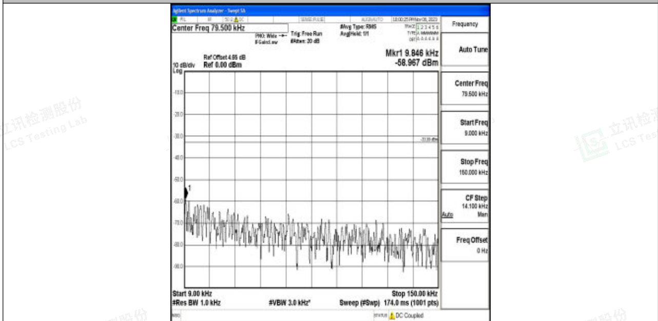
Band5_5MHz_QPSK_20425_1RB#0_0.009~0.15_0.009~0.15
