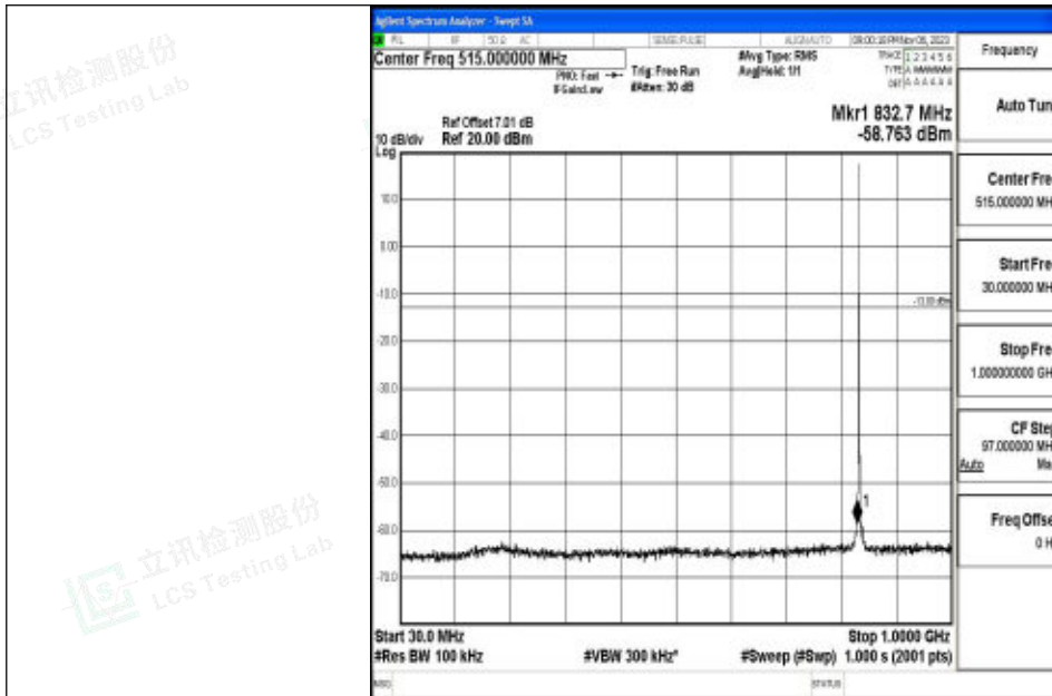
Band5_1.4MHz_QPSK_20525_1RB#0_30~1000_30~1000
