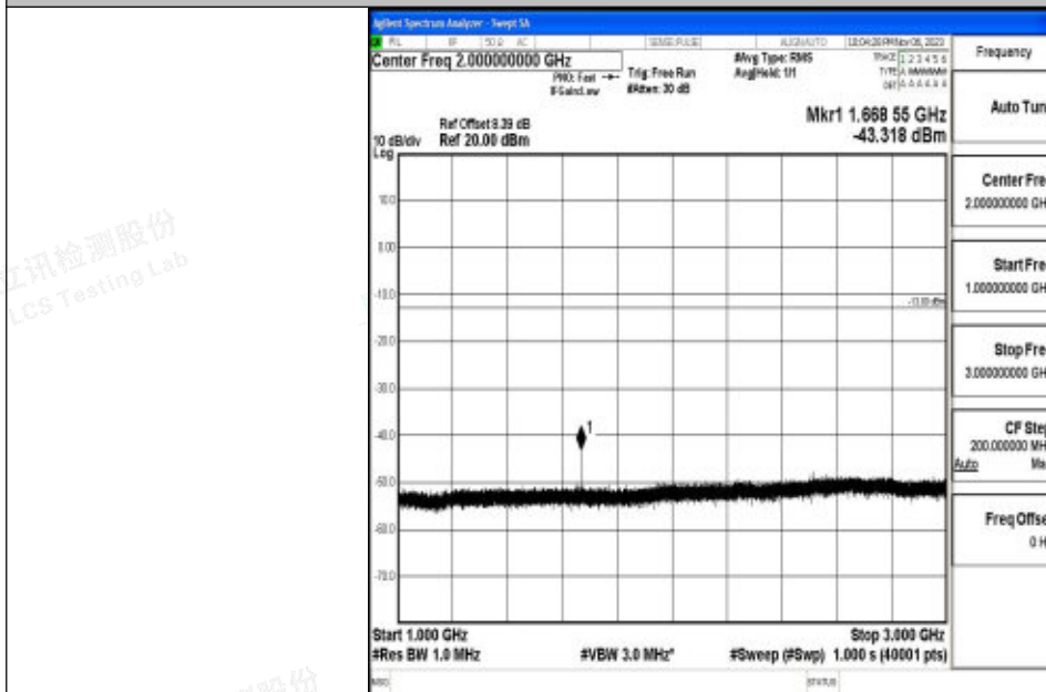
Band5_5MHz_64QAM_20525_1RB#0_1000~3000_1000~3000
