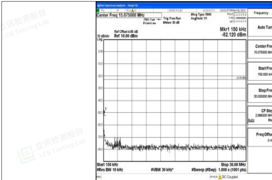
Band5_5MHz_64QAM_20425_1RB#0_0.15~30_0.15~30
