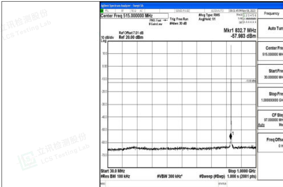
Band5_1.4MHz_64QAM_20525_1RB#0_30~1000_30~1000
