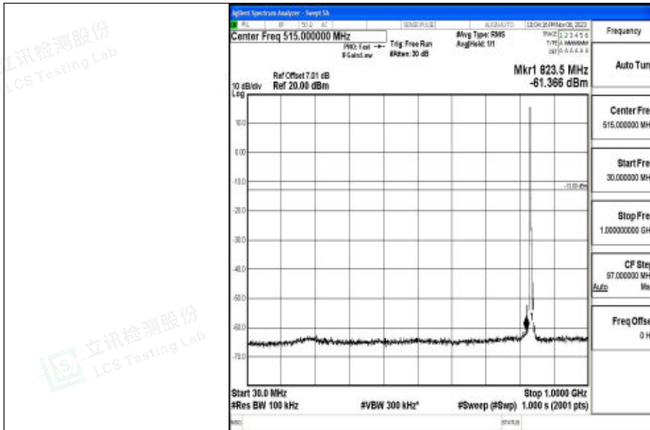
Band5_5MHz_64QAM_20525_1RB#0_30~1000_30~1000
