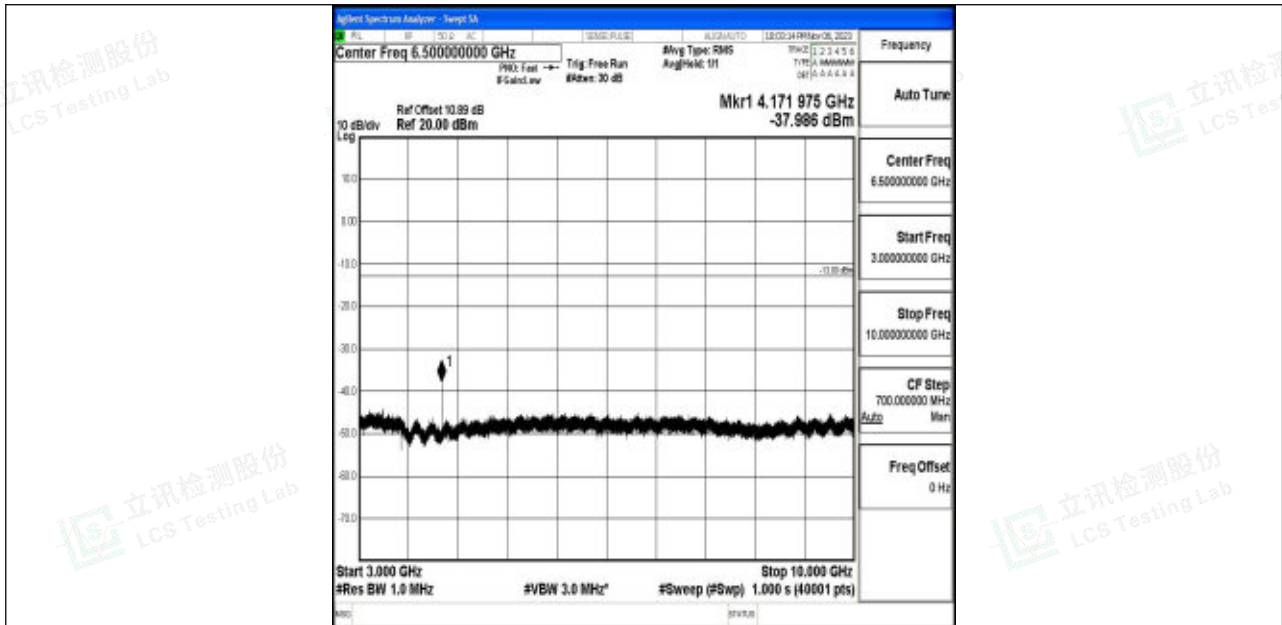
Band5_5MHz_QPSK_20525_1RB#0_3000~10000_3000~10000
