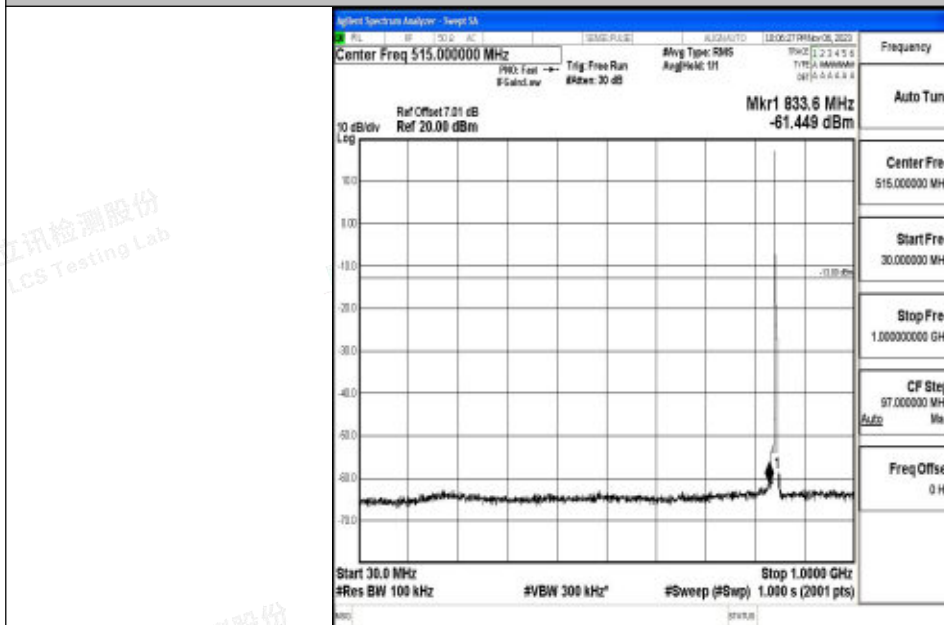
Band5_5MHz_64QAM_20625_1RB#0_30~1000_30~1000
