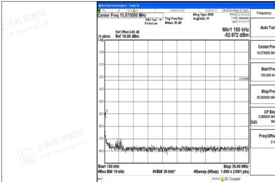
Band5_10MHz_QPSK_20525_1RB#0_0.15~30_0.15~30
