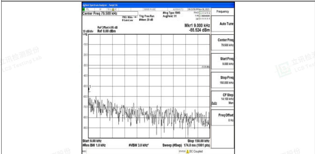
Band5_1.4MHz_64QAM_20643_1RB#0_0.009~0.15_0.009~0.15
