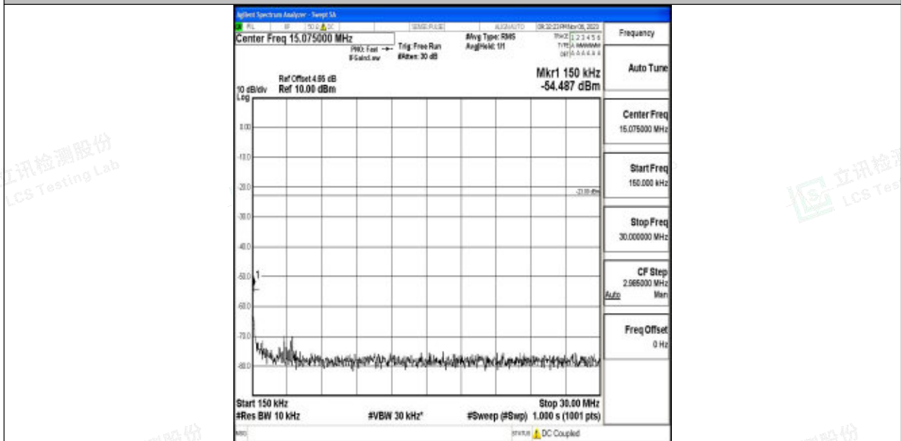
Band5_3MHz_16QAM_20525_1RB#0_0.15~30_0.15~30
