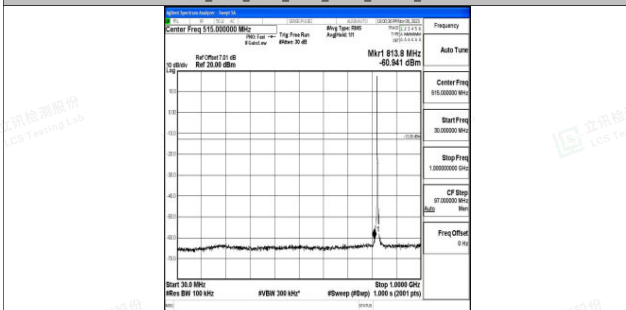
Band5_5MHz_QPSK_20425_1RB#0_30~1000_30~1000
