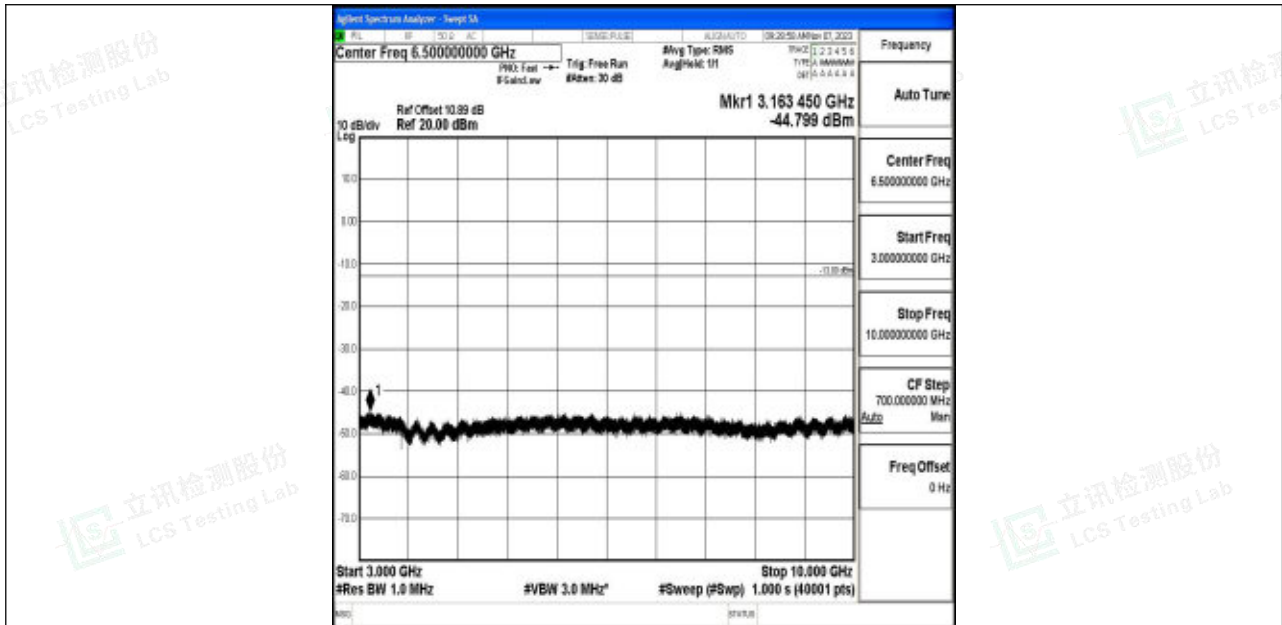
Band5_10MHz_QPSK_20450_1RB#0_3000~10000_3000~10000
