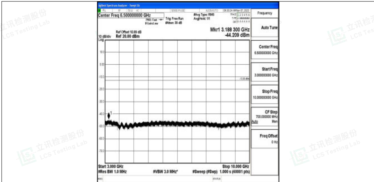
Band5_10MHz_64QAM_20450_1RB#0_3000~10000_3000~10000
