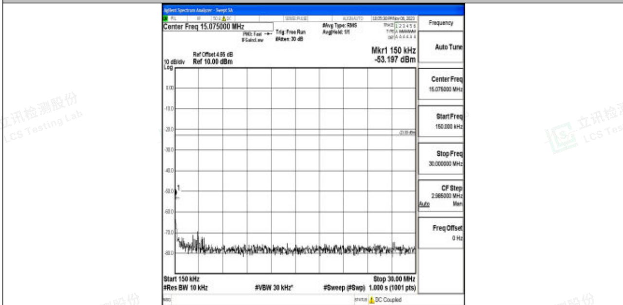
Band5_5MHz_16QAM_20625_1RB#0_0.15~30_0.15~30
