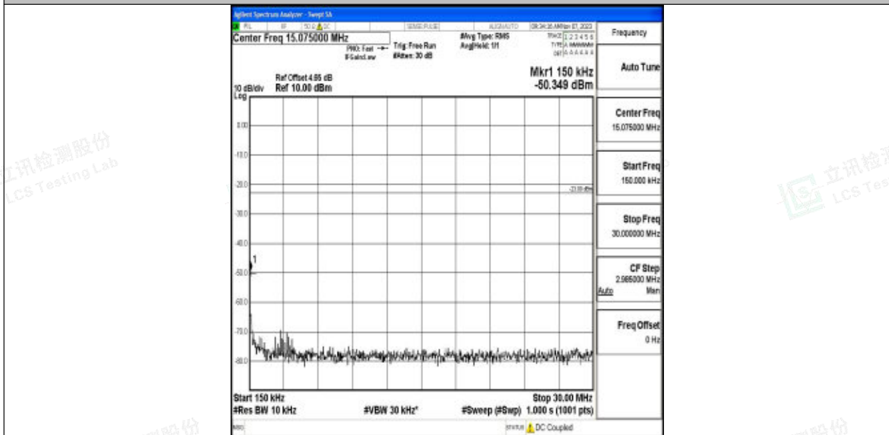
Band5_10MHz_64QAM_20600_1RB#0_0.15~30_0.15~30
