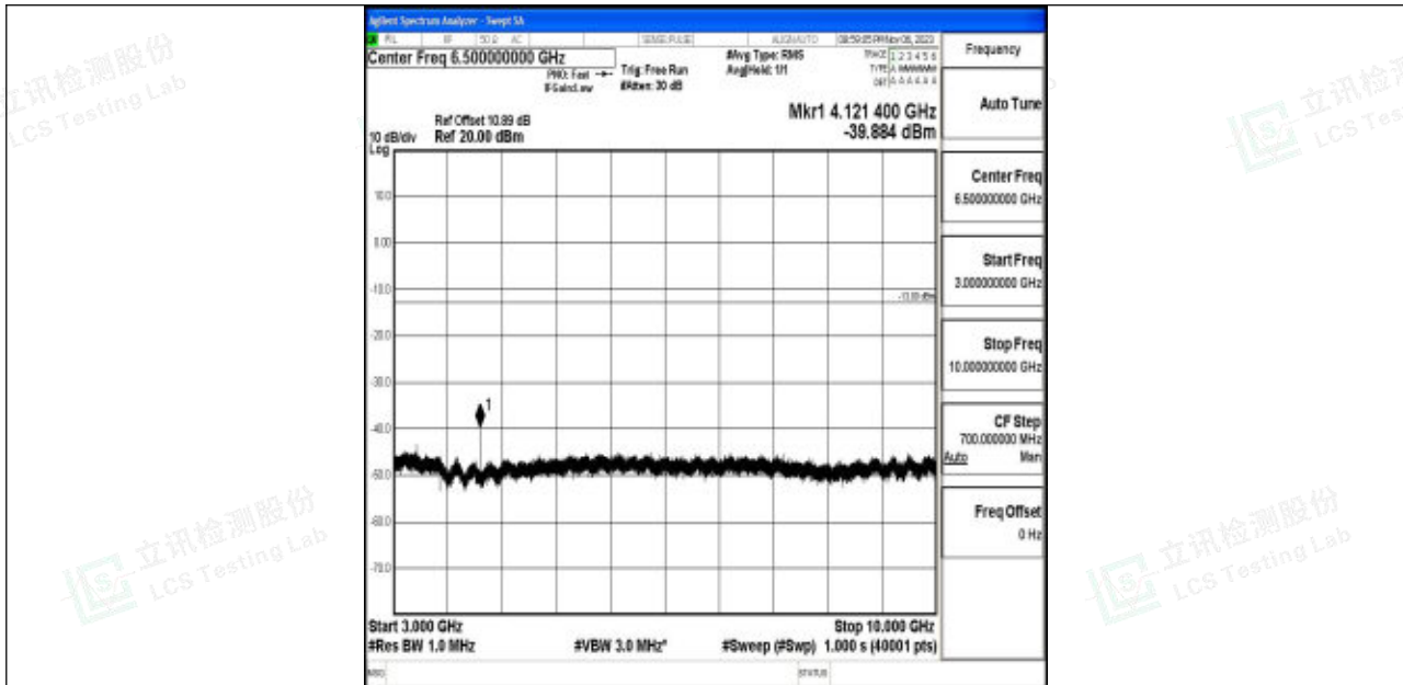
Band5_1.4MHz_16QAM_20407_1RB#0_3000~10000_3000~10000
