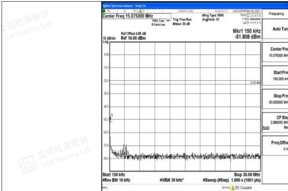
Band5_5MHz_16QAM_20525_1RB#0_0.15~30_0.15~30
