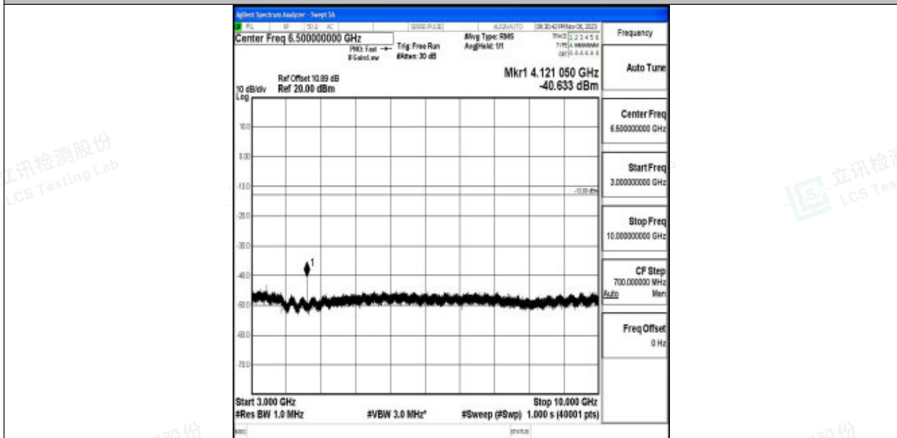
Band5_3MHz_16QAM_20415_1RB#0_3000~10000_3000~10000
