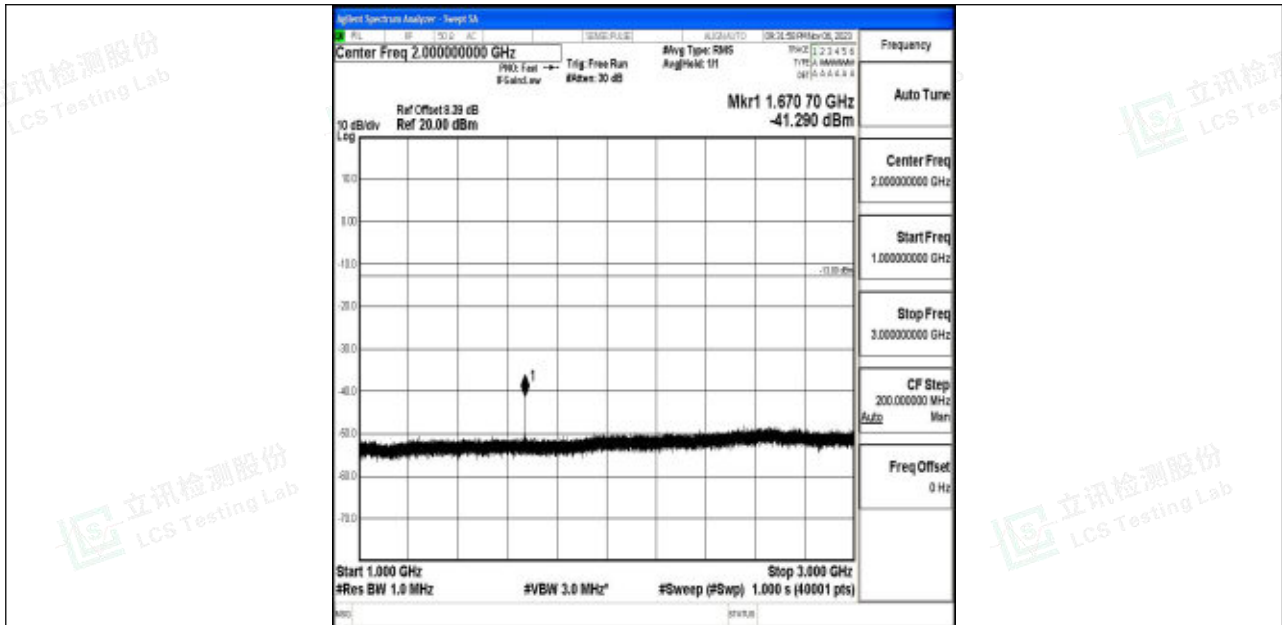
Band5_3MHz_QPSK_20525_1RB#0_1000~3000_1000~3000
