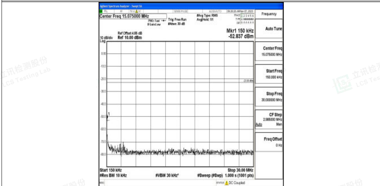
Band5_10MHz_QPSK_20450_1RB#0_0.15~30_0.15~30
