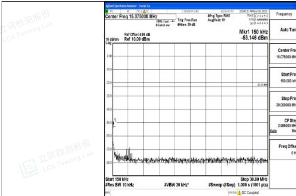
Band5_5MHz_64QAM_20625_1RB#0_0.15~30_0.15~30
