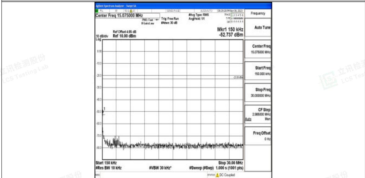
Band5_3MHz_QPSK_20415_1RB#0_0.15~30_0.15~30
