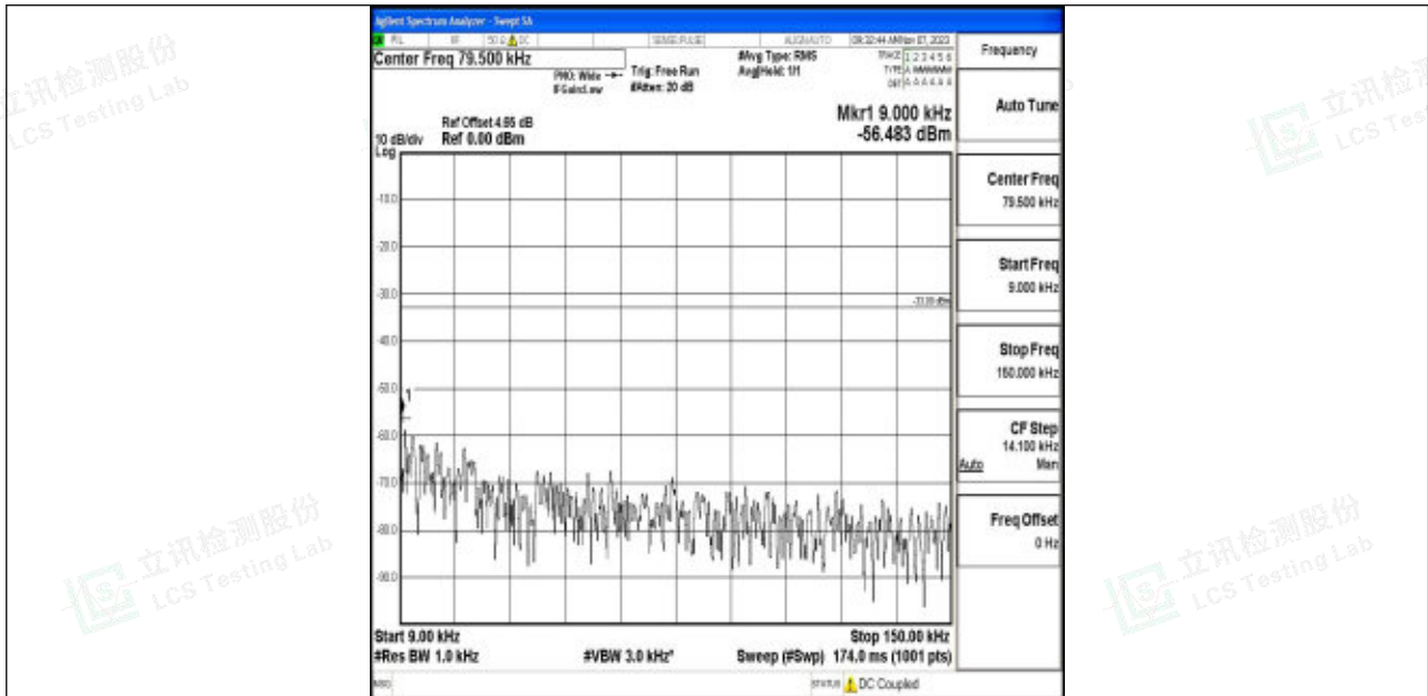
Band5_10MHz_QPSK_20600_1RB#0_0.009~0.15_0.009~0.15
