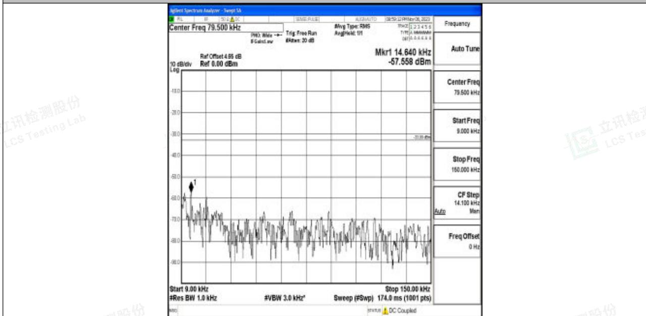
Band5_1.4MHz_64QAM_20407_1RB#0_0.009~0.15_0.009~0.15
