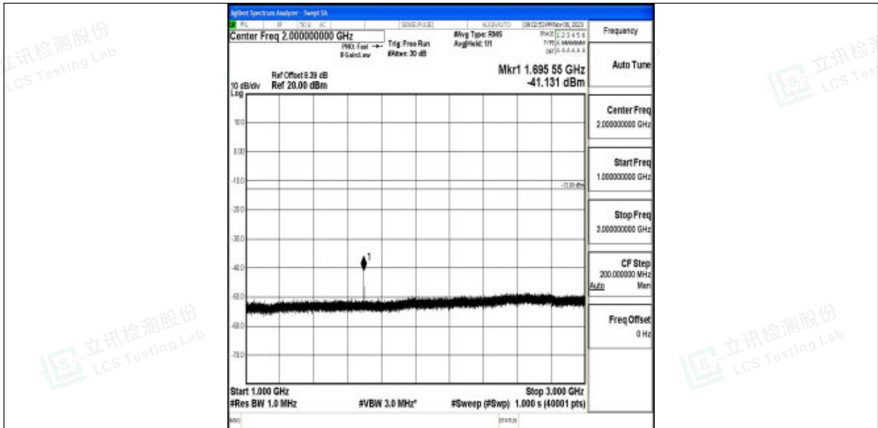
Band5_1.4MHz_QPSK_20643_1RB#0_1000~3000_1000~3000
