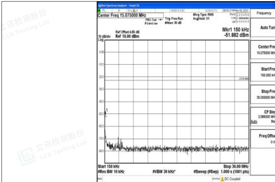
Band5_1.4MHz_64QAM_20407_1RB#0_0.15~30_0.15~30
