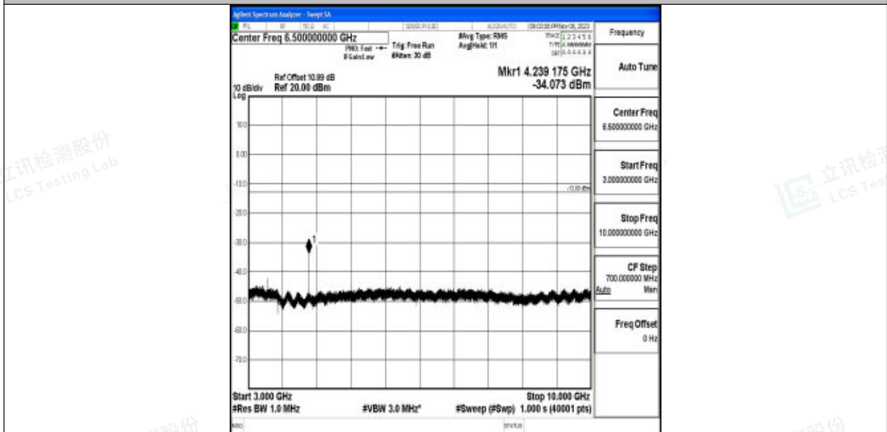
Band5_1.4MHz_QPSK_20643_1RB#0_3000~10000_3000~10000
