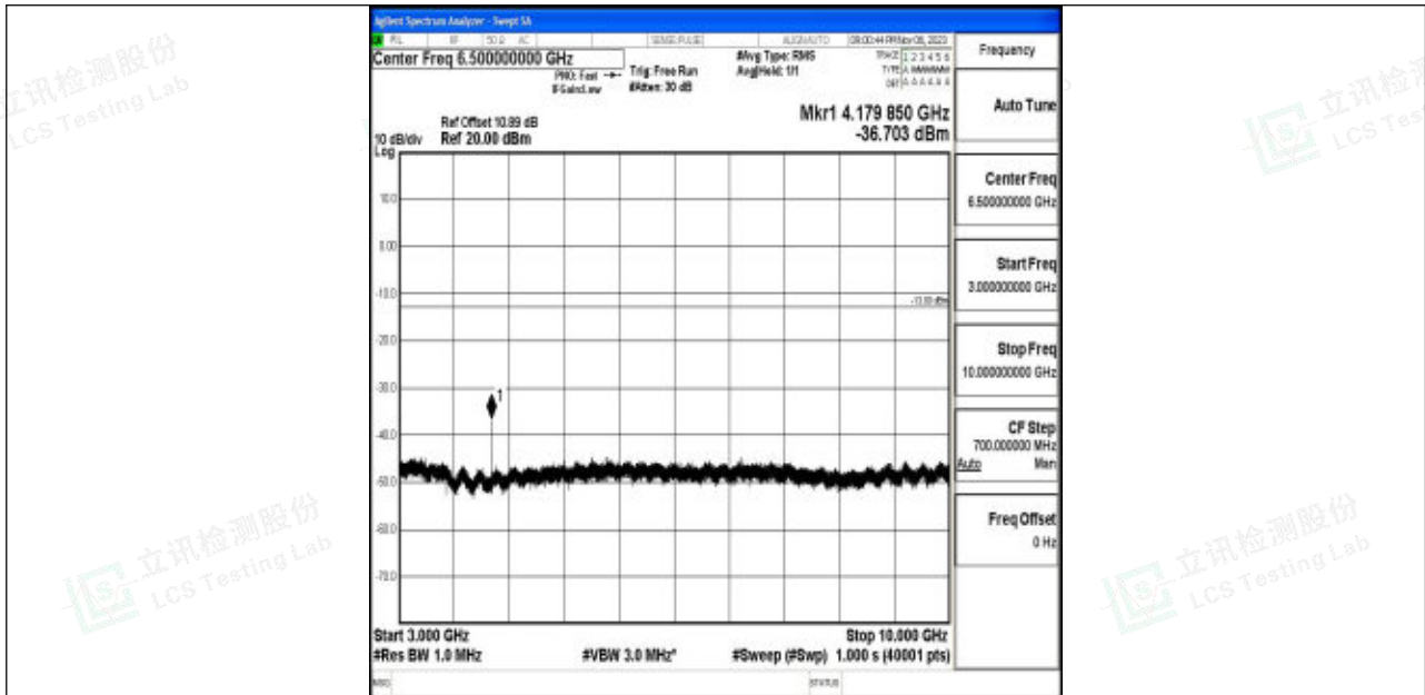
Band5_1.4MHz_QPSK_20525_1RB#0_3000~10000_3000~10000
