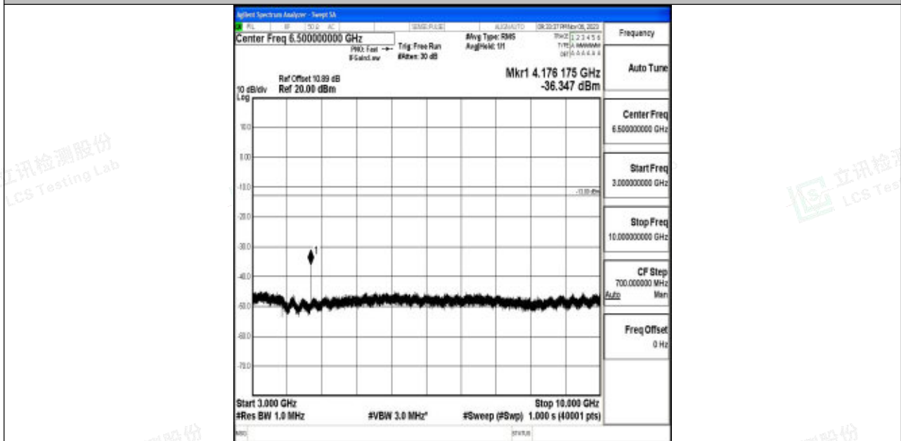
Band5_3MHz_64QAM_20525_1RB#0_3000~10000_3000~10000
