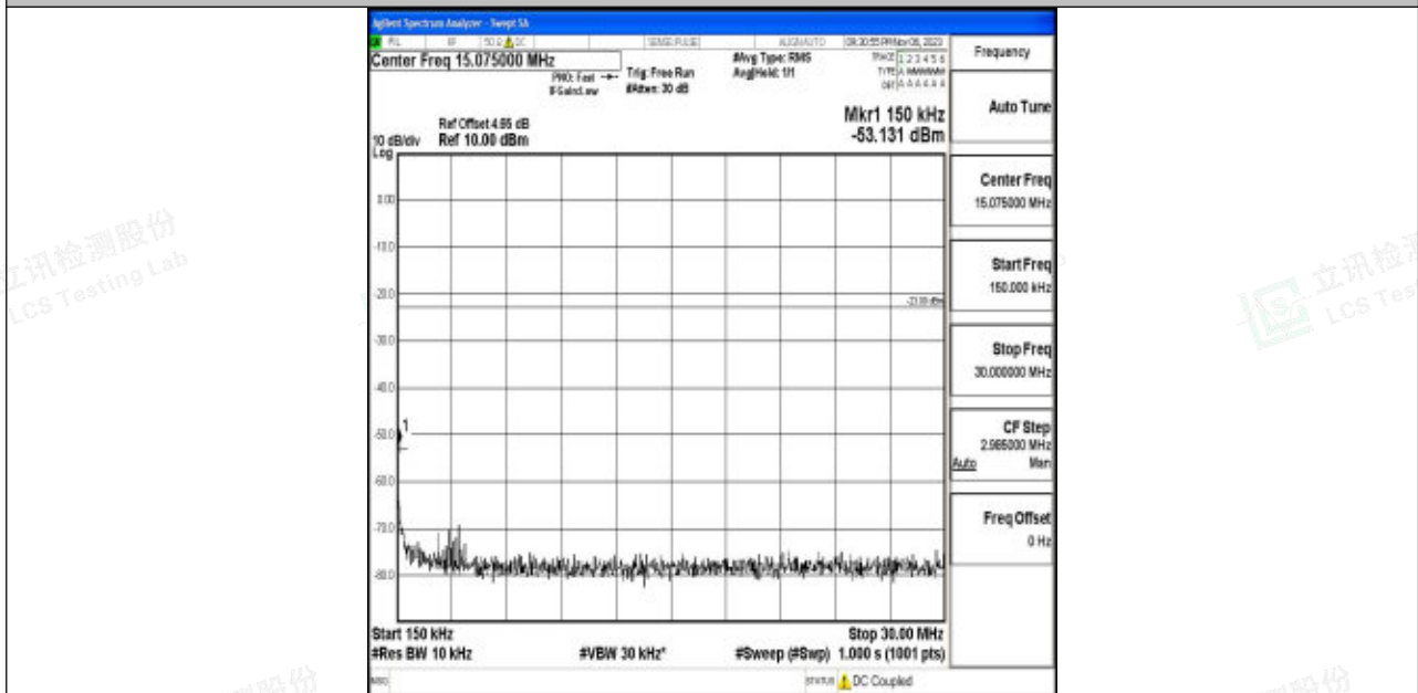
Band5_3MHz_64QAM_20415_1RB#0_0.15~30_0.15~30
