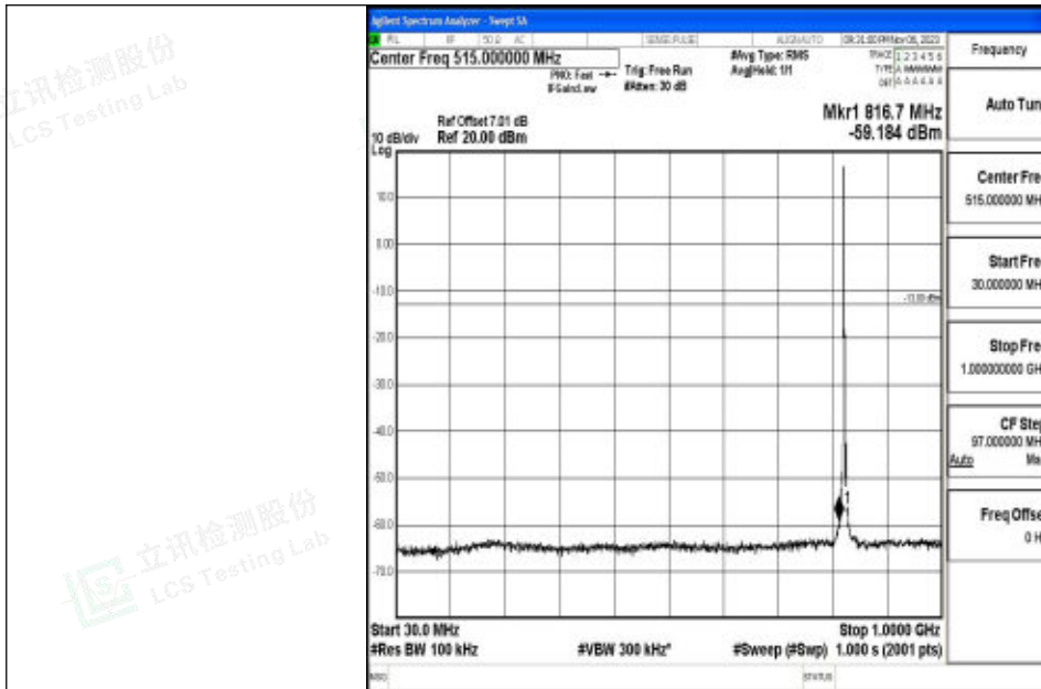
Band5_3MHz_64QAM_20415_1RB#0_30~1000_30~1000
