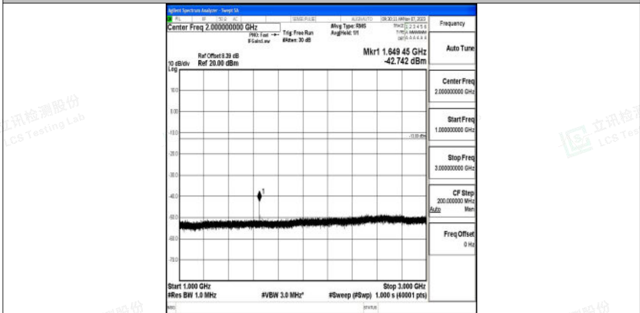
Band5_10MHz_64QAM_20450_1RB#0_1000~3000_1000~3000
