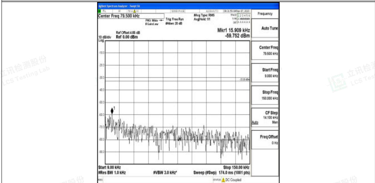
Band5_10MHz_64QAM_20525_1RB#0_0.009~0.15_0.009~0.15
