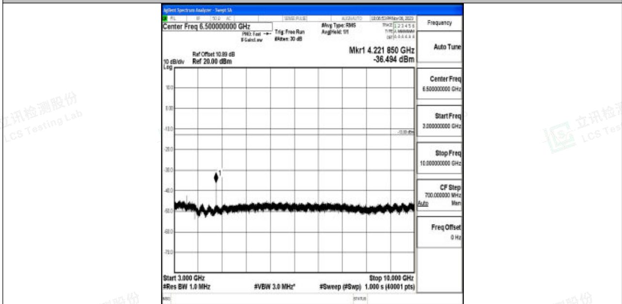
Band5_5MHz_64QAM_20625_1RB#0_3000~10000_3000~10000
