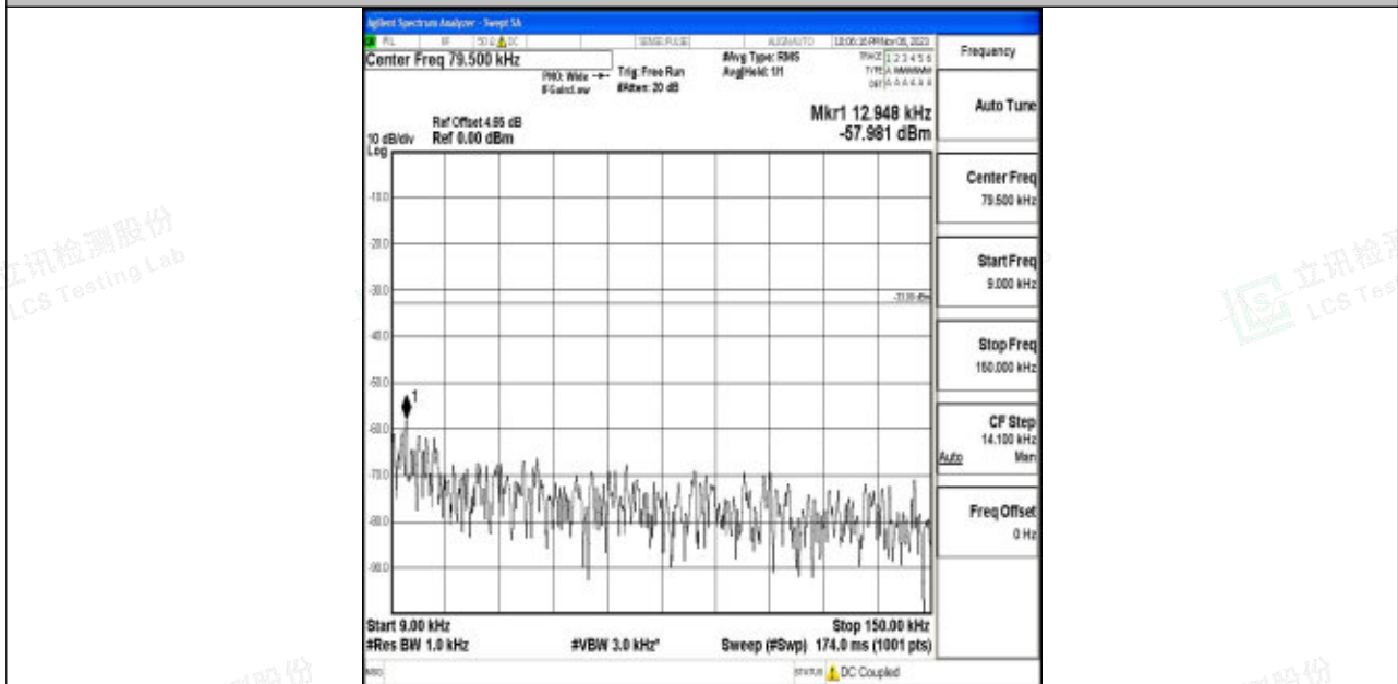
Band5_5MHz_64QAM_20625_1RB#0_0.009~0.15_0.009~0.15
