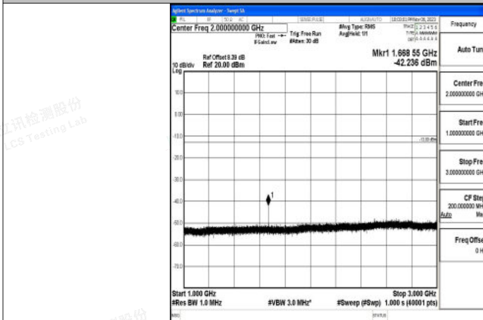
Band5_5MHz_QPSK_20525_1RB#0_1000~3000_1000~3000
