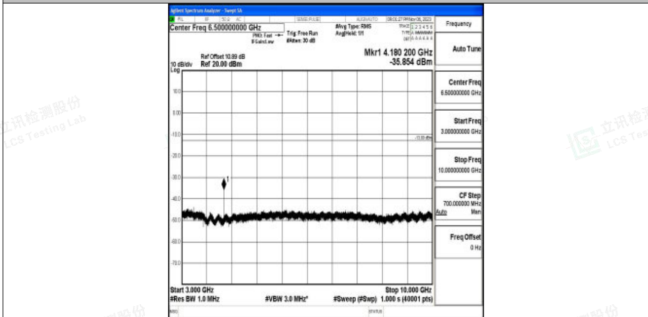
Band5_1.4MHz_16QAM_20525_1RB#0_3000~10000_3000~10000
