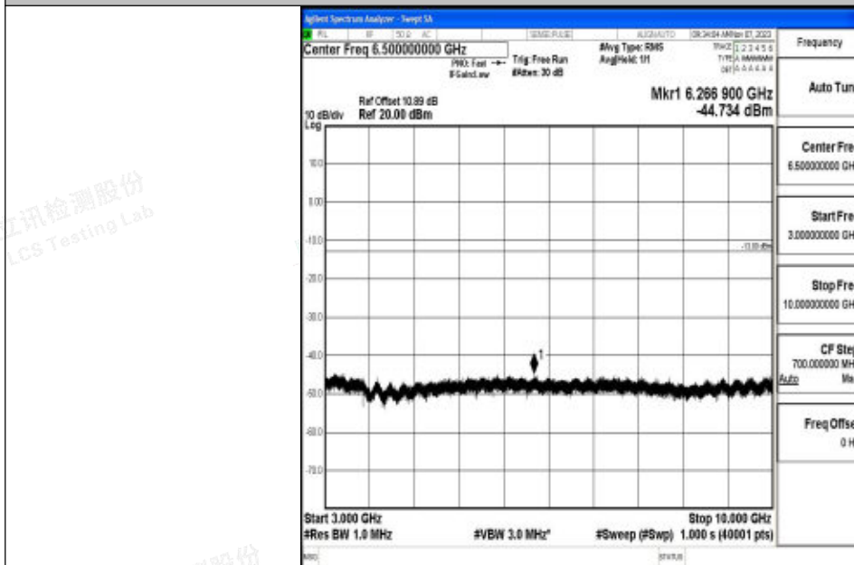
Band5_10MHz_16QAM_20600_1RB#0_3000~10000_3000~10000
