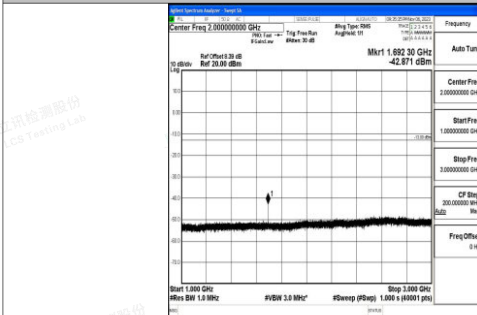
Band5_3MHz_64QAM_20635_1RB#0_1000~3000_1000~3000
