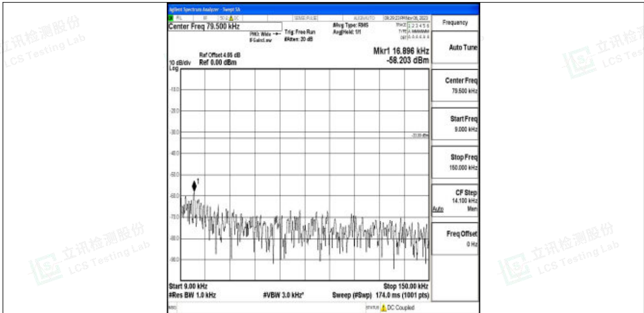
Band5_3MHz_QPSK_20415_1RB#0_0.009~0.15_0.009~0.15
