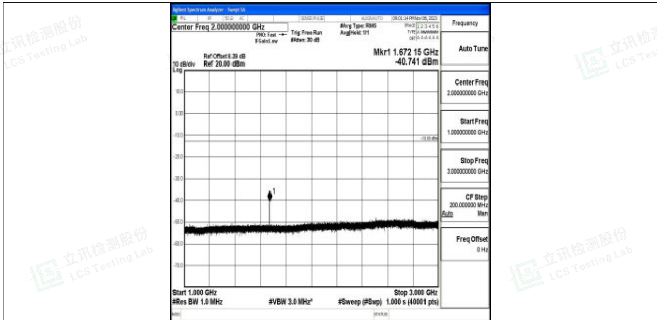
Band5_1.4MHz_16QAM_20525_1RB#0_1000~3000_1000~3000
