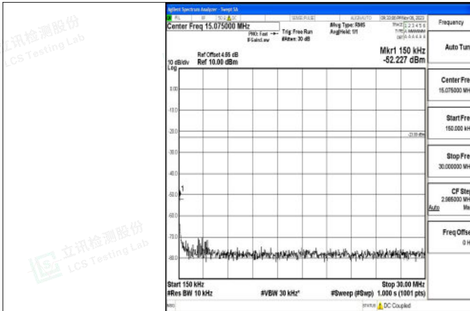
Band5_3MHz_64QAM_20525_1RB#0_0.15~30_0.15~30
