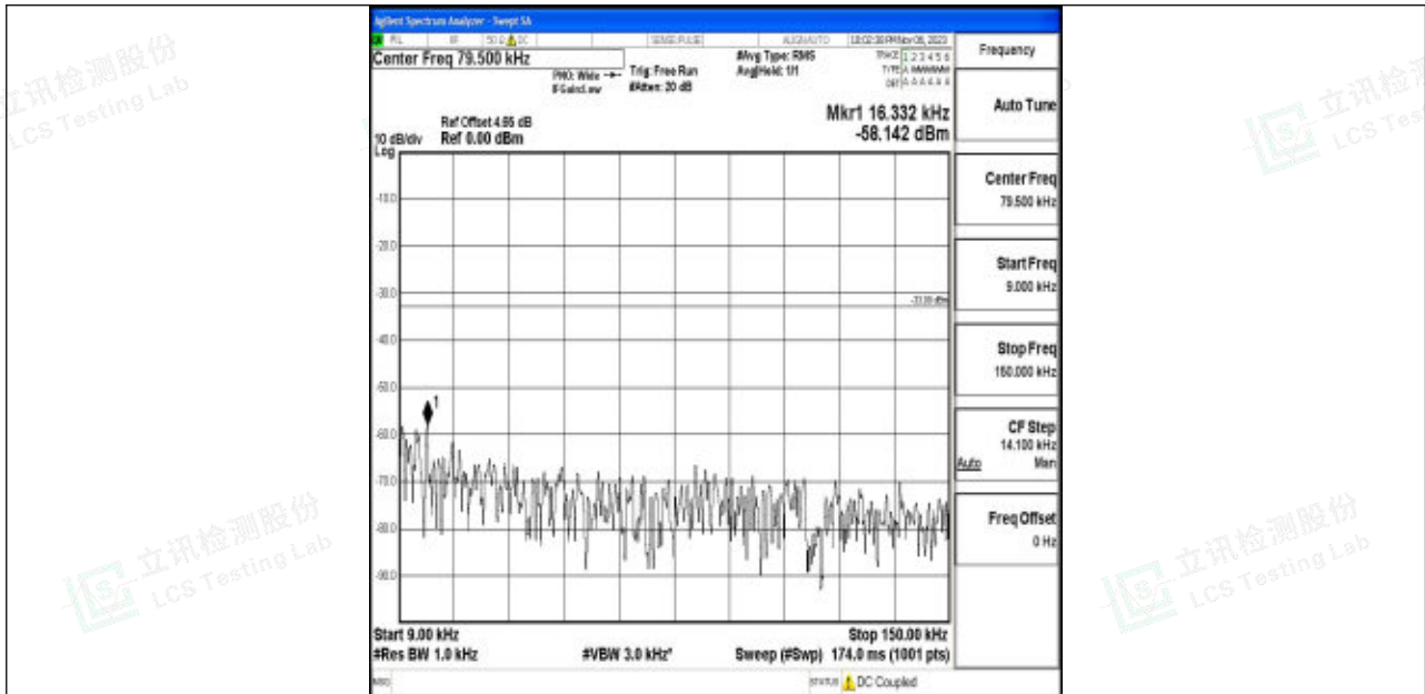
Band5_5MHz_QPSK_20525_1RB#0_0.009~0.15_0.009~0.15
