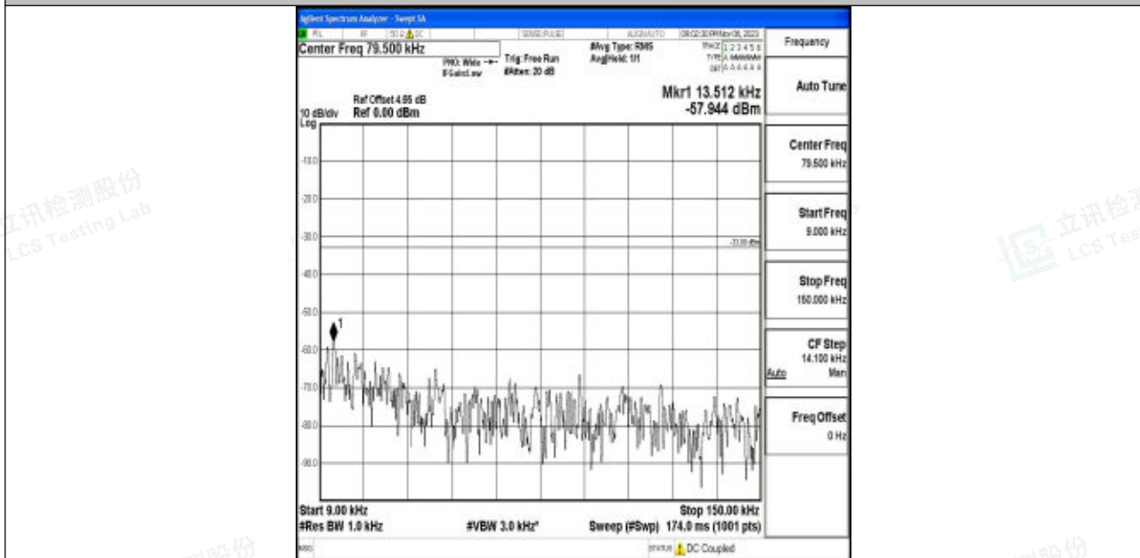
Band5_1.4MHz_QPSK_20643_1RB#0_0.009~0.15_0.009~0.15
