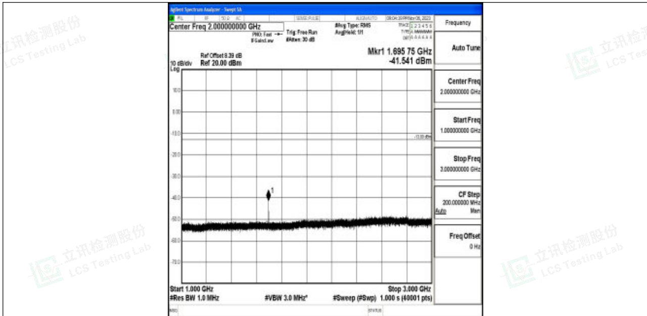
Band5_1.4MHz_64QAM_20643_1RB#0_1000~3000_1000~3000
