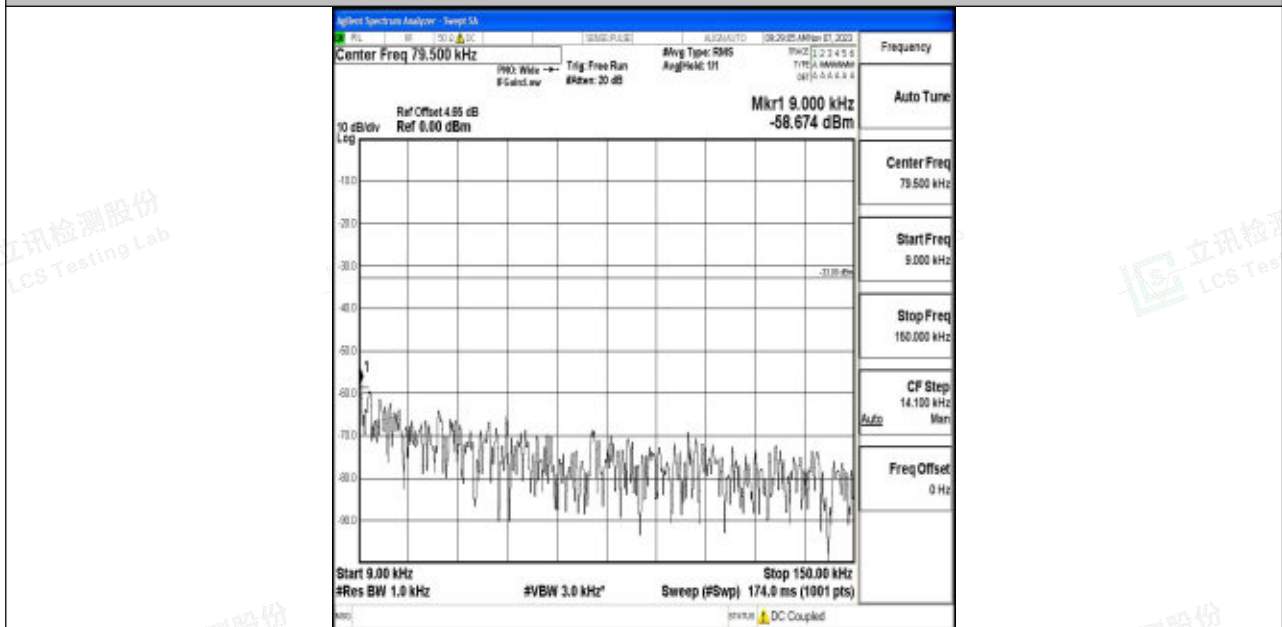
Band5_10MHz_16QAM_20450_1RB#0_0.009~0.15_0.009~0.15
