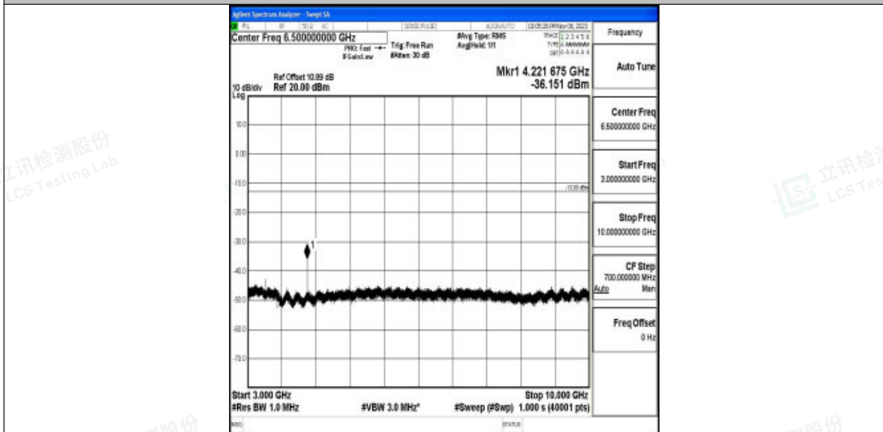
Band5_5MHz_QPSK_20625_1RB#0_3000~10000_3000~10000
