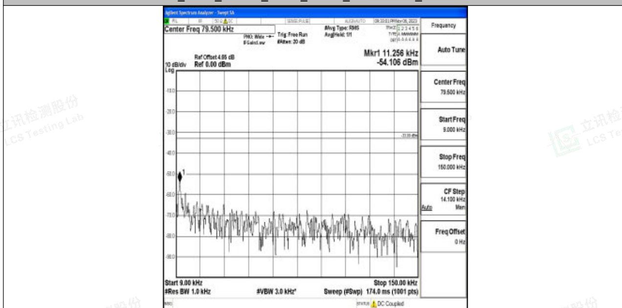
Band5_3MHz_64QAM_20525_1RB#0_0.009~0.15_0.009~0.15
