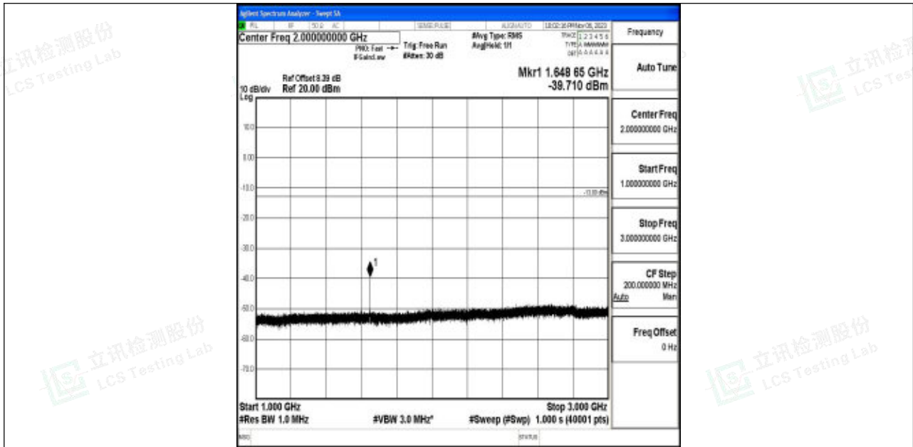
Band5_5MHz_64QAM_20425_1RB#0_1000~3000_1000~3000
