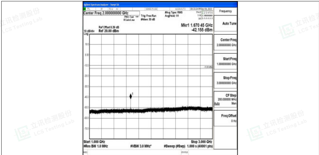
Band5_3MHz_64QAM_20525_1RB#0_1000~3000_1000~3000
