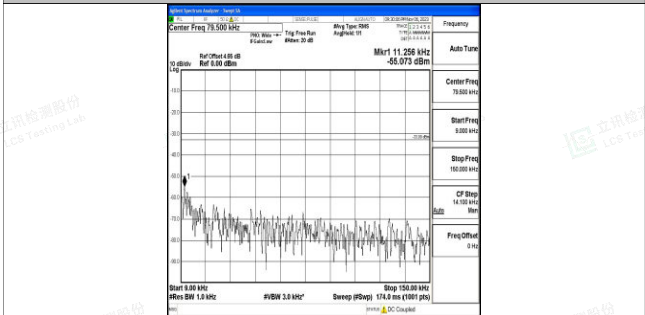
Band5_3MHz_16QAM_20415_1RB#0_0.009~0.15_0.009~0.15
