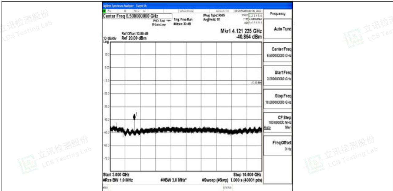
Band5_3MHz_QPSK_20415_1RB#0_3000~10000_3000~10000
