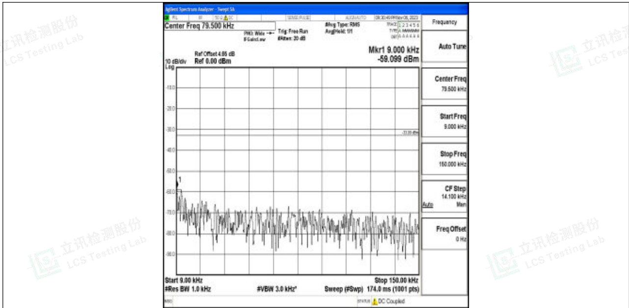
Band5_3MHz_64QAM_20415_1RB#0_0.009~0.15_0.009~0.15
