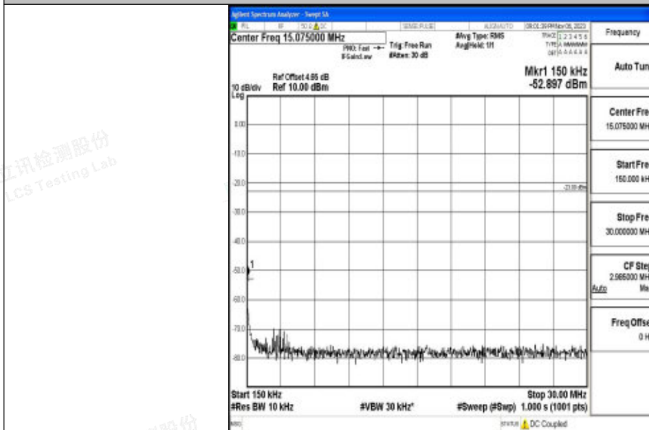
Band5_1.4MHz_64QAM_20525_1RB#0_0.15~30_0.15~30
