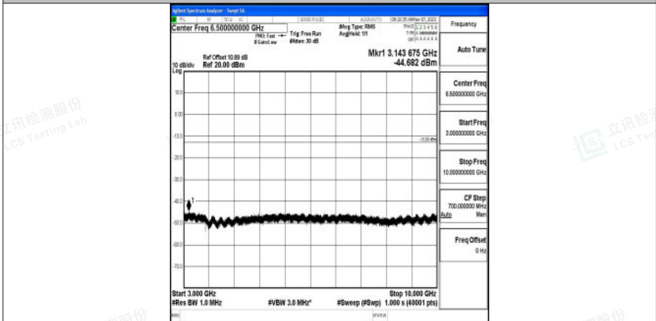
Band5_10MHz_64QAM_20525_1RB#0_3000~10000_3000~10000
