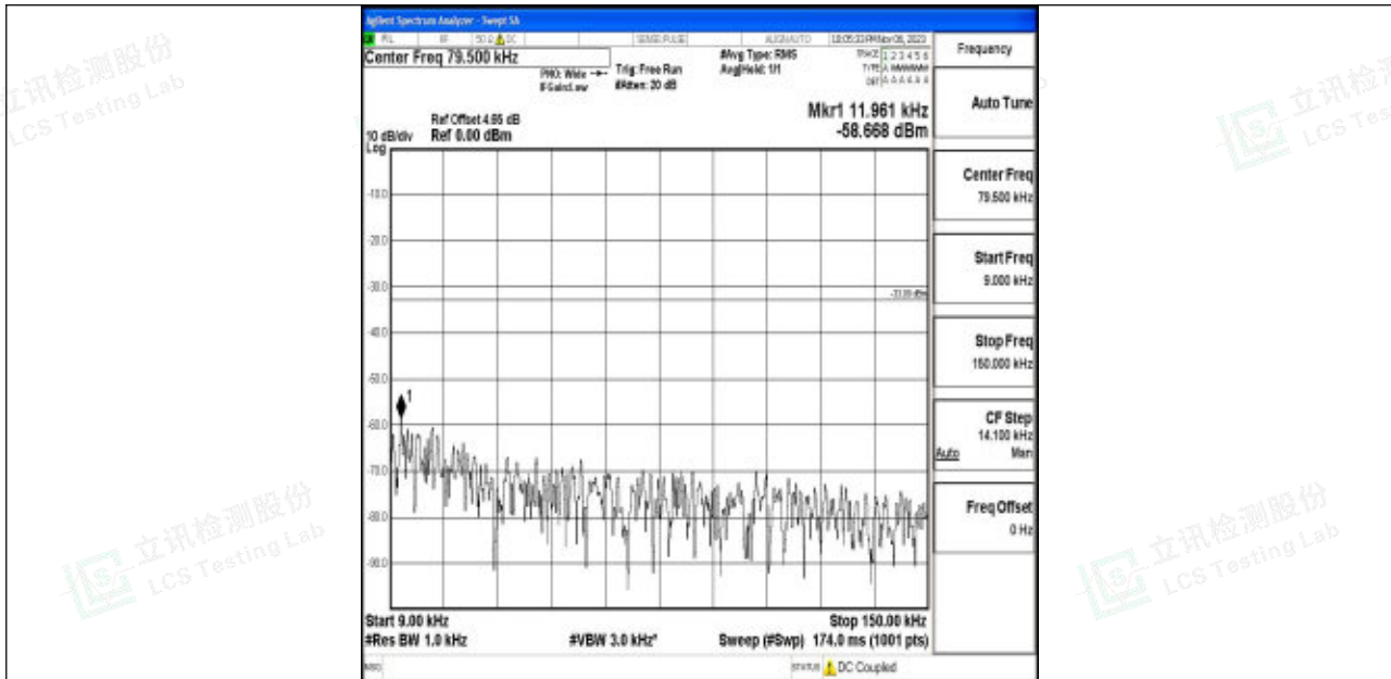
Band5_5MHz_16QAM_20625_1RB#0_0.009~0.15_0.009~0.15
