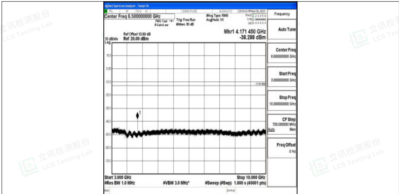
Band5_5MHz_64QAM_20525_1RB#0_3000~10000_3000~10000
