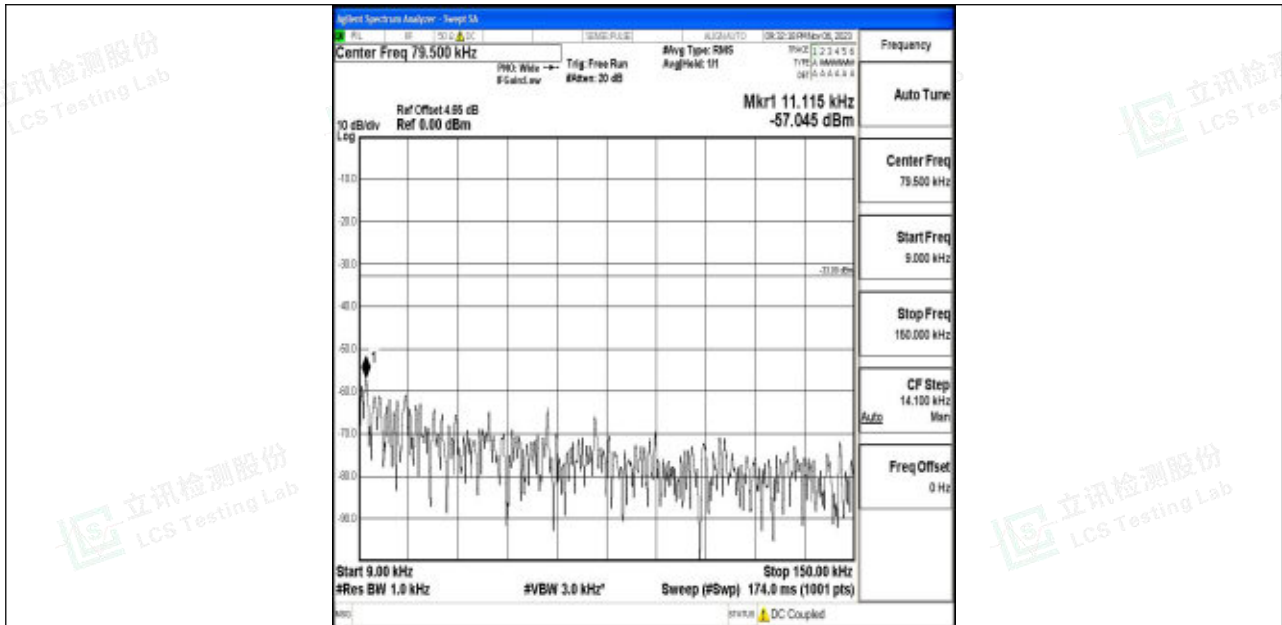
Band5_3MHz_16QAM_20525_1RB#0_0.009~0.15_0.009~0.15
