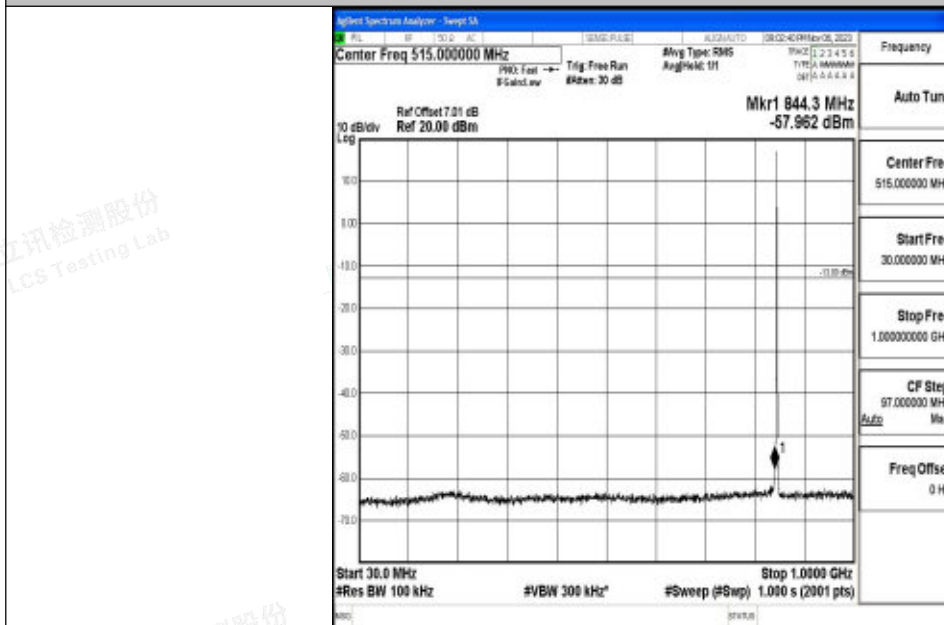
Band5_1.4MHz_QPSK_20643_1RB#0_30~1000_30~1000
