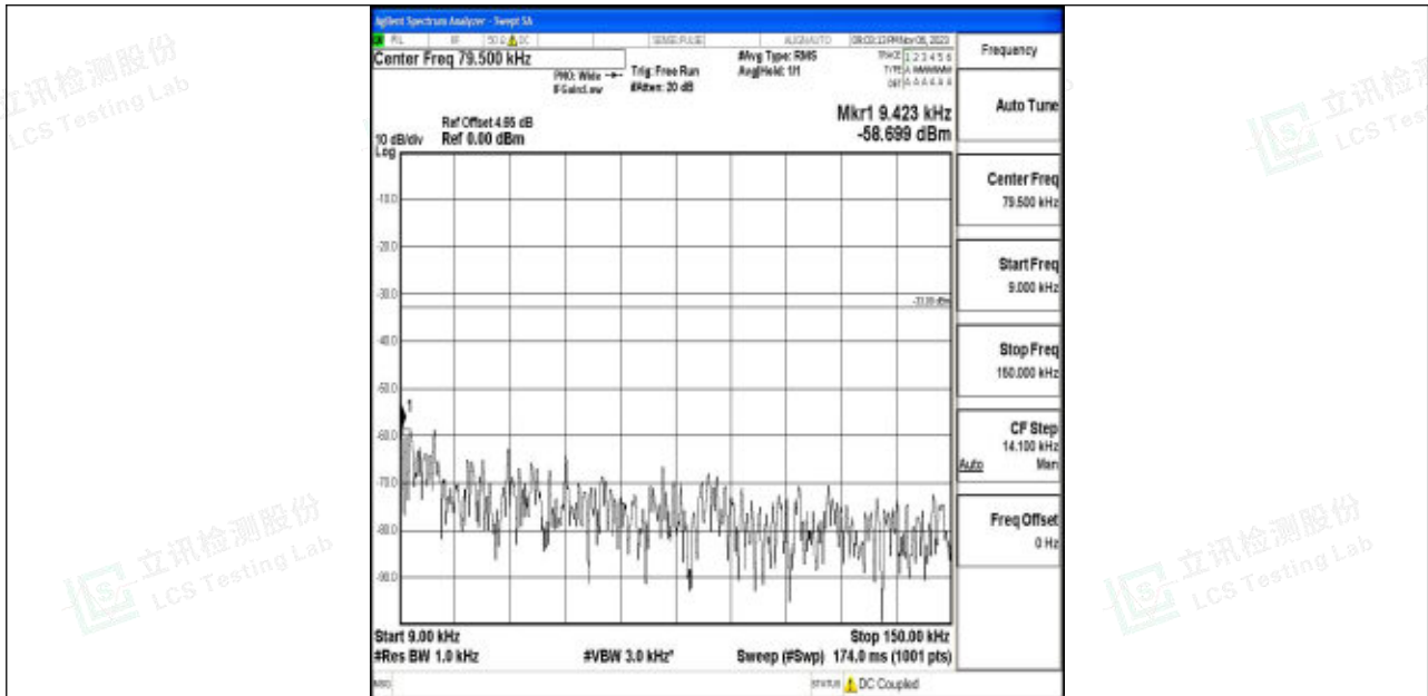
Band5_1.4MHz_16QAM_20643_1RB#0_0.009~0.15_0.009~0.15
