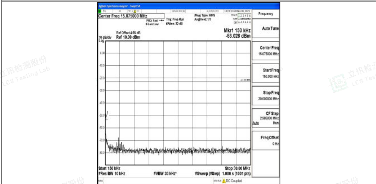
Band5_5MHz_16QAM_20425_1RB#0_0.15~30_0.15~30
