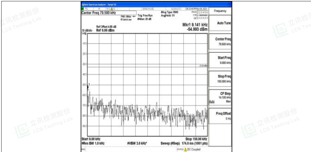
Band5_3MHz_QPSK_20635_1RB#0_0.009~0.15_0.009~0.15
