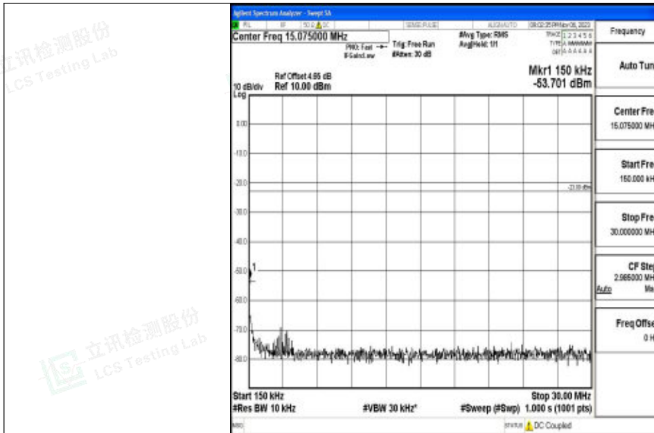
Band5_1.4MHz_QPSK_20643_1RB#0_0.15~30_0.15~30
