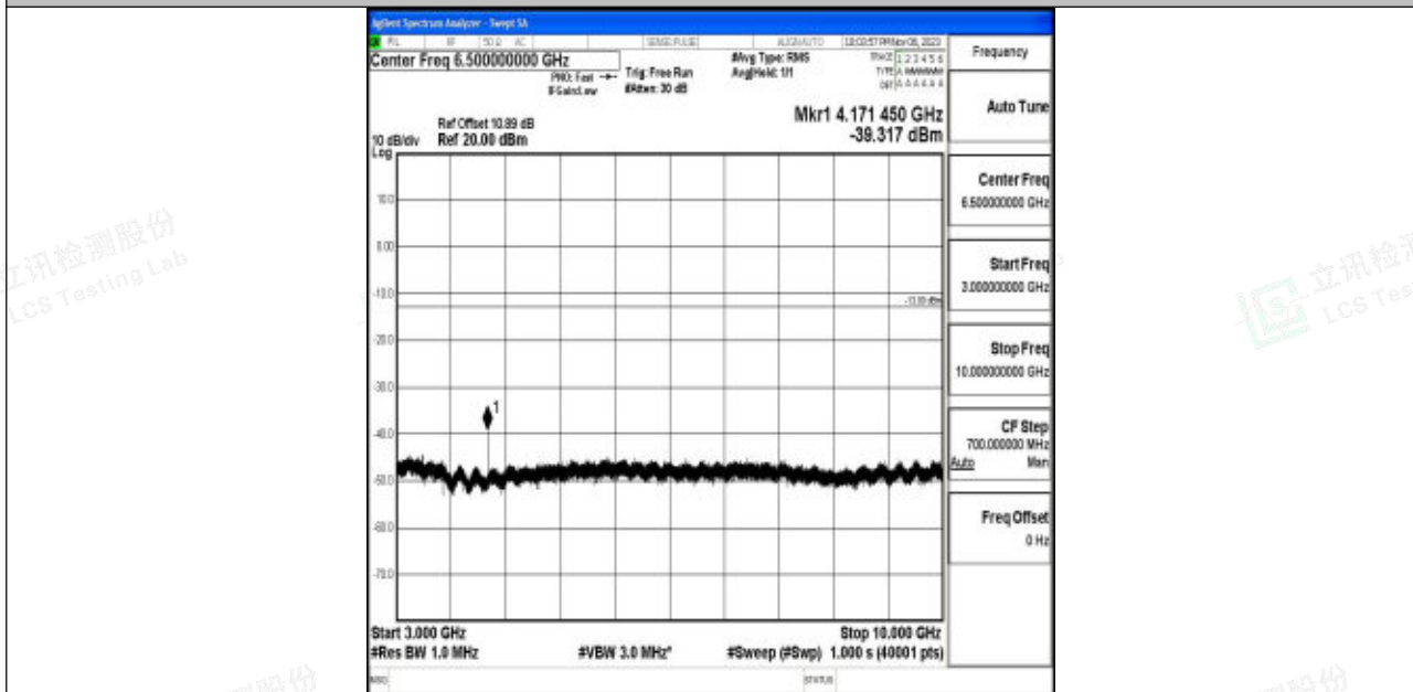
Band5_5MHz_16QAM_20525_1RB#0_3000~10000_3000~10000
