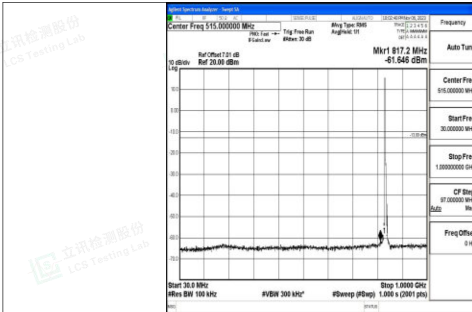
Band5_5MHz_QPSK_20525_1RB#0_30~1000_30~1000
