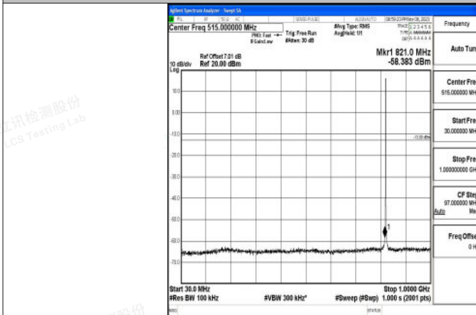
Band5_1.4MHz_64QAM_20407_1RB#0_30~1000_30~1000
