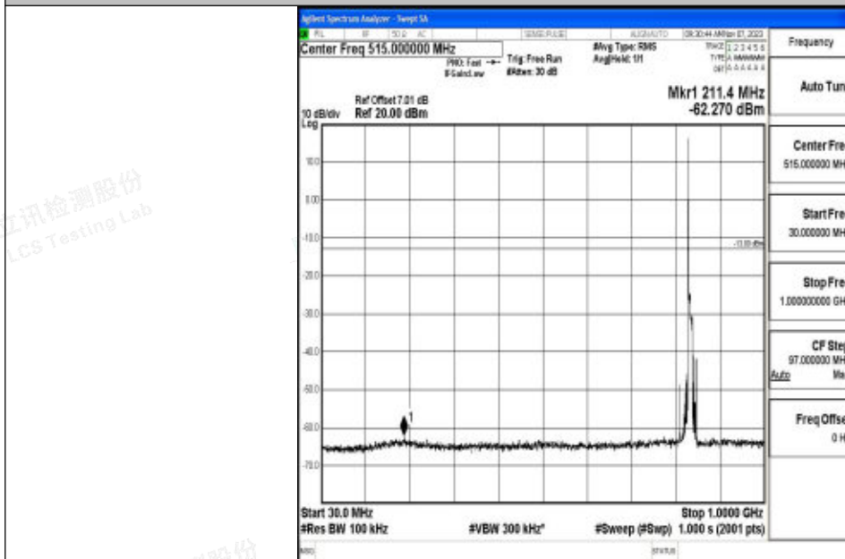
Band5_10MHz_QPSK_20525_1RB#0_30~1000_30~1000
