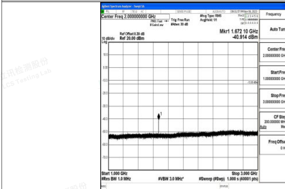
Band5_1.4MHz_64QAM_20525_1RB#0_1000~3000_1000~3000
