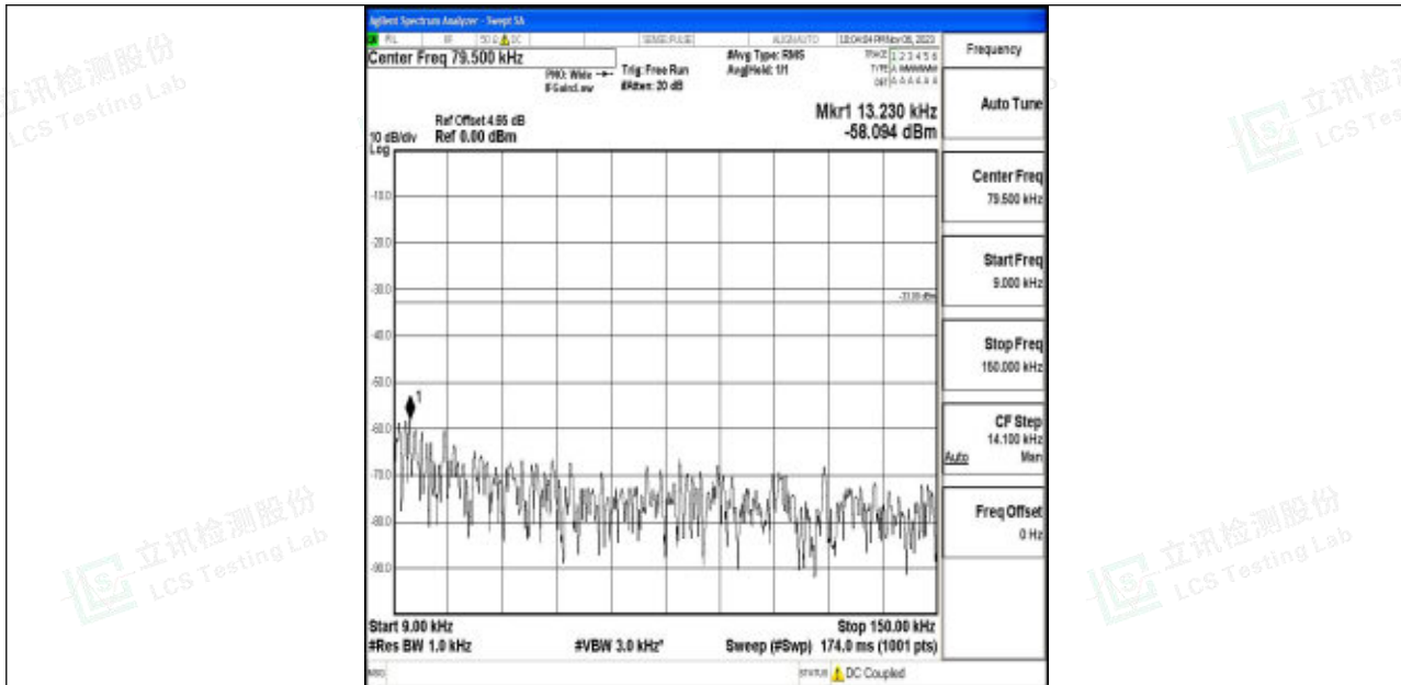
Band5_5MHz_64QAM_20525_1RB#0_0.009~0.15_0.009~0.15
