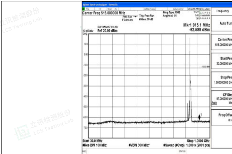
Band5_10MHz_QPSK_20600_1RB#0_30~1000_30~1000
