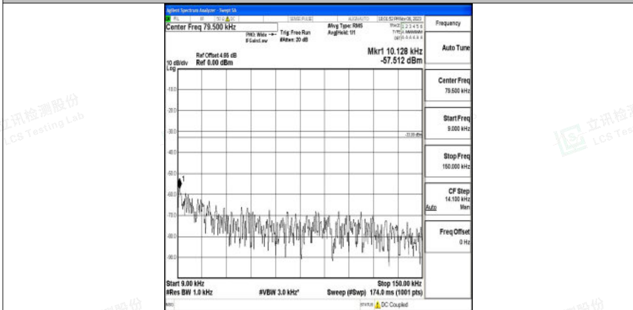
Band5_5MHz_64QAM_20425_1RB#0_0.009~0.15_0.009~0.15
