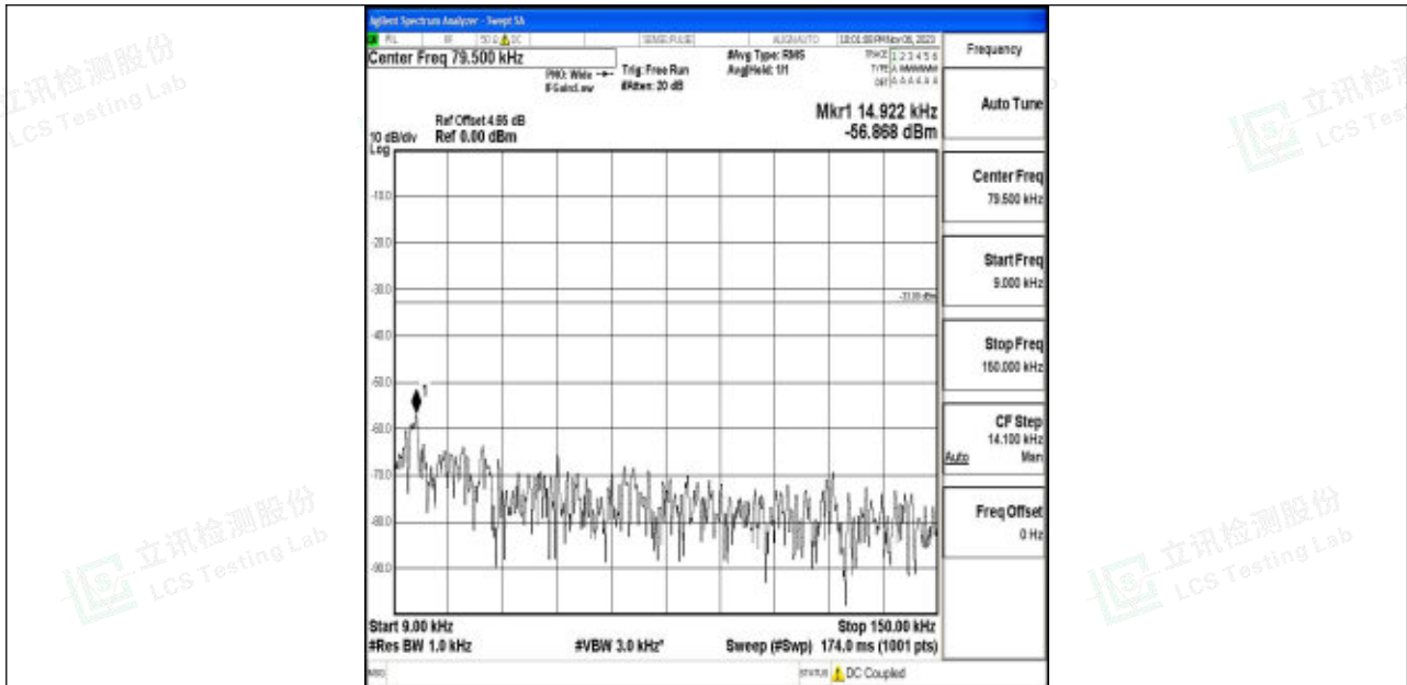
Band5_5MHz_16QAM_20425_1RB#0_0.009~0.15_0.009~0.15
