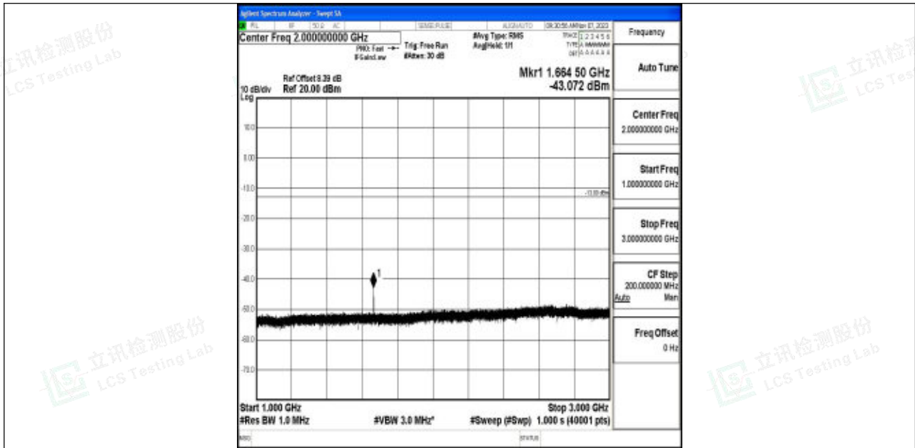
Band5_10MHz_QPSK_20525_1RB#0_1000~3000_1000~3000
