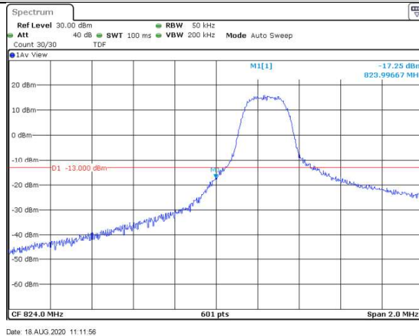
Band5-3MHz-16QAM-20415-15RB#0
