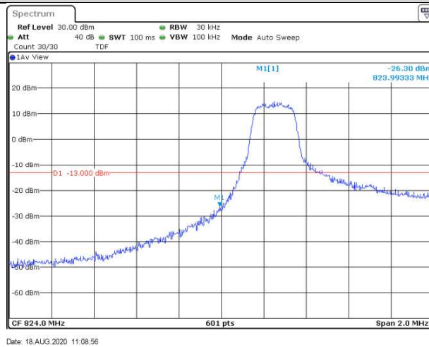
Band5-1.4MHz-16QAM-20407-1RB#5
