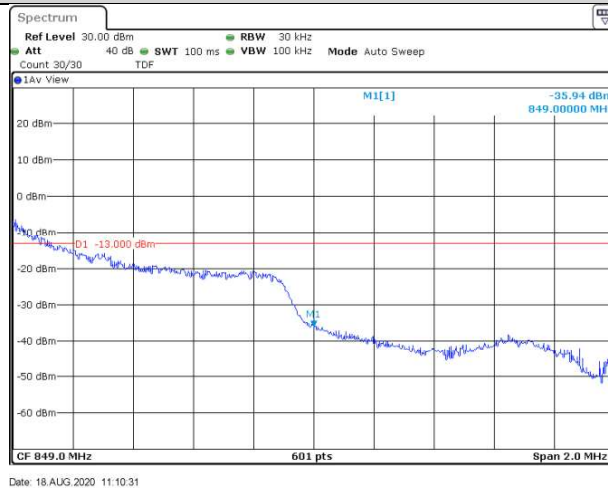
Band5-1.4MHz-16QAM-20643-6RB#0
