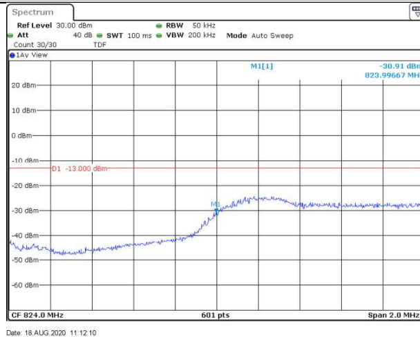
Band5-3MHz-QPSK-20415-15RB#0
