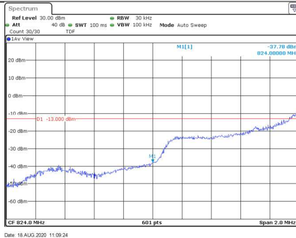
Band5-1.4MHz-16QAM-20407-6RB#0
