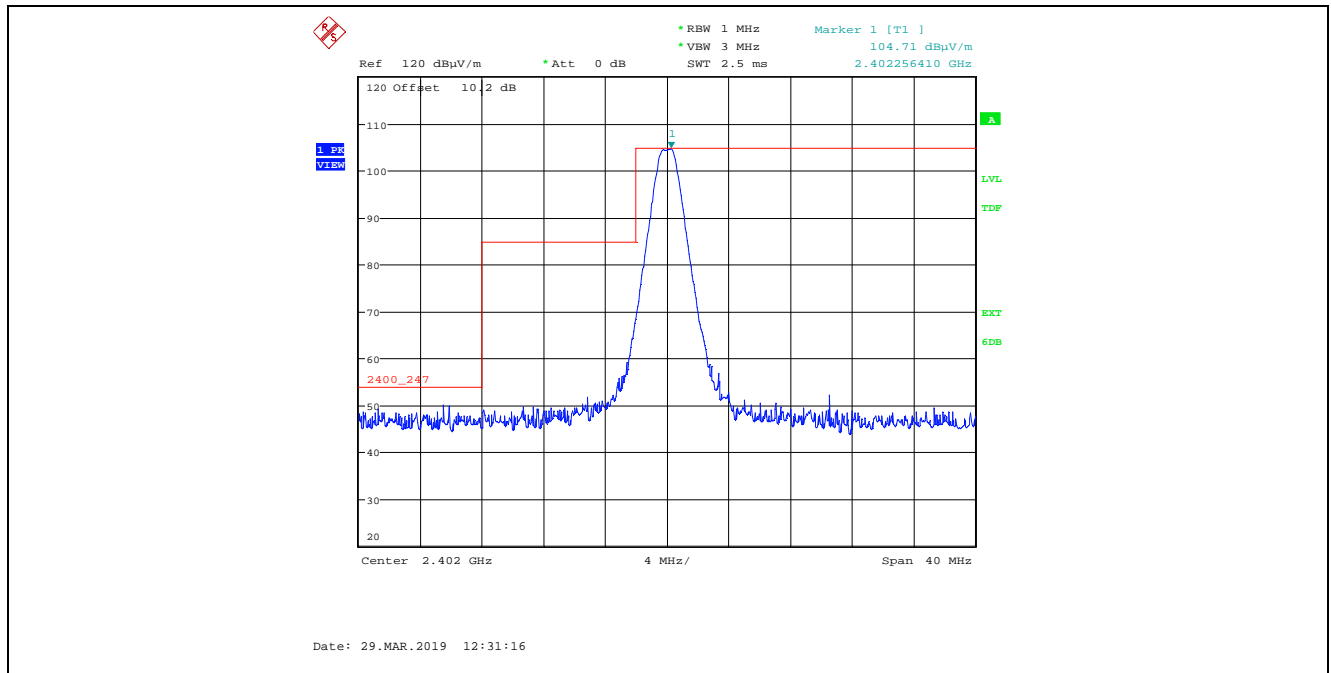
Plot 5.2.4.2.1. Band-Edge Radiated Emissions, Lower Band- edge, Peak Detector Rx Antenna in Vertical Polarization, GFSK Modulation, 1 Mbps, Power Setting 90, Ch 00, 2402 MHz
