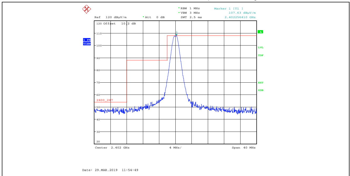
Plot 5.2.4.2.2. Band-Edge Radiated Emissions, Lower Band-edge, Peak Detector Rx Antenna in Horizontal Polarization, GFSK Modulation, 1 Mbps, Power Setting 90, Ch 00, 2402 MHz
