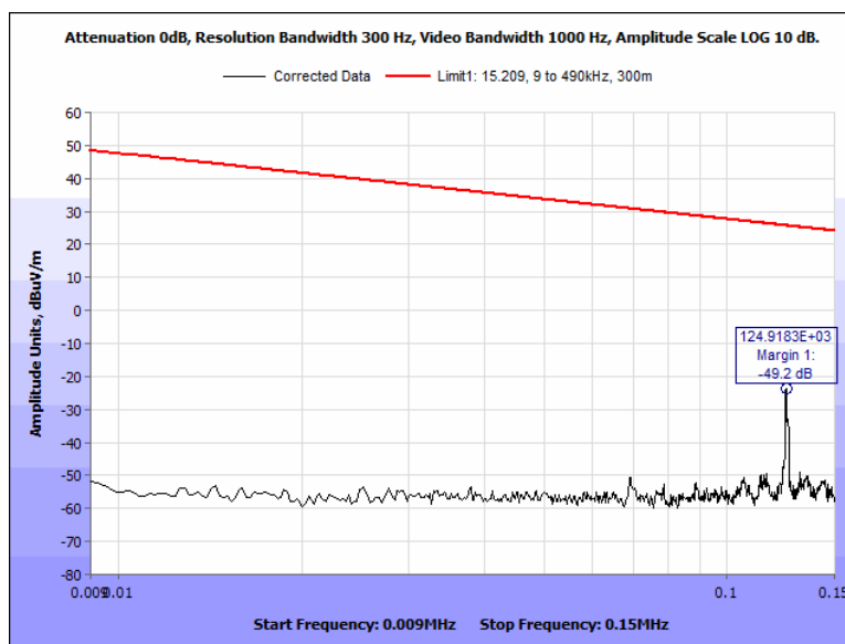
Figure 21. Spurious Emissions, Outside the Bands 13.110 - 14.010 MHz, 0.009 – 0.150 MHz, 0 degrees
