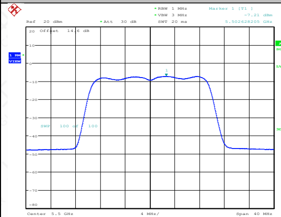
11AX20MIMO-Ant2-5500-PASS
