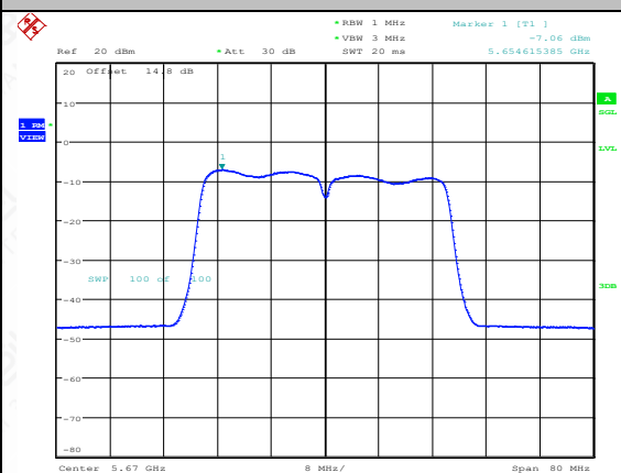
11AC40SISO-Ant2-5670-PASS
