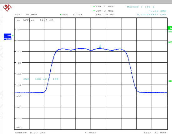
11AX20SISO-Ant1-5320-PASS
