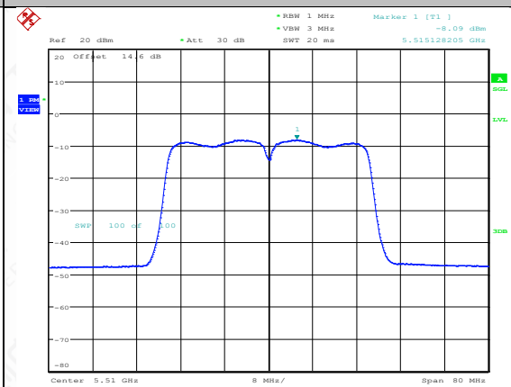
11AC40MIMO-Ant2-5510-PASS
