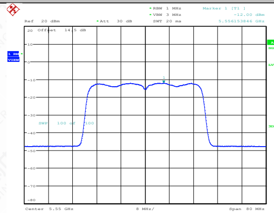
11AX40MIMO-Ant1-5550-PASS
