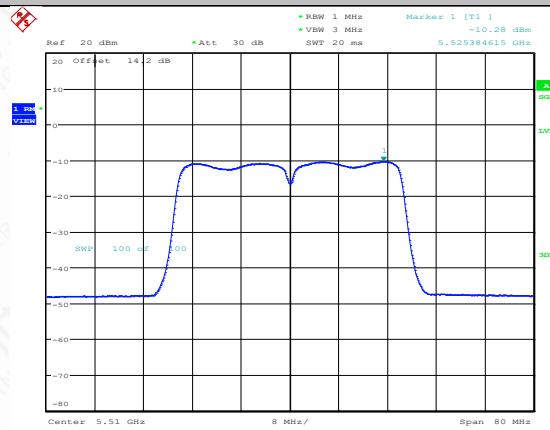
11AC40SISO-Ant1-5510-PASS
