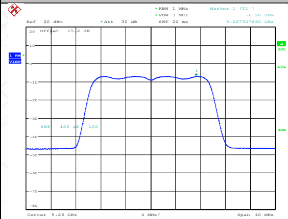
11AX20SISO-Ant2-5260-PASS
