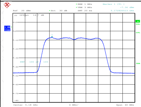
11AX20MIMO-Ant2-5180-PASS
