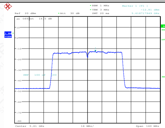
11AC80MIMO-Ant1-5610-PASS
