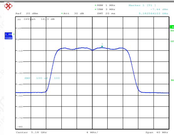
11AX20MIMO-Ant1-5180-PASS
