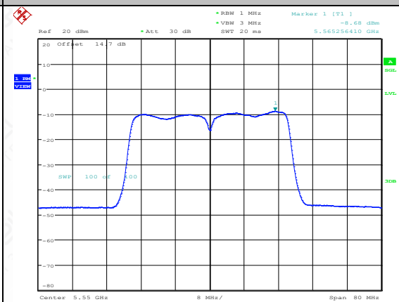
11AC40MIMO-Ant2-5550-PASS
