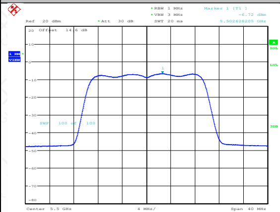
11AX20SISO-Ant2-5500-PASS
