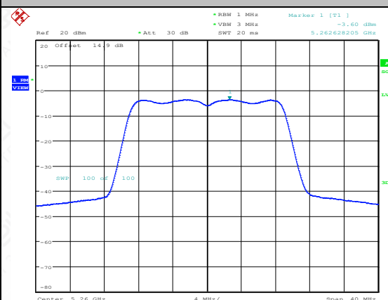
11AC20SISO-Ant2-5260-PASS
