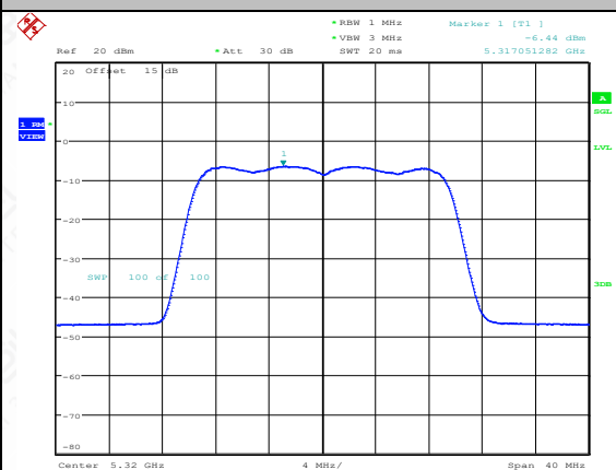
11AX20SISO-Ant2-5320-PASS
