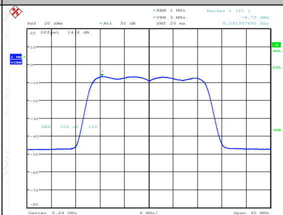
11AX20SISO-Ant2-5240-PASS
