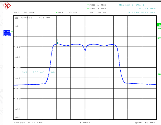
11N40MIMO-Ant1-5270-PASS
