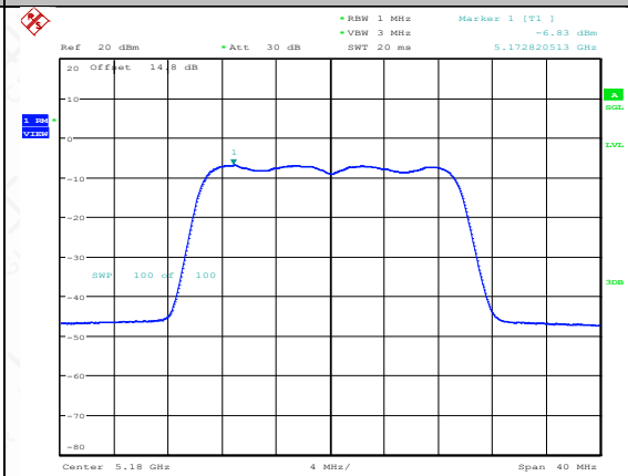
11AX20SISO-Ant2-5180-PASS
