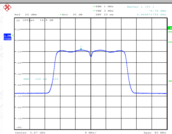
11AC40SISO-Ant1-5670-PASS
