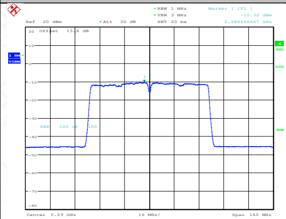
11AC80MIMO-Ant2-5290-PASS
