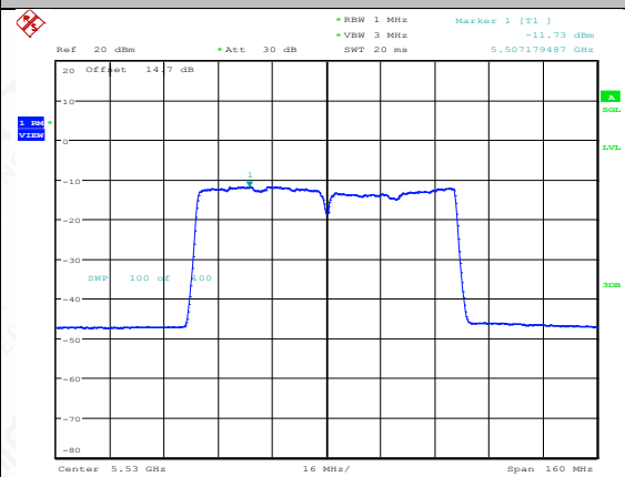
11AC80MIMO-Ant2-5530-PASS
