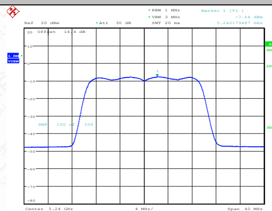
11AX20MIMO-Ant1-5240-PASS
