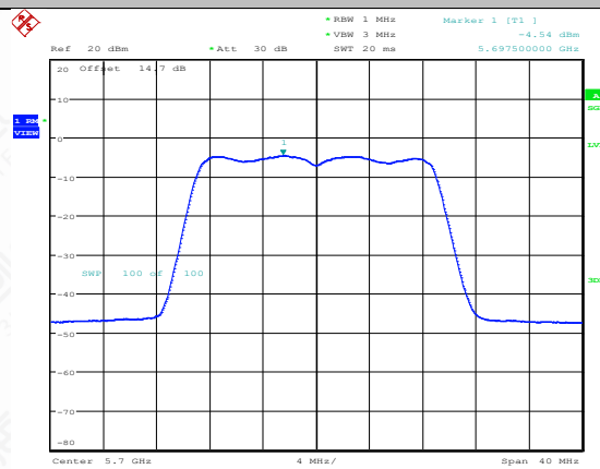
11AC20MIMO-Ant1-5700-PASS
