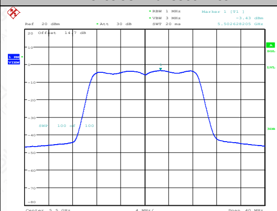
11AC20SISO-Ant2-5500-PASS
