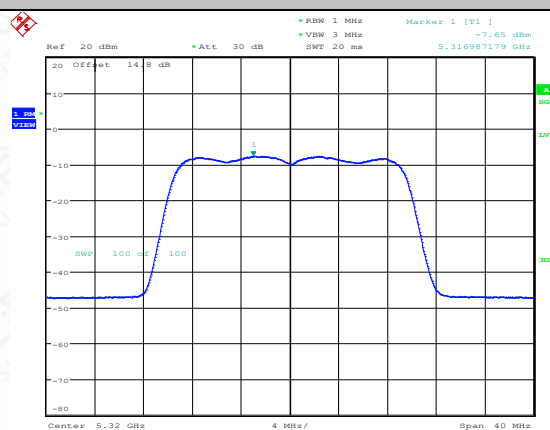
11AX20MIMO-Ant1-5320-PASS
