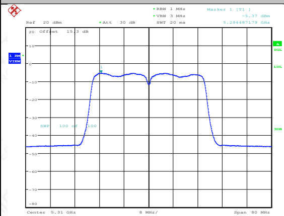
11N40MIMO-Ant2-5310-PASS
