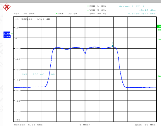
11N40MIMO-Ant1-5510-PASS
