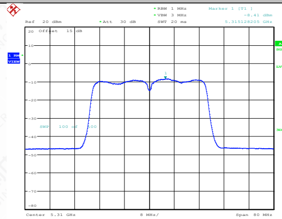
11AC40MIMO-Ant1-5310-PASS
