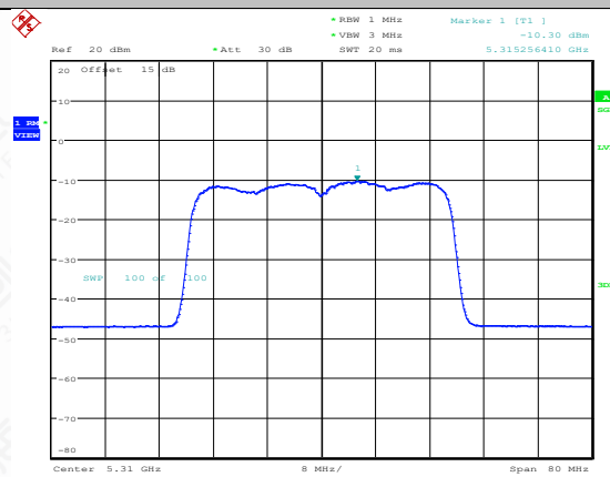
11AX40MIMO-Ant1-5310-PASS
