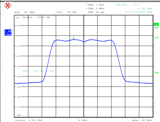
11AC20MIMO-Ant2-5580-PASS
