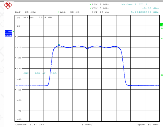
11AX40SISO-Ant2-5310-PASS
