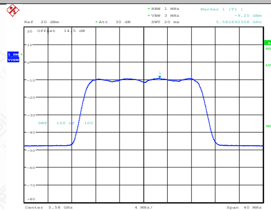
11AX20MIMO-Ant1-5580-PASS
