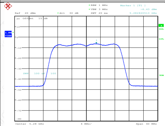
11AX20MIMO-Ant2-5280-PASS
