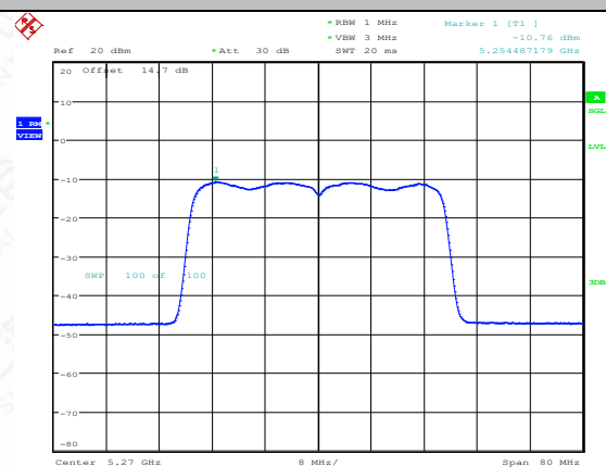
11AX40SISO-Ant1-5270-PASS
