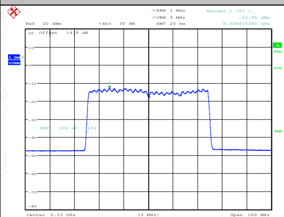
11AX80MIMO-Ant2-5530-PASS
