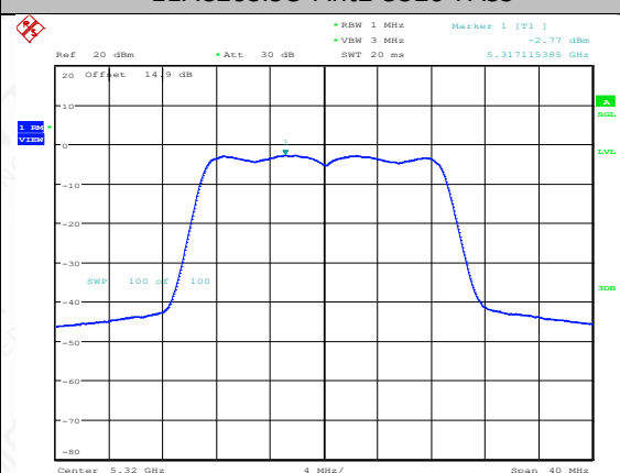
11AC20SISO-Ant2-5320-PASS
