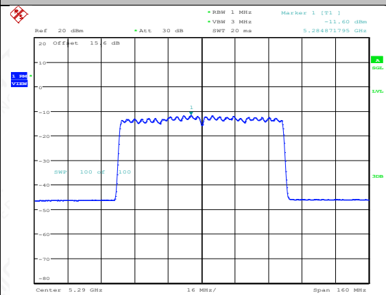
11AX80MIMO-Ant2-5290-PASS
