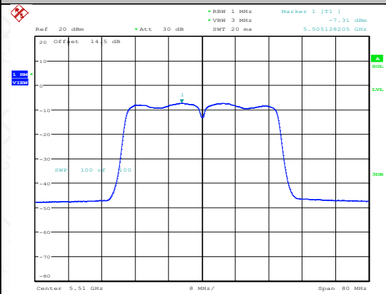
11AC40SISO-Ant2-5510-PASS
