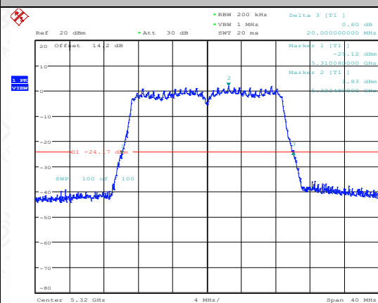
11N20MIMO-Ant2-5320
