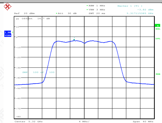
11AC20MIMO-Ant1-5320-PASS
