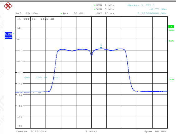
11AC40SISO-Ant1-5230-PASS
