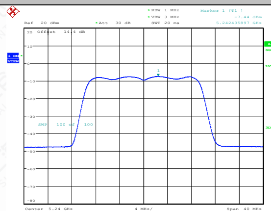
11AX20SISO-Ant1-5240-PASS
