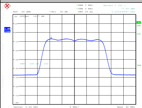
11AX20MIMO-Ant2-5240-PASS
