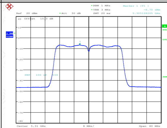
11AC40SISO-Ant2-5310-PASS
