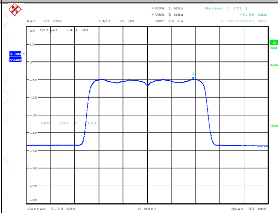
11AX40SISO-Ant2-5190-PASS
