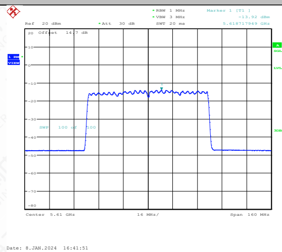
11AX80MIMO-Ant1-5610-PASS
