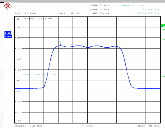
11AX20SISO-Ant1-5200-PASS
