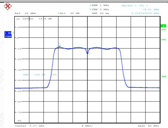
11AC40SISO-Ant1-5270-PASS
