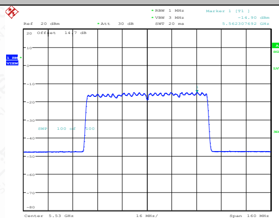
11AX80MIMO-Ant1-5530-PASS
