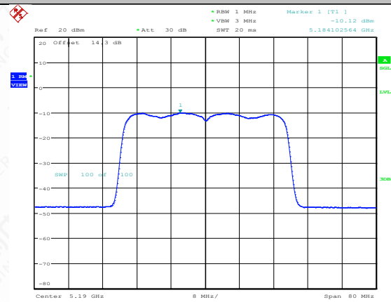
11AX40SISO-Ant1-5190-PASS
