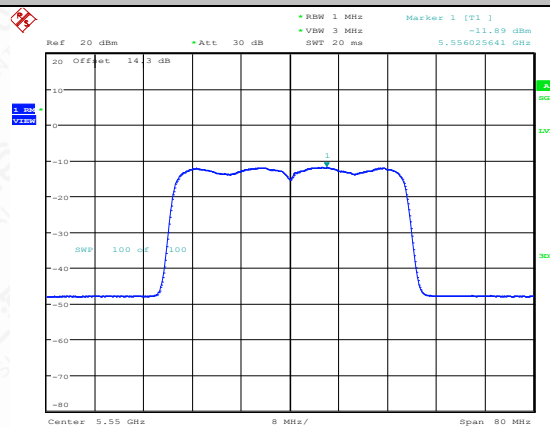
11AX40SISO-Ant1-5550-PASS
