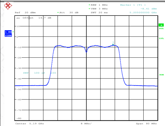
11AC40MIMO-Ant2-5190-PASS
