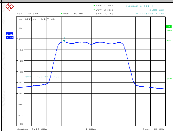
11AC20SISO-Ant2-5180-PASS
