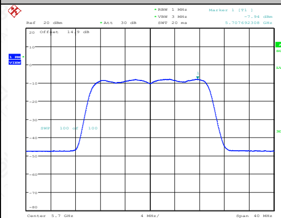
11AX20MIMO-Ant2-5700-PASS
