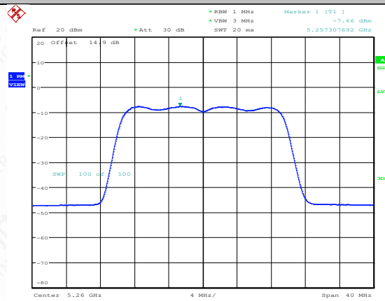
11AX20SISO-Ant1-5260-PASS
