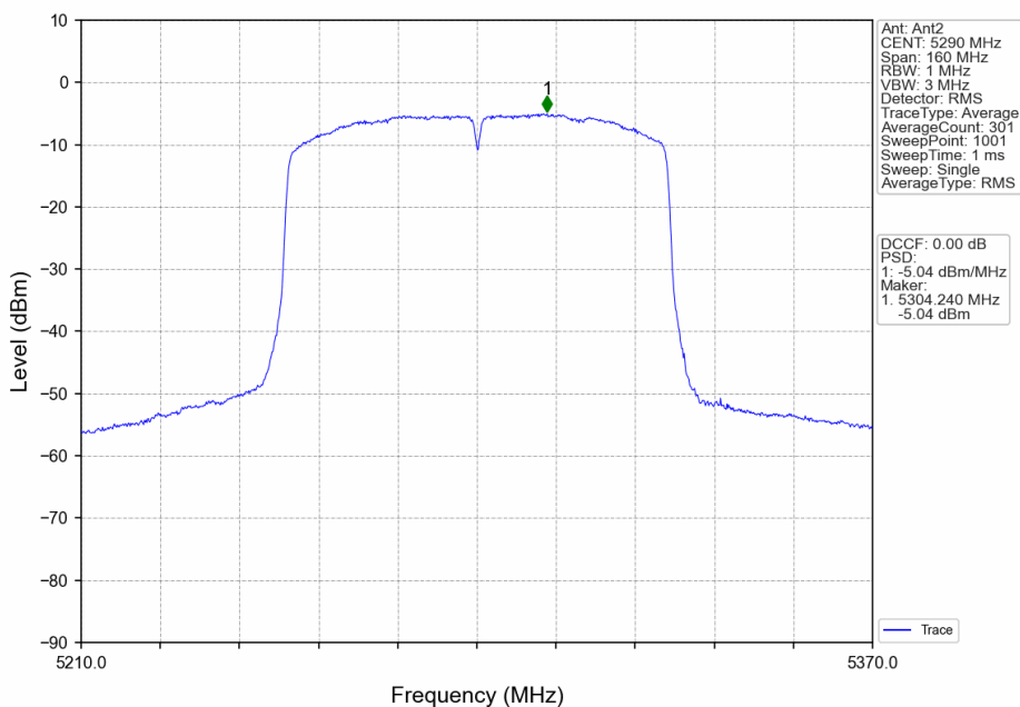
802.11ac(VHT80)_MCH_5290MHz_MIMO_NTNV
