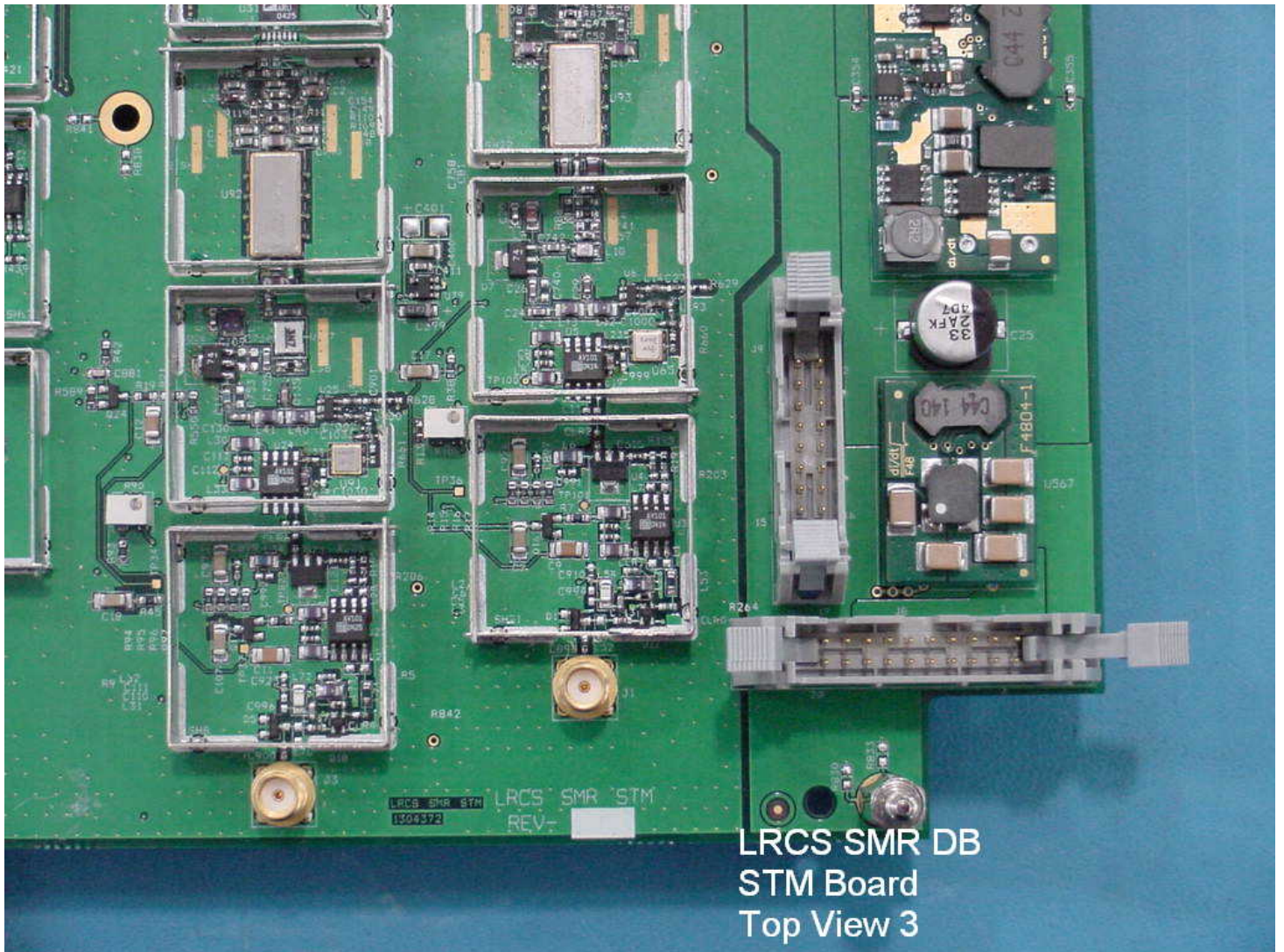
Digivance Street Coverage Solution (SCS) (labeled as SMR DB in photo) STM Board Top View - Lower Right
